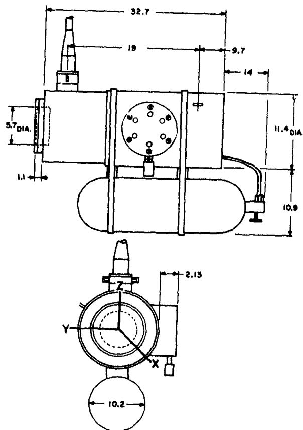
Fig. W2. Dimensions (in centimeters) and orientation of type J9S transducer.
