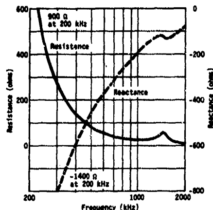
Fig. B3. Typical equivalent series impedance, type E8 transducer with 2.4 m of RG-62/U coaxial cable.
