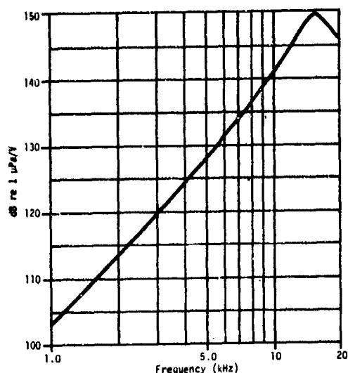
Fig. I3. Typical transmitting voltage response, type F40 transducer, unbalanced, black lead and shield grounded, 30-m cable.
