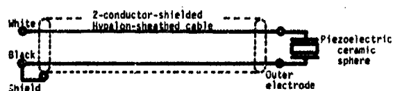
Fig. I2. Wiring diagram, type F40 transducer.
