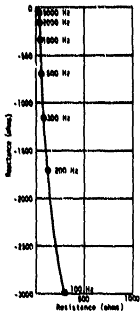
Fig. 06. (Left) Typical impedance of type G34 transducer under free-field conditions in water.
