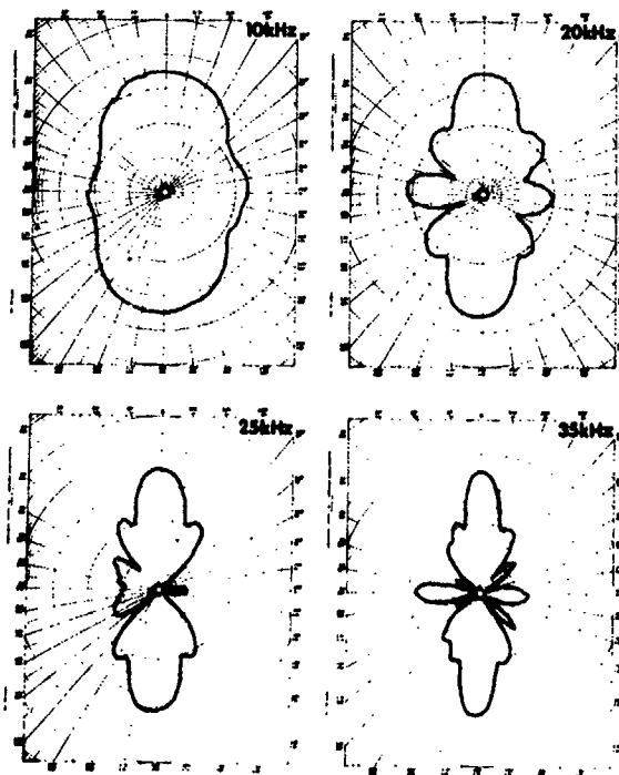
Fig. H4. Typical directivity patterns in the vertical (XZ) plane, type F37 transducer. Scale: center to top of grid, each pattern, equals 50 dB.
