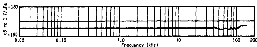
Fig. T3. Typical free-field voltage sensitivity, type H52 hydrophone; open-circuit voltage at end of 23-m cable.
