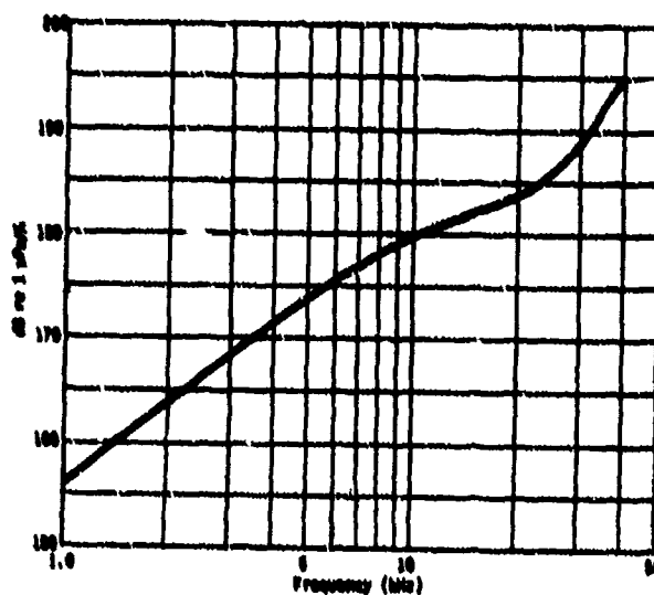
Fig. D2. Typical transmitting current response, type F27 transducer.
