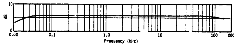
Fig. S2. Typical coupling loss, transistorized preamplifier of type H23 hydrophone (ratio in decibels of open-circuit voltage at preamplifier output to open-circuit crystal voltage).
