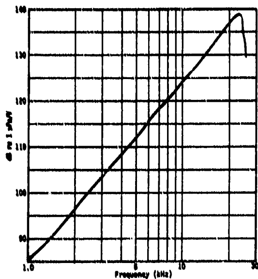
Fig. G3. Typical transmitting voltage response, type F36 transducer.
