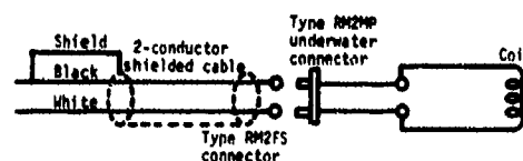
Fig. BB2. (Right) Cable connections for type J15-1 transducer; d-c resistance between white and black leads: 25 \Omega (approx).
