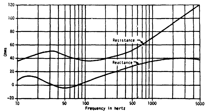
Fig. CC4. Typical impedance, each driver assembly, type J15-3 transducer.
