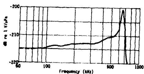
Fig. C3. Typical free-field voltage sensitivity, type E27 transducer.
