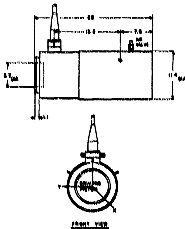
Fig. V5. Dimensions (in centimeters) and orientation of type J9 transducer.
