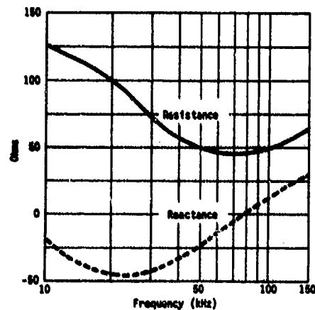
Fig. E5. Typical equivalent series impedance, type F30 transducer.
