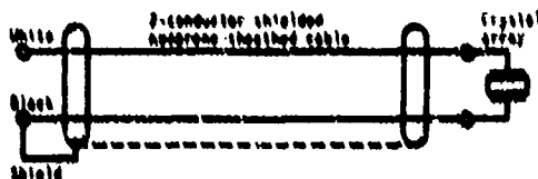
Fig. K2. Schematic circuit diagram, type F41 transducer.
