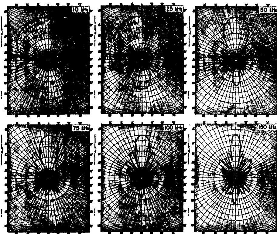
Fig. E6b. Typical directivity patterns in the XZ (vertical) plane, type F30 transducer. Scale: Center to top of grid, each patterns, equals 50 dB.
