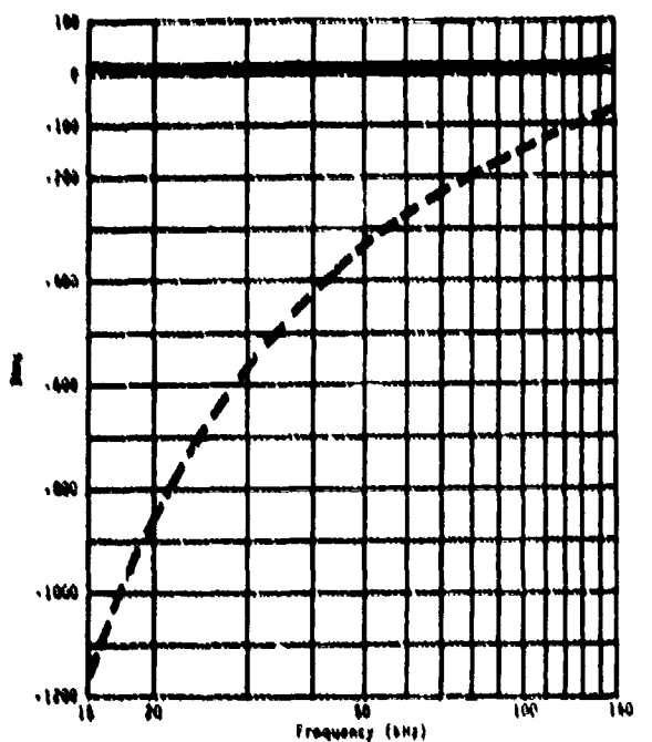
Fig. K5. Typical equivalent series impedance, type F41 transducer.
