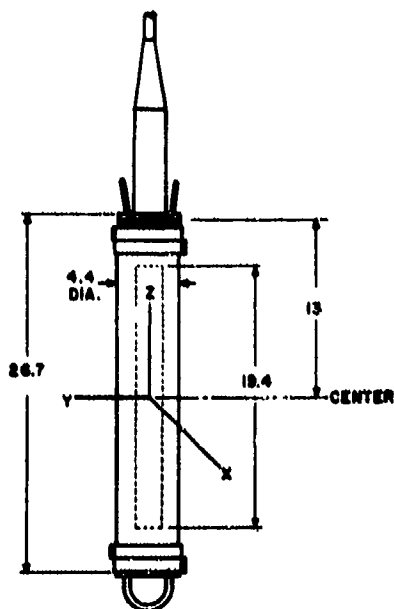
Fig. G5. (Left) Dimensions in centimeters) and orientation of type F36 transducer.
