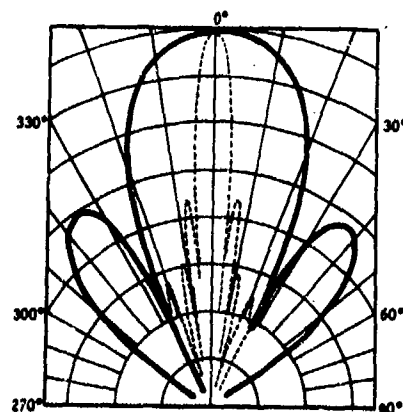
Fig. B6. Directivity, type E8 transducer, in planes that include the X axis. Scale, center to top of grid, equals 40 dB.
