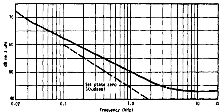
Fig. T4. Typical equivalent noise pressure, type H52 hydrophone.
