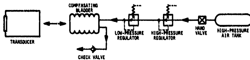
Fig. AA3. Gas flow in the system.
