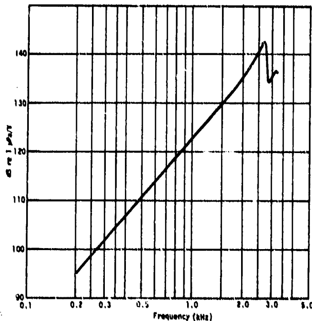
Fig. 03. (Left) Typical transmitting voltage response, type G34 transducer, unbalanced, black lead and shield grounded, 76-m cable. Serials 10 and higher operate satisfactorily above 3 kHz.
