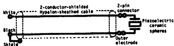
Fig. J2. (Above) Wiring diagram, type F40A transducer.
