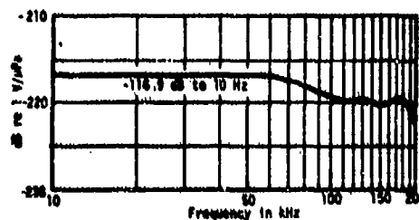
Fig. A3. Typical free-field voltage sensitivity, type A42 hydrophone; open-circuit voltage at output of preamplifier.
