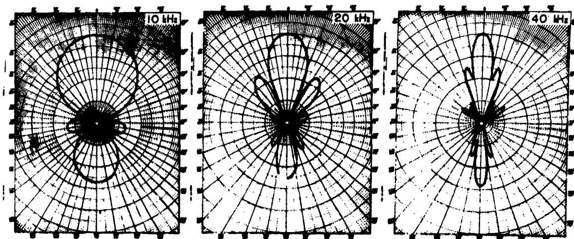
Fig. F5. Typical directivity patterns in the horizontal (XY) plane, type F33 transducer, both sections in parallel. Scale: Center to top of grid, each pattern, equals 50 dB.
