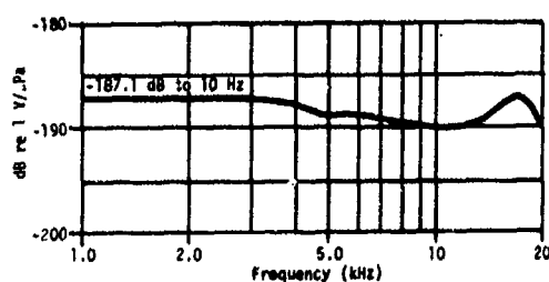
Fig. I5. Typical free-field voltage sensitivity, type F40 transducer; open-circuit voltage at end of 30-m cable; unbalanced, black lead and shield grounded.
