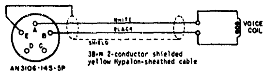
Fig. X2. (Left) Cable connections for type J11 transducer.
