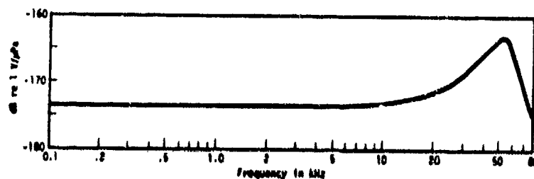
Fig. U3. Typical free-field voltage sensitivity, type H56 hydrophone, 3:1-area-ratio capped-tube model; open-circuit crystal voltage at the end of a 23-m cable.
