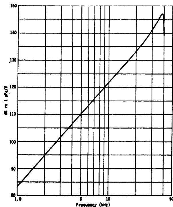
Fig. H3. Typical transmitting voltage response, type F37 transducer.
