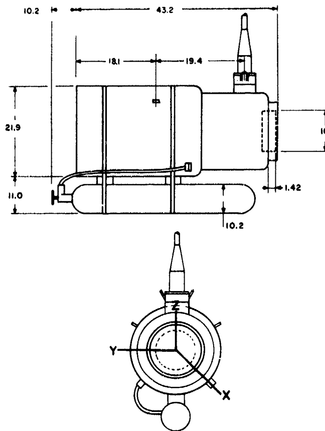
Fig. Y2. Dimensions (in centimeters) and orientation of type J11S transducer.
