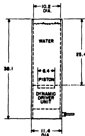
Fig. N2. Dimensions (in centimeters), type G19 calibrator.
