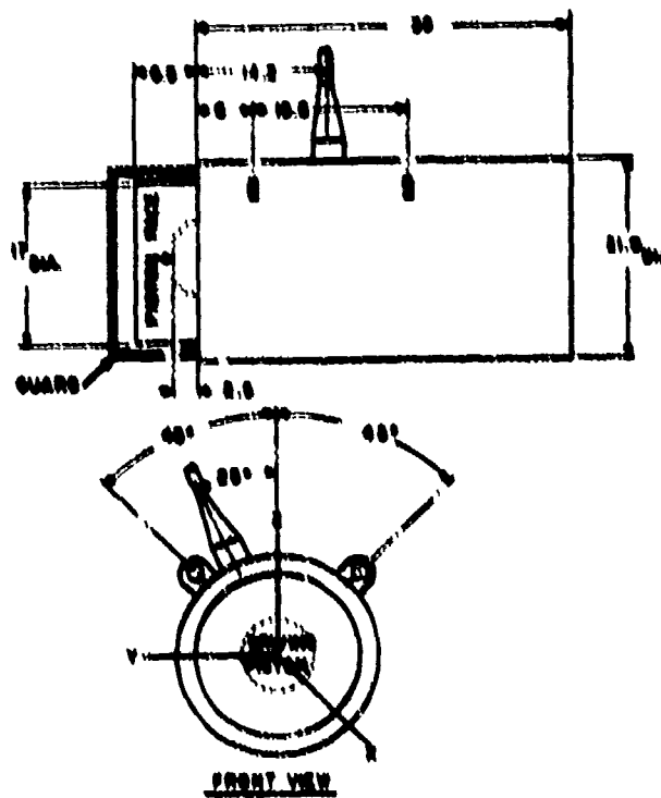
Fig. 25. Dimensions (in centimeters) and orientation of type J13 transducer.
