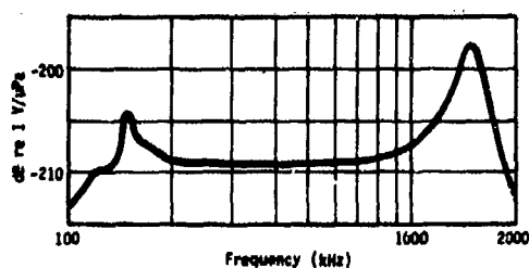
Fig. B5. Typical free-field voltage sensitivity, type E8 transducer with 2.4-m cable.
