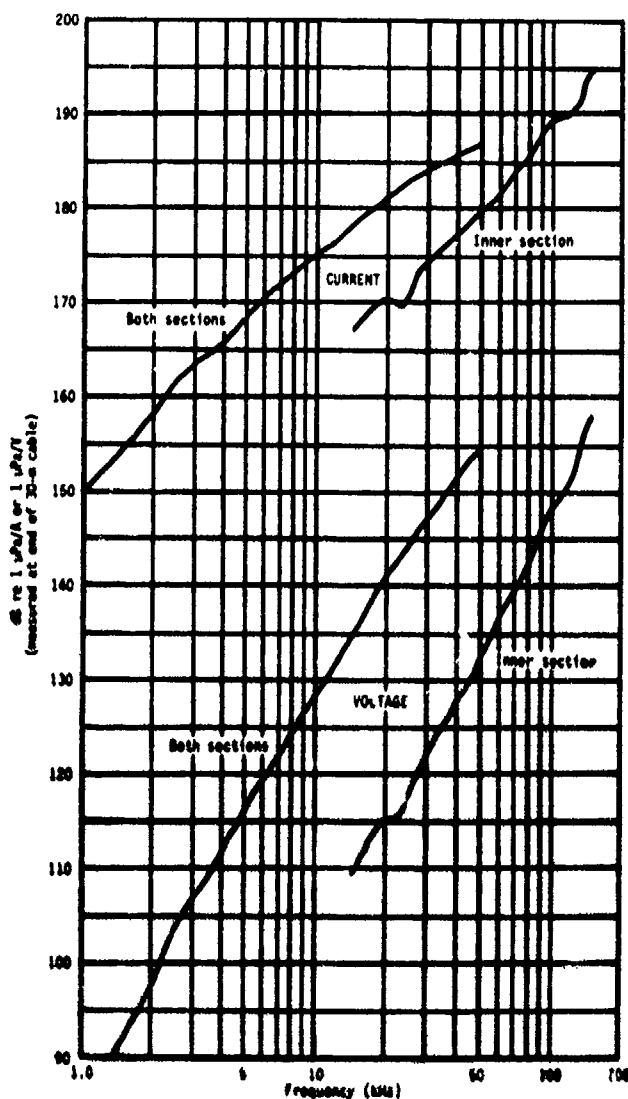
Fig. F3. (Left) Transmitting current and voltage responses, type F33 transducer.
