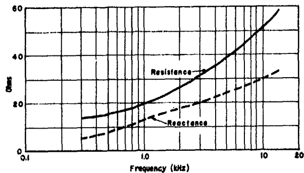
Fig. X4. (Right) Typical impedance, type J11 transducer.
