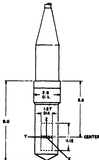
Fig. M6. (Right) Dimensions (in centimeters) and orientation of type F50 transducer.
