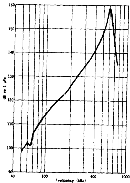
Fig. C4. Typical transmitting voltage response, type E27 transducer.
