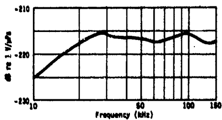
Fig. E4. Typical free-field voltage sensitivity, type F30 transducer.
