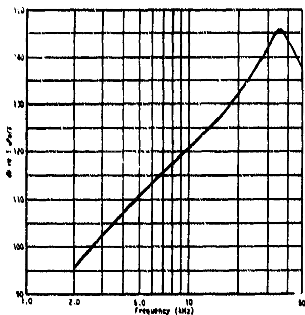
Fig. L3. Typical transmitting voltage response, type F42 transducer, unbalanced, black lead and shield grounded, 16-m cable.
