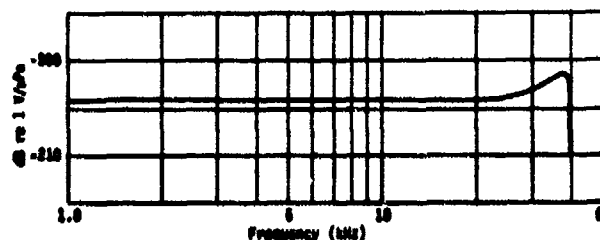
Fig. H2. Typical free-field voltage sensitivity, type F37 transducer.
