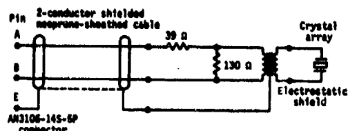
Fig. E2. Schematic circuit diagram, type F30 transducer.
