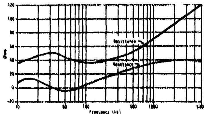
Fig. 24. Typical impedance, type J13 transducer.
