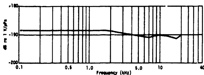
Fig. J4. (Right) Typical free-field voltage sensitivity, type F40A transducer; open-circuit voltage at end of 30-m cable; unbalanced, black lead and shield grounded.
