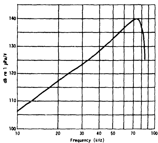
Fig. M3. (Left) Typical transmitting voltage response, type F50 transducer.
