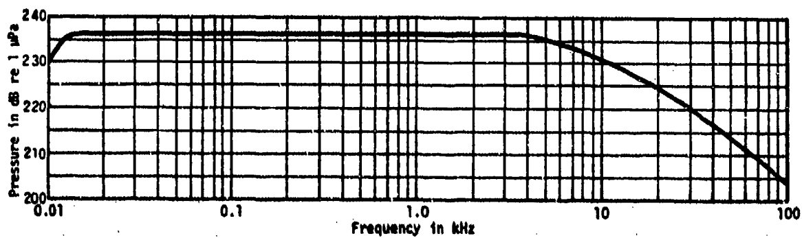
Fig. A5. Typical hydrophone pressure overload level for 1% distortion in output voltage, type A42 hydrophone.
