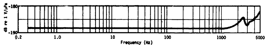
Fig. P4. Typical free-field voltage sensitivity, type H11 hydrophon, in terms of open-circuit voltage at end of 12-m cable.
