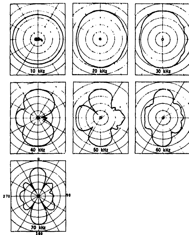
Fig. M5. (Left) Typical directivity patterns in the vertical (XZ) plane, type F50 transducer. Scale: center to top of grid, each pattern, equals 50 dB.
