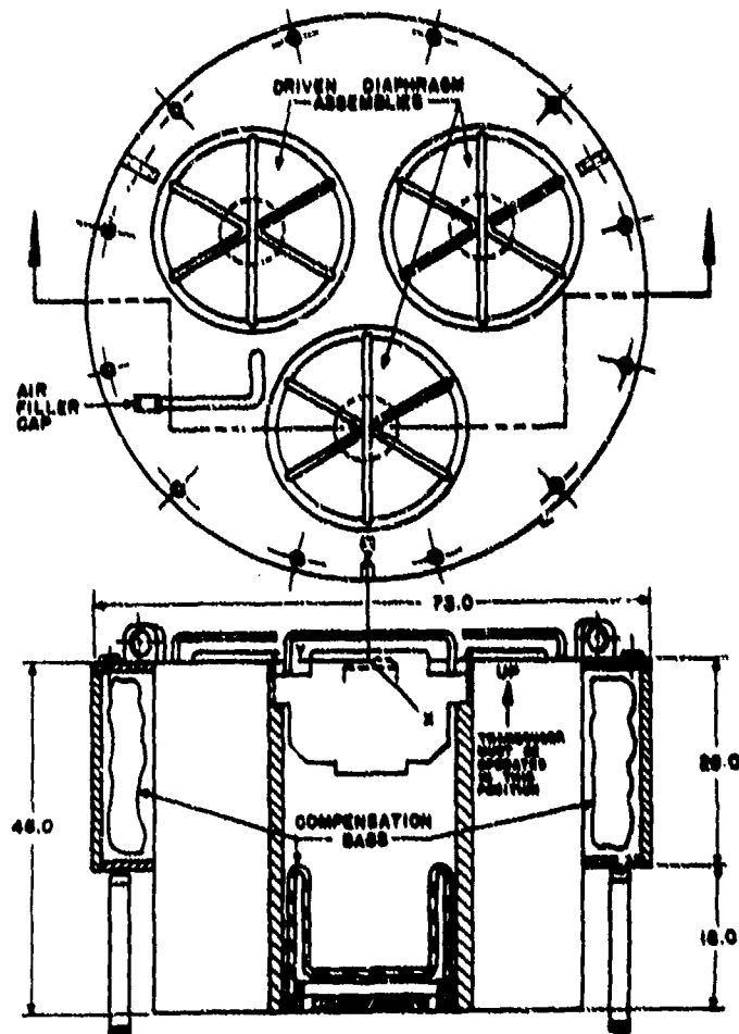
Fig. CC6. Dimensions (in centimeters) and orientation of type J15-3 transducer.
