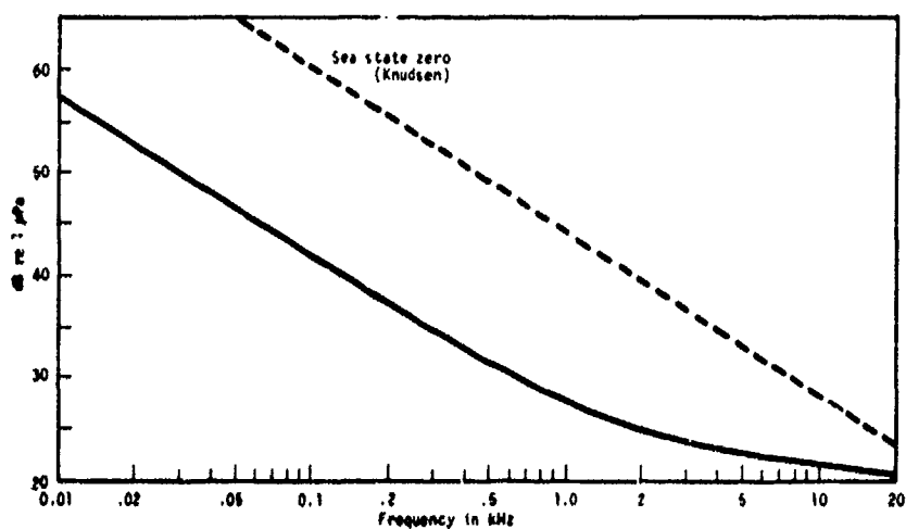
Fig. U5. Equivalent noise spectrum of type H56 hydrophone (computed from noise voltage measured at the end of a 12-m cable).
