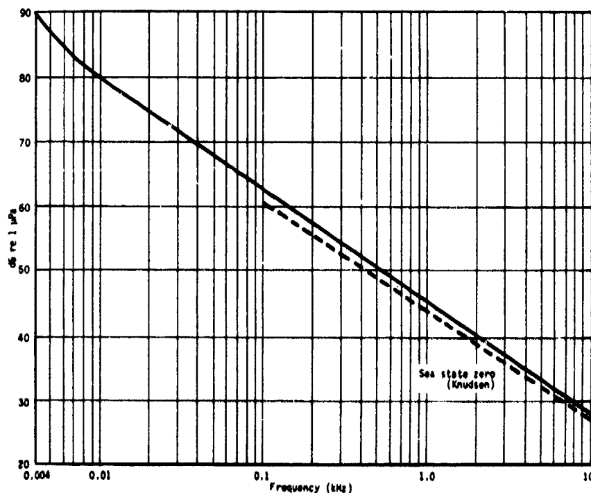
Fig. P5. (Above) Typical equivalent noise pressure computed from noise voltage at end of cable, type H11 hydrophone.
