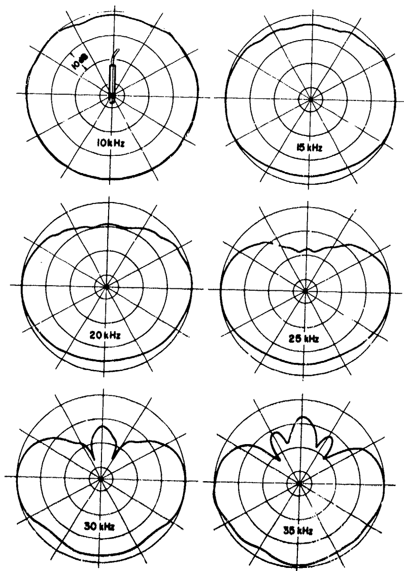
Fig. U6. Directivity patterns in the vertical (XZ) plane of type H56 hydrophone, 3:1-area-ratio capped-tube model.
