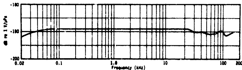
Fig. S4. Typical free-field voltage sensitivity, type H23 hydrophone (open-circuit voltage at end of 23-m cable).
