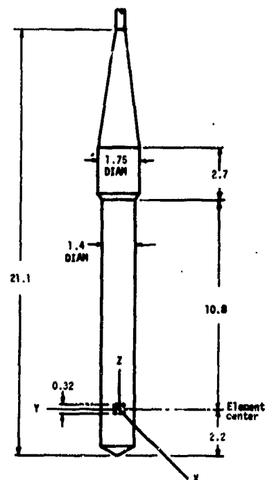
Fig. A7. Dimensions (in centimeters) and orientation of USRD type A42 hydrophone.
