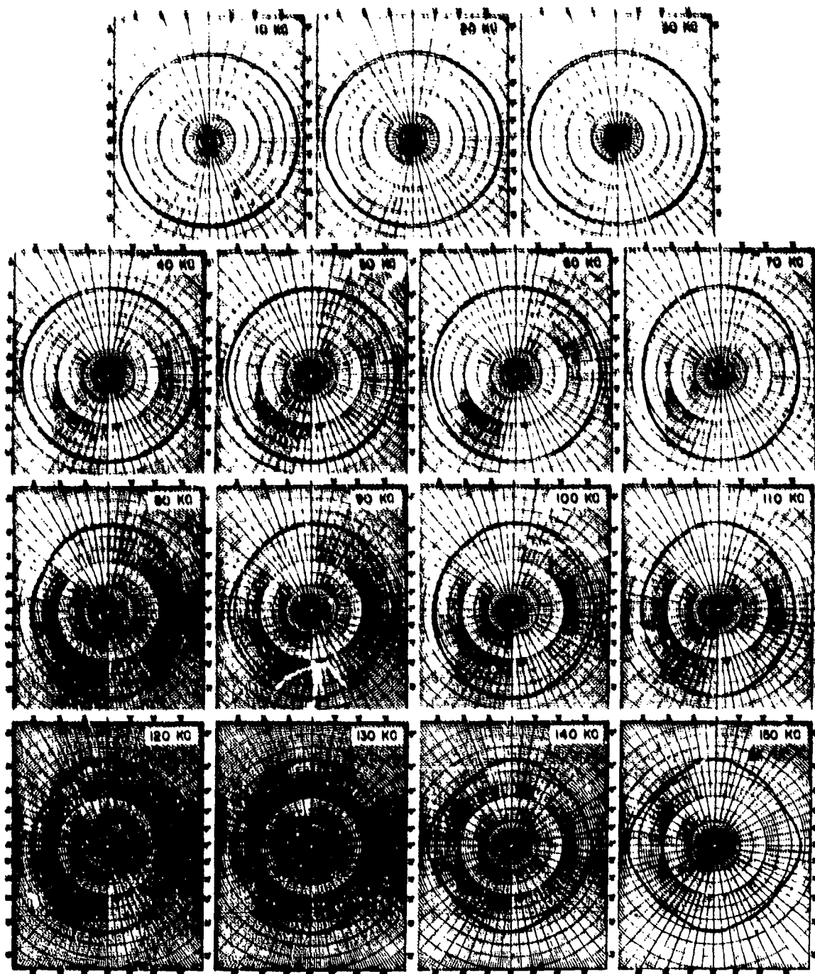
Fig. Q6. Typical directivity patterns in the XY plane, type H17 hydrophone. Scale: Center to top of grid, each pattern, equals 50 dB.
