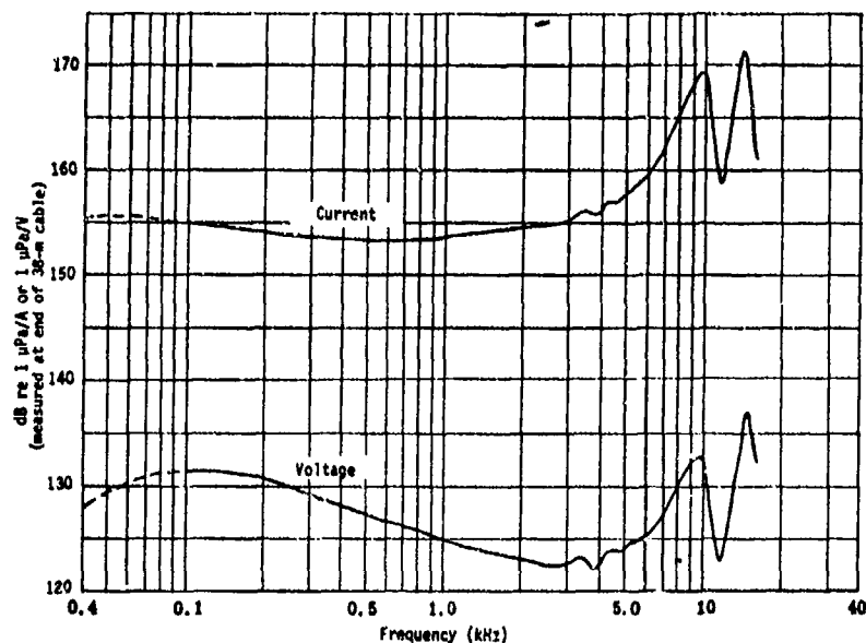
Fig. X3. Typical transmitting current and voltage responses, type J11 transducer. Response below 0.1 kHz is a function of depth.
