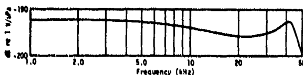
Fig. L5. Typical free-field voltage sensitivity, type F42 transducer, open-circuit voltage at end of 11-m cable; unbalanced, black lead and shield grounded.
