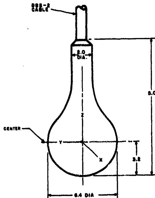
Fig. L6. (Right) Dimensions (in centimeters) and orientation, type F42 transducer.
