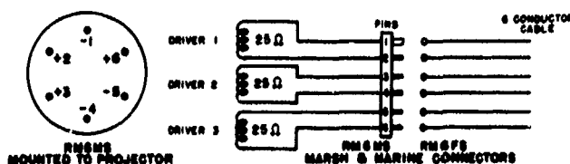
Fig. CC2. (Right) Cable connections, type J15-3 transducer.
