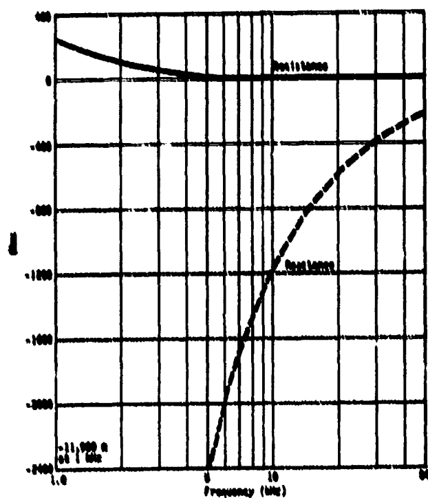
Fig. D4. Typical equivalent series impedance, type F27 transducer.
