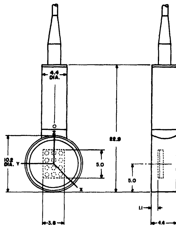
Fig. K7. Dimensions (in centimeters) and orientation of type F41 transducer.
