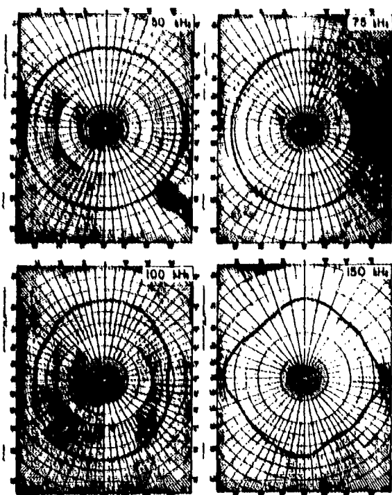
Fig. S6. (Right) Typical directivity patterns in the horizontal (XY) plane, type H23 hydrophone. Scale: center to top of grid, each pattern, equals 50 dB.
