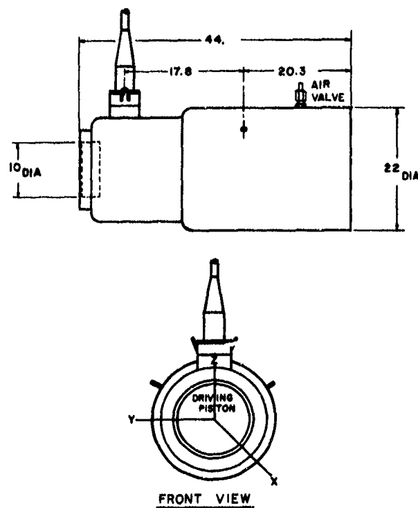
Fig. X5. Dimensions (in centimeters) and orientation of type J11 transducer.
