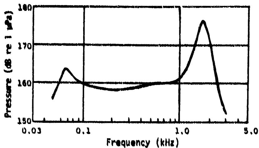
Fig. N6. Typical sound pressure in type G19 calibrator as measured by a constant-sensitivity hydrophone for a 5-V input to calibrator.
