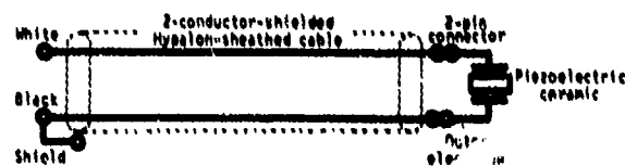
Fig. 02. (Right) Wiring diagram, type G34 transducer.
