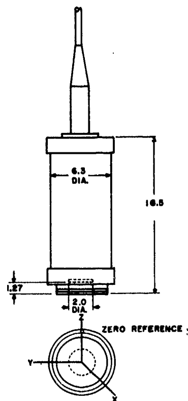
Fig. B7. Dimensions (in centimeters) and orientation of type E8 transducer.
