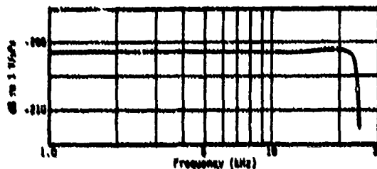
Fig. G2. Typical free-field voltage sensitivity, type F36 transducer.
