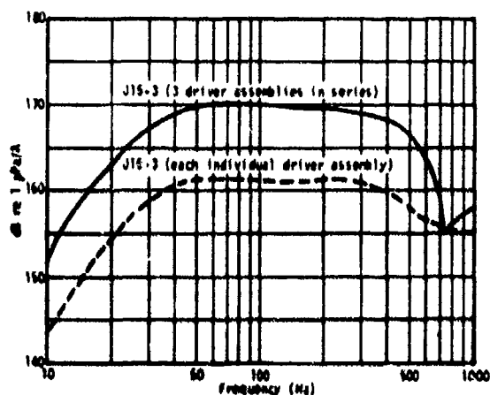
Fig. CC3. (Right) Typical transmitting current response, type J15-3 transducer.
