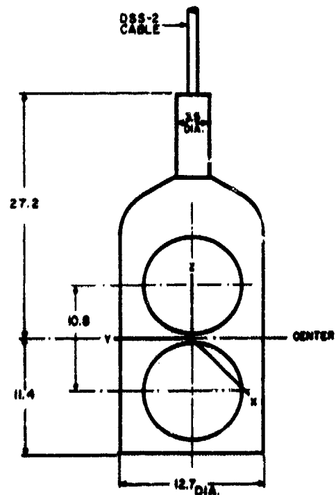
Fig. J7. (Right) Dimensions (in centimeters) and orientation, type F40A transducer.
