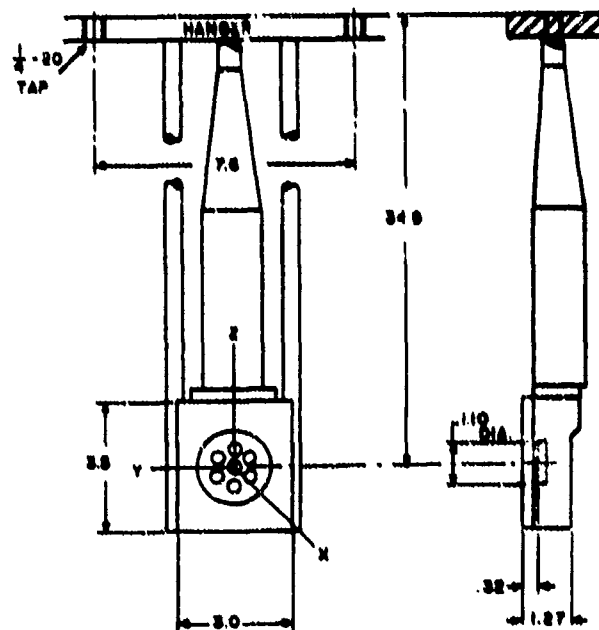
Fig. C6. Dimensions (in centimeters) and orientation of type E27 transducer (tap: UNC).
