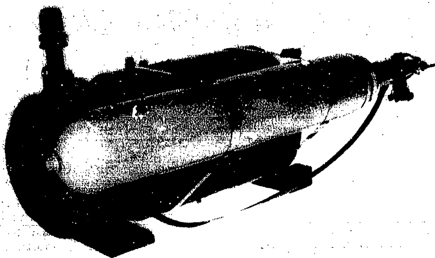
Fig Y1. USRD type J11S transducer.
