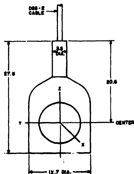
Fig. I6. Dimensions (in centimeters) and orientation of type F40 transducer.
