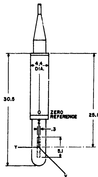
Fig. S8. (Right) Dimensions (in centimeters) and orientation of type H23 hydrophone.
