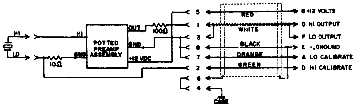
Fig. S3. Wiring diagram, type H23 hydrophone.
