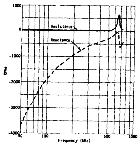
Fig. C2. Typical equivalent series impedance, type E27 transducer.
