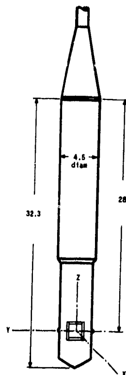
Fig. U7. Dimensions (in centimeters) and orientation of type H56 hydrophone.
