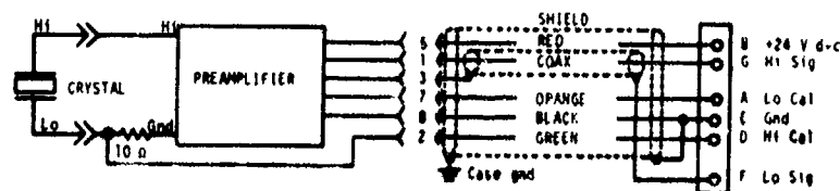
Fig. U2. Wiring diagram of circuitry associated with the integral preamplifier of type H56 hydrophone.
