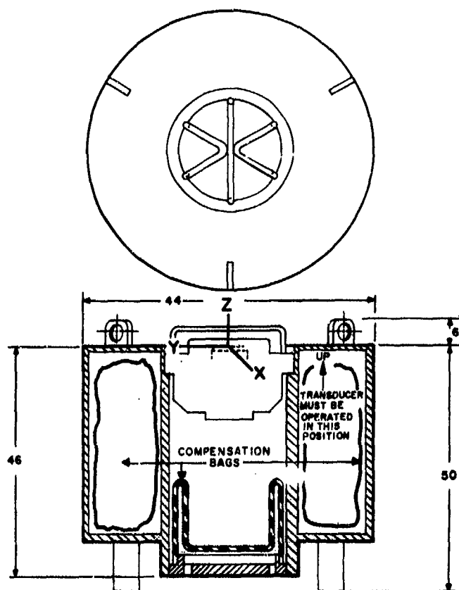
Fig. BB5. Dimensions (in centimeters) and orientation of type J15-1 transducer.
