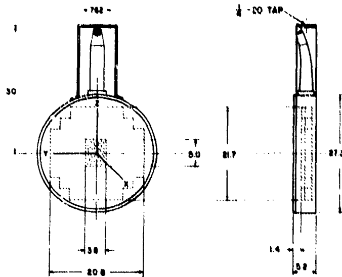
Fig. F7. (Right) Dimensions (in centimeters) and orientation of type F33 transducer (tap: UNC).
