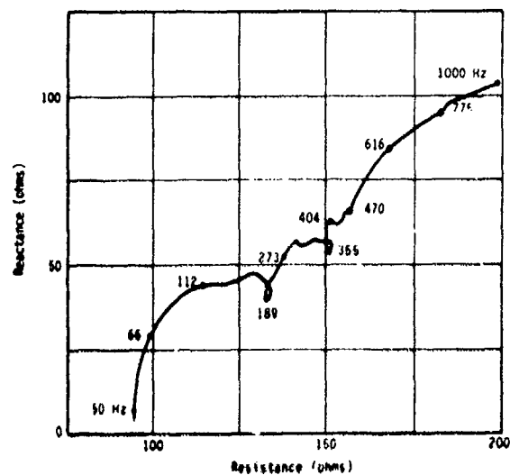
Fig. CC5. Typical impedance, three driver assembly coils in series, type J15-3 transducer.
