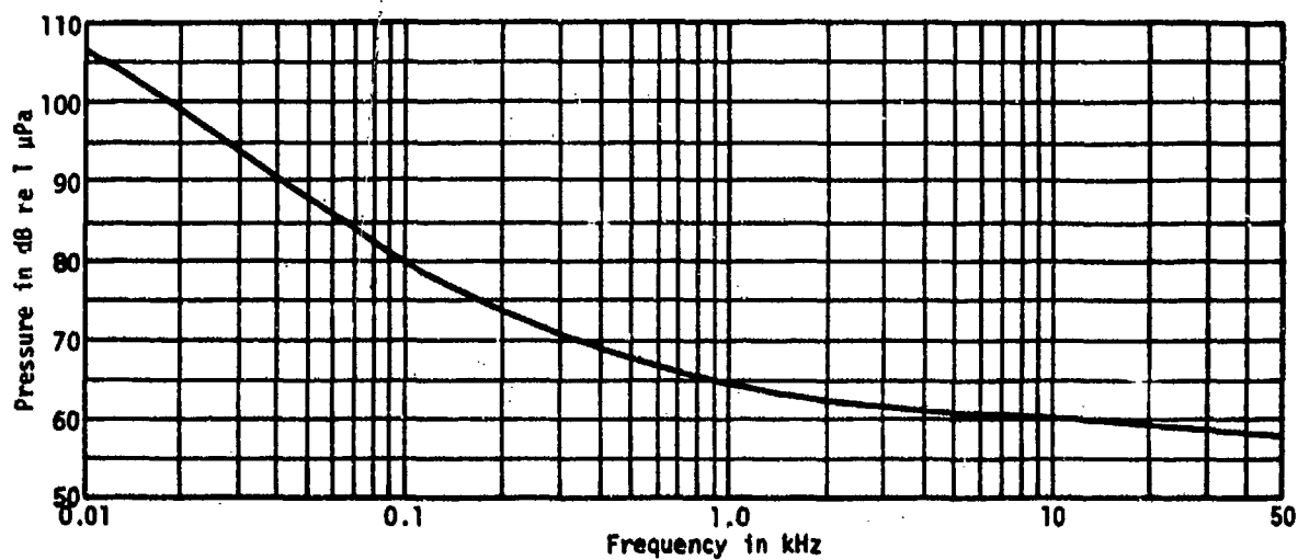
Fig. A4. Equivalent noise pressure level, type A42 hydrophone.
