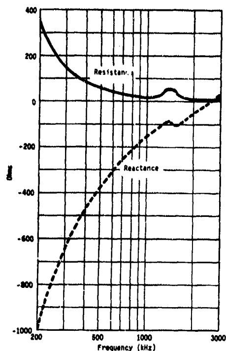
Fig. B4. Typical equivalent series impedance, type E8 transducer with 7.6-m cable.
