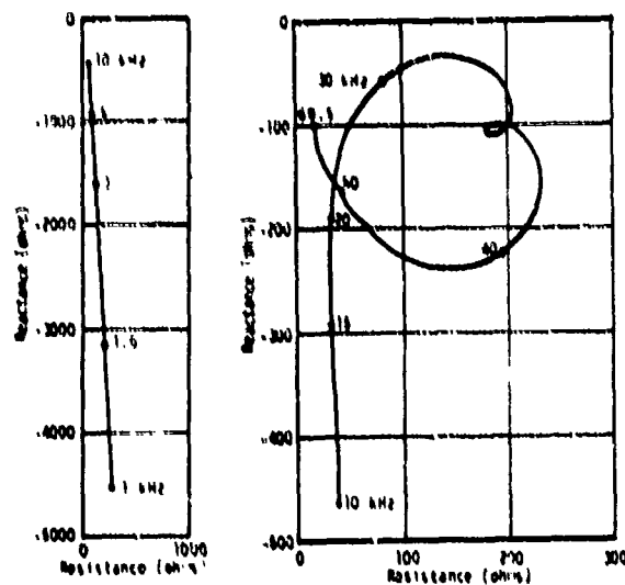
Fig. L4. Typical impedance, type F42 transducer, unbalanced, black lead and shield grounded, 11-m cable.
