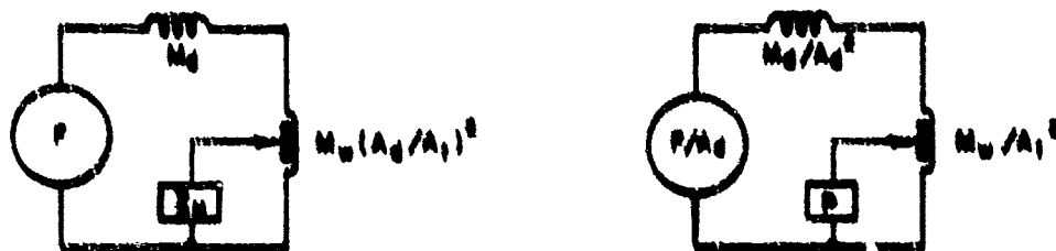
Fig. N5. Simplified equivalent mechanical (left) and acoustical (right) circuits, type G19 calibrator.
