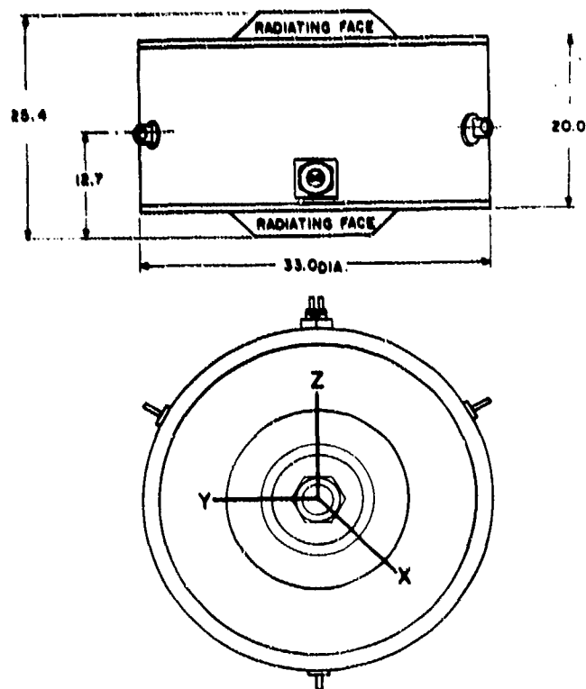
Fig. 08. Dimensions (in centimeters) and orientation, type G34 transducer.
