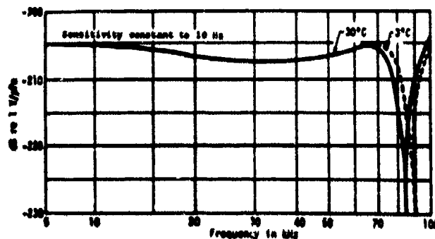
Fig. M2. Typical free-field voltage sensitivity, type F50 transducer, open-circuit voltage at end of a 23-m coaxial cable.
