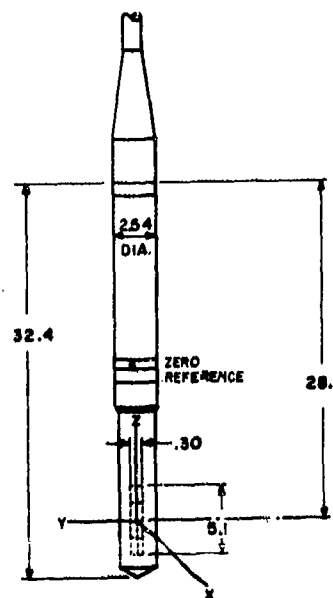
Fig. T7. (Right) Dimensions (in centimeters) and orientation of type H52 hydrophone.
