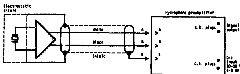
Fig. A2. Schematic circuit diagram, type A42 probe hydrophone.
