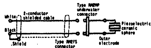
Fig. L2. Wiring diagram, type F42 transducer.
