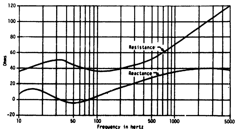
Fig. BB3. Typical transmitting current response, type J15-1 transducer.
