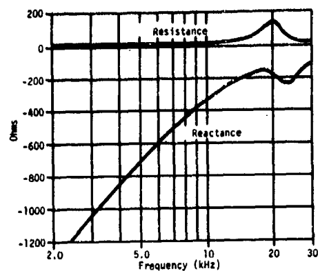
Fig. I4. Typical equivalent series impedance, type F40 transducer, unbalanced, black lead and shield grounded, 30-m cable.
