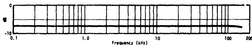
Fig. Q2. Typical preamplifier coupling characteristic, type H17 hydrophone (ratio in decibels of open-circuit voltage at preamplifier output to open-circuit crystal voltage).
