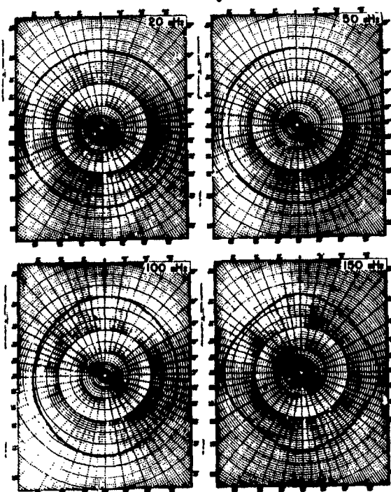
Fig. R5. Typical directivity patterns in the horizontal (XY) plane, type H17M hydrophone. Scale: center to top of grid, each pattern, equals 50 dB.
