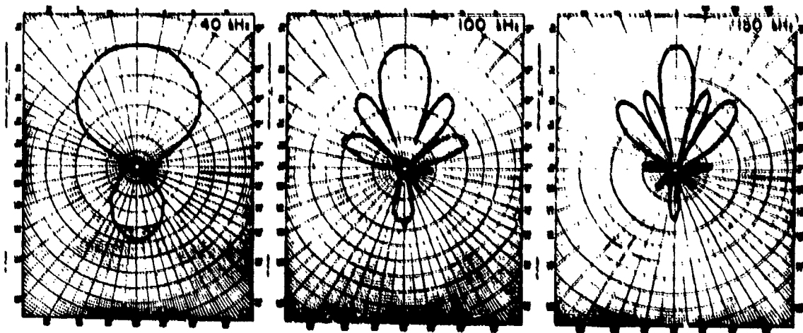
Fig. F6. Typical directivity patterns in the horizontal (XY) plane, type F33 transducer, inner section only. Scale: Center to top of grid, each pattern, equals 50 dB.
