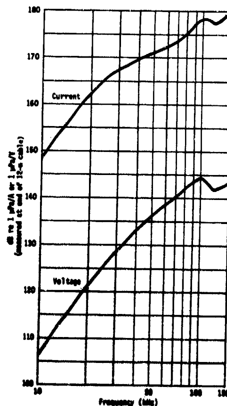
Fig. E3. (Right) Typical transmitting current and voltage responses, type F30 transducer.
