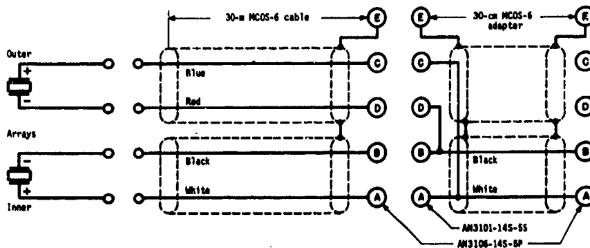
Fig. F2. (Right) Schematic diagram of cable, type F33 transducer.
