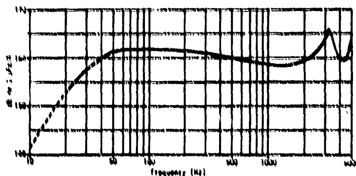
Fig. 23. Typical transmitting current response, type J13 transducer with 30-m cable.
