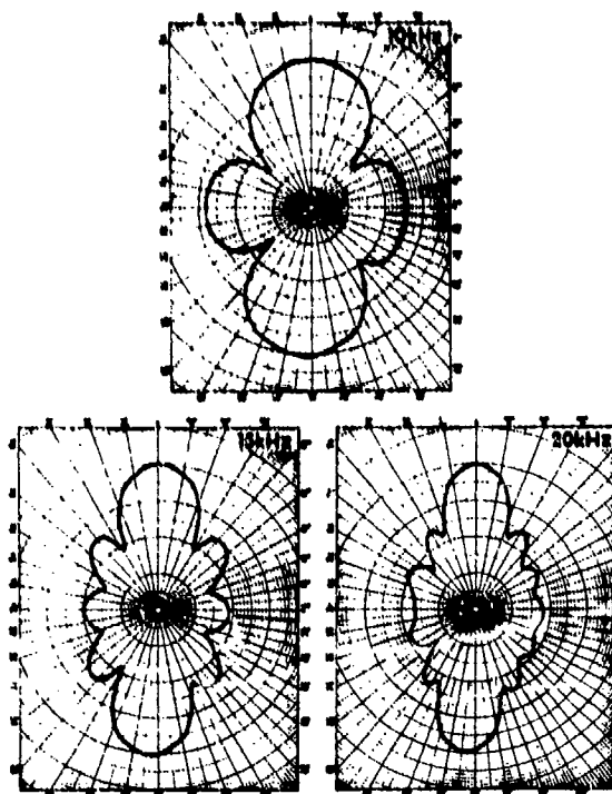
Fig. G4. Typical directivity patterns in the vertical (XZ) plane, type F36 transducer. Scale: center to top of grid, each pattern, equals 50 dB.
