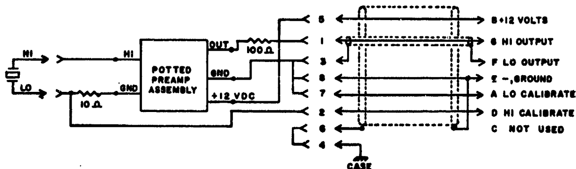
Fig. R2. Wiring diagram, type H17M hydrophone.
