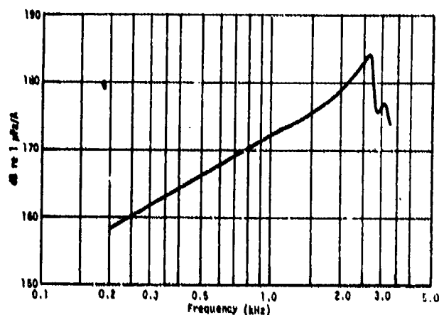
Fig. 04. (Right) Typical transmitting current response, type G34 transducer, unbalanced, black lead and shield grounded, 76-m cable.
