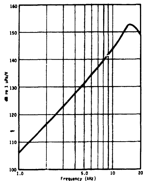
Fig. J3. (Right) Typical transmitting voltage response, type F40A transducer; unbalanced, black lead and shield grounded, 30-m cable.
