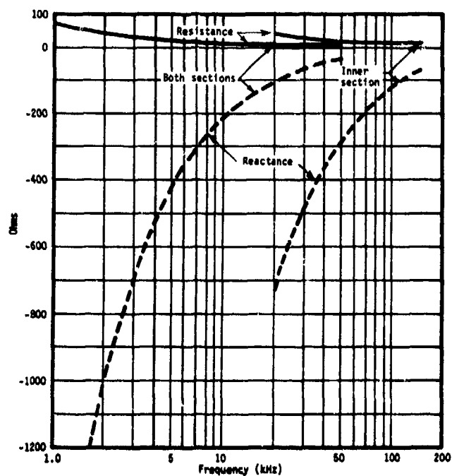
Fig. F4. (Right) Typical equivalent series impedance, type F33 transducer.
