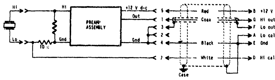
Fig. T2. Wiring diagram, type H52 hydrophone.
