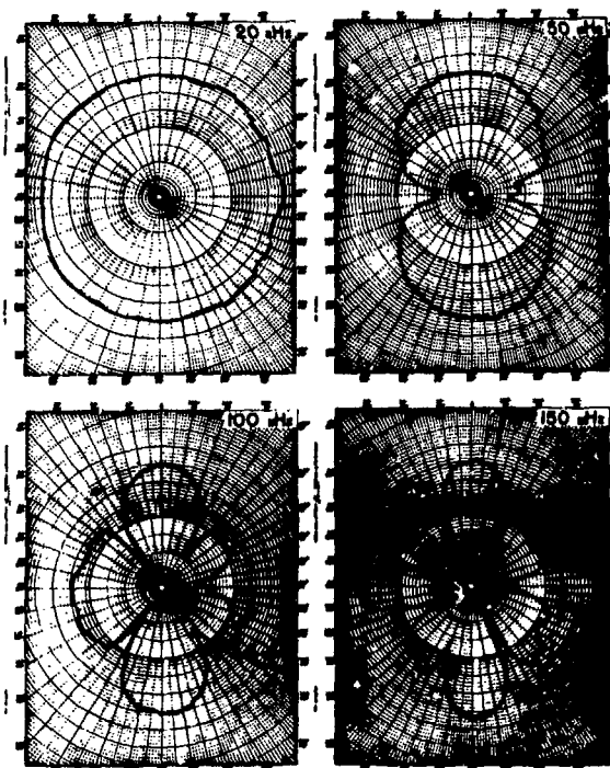
Fig. R6. Typical directivity patterns in the vertical (XZ) plane, type H17M hydrophone. Scale: center to top of grid, each pattern, equals 50 dB.
