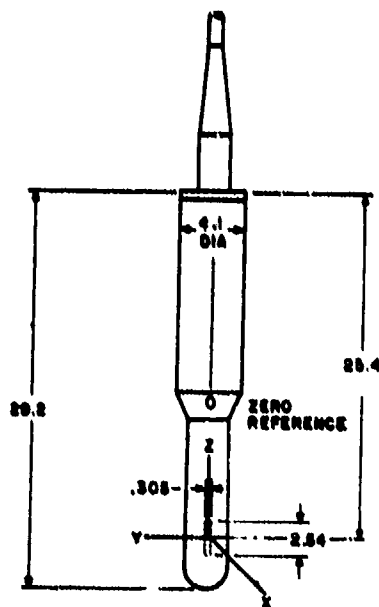
Fig. Q9. Dimensions (in centimeters) and orientation of type H17 hydrophone.
