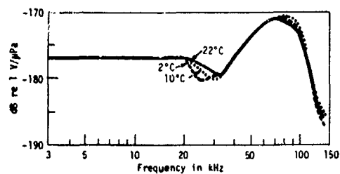
Fig. U4. (Right) Effect of temperature on the free-field voltage sensitivity of the striped ceramic tube model, type H56 hydrophone.
