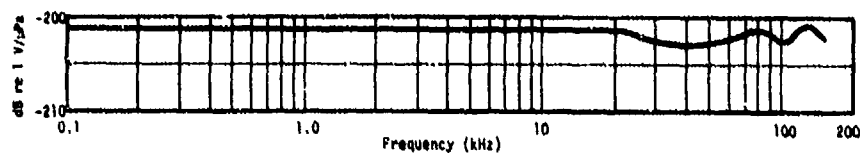
Fig. Q4. Typical free-field voltage sensitivity, type H17 hydrophone (open-circuit voltage at end of 12-m cable).
