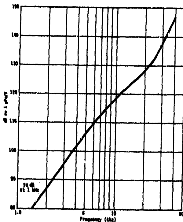
Fig. D3. Typical transmitting voltage response, type F27 transducer.
