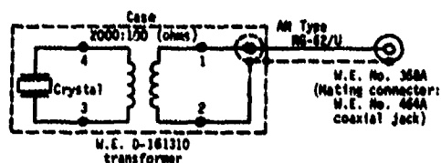
Fig. B2. Circuit diagram, type E8 transducer.
