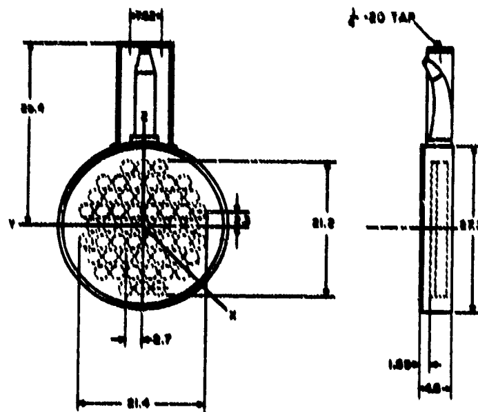
Fig. D6. Dimensions (in centimeters) and orientation of type F27 transducer (tap: UNC).
