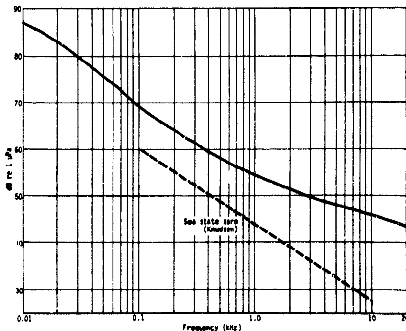
Fig. R4. (Right) Typical equivalent noise pressure measured at end of 12-m cable, type H17M hydrophone.
