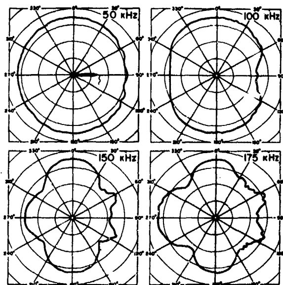
Fig. A6. Directional characteristics in the vertical (XZ) plane, type A42 probe hydrophone; center to top of grid, each pattern, equals 40 dB.
