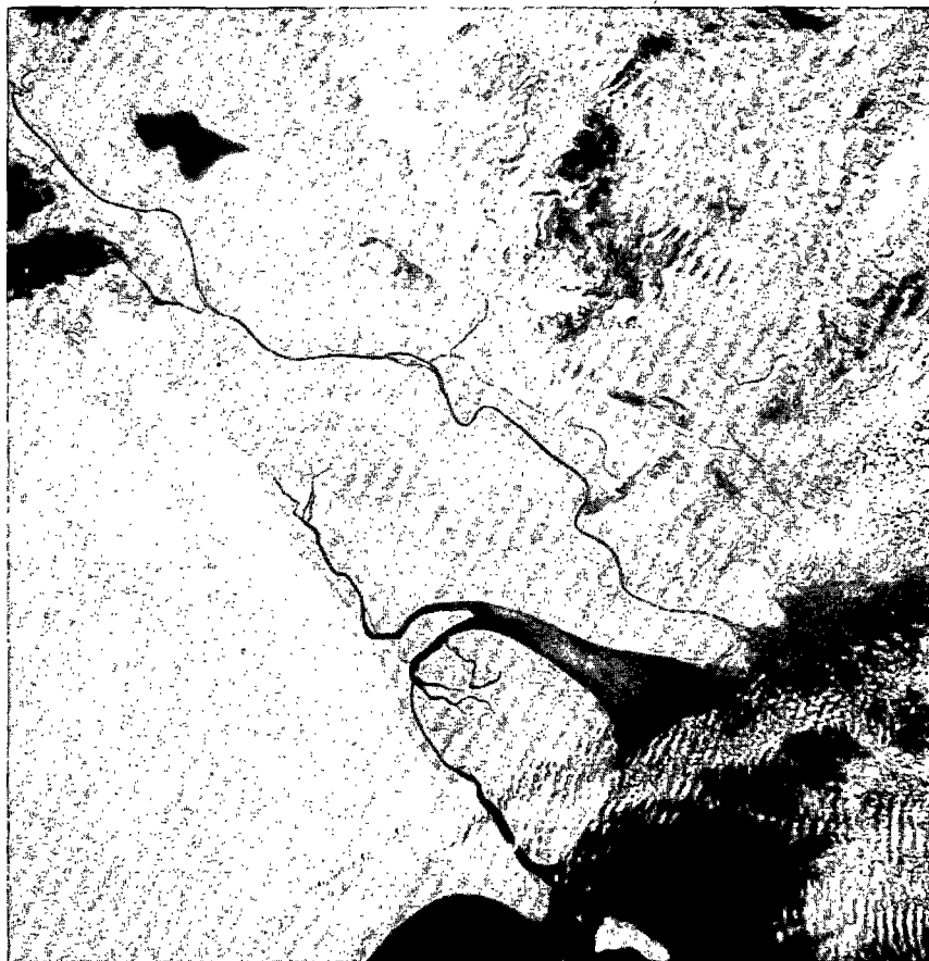
Figure 53. ERTS satellite image of the Shatt-al-Arab Delta.
