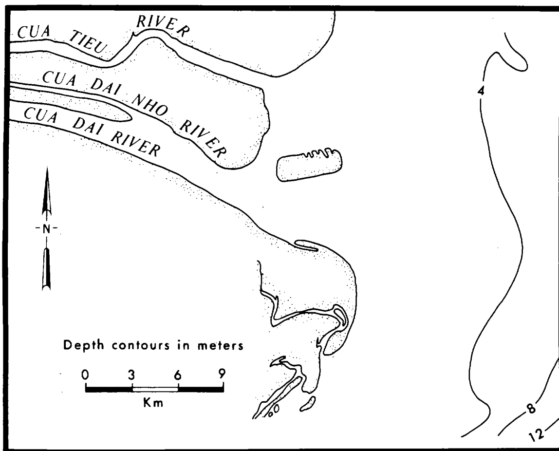
Figure 61. Mouths of the Mekong River.
