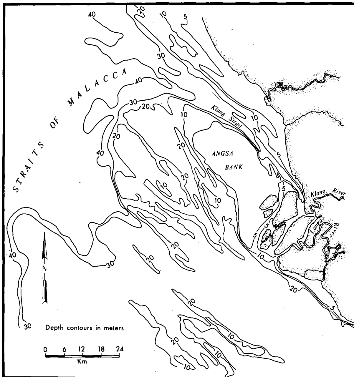
Figure 27. Bathymetric chart of the Klang Delta.
