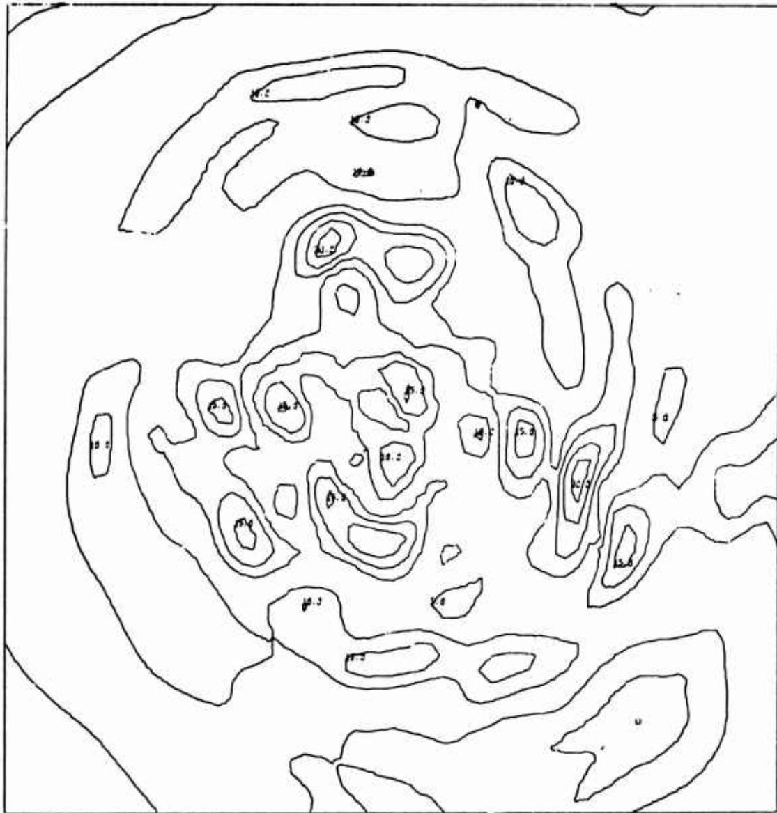
CHART Q. 925 MB Level Isotach Field (Experiment V)
