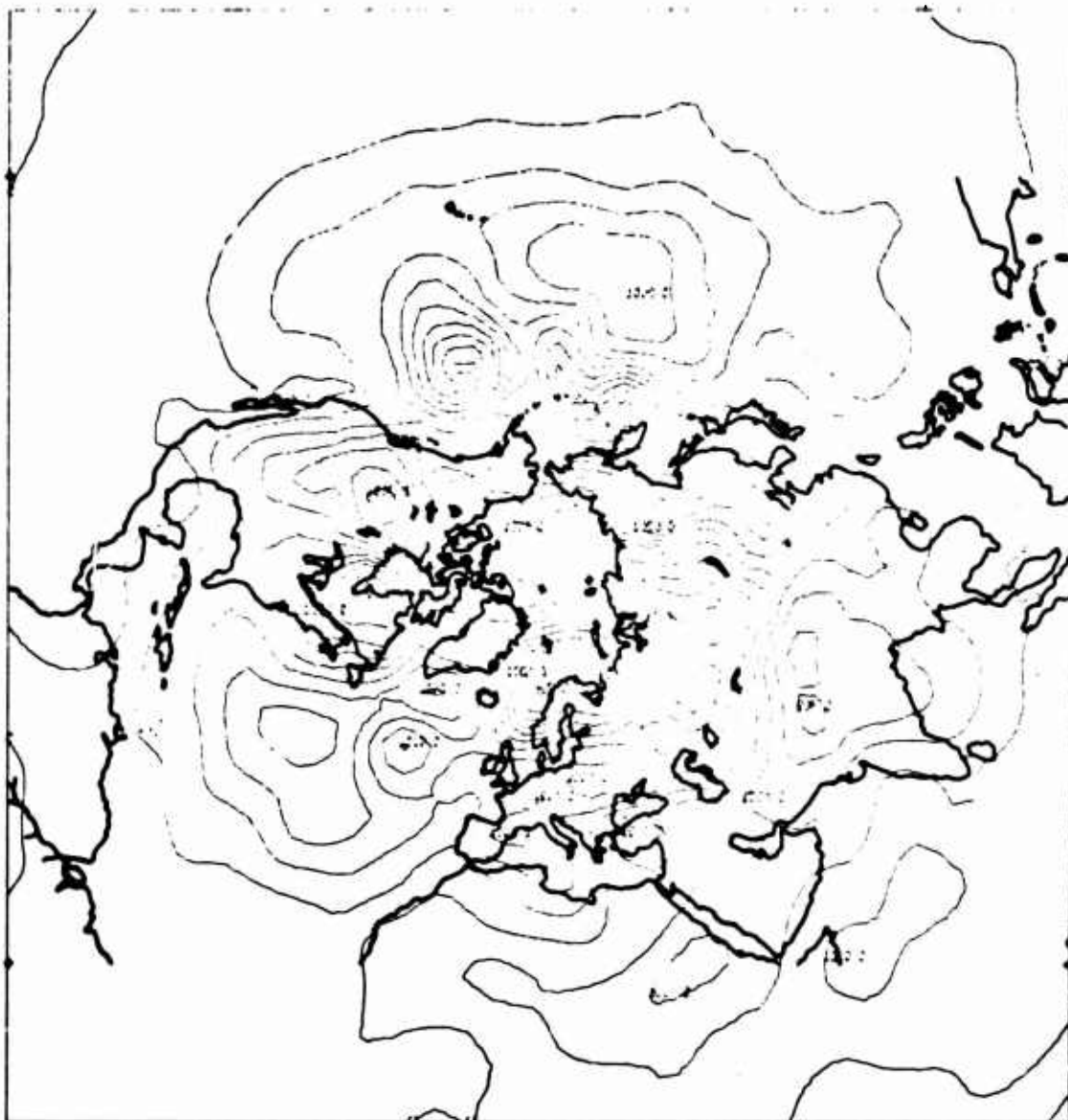
CHART DD. PNWC Objective Surface Pressure Analysis 12 Z 13 May 73 (Experiment VIII)
