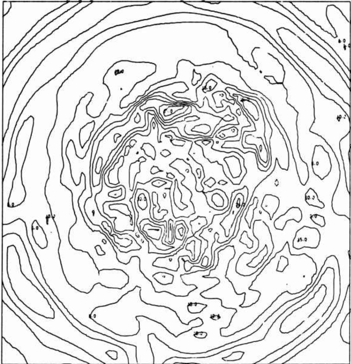
CHART V. 0.5 Sigma Level Isotach Field (Experiment V)
