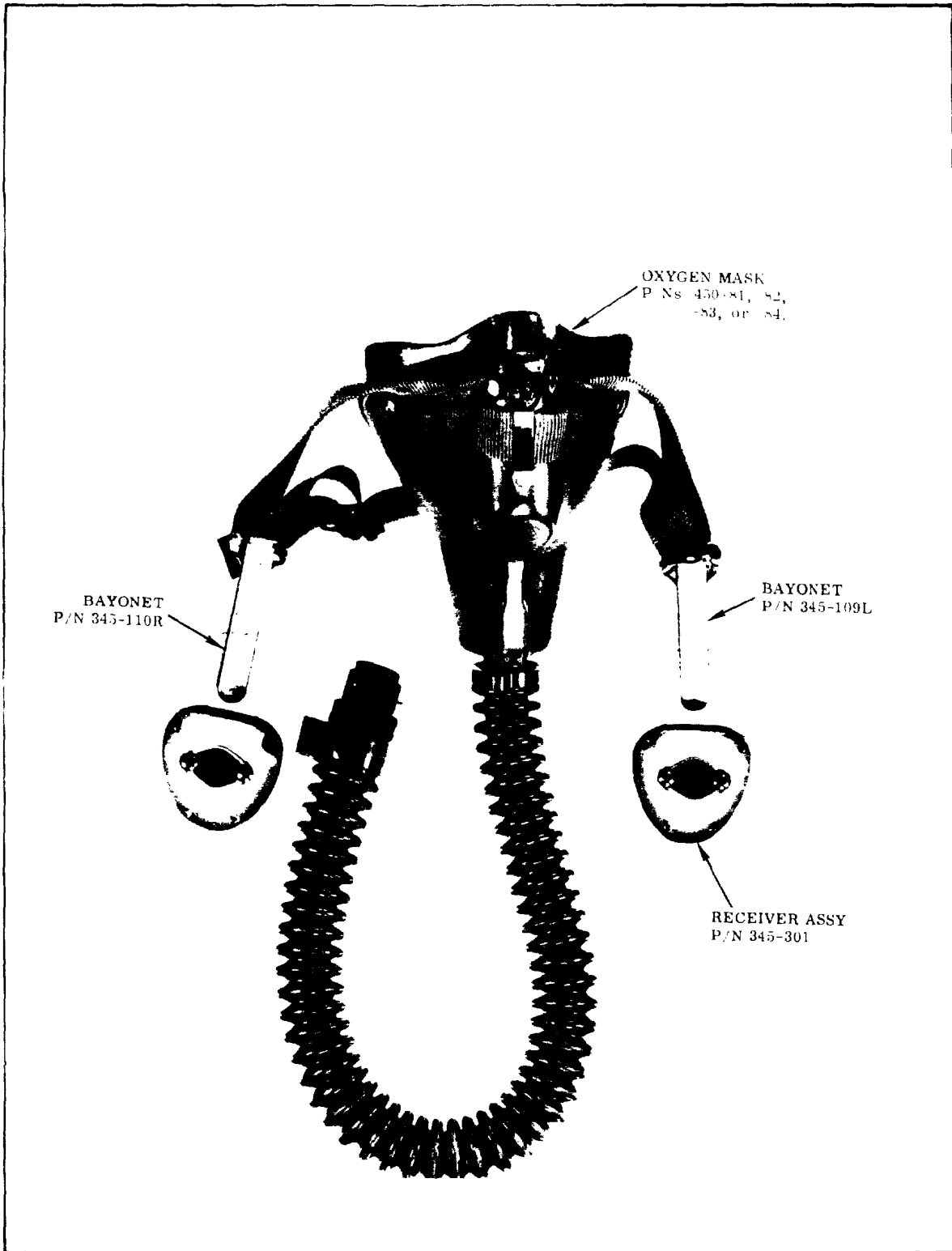
Figure 1-1. Pressure Demand Breathing Oxygen Mask, Type MBU-5 'P', and Accessories (sheet 1 of 5)
