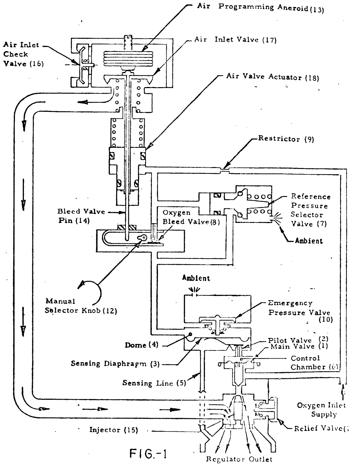
SCHEMATIC, SYSTEM - MILITARY DILUTER
