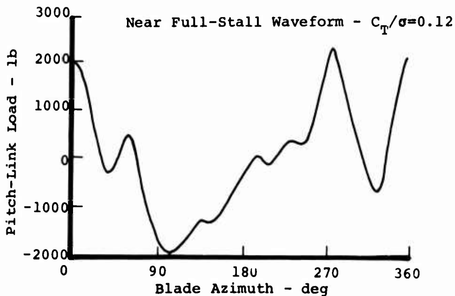
Figure 33. Typical Pitch-Link Load Waveforms for the 3/Rev Blade at 125 Knots, \mu = 0.289 .
