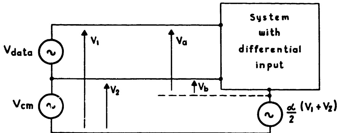
Fig.11 Equivalent circuit of a differential switch and amplifier
