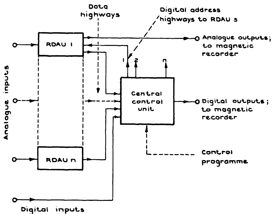
Fig.8 PCM sub-system with remote acquisition and central control
