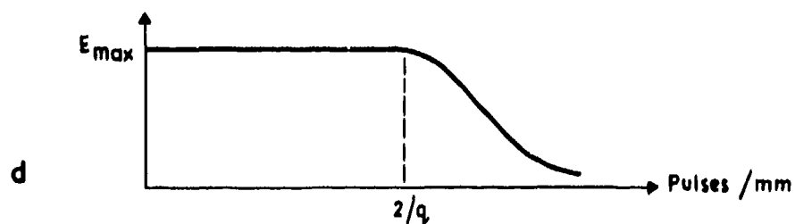
Fig.20 Pulse crowding
