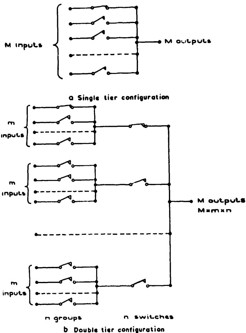
Fig.13 a&amp;b Multiplexer configurations
