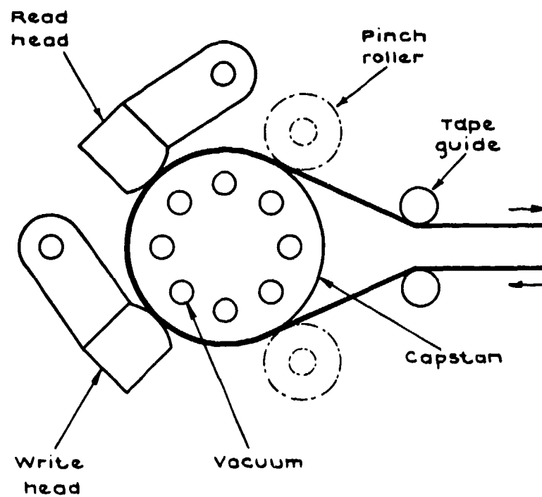
Fig.33 Zero-loop drive system
