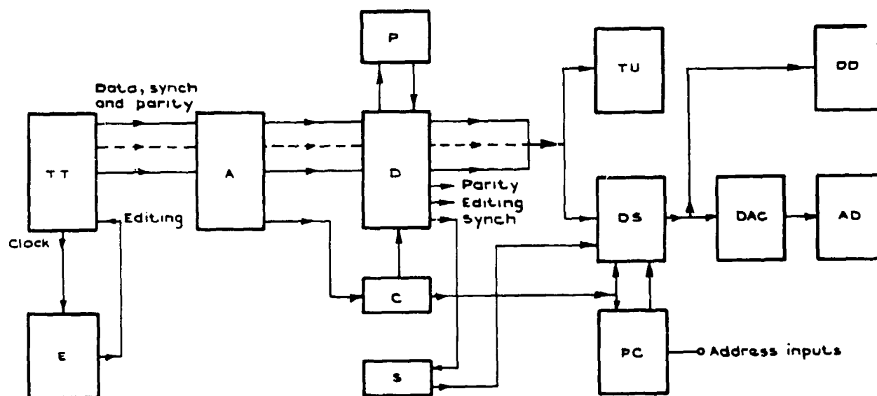
Fig.1 PCM (with TDM) record sub-system
