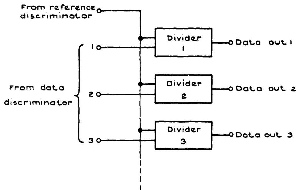
Fig.30 Multiplicative compensation of FM data
