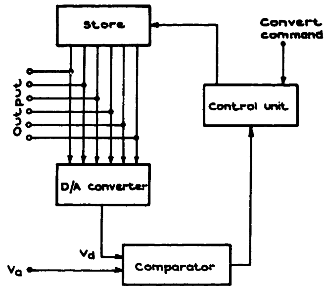
Fig.15 Basic feedback analogue/digital converter
