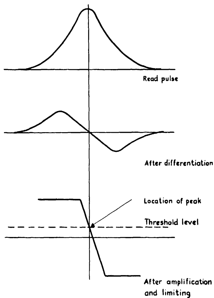
Fig.28 Peak sensing of the read pulse
