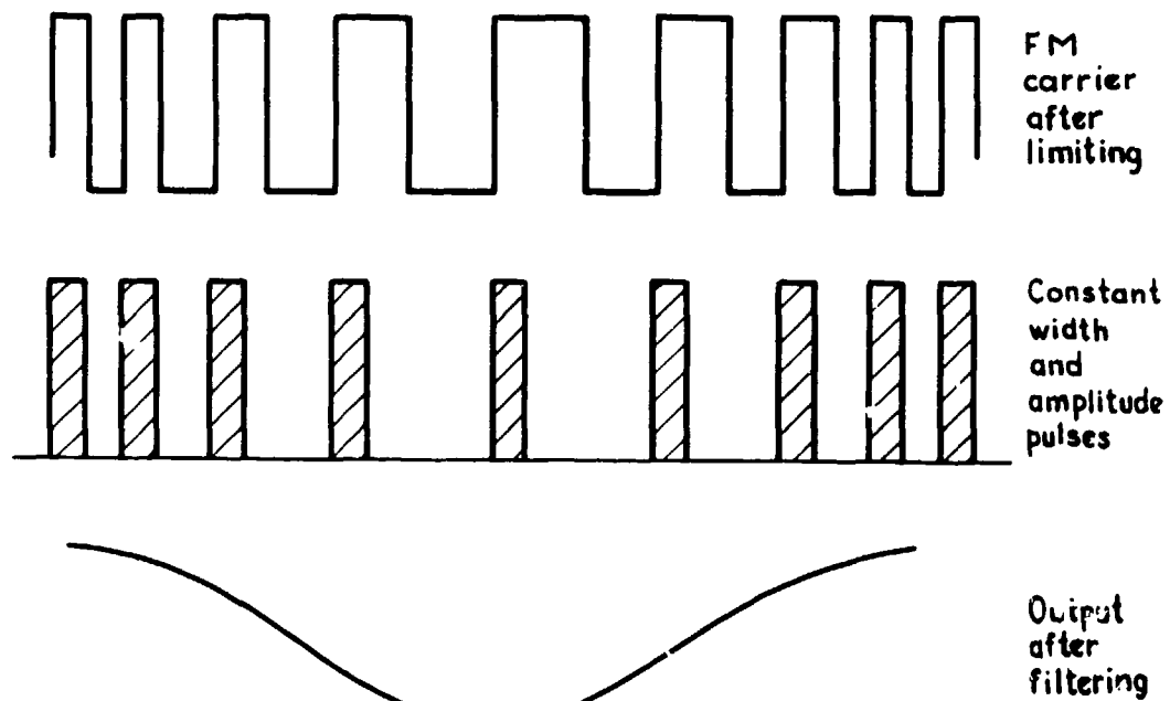
Fig.23 Pulse type FM discriminator
