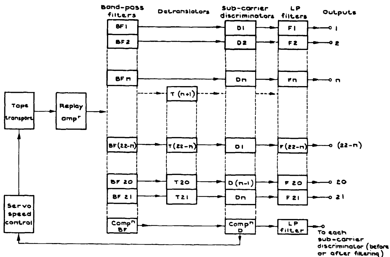
Fig.6 Frequency-division multiplexed FM replay sub-system
