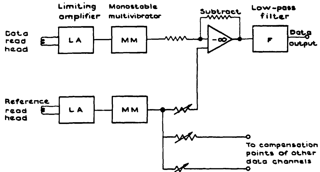
Fig.29 FM demodulation with subtractive compensation
