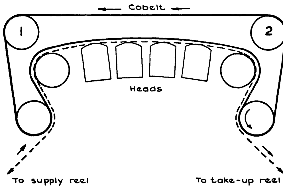
Fig.34 Cobelt drive system
