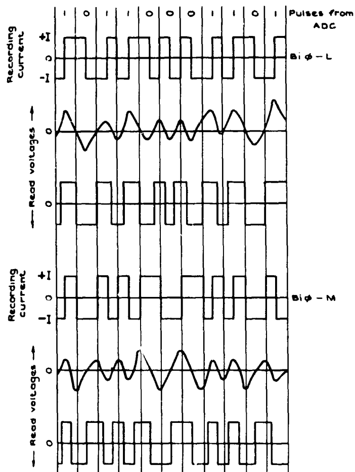
Fig.26 Phase modulation waveforms (Biφ-L and Biφ-M)
