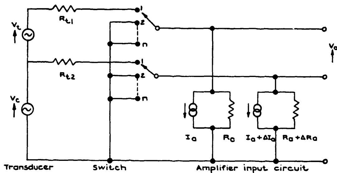
Fig.9 Model of differential switch and amplifier
