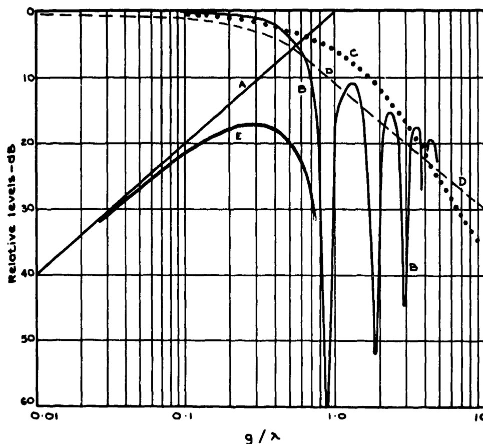
Fig.17 Head/tape relationship for ring-type head
