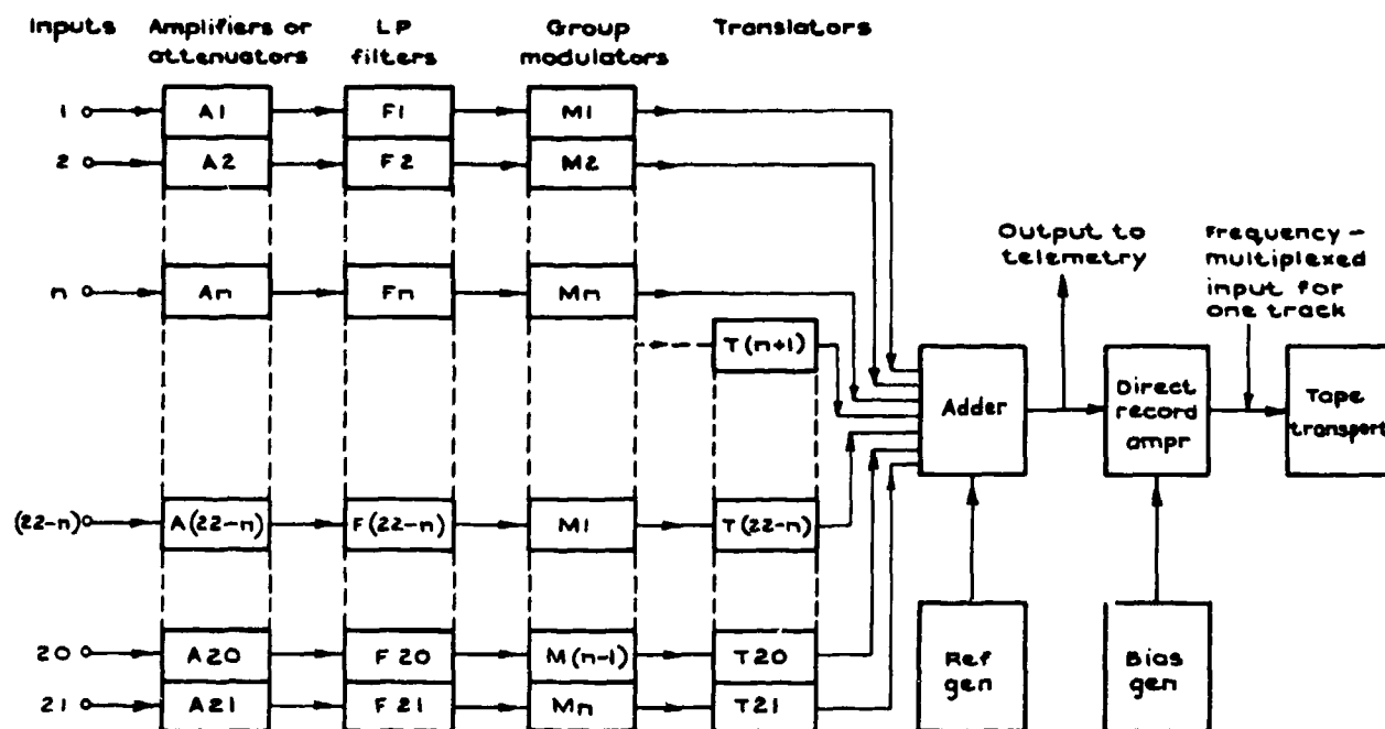
Fig.5 Frequency-division multiplexed FM record sub-system
