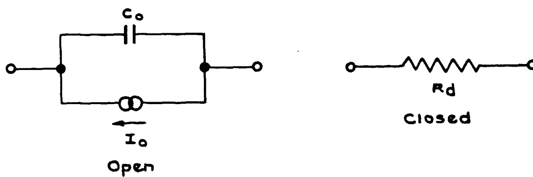
Fig.10 Equivalent circuit of a switching element
