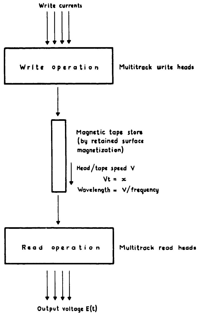
Fig.16 Representation of the magnetic recording process
