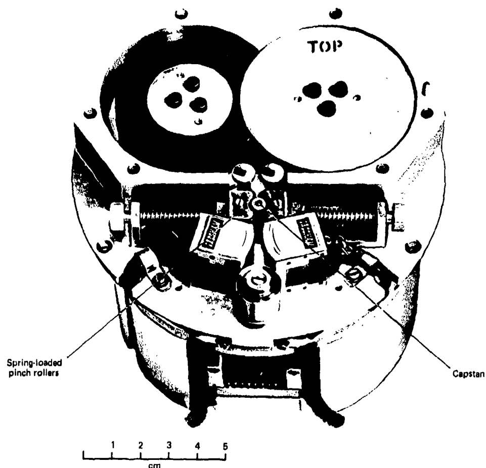
Fig.39 Weapon-borne transport with integral power unit
