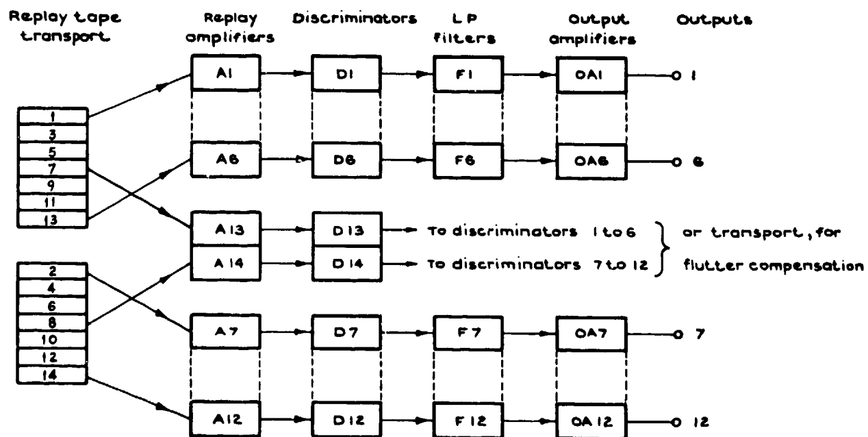
Fig.4 Single-carrier FM replay sub-system
