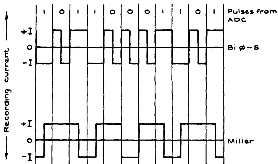
Fig.27 Biφ-S and Miller codes
