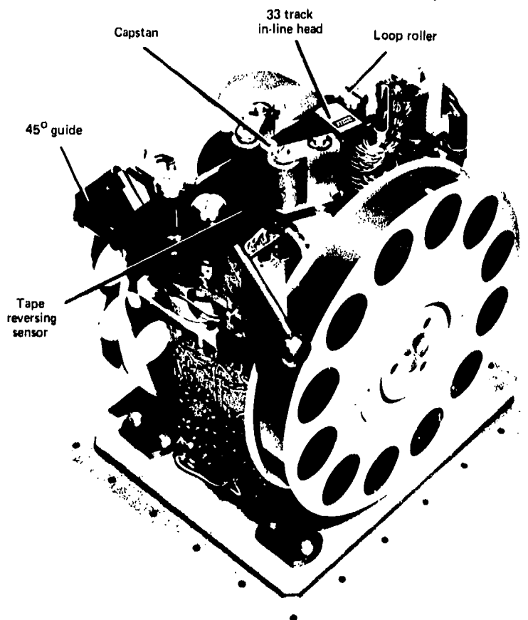
Fig.37 Airborne tape transport with dual capstan drive
