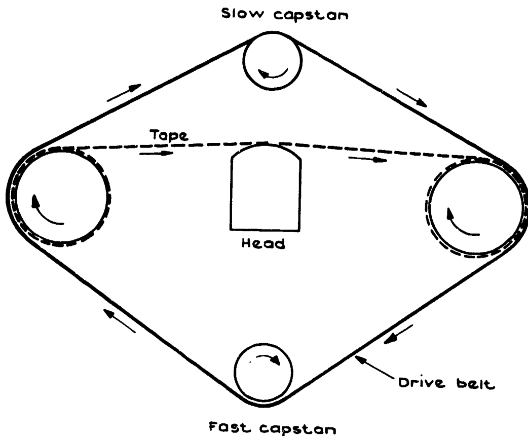
Fig.35 ISO-elastic drive system
