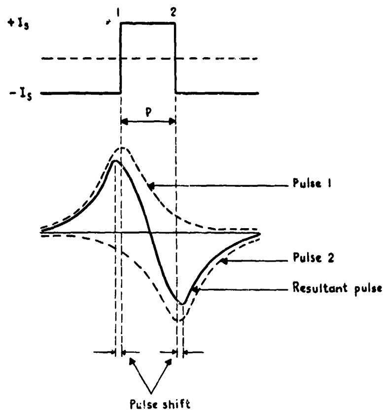
Fig.21 Superposition of two adjacent saturation reversals
