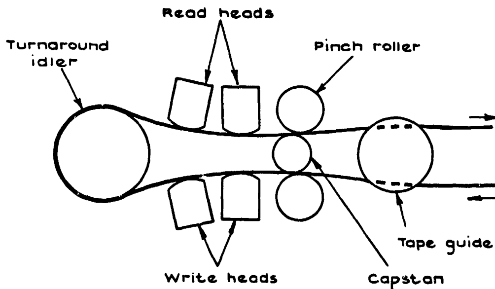
Fig.32 Closed loop drive system
