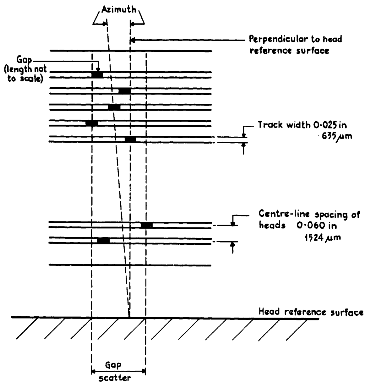
Fig.41 16-Track 25.4mm digital head showing azimuth and gap scatter
