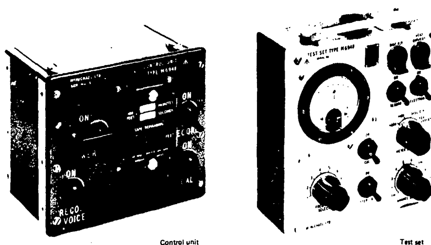
Fig.24 Airborne package of single-carrier FM record electronics (manufactured by McMichael Ltd.)
