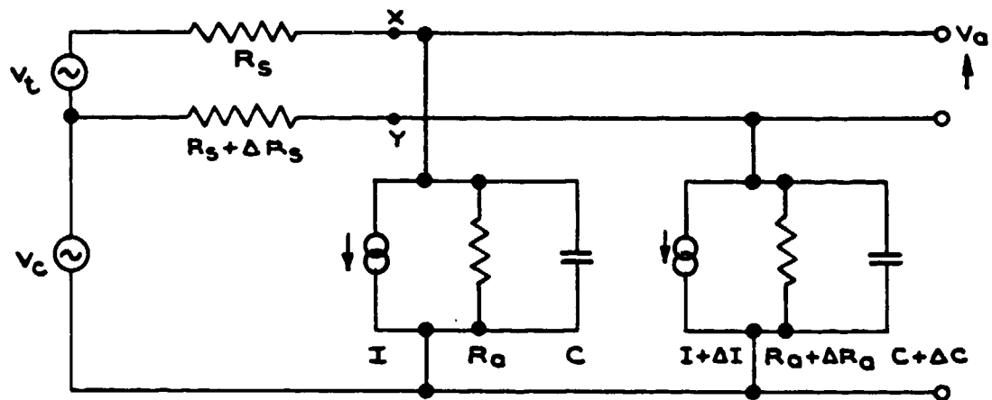
Fig.11 Equivalent circuit of a differential switch and amplifier
