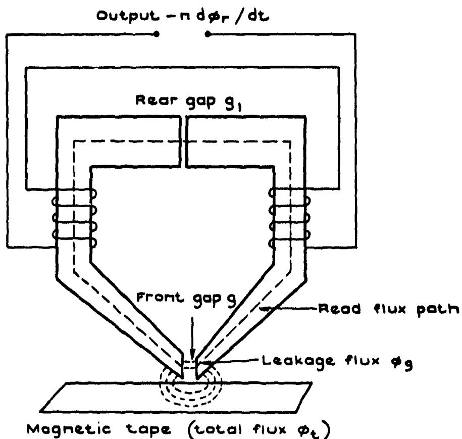
Fig.40 Read head operation
