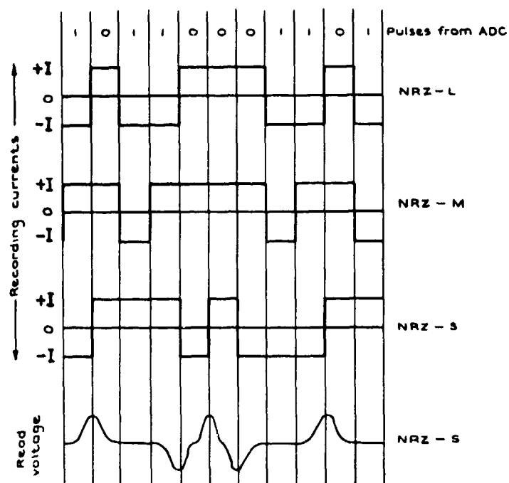
Fig.25 Non-return-to-zero recording waveforms
