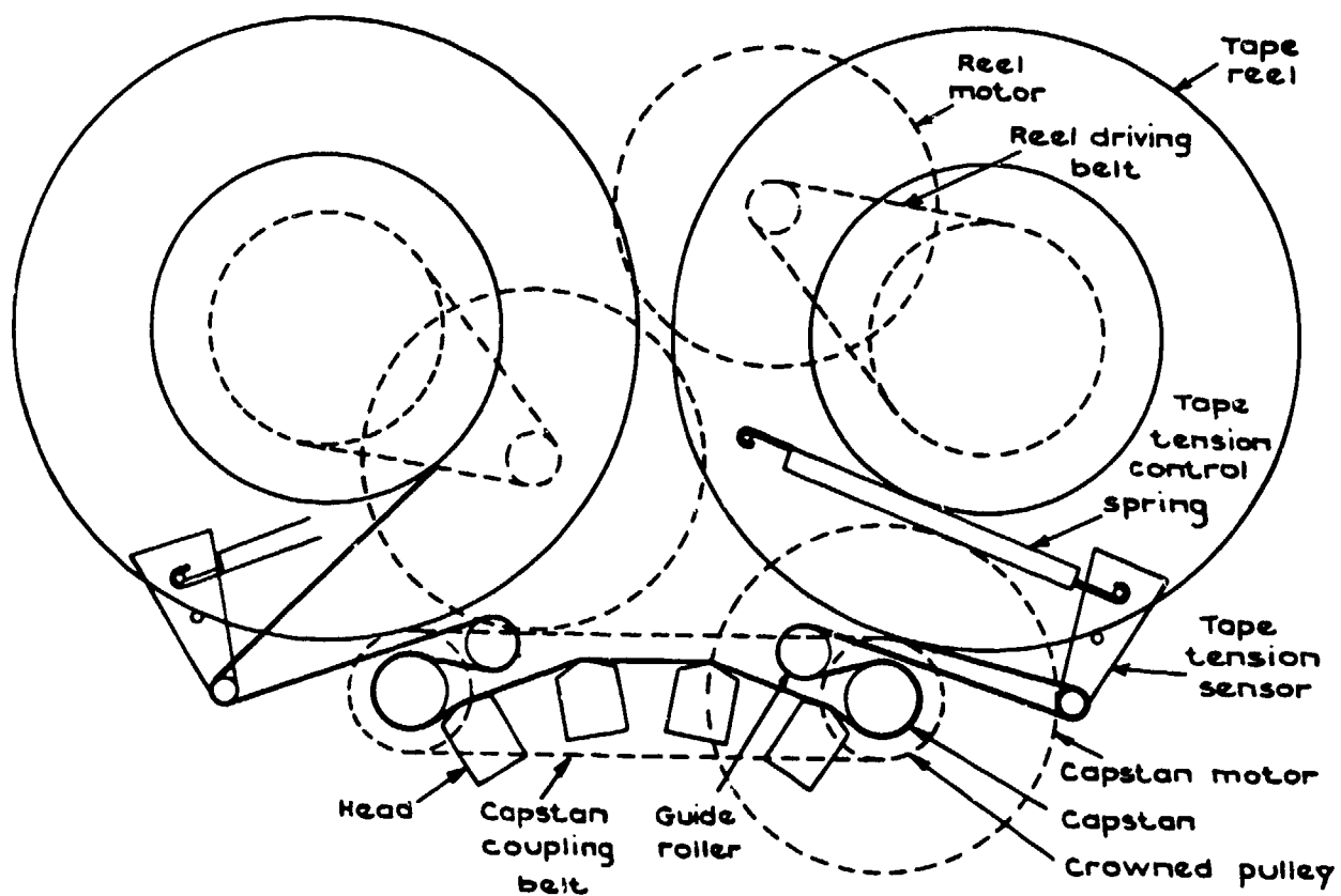
Fig.36 Dual - capstan drive system
