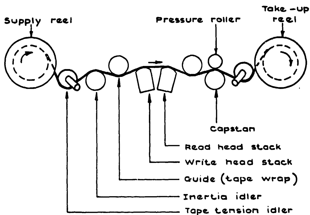
Fig.31 Open-loop drive system
