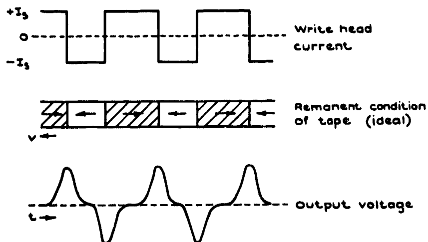
Fig.19 Digital recording transitions
