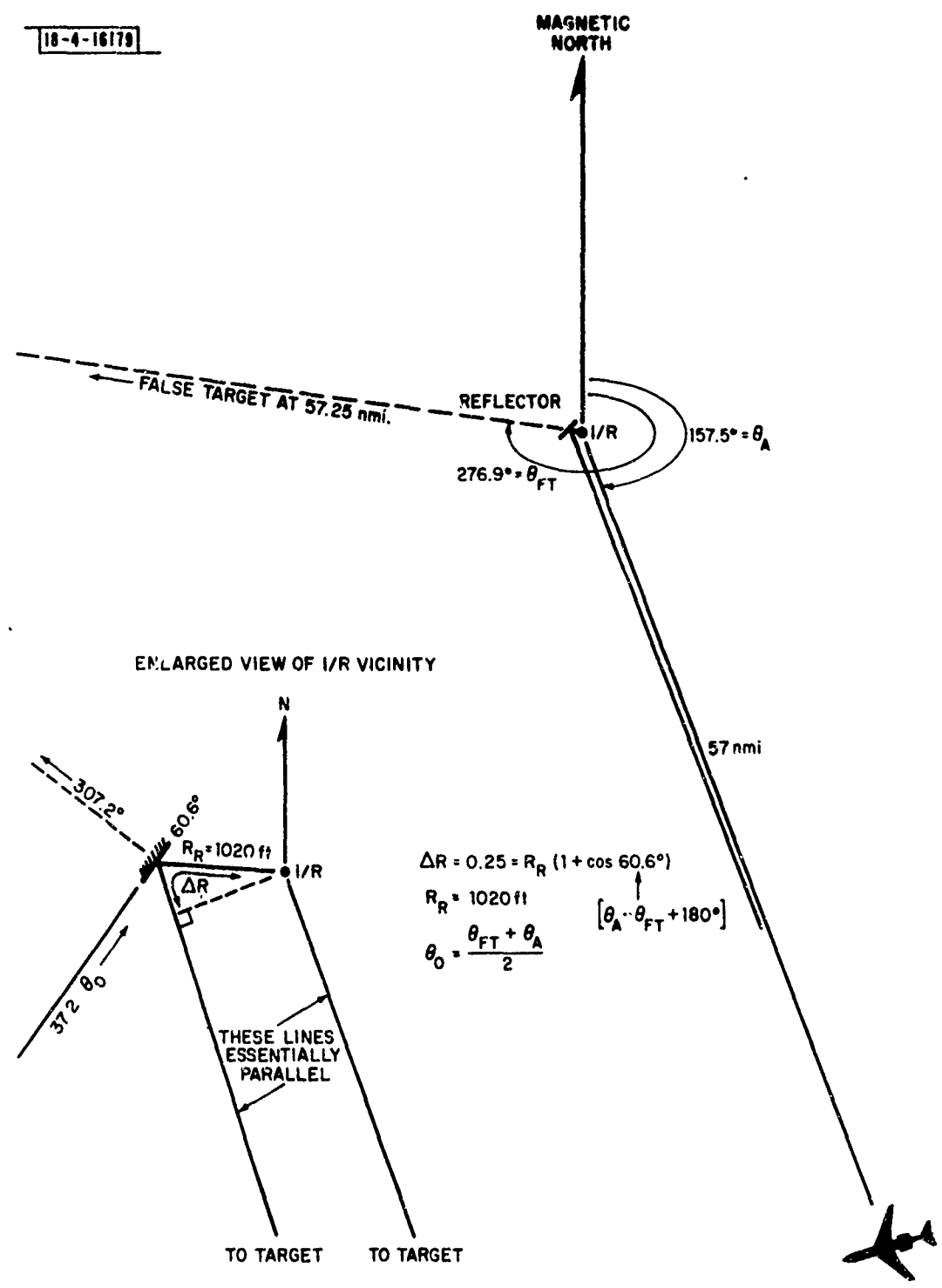
Fig. 4. Simplified geometry ( R_A \gg R_R ).
