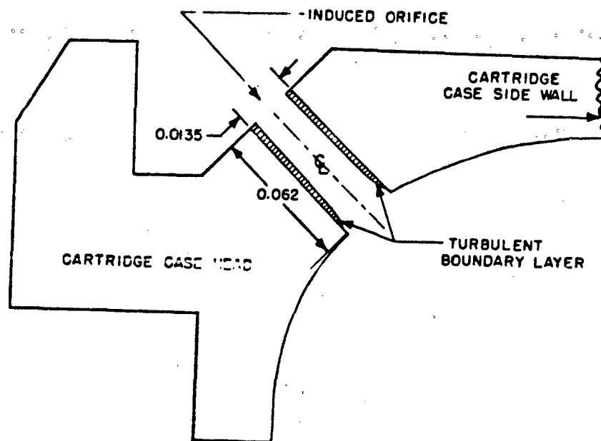
Figure 4. Head Region of 5.56mm Aluminum Alloy Cartridge Case
