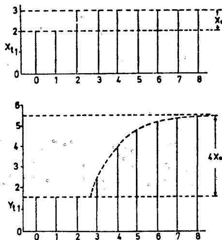
FIG. 5. Delayed exponential response to a step change produced by (1 + \nabla)(Y_{t+1} - 1.5) = 4(1 - 0.5\nabla)(X_t - 2) or (1 + \nabla)Y_{t+1} = -6.5 + 4(1 - 0.5\nabla)X_t
