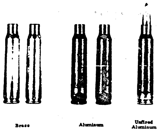
Figure 1. Drilled Hole Experiment
