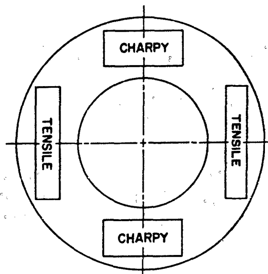
Figure 1. Schematic Showing Test Specimen Sampling Plan Along Tube Length
