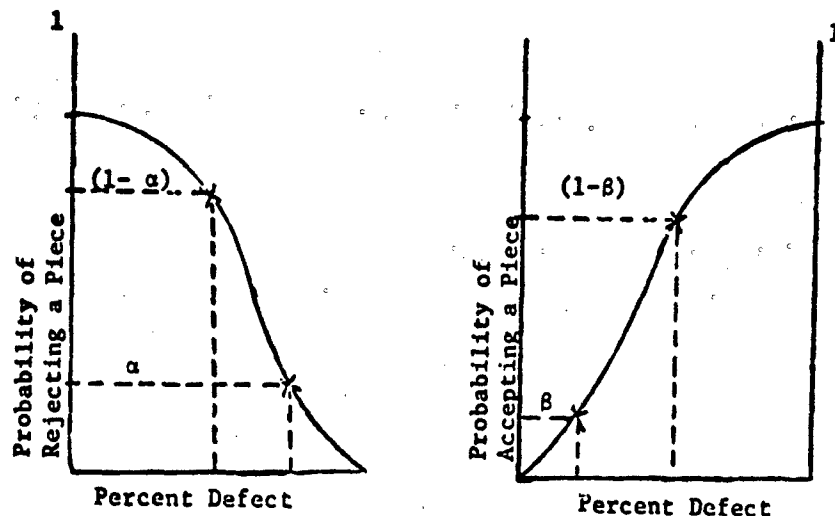
Figure 3. Operating Characteristic Curves for Individual Inspections
