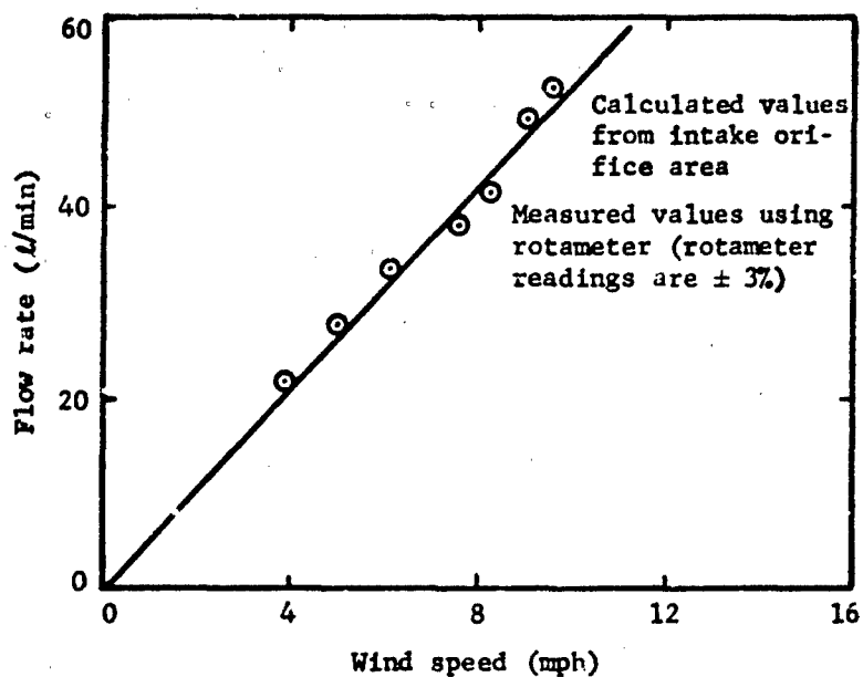
Figure 11. Flow Rate Through the Isokinetic Sampler
