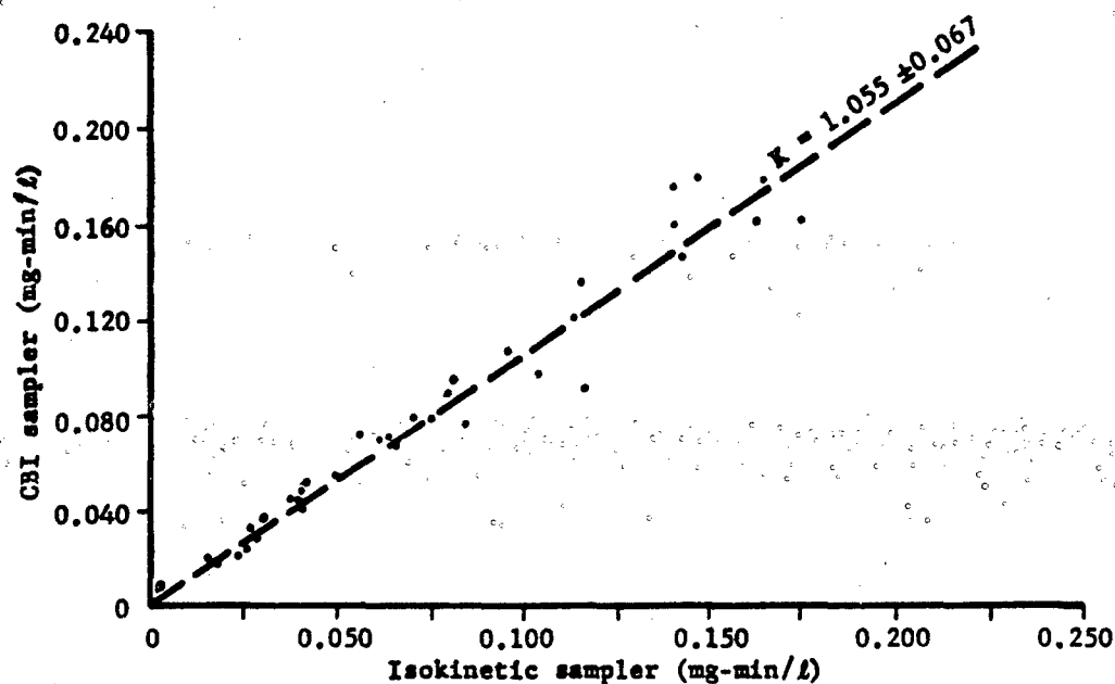
Figure 15. Isokinetic Sampler vs. CBI and CI Sampler (Regression Analysis)
