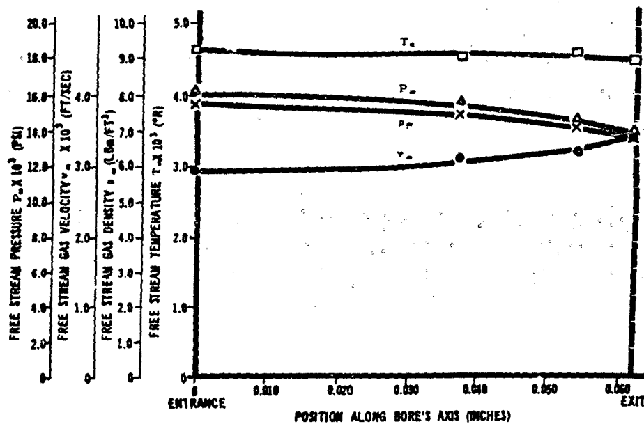
Figure 7. Free Stream Conditions vs Position Along Bore's Axis ( f = 0.002 )
