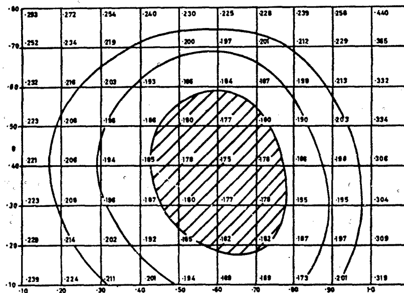
FIG. 3. Sum of squares grid and contours of S(\theta, \Theta) for airline data with approximate 95% confidence region shaded
