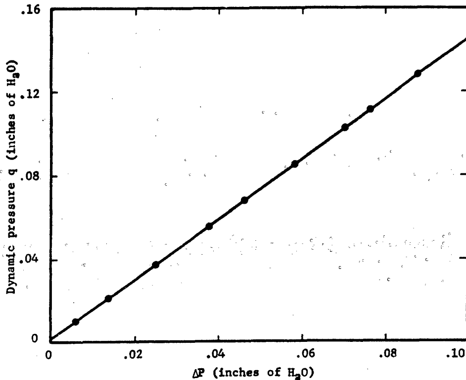
Figure 8. Calibration of Speed Rings
