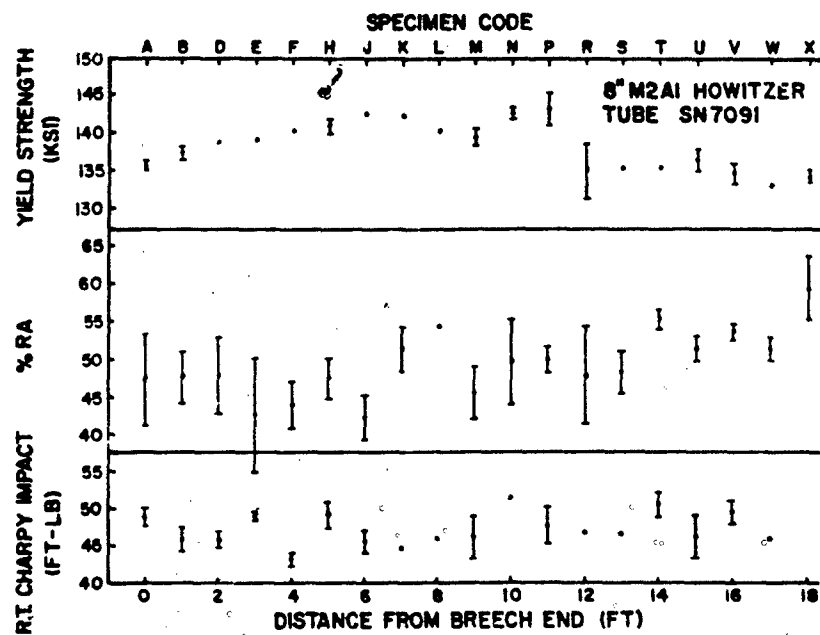
Figure 11. Mechanical Property Variations in 8" M2A1 Howitzer Tube SN7091
