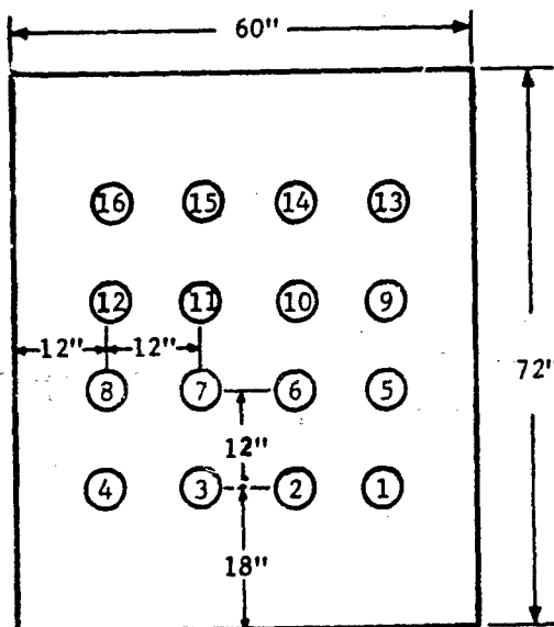
Figure 3. Pitot Tube Configuration at the Test Section (Downstream View)
