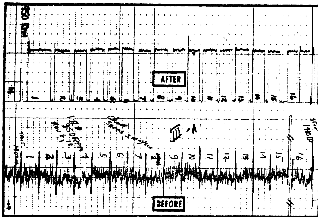
Figure 4. Dynamic Pressure Measurements Before and After Modification
