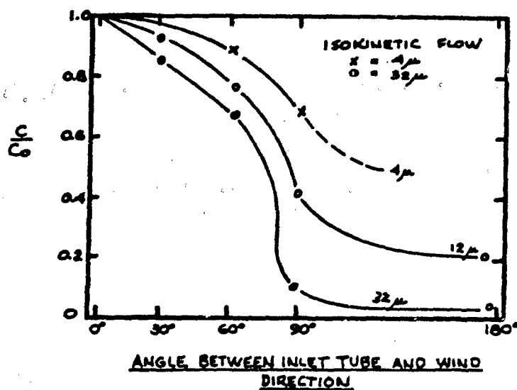
Figure 19. Isokinetic Sampling Factors with the Inlet Tube Aligned at Various Angles to the Windstream (after Mayhood and Langstroth) (1)
