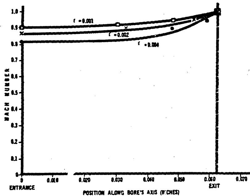
Figure 6. Mach Number as a Function of Position Along the Bore (Friction Factor as Indicated)
