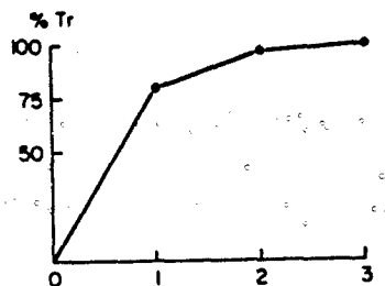
FIGURE 6 A plot of percentual eigenvalues for [S_4] .
