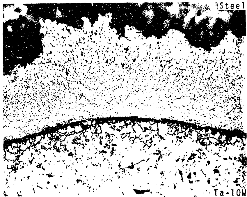
FIGURE 16 Specimen No. 5, 400X, after Swabbing with and by Immersion in Lactic, Nitric, and Hydrofluoric Acid Etchant which Chemically Polishes the Ta Alloy and Dissolves the Steel
