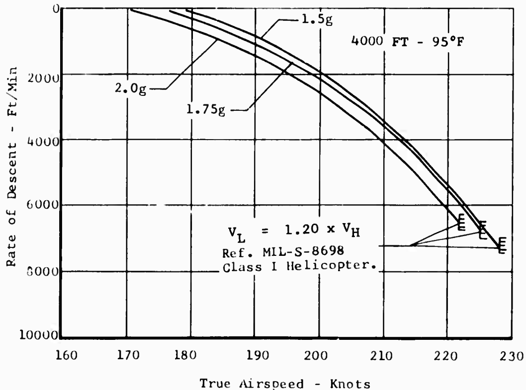
Figure 92. Rate of Descent at Normal Rated Power.
