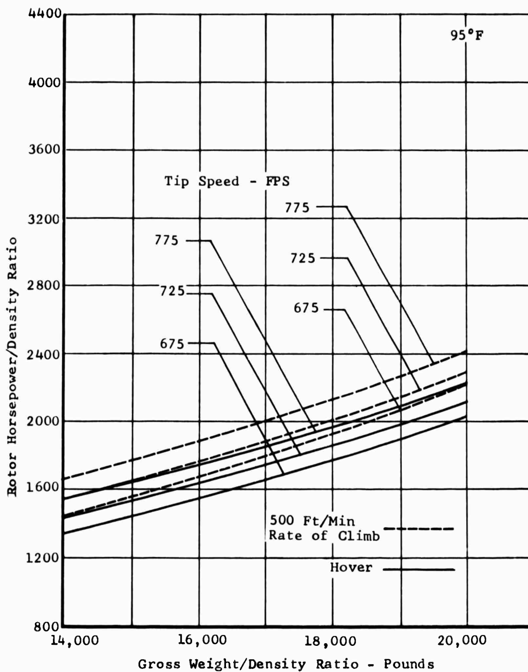
Figure 2. Task I - Wingless Helicopter, Hover Power Required, Solidity = 0.11.
