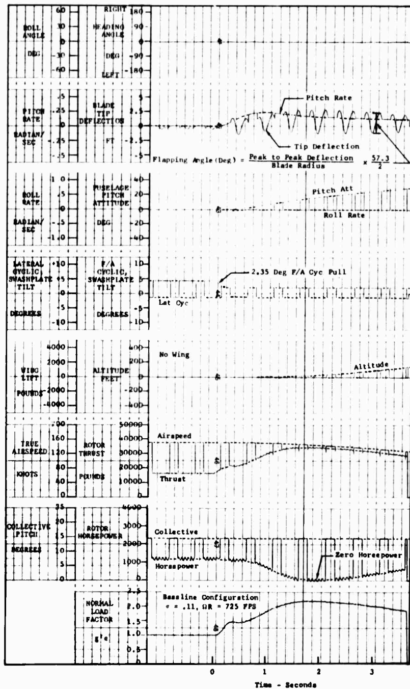
Figure 7. Maneuver Time History, F/A Cyclic Pullup, Maneuver Limited by Zero Horsepower.
