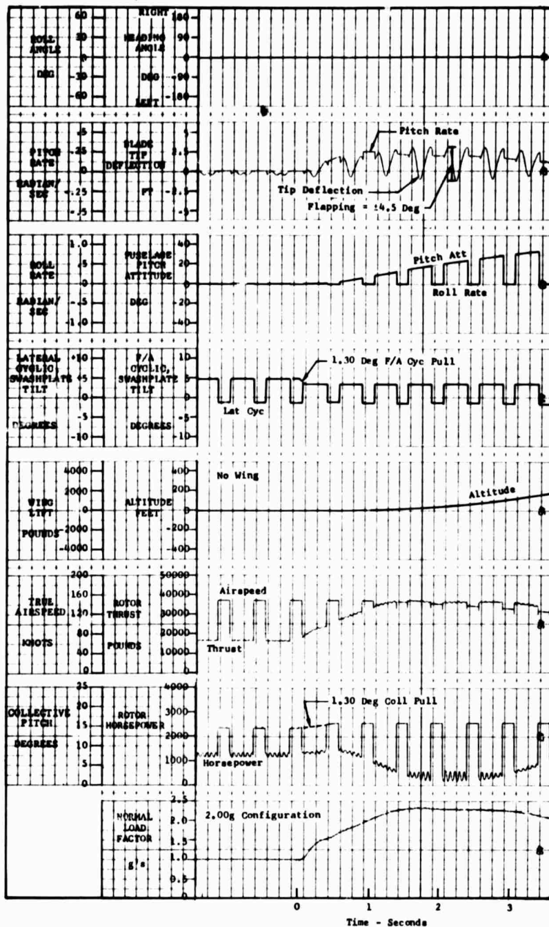
Figure 77. Maneuver Time History, 2.00g Configuration, Limiting Collective + Cyclic Pullup at 150 KTAS.
