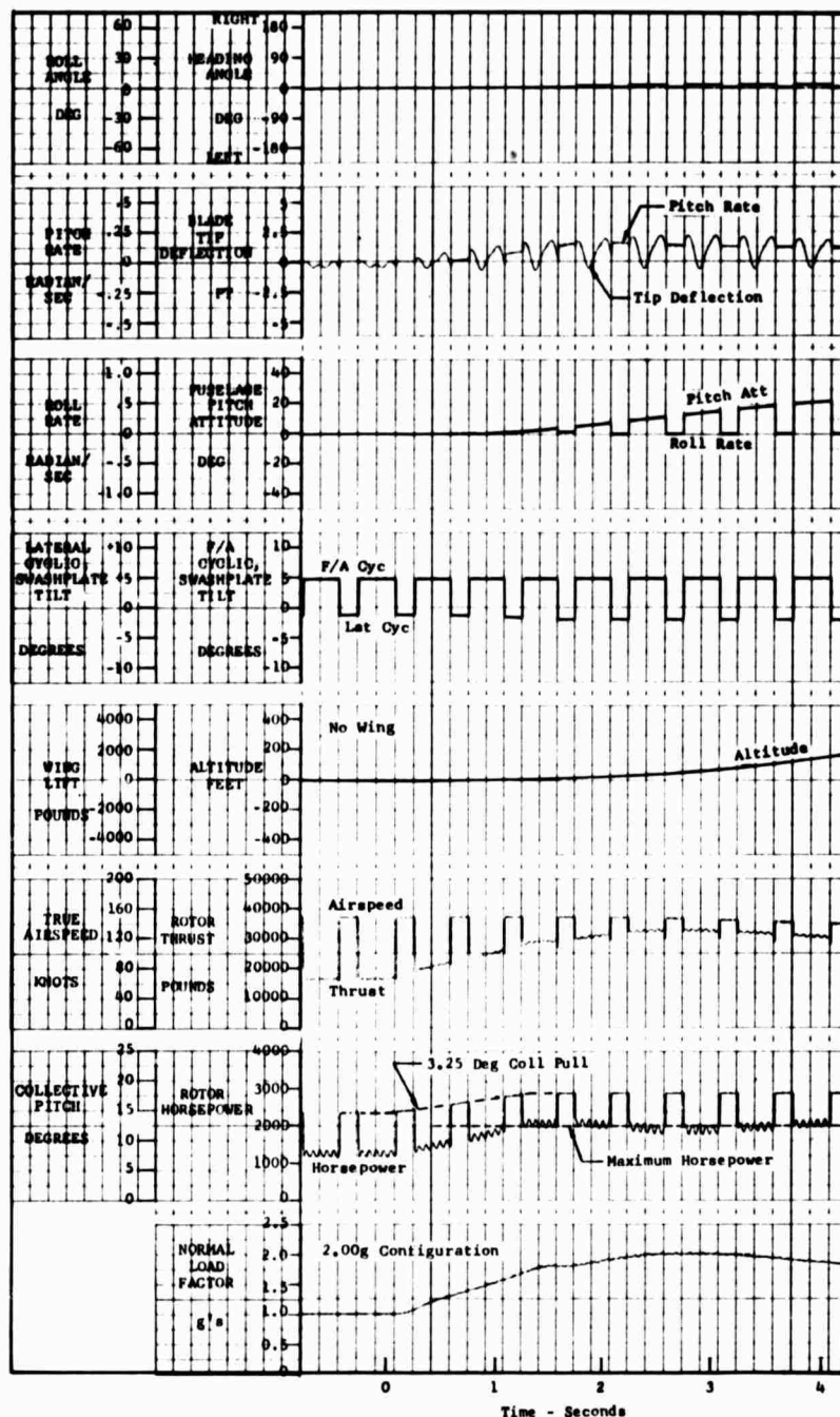
Figure 76. Maneuver Time History, 2.00g Configuration, Limiting Collective Pullup at 150 KTAS.
