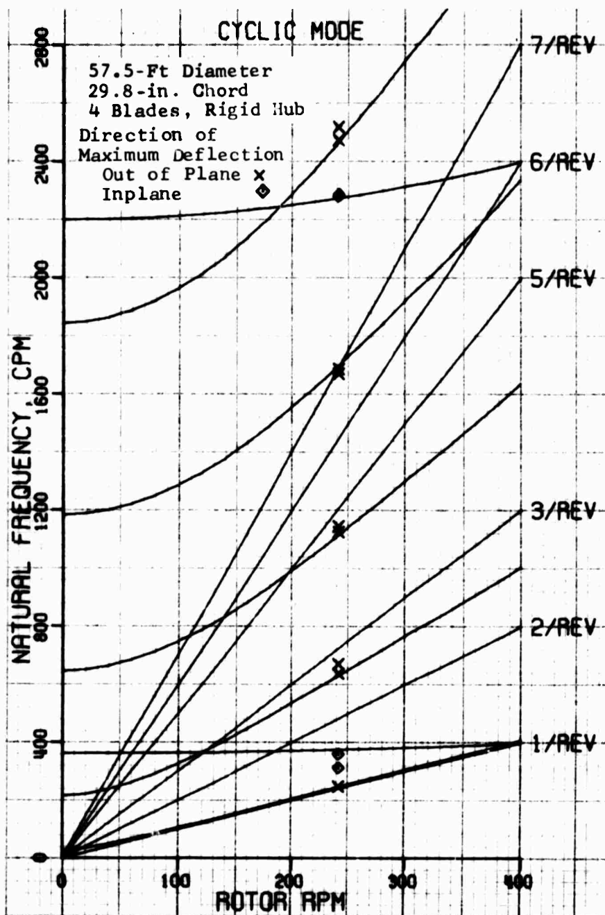
Figure 87. Cyclic Mode Frequencies for Baseline Rotor.
