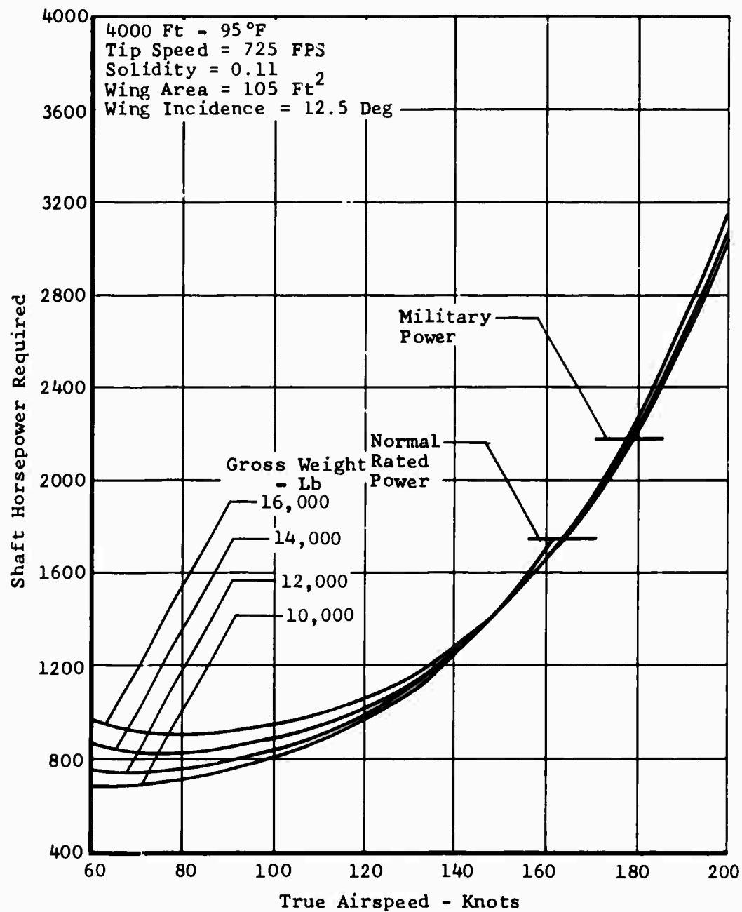
Figure 115. Task II - Winged Helicopter, Speed Power Polar.
