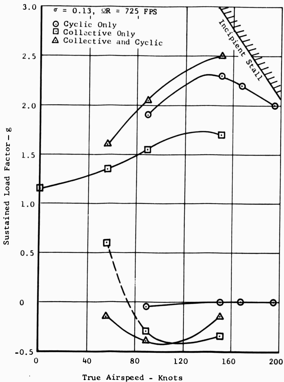
Figure 16. Task I - Maneuver Results, High Solidity Configuration.
