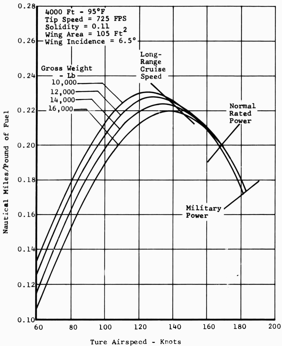
Figure 131. Task II - Winged Helicopter, Specific Range.
