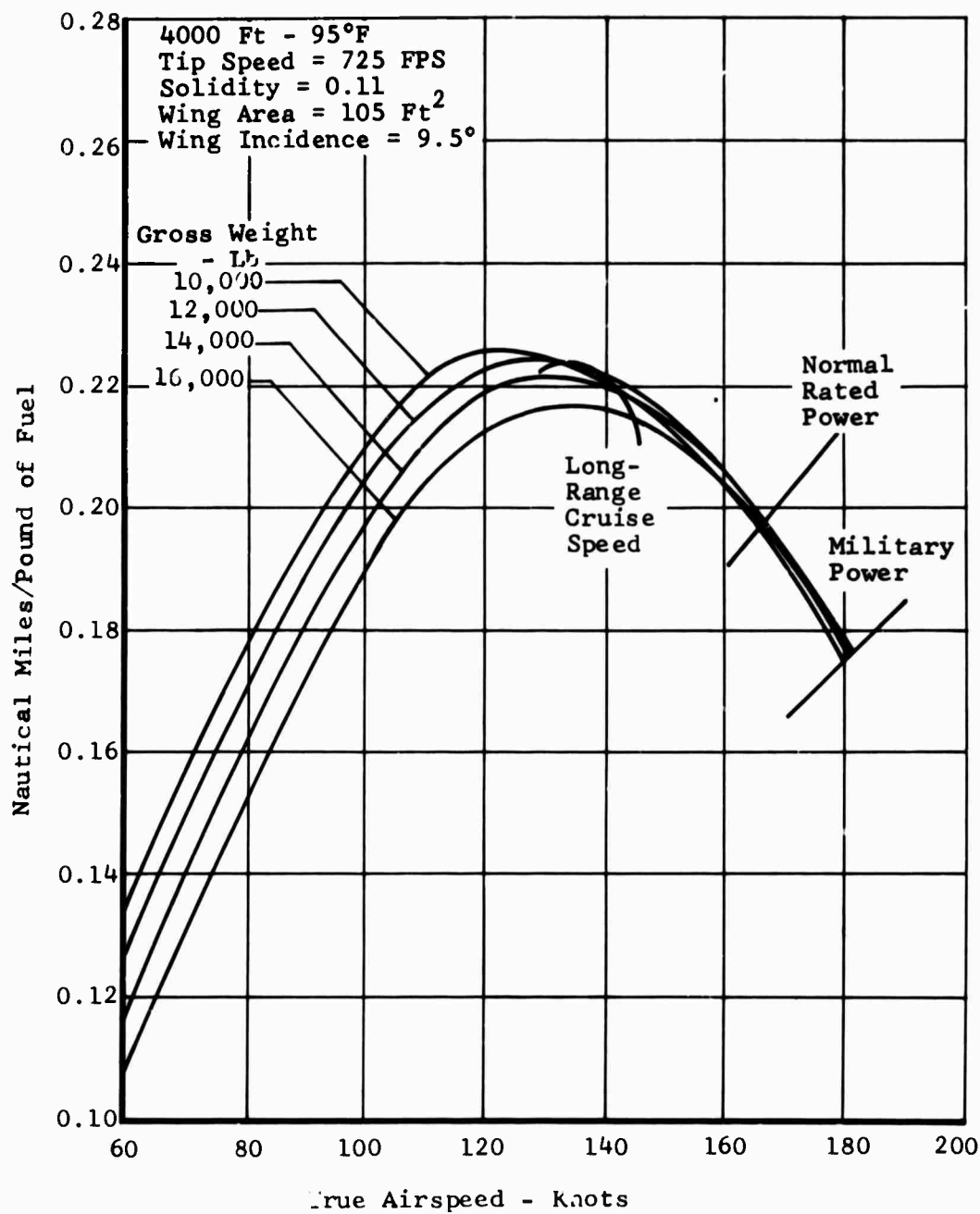
Figure 132. Task II - Winged Helicopter, Specific Range.
