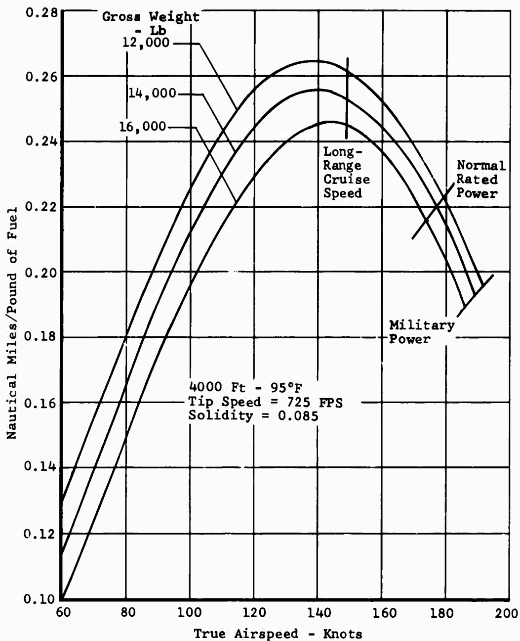
Figure 66. Task III - Wingless Helicopter, Specific Range, 1.50g Design.
