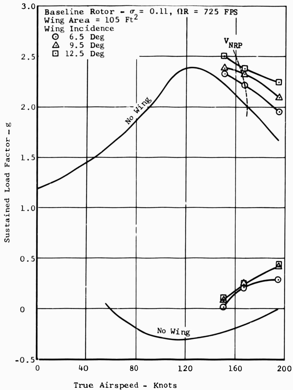
Figure 38. Task II - Maneuver Results, Baseline Rotor, Large Wing.
