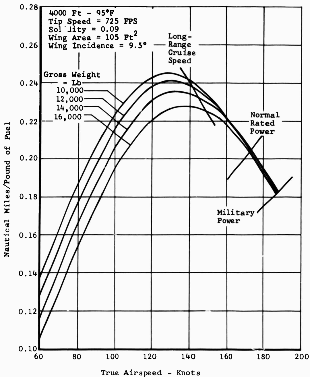
Figure 135. Task II - Winged Helicopter, Specific Range.
