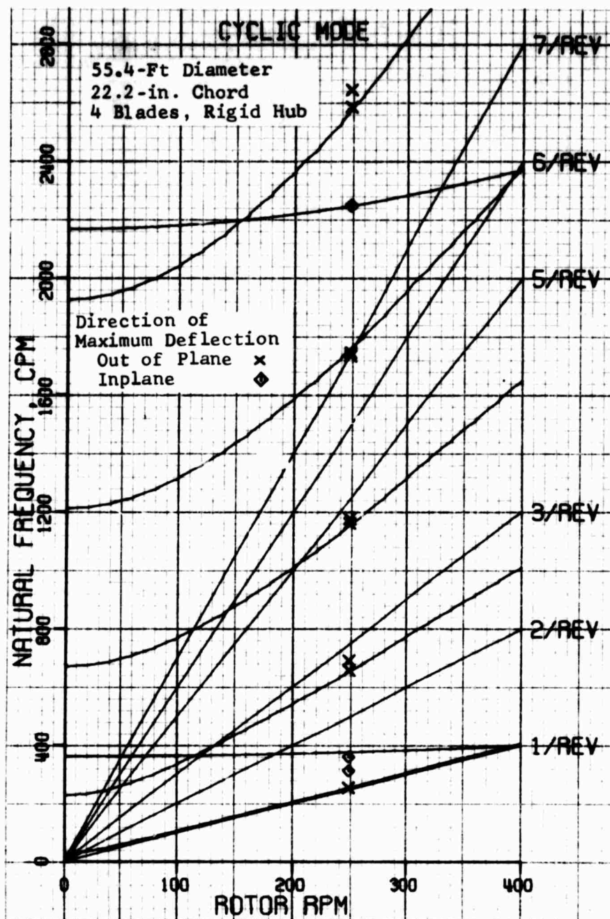
Figure 90. Cyclic Mode Frequencies for Alternate Rotor.
