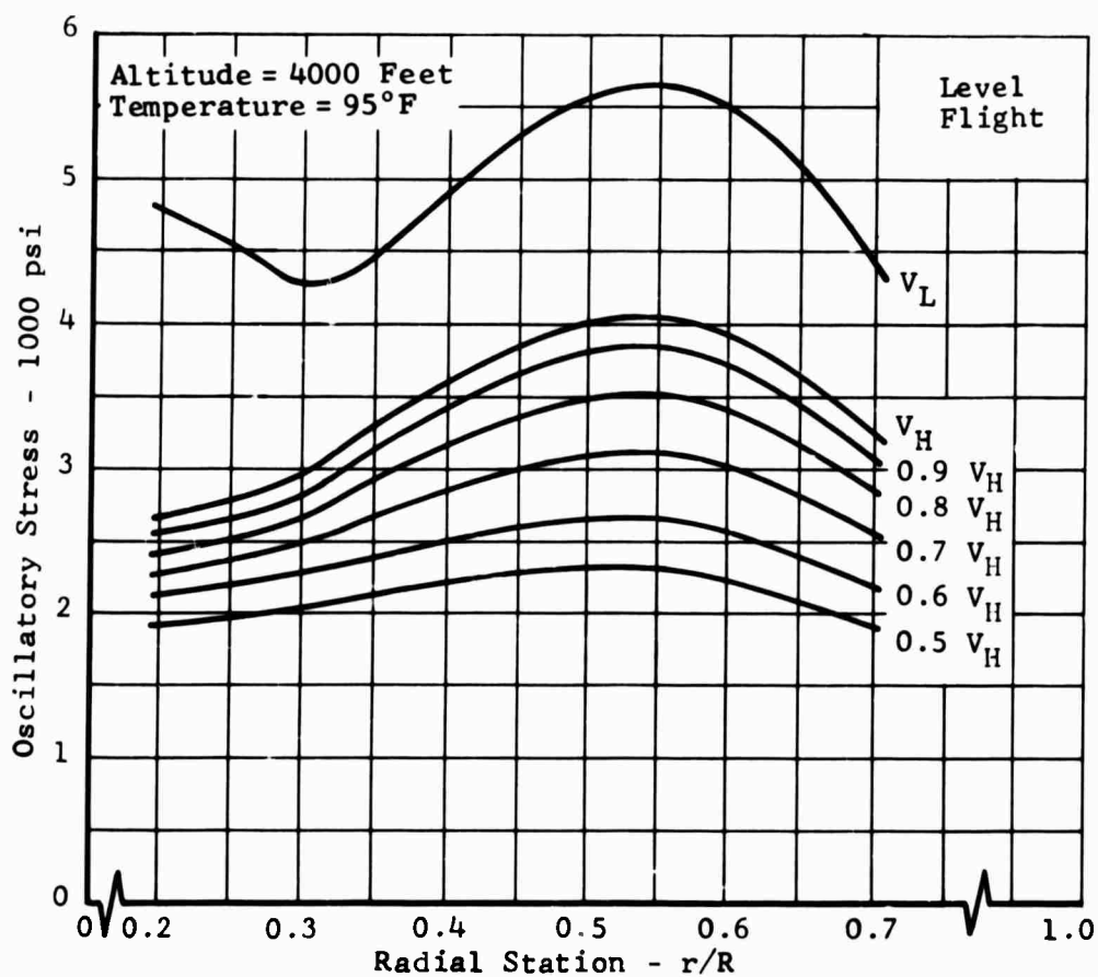
Figure 88. Oscillatory Stress Distributions for Baseline Rotor.
