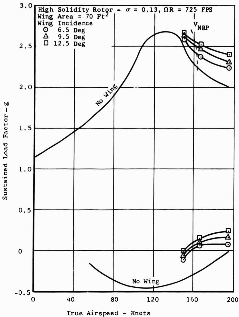
Figure 41. Task II - Maneuver Results, High Solidity Rotor, Small Wing.
