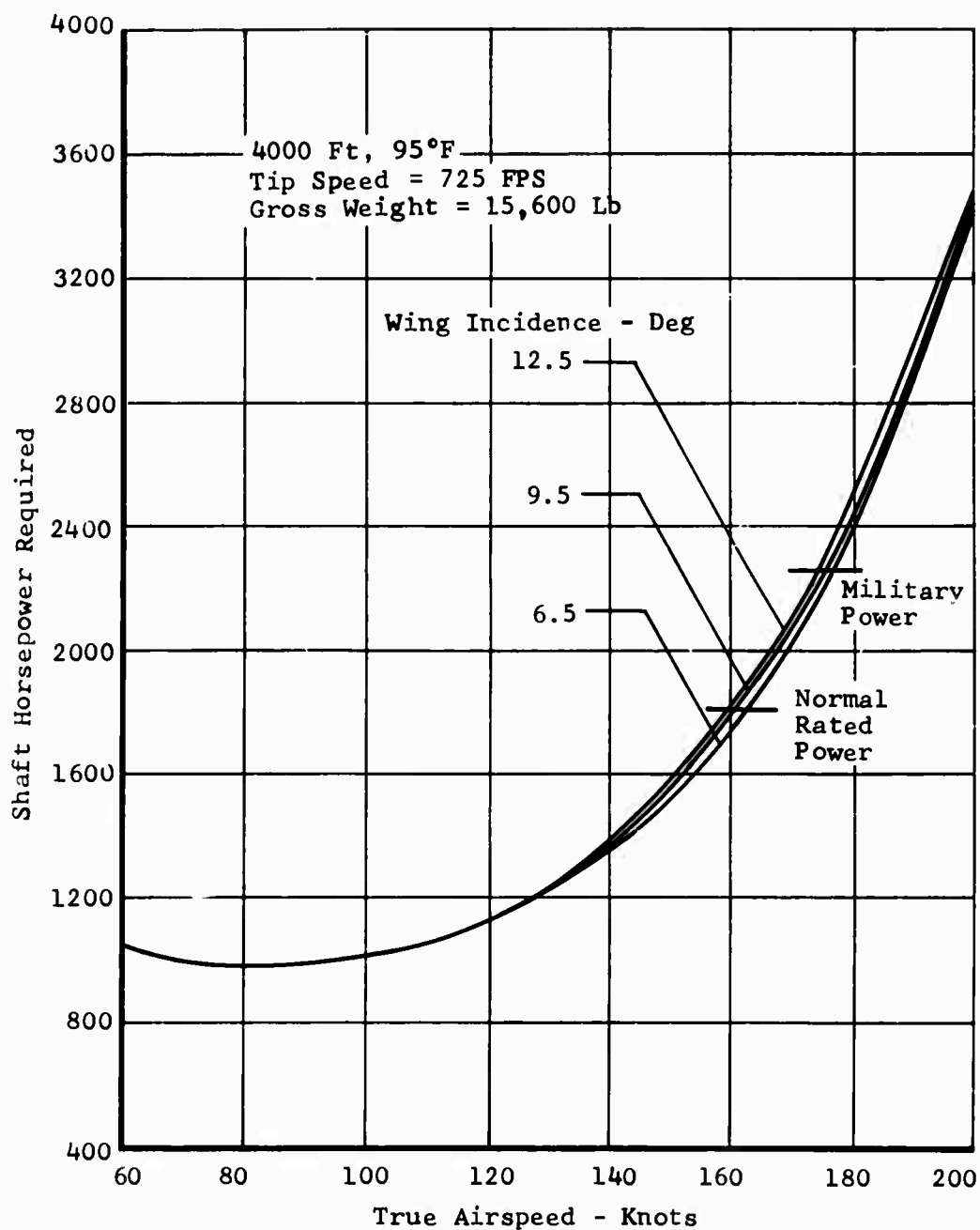
Figure 30. Task II - Winged Helicopter Speed Power Polar, Solidity = 0.13, Wing Area = 70 Ft 2 .
