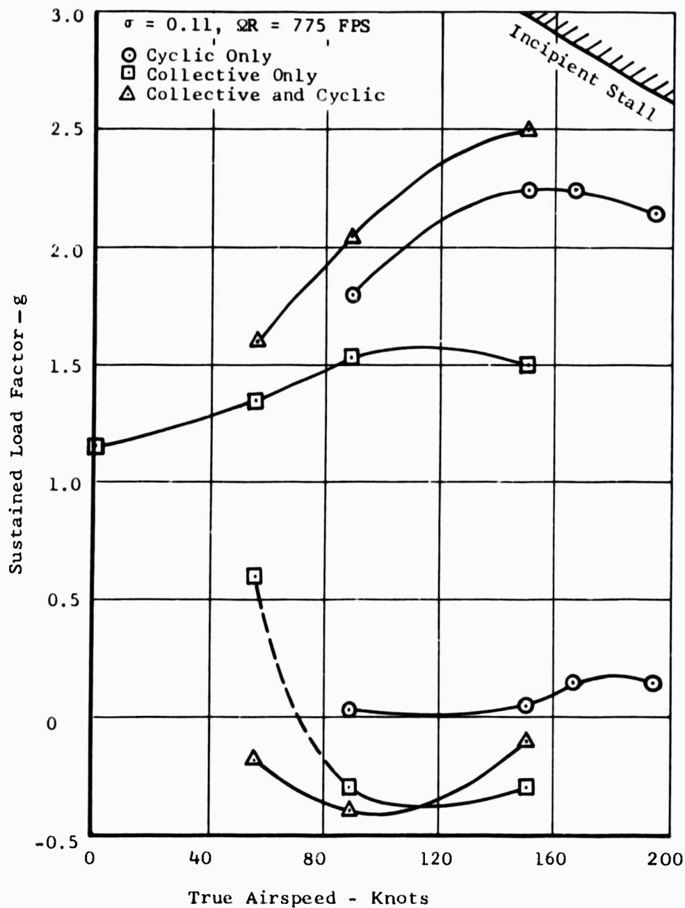
Figure 14. Task I - Maneuver Results, High Tip Speed Configuration.
