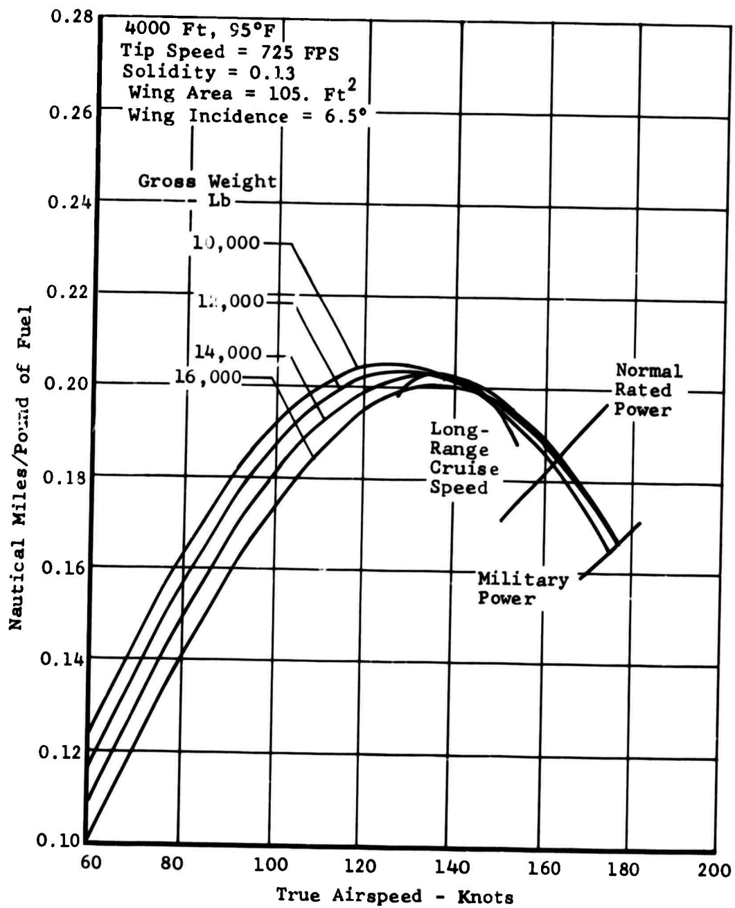
Figure 137. Task II - Winged Helicopter, Specific Range.
