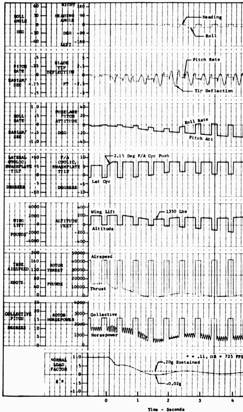
Figure 47. Maneuver Time History, F/A Cyclic Pushover, Baseline Rotor, Small Wing, Maneuver Limited by Flapping.
