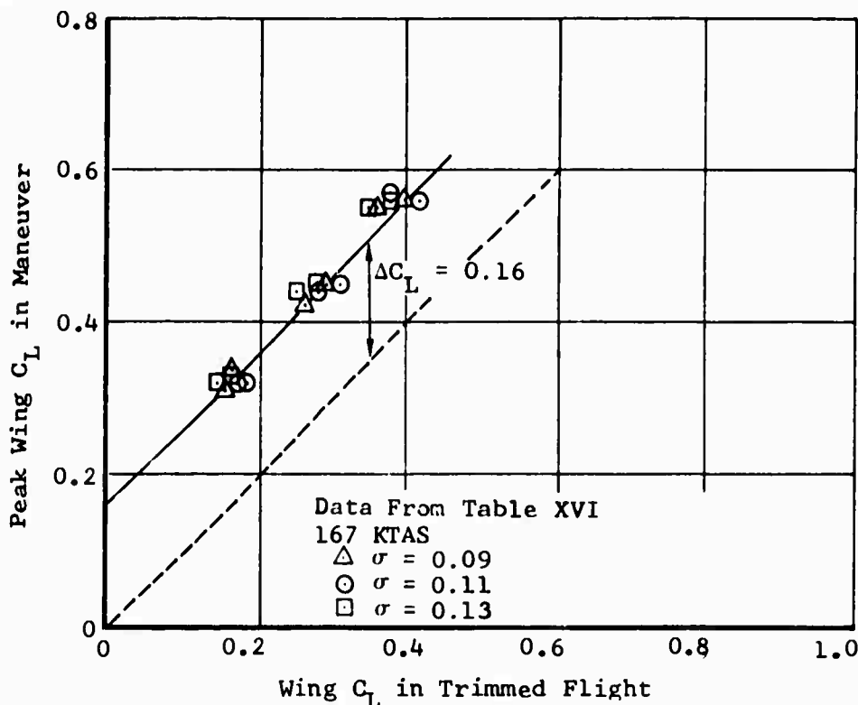
Figure 49. Relationship of Wing C_L in Trimmed Flight to Peak Wing C_L in Pullup Maneuver.
