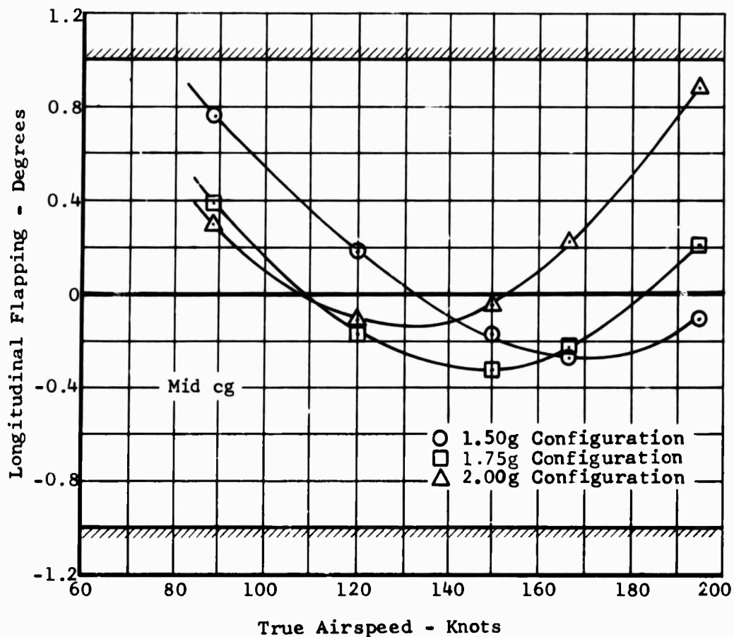
Figure 56. Task III Configurations - Longitudinal Flapping Versus Airspeed.
