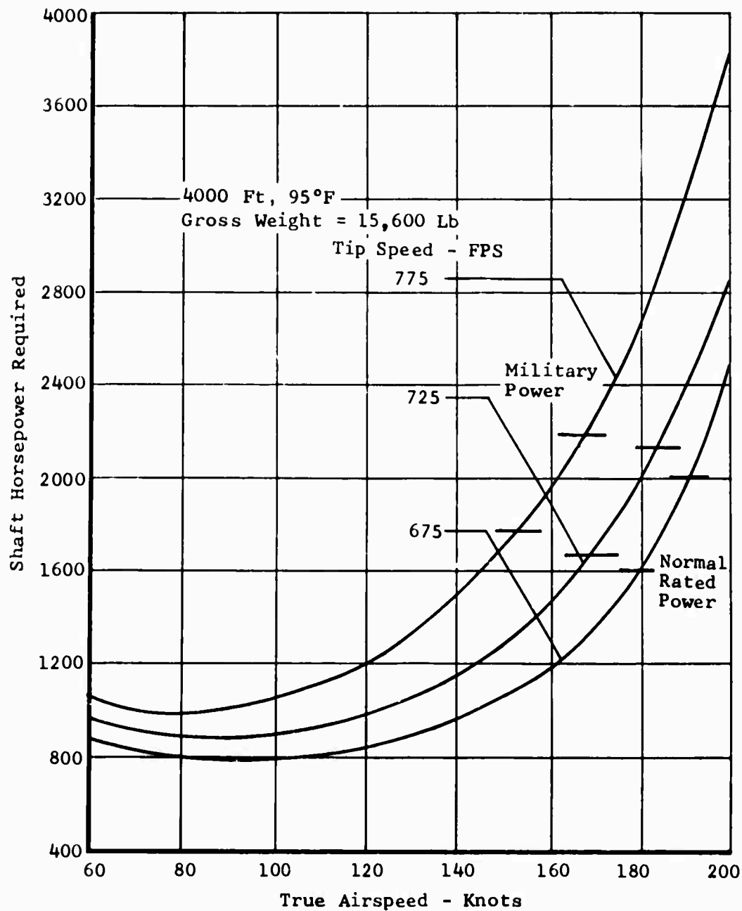
Figure 4. Task I - Wingless Helicopter, Speed Power Polar, Solidity = 0.11.
