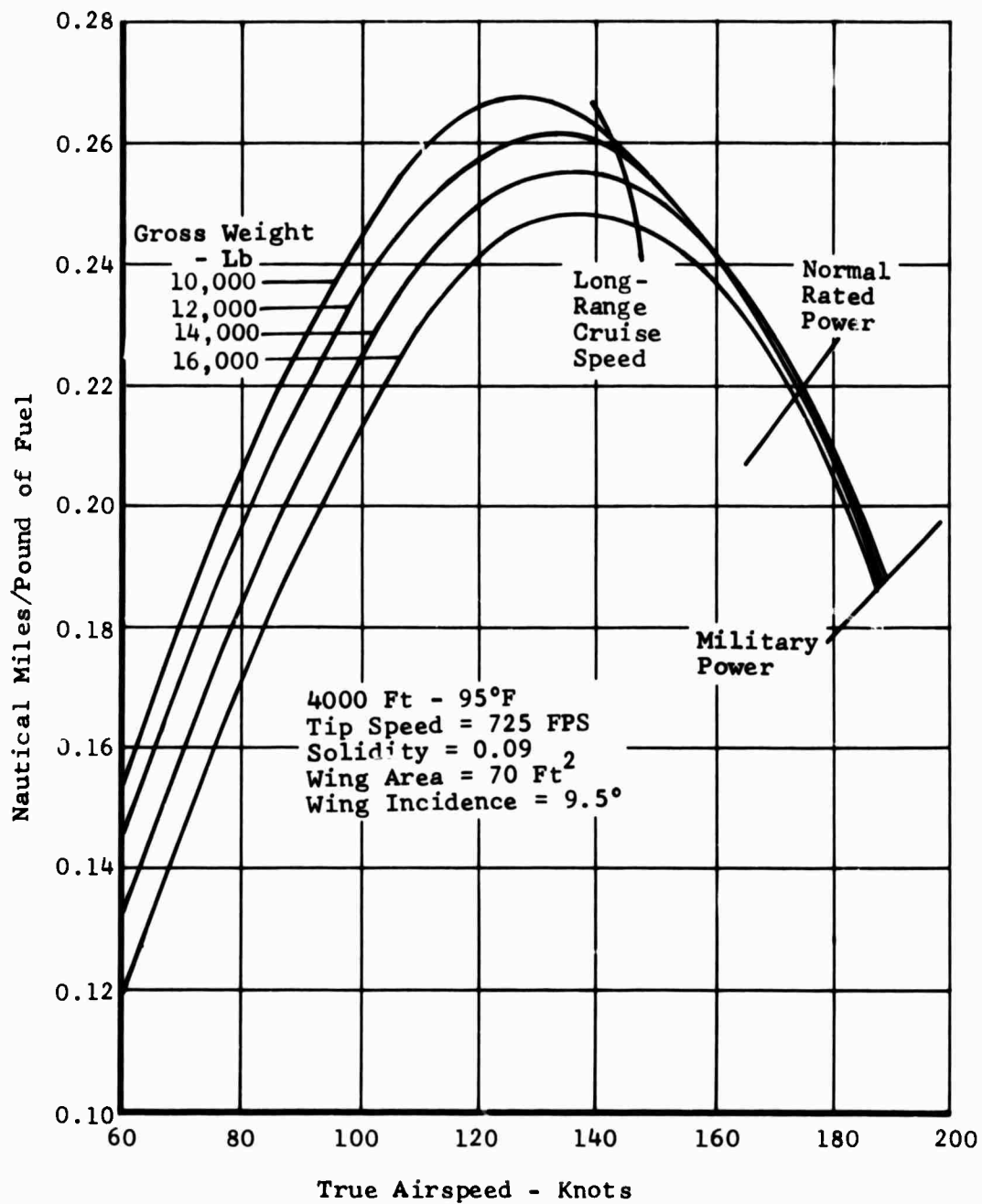
Figure 126. Task II - Winged Helicopter, Specific Range.
