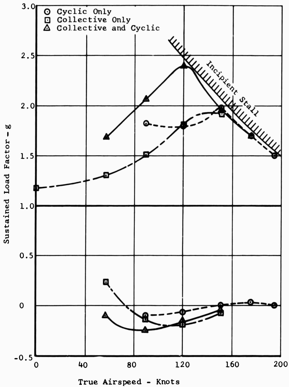
Figure 70. Task III - Maneuver Results, 1.75g Design.
