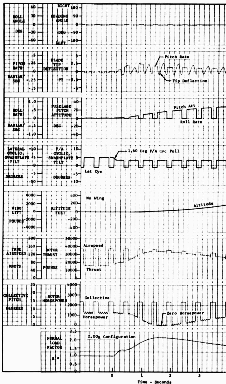
Figure 75. Maneuver Time History, 2.00g Configuration, Limiting Cyclic Pullup at 150 KTAS.
