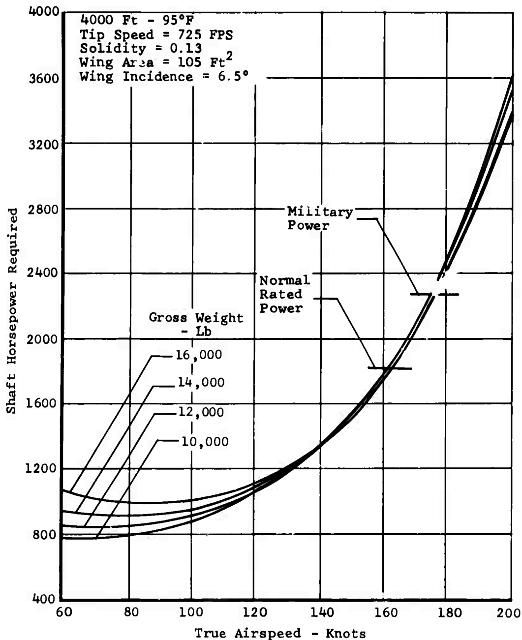
Figure 119. Task II - Winged Helicopter, Speed Power Polar.
