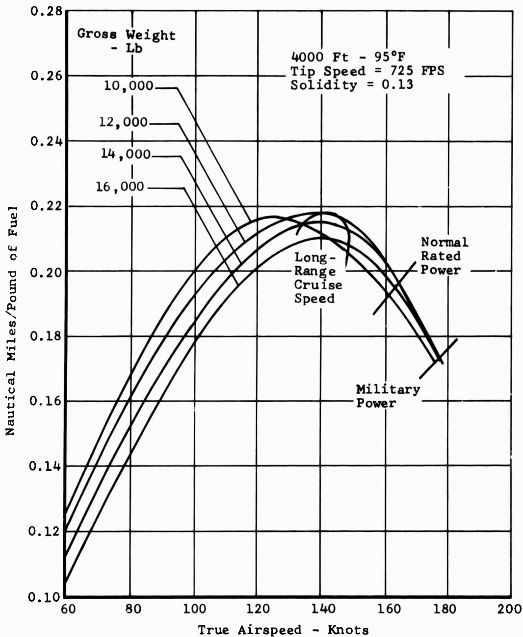
Figure 101. Task I - Wingless Helicopter, Specific Range.
