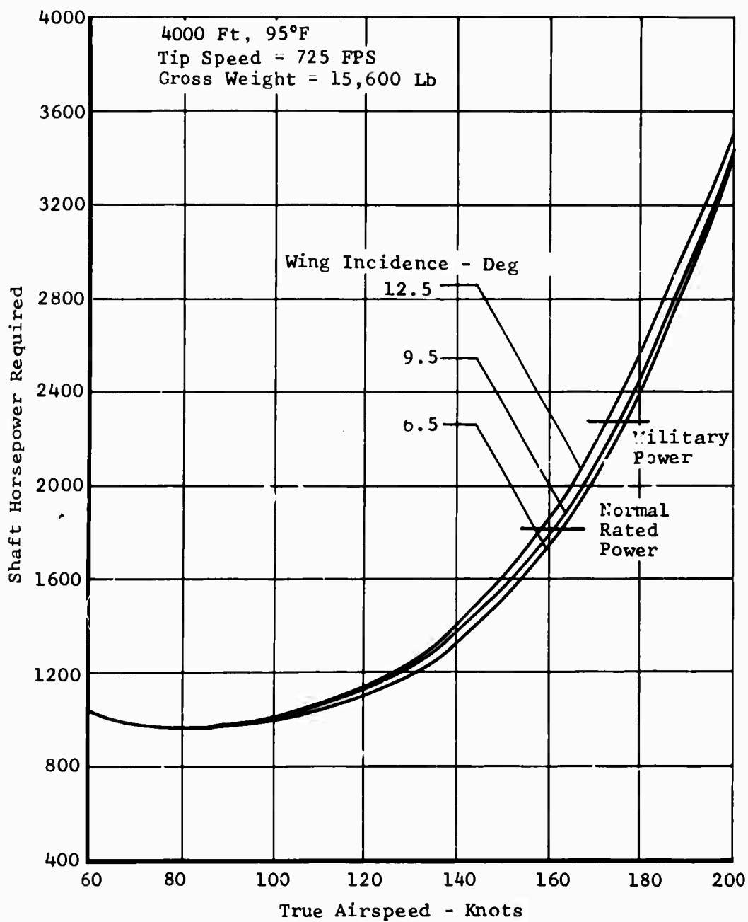
Figure 33. Task II - Winged Helicopter, Speed Power Polar, Solidity = 0.13, Wing Area = 105 Ft 2 .
