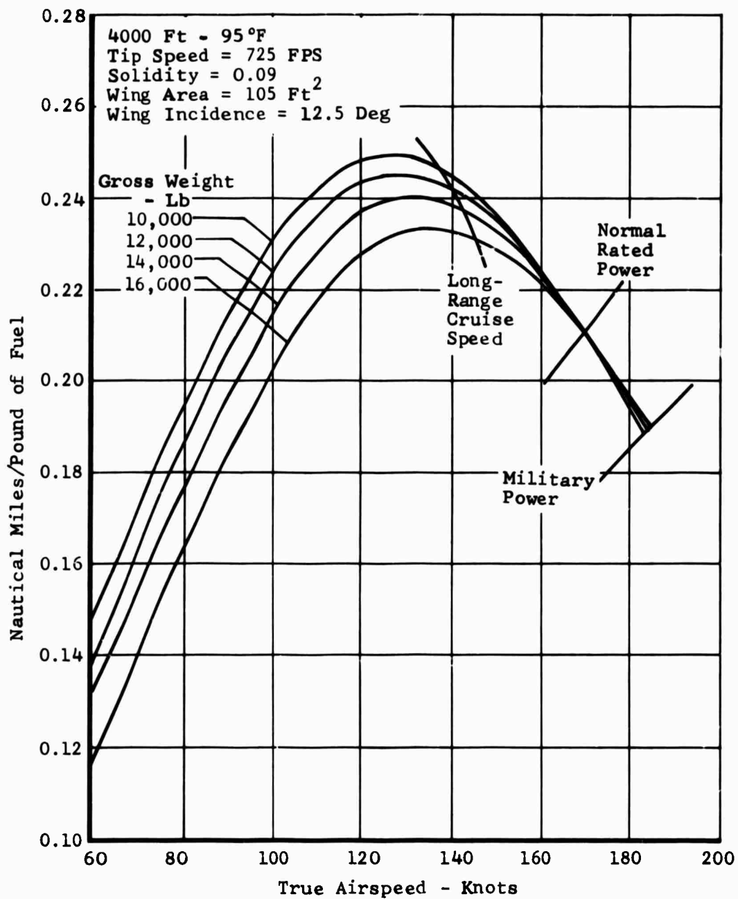
Figure 136. Task II - Winged Helicopter, Specific Range.
