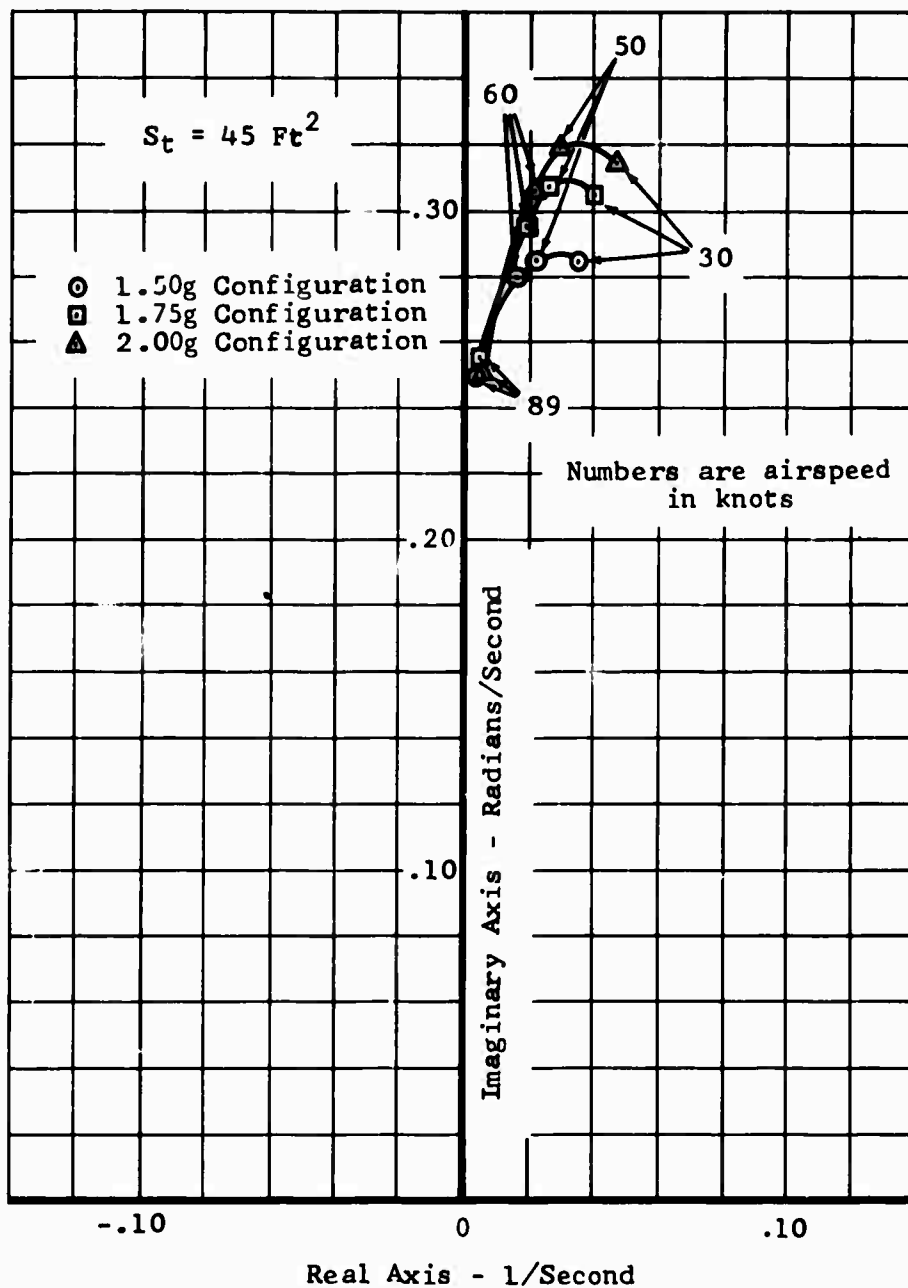
Figure 60. Task III Configuration-Phugoid Mode Root Locus Plot, aft cg.
