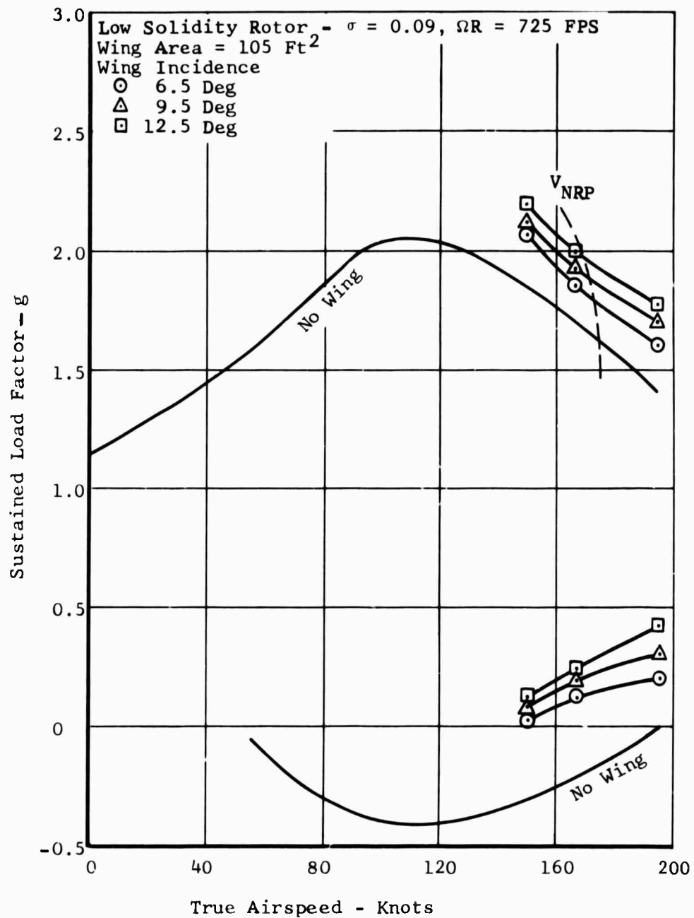
Figure 40. Task II - Maneuver Results, Low Solidity Rotor, Large Wing.
