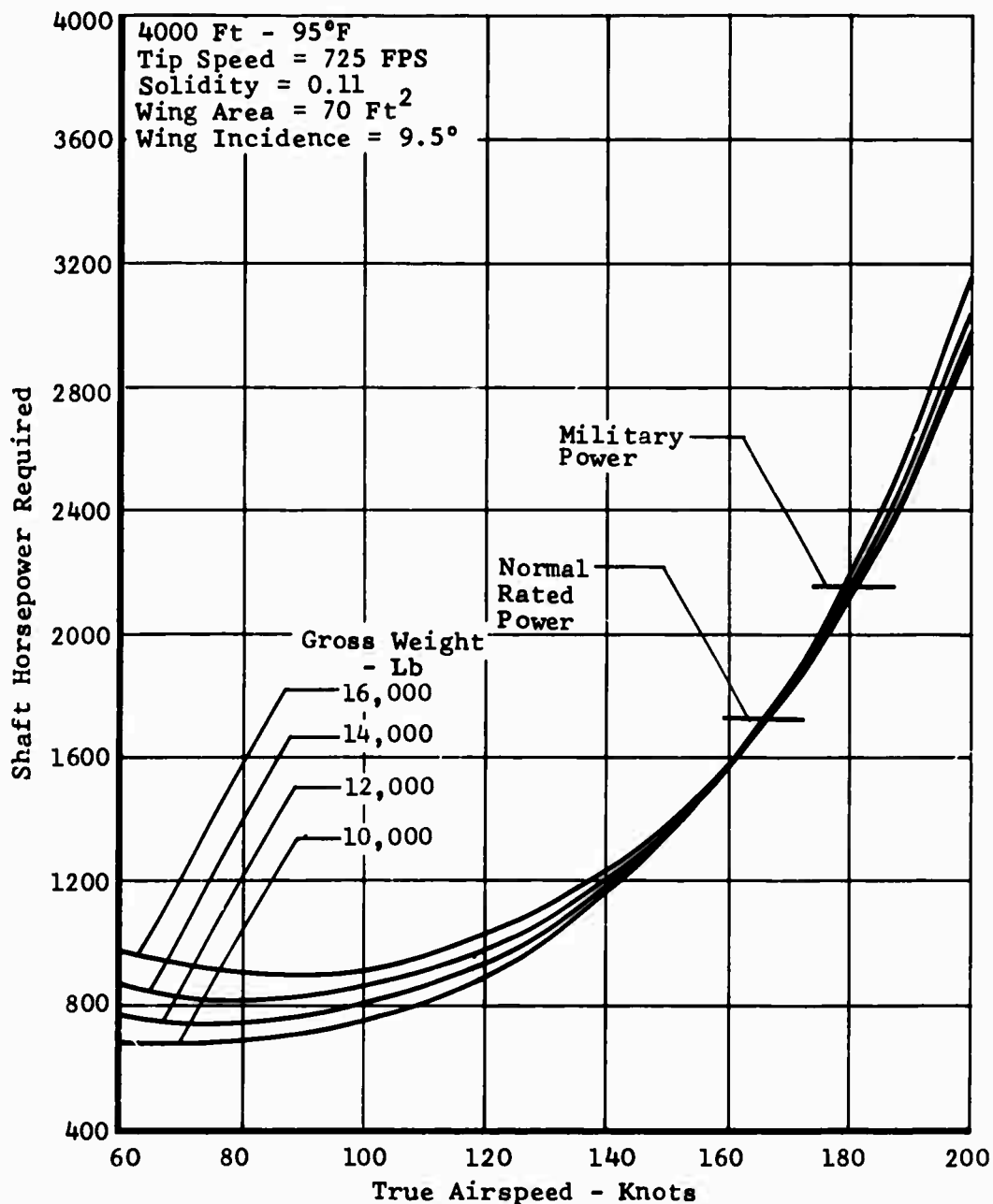
Figure 105. Task II - Winged Helicopter, Speed Power Polar.
