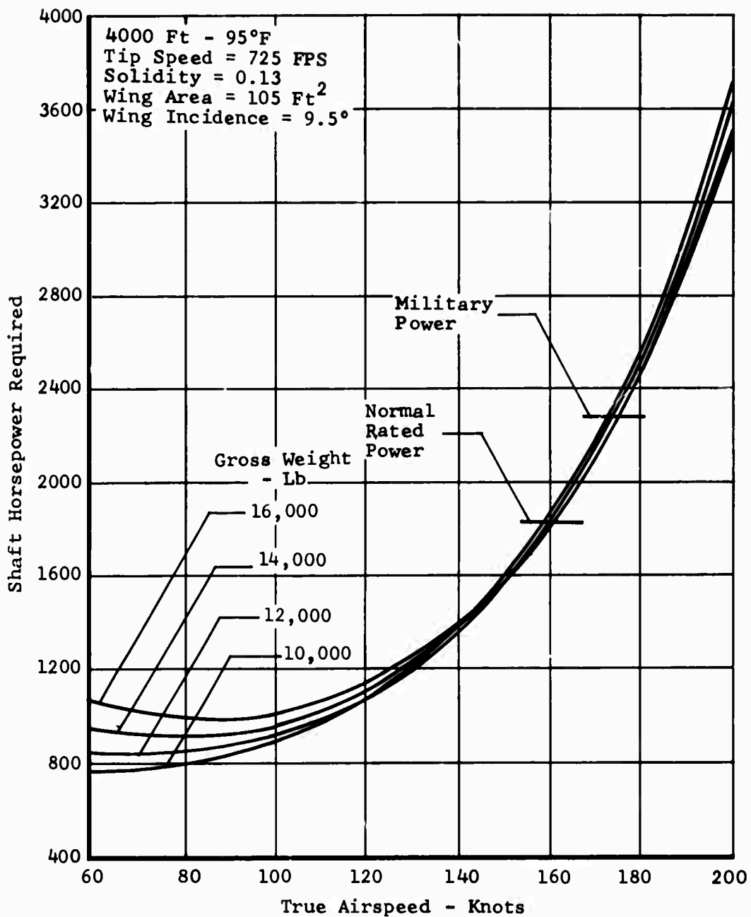
Figure 120. Task II - Winged Helicopter, Speed Power Polar.
