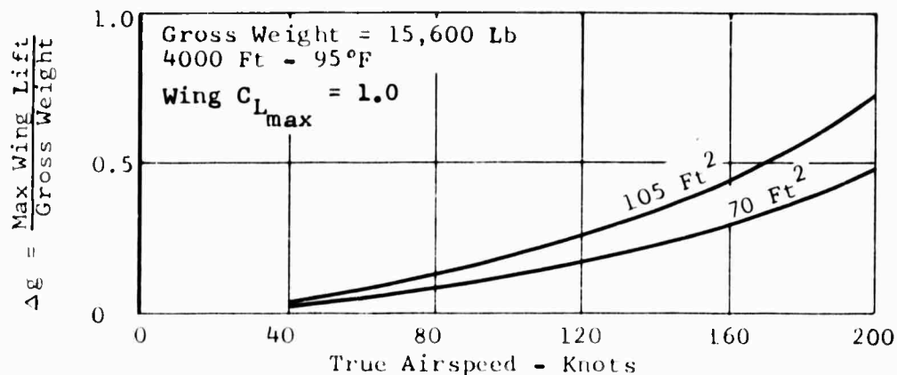
Figure 36. Potential Increase in Load Factor, Wing at Maximum Lift.
