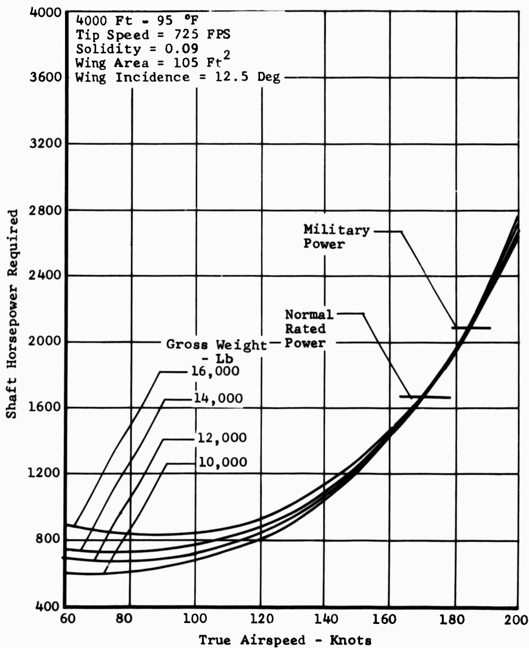
Figure 118. Task II - Winged Helicopter, Speed Power Polar.
