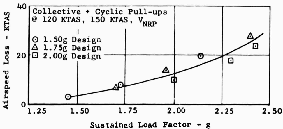
Figure 79. Task III Configurations, Airspeed Loss in Pullup Maneuvers After Three Seconds.
