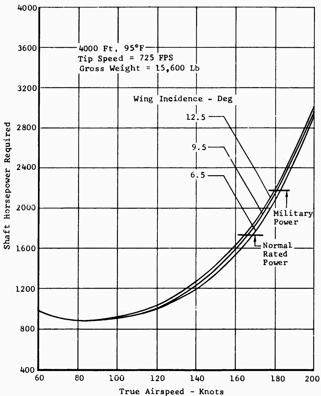
Figure 28. Task II - Winged Helicopter, Speed Power Polar, Solidity = 0.11, Wing Area = 70 Ft 2 .
