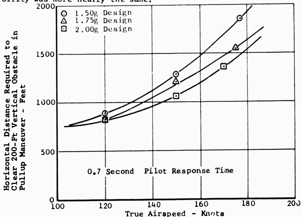
Figure 80. Effect of Design g-Capability on Distance Required to Clear 200-Foot Obstacle.
