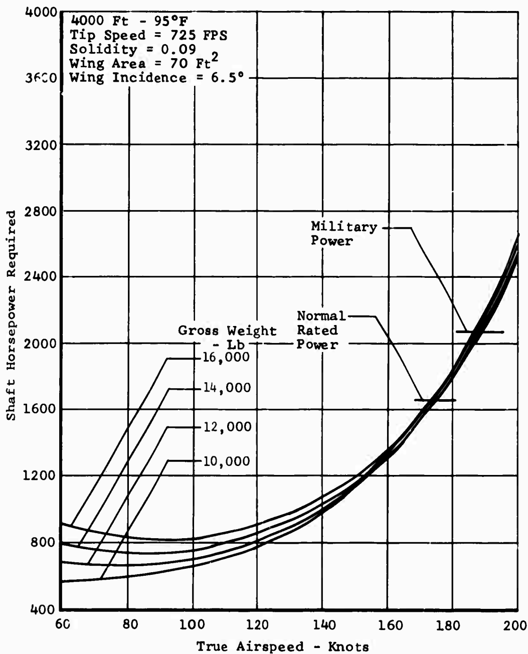
Figure 107. Task II - Winged Helicopter, Speed Power Polar.
