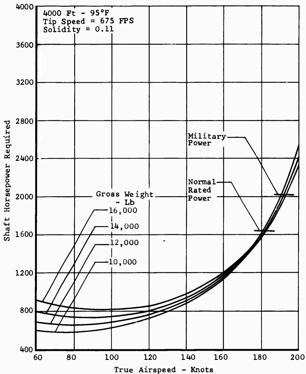
Figure 97. Task I - Wingless Helicopter, Speed Power Polar.
