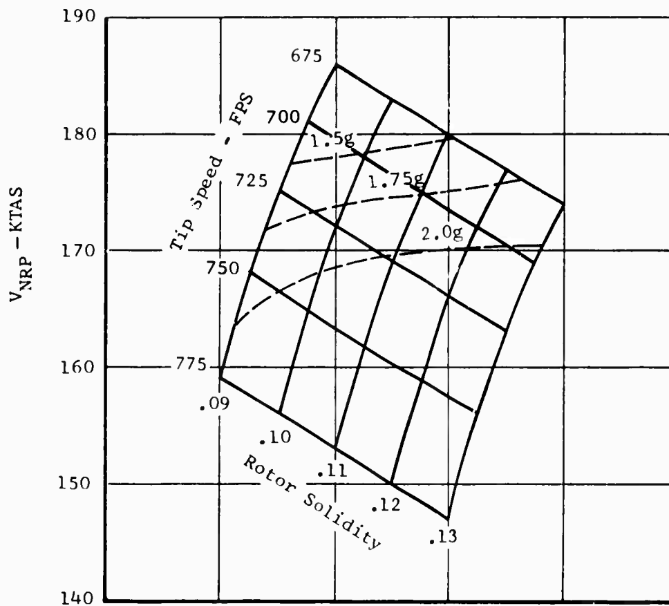
Figure 20. Effects of Rotor Solidity and Tip Speed on V_{NRP} and Design g-Capability.
