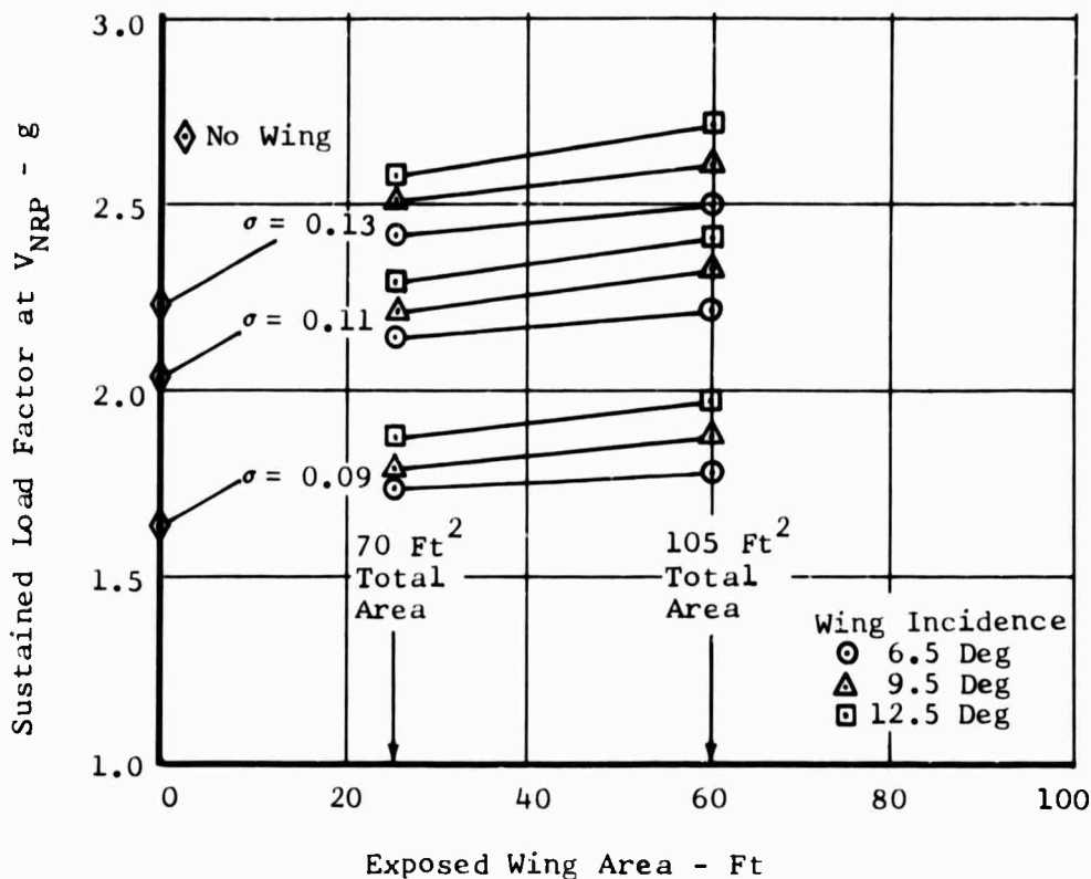
Figure 51. Effects of Wing Area on Load Factor Capability at V_{NRP} .
