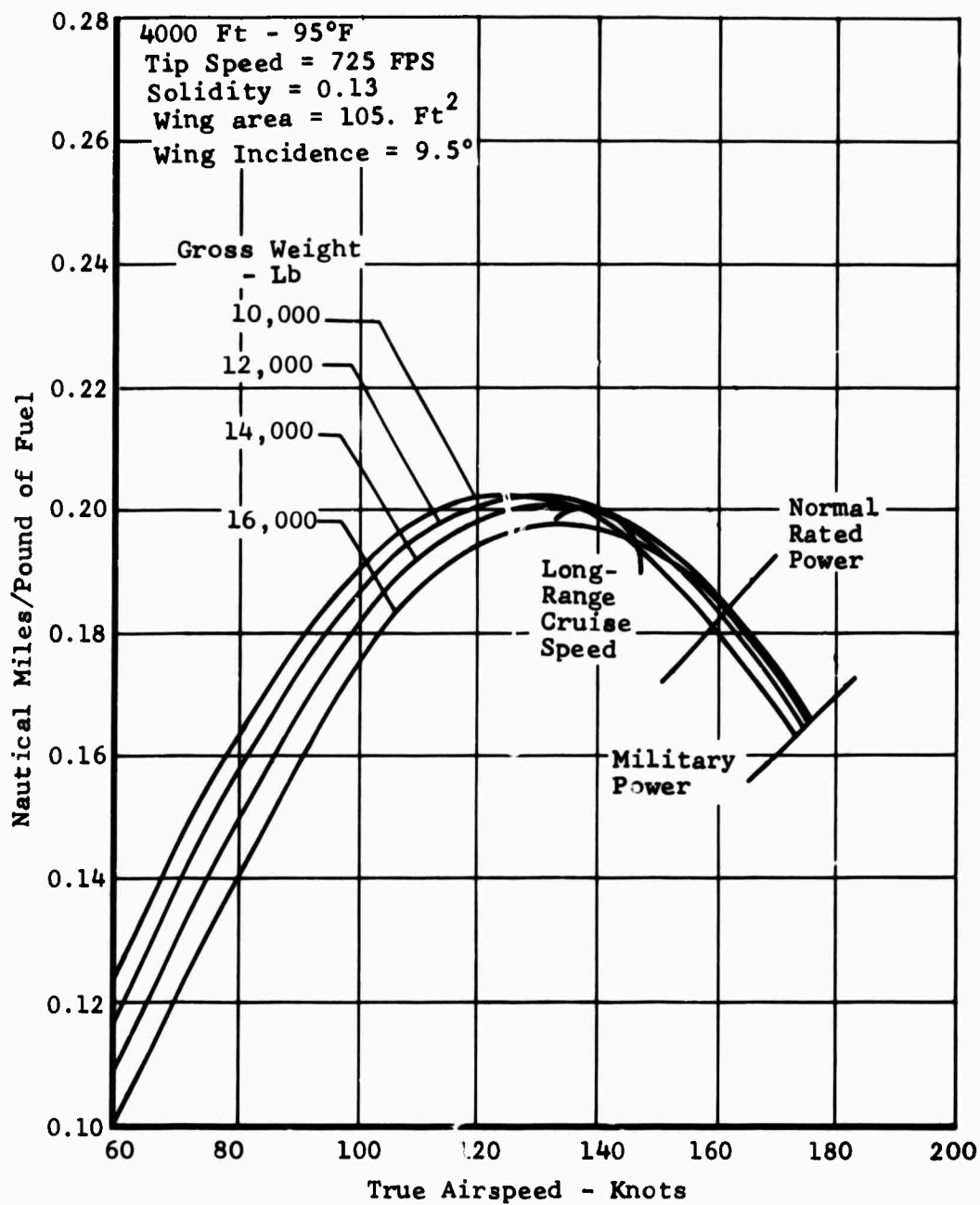
Figure 138. Task II - Winged Helicopter, Specific Range.
