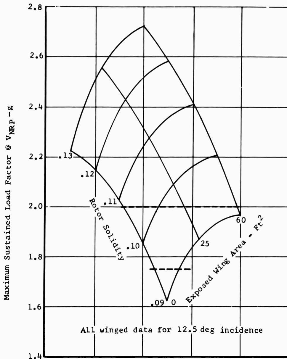
Figure 52. Effects of Rotor Solidity and Wing Area on g-Capability at V_{NRP} .
