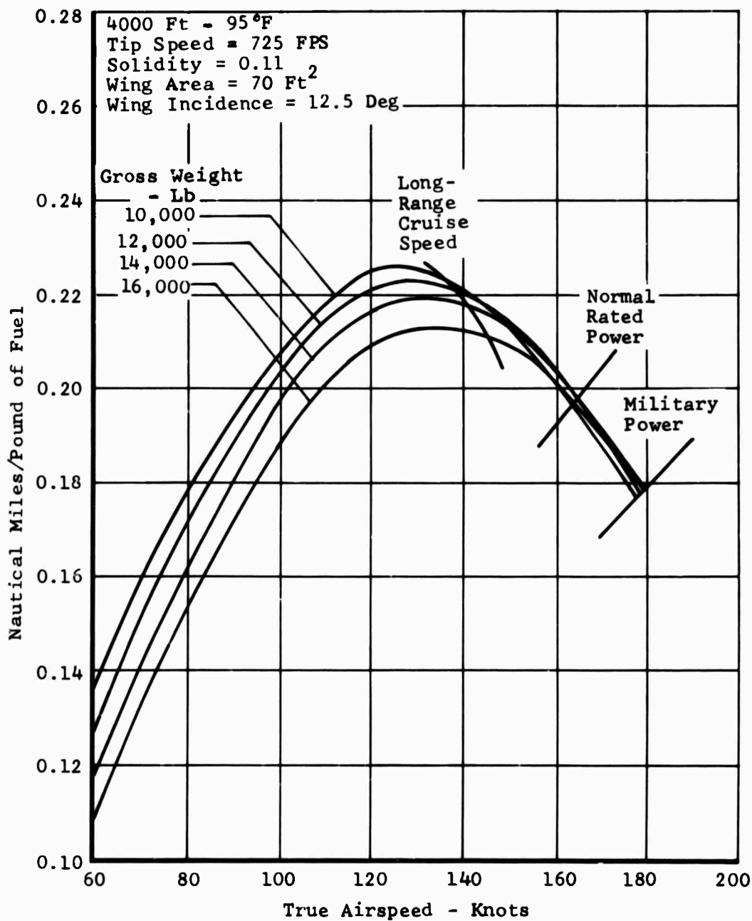
Figure 124. Task II - Winged Helicopter, Specific Range.
