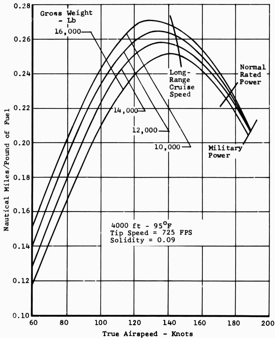
Figure 100. Task I - Wingless Helicopter, Specific Range.
