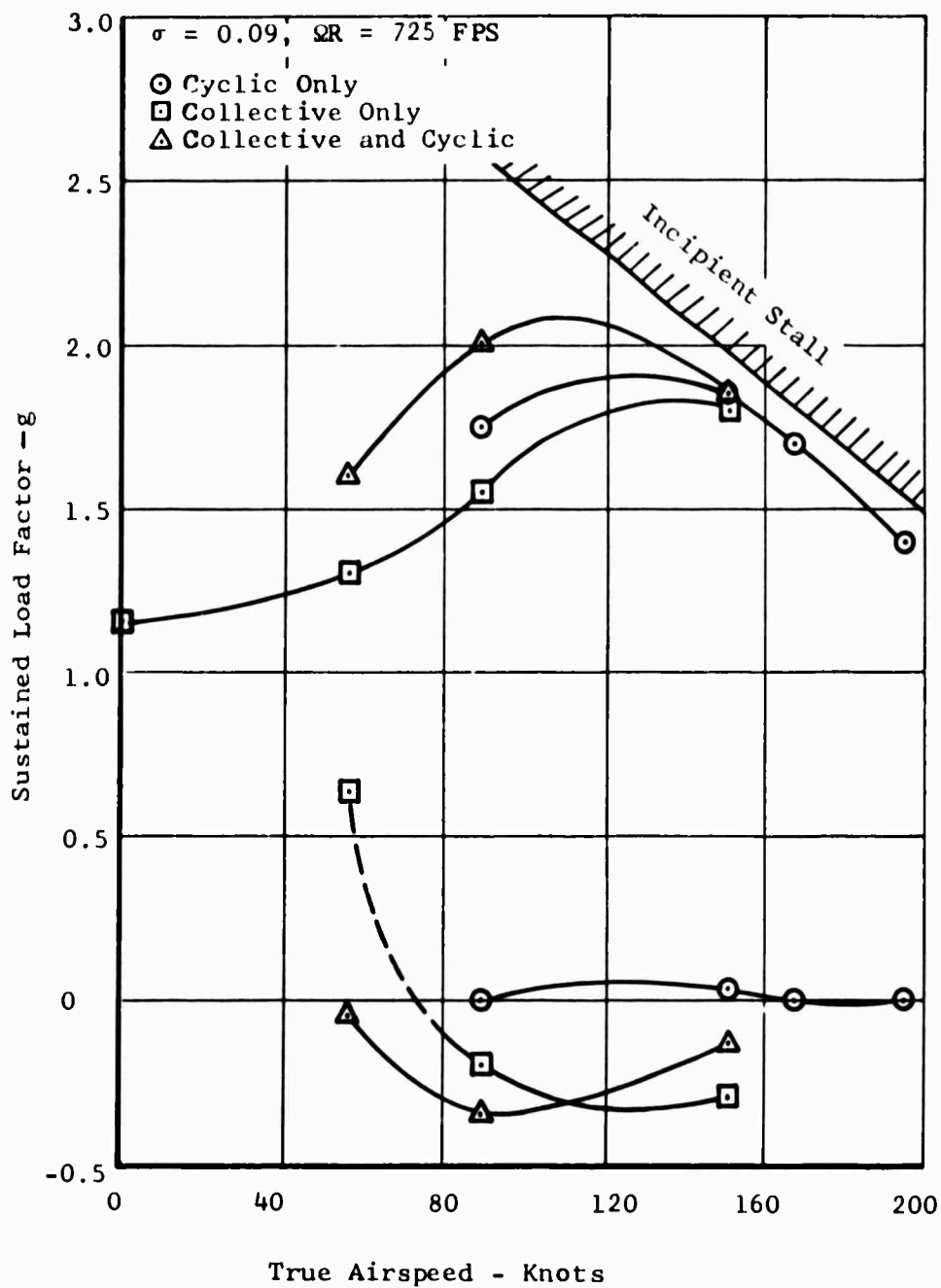
Figure 15. Task I - Maneuver Results, Low Solidity Configuration.
