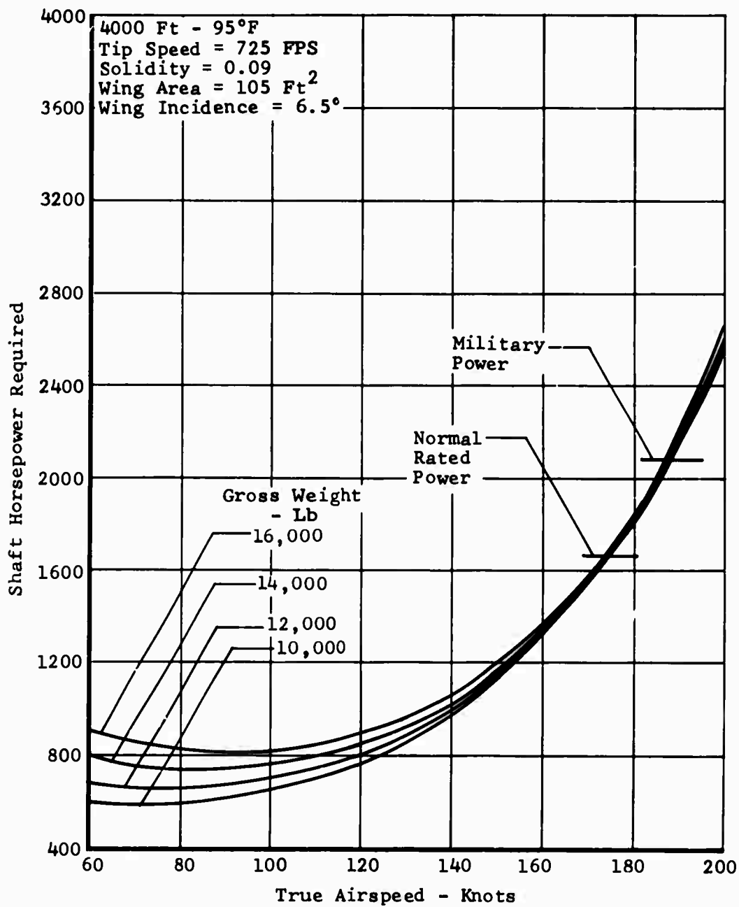
Figure 116. Task II - Winged Helicopter, Speed Power Polar.
