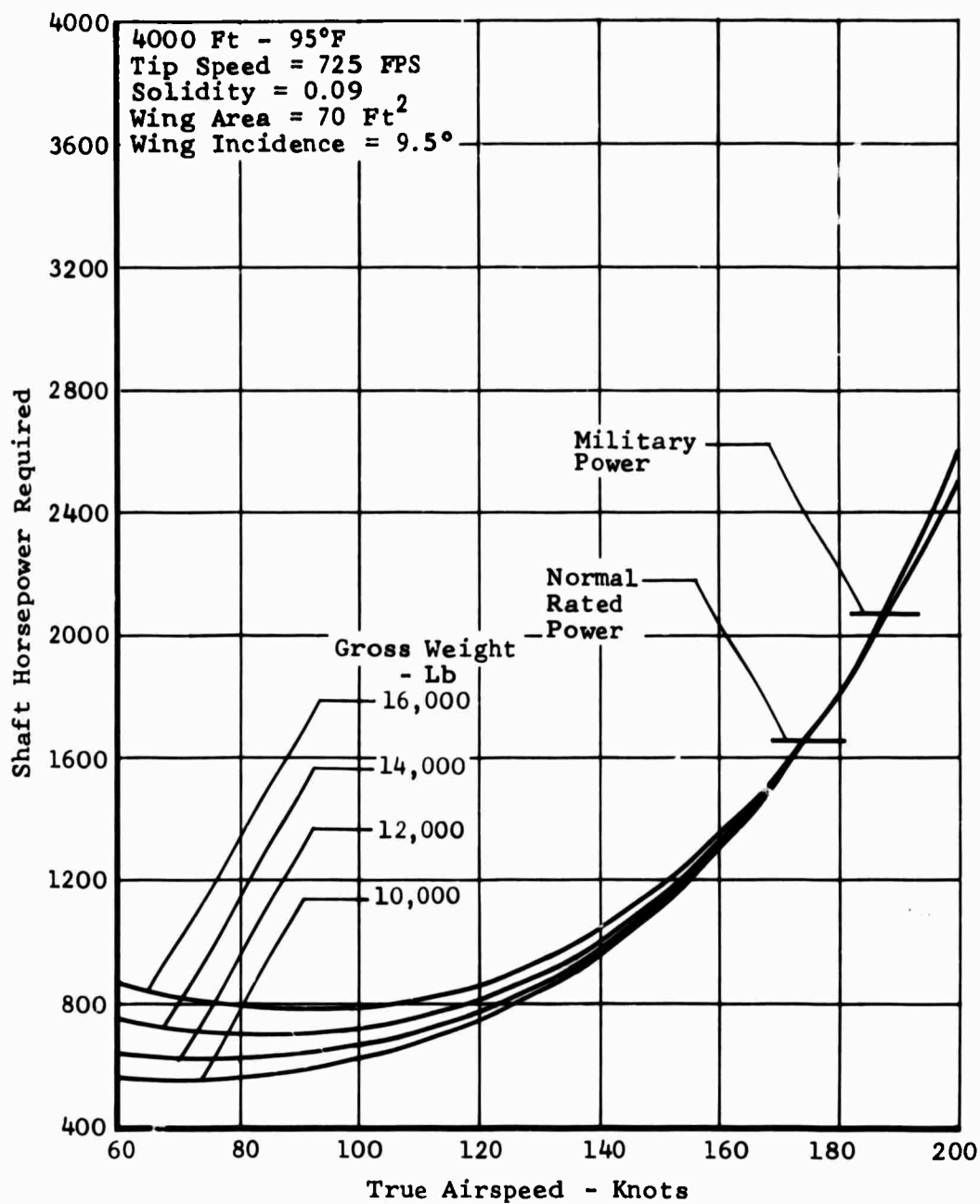
Figure 108. Task II - Winged Helicopter, Speed Power Polar.
