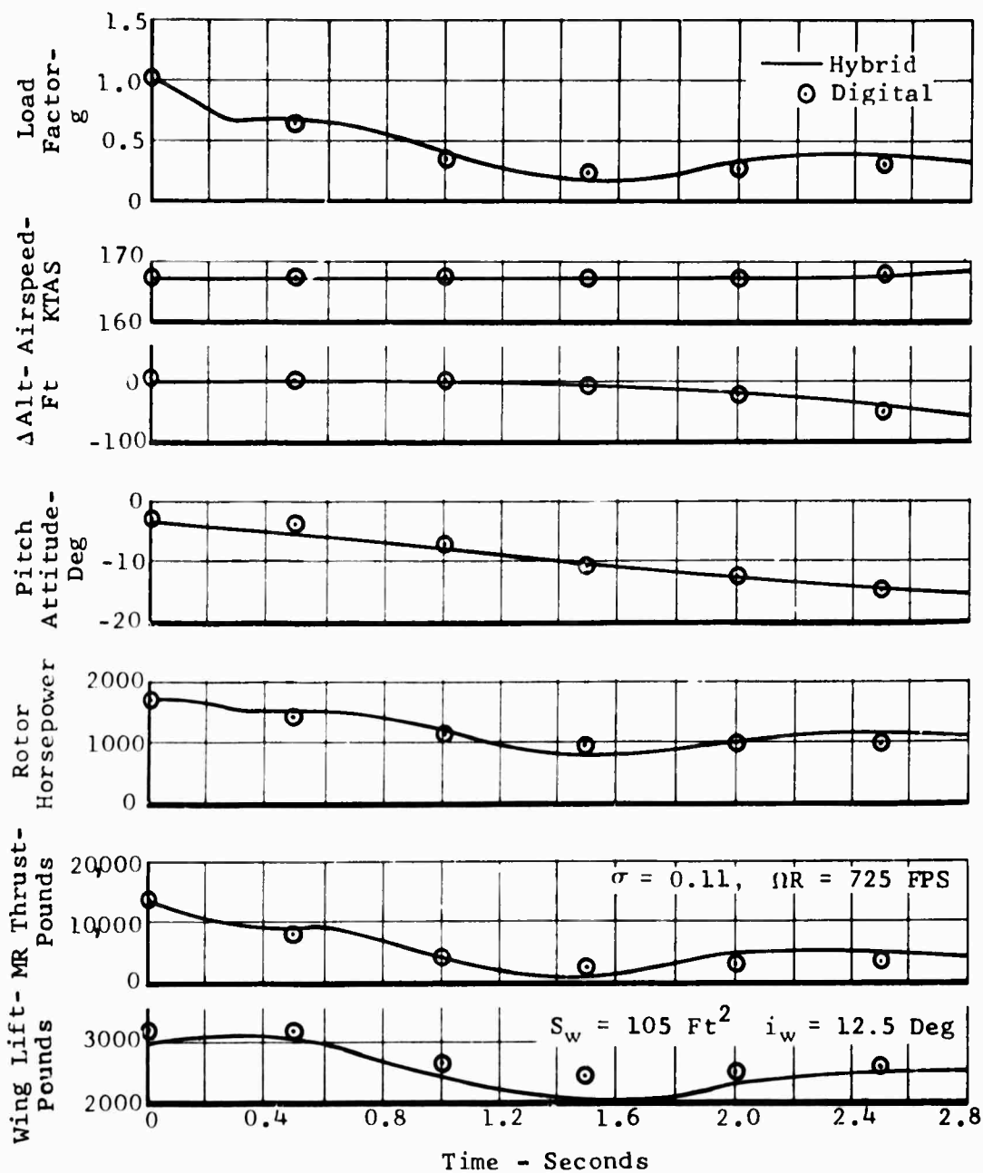
Figure 35. Comparison of Hybrid and Digital Maneuver, Baseline Rotor - Winged Configuration, 1.75-Degree Cyclic Pushover at 167 KTAS.
