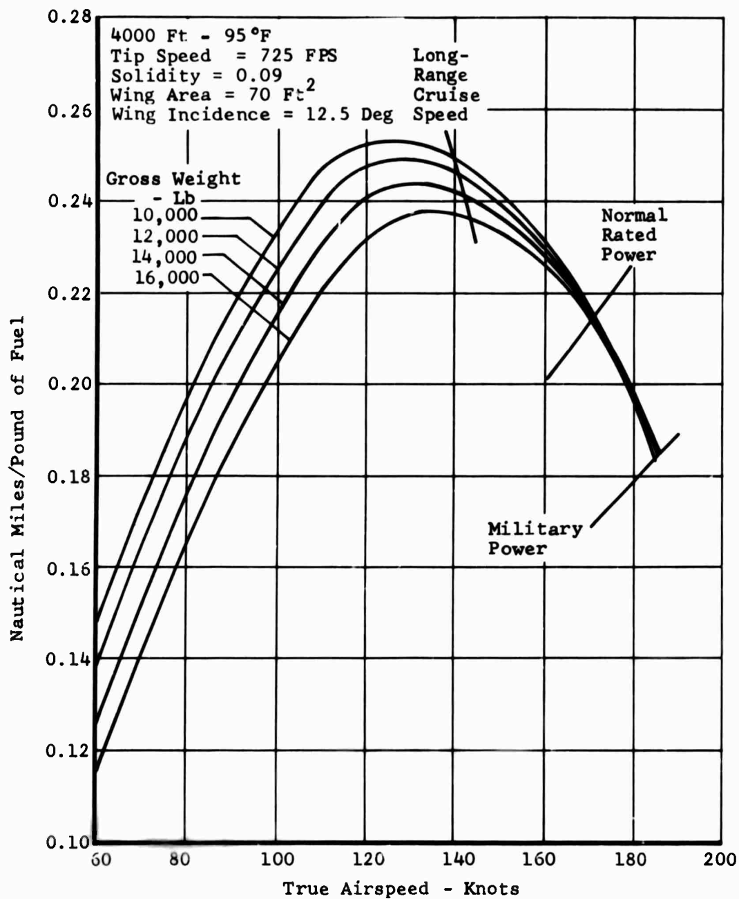
Figure 127. Task II - Winged Helicopter, Specific Range.
