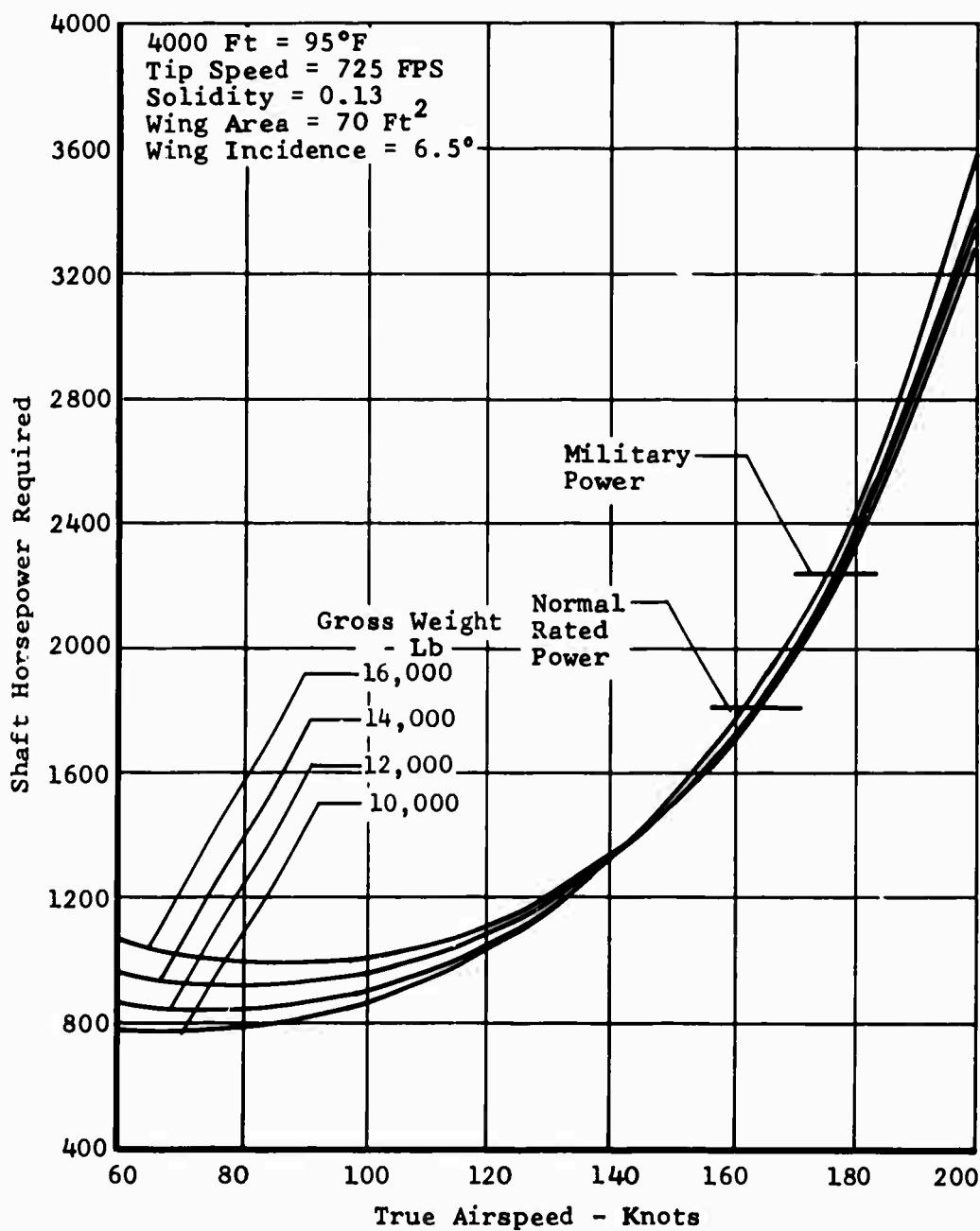
Figure 110. Task II - Winged Helicopter, Speed Power Polar,
