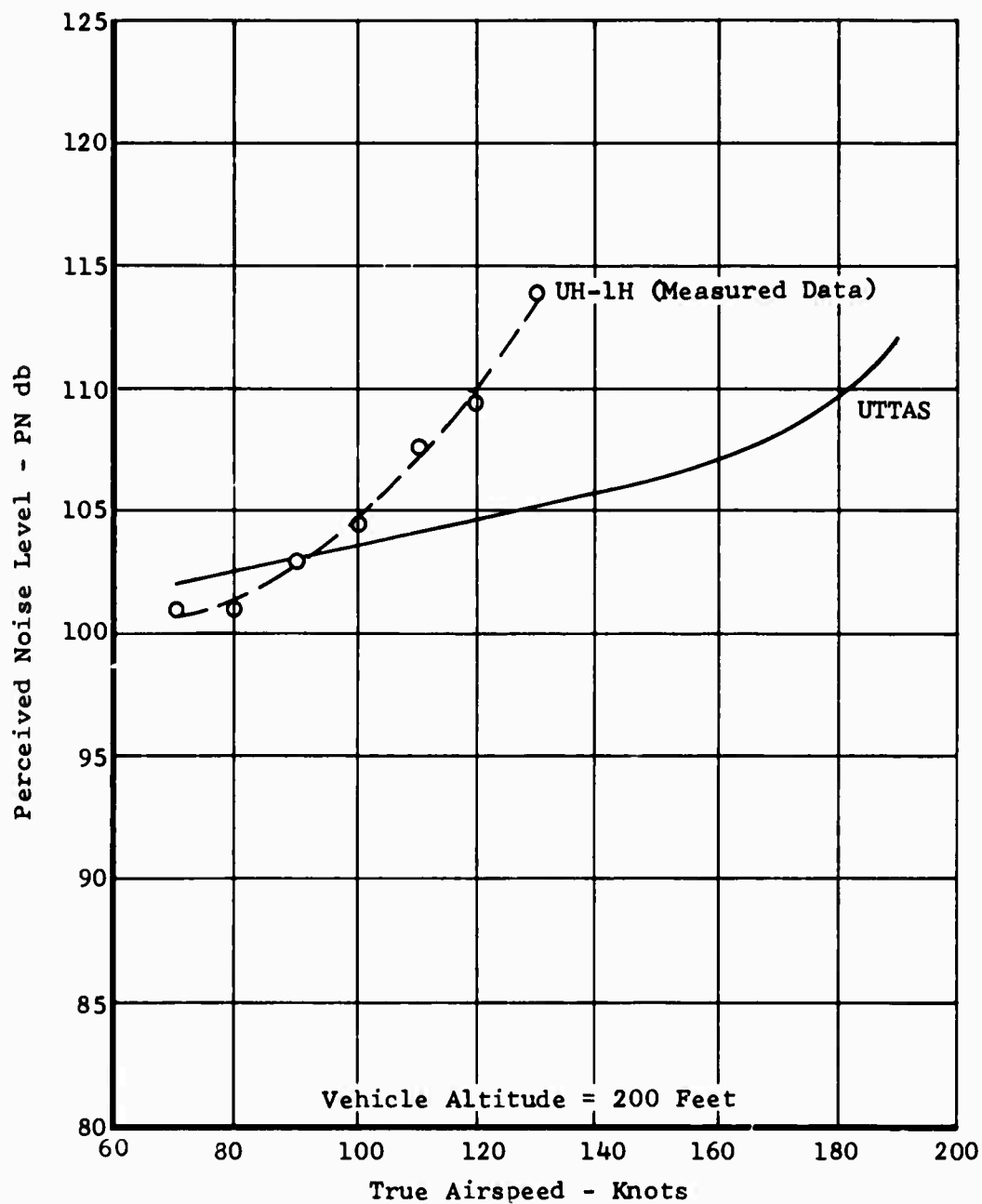
Figure 83. Estimated External Noise Level During Flyover.
