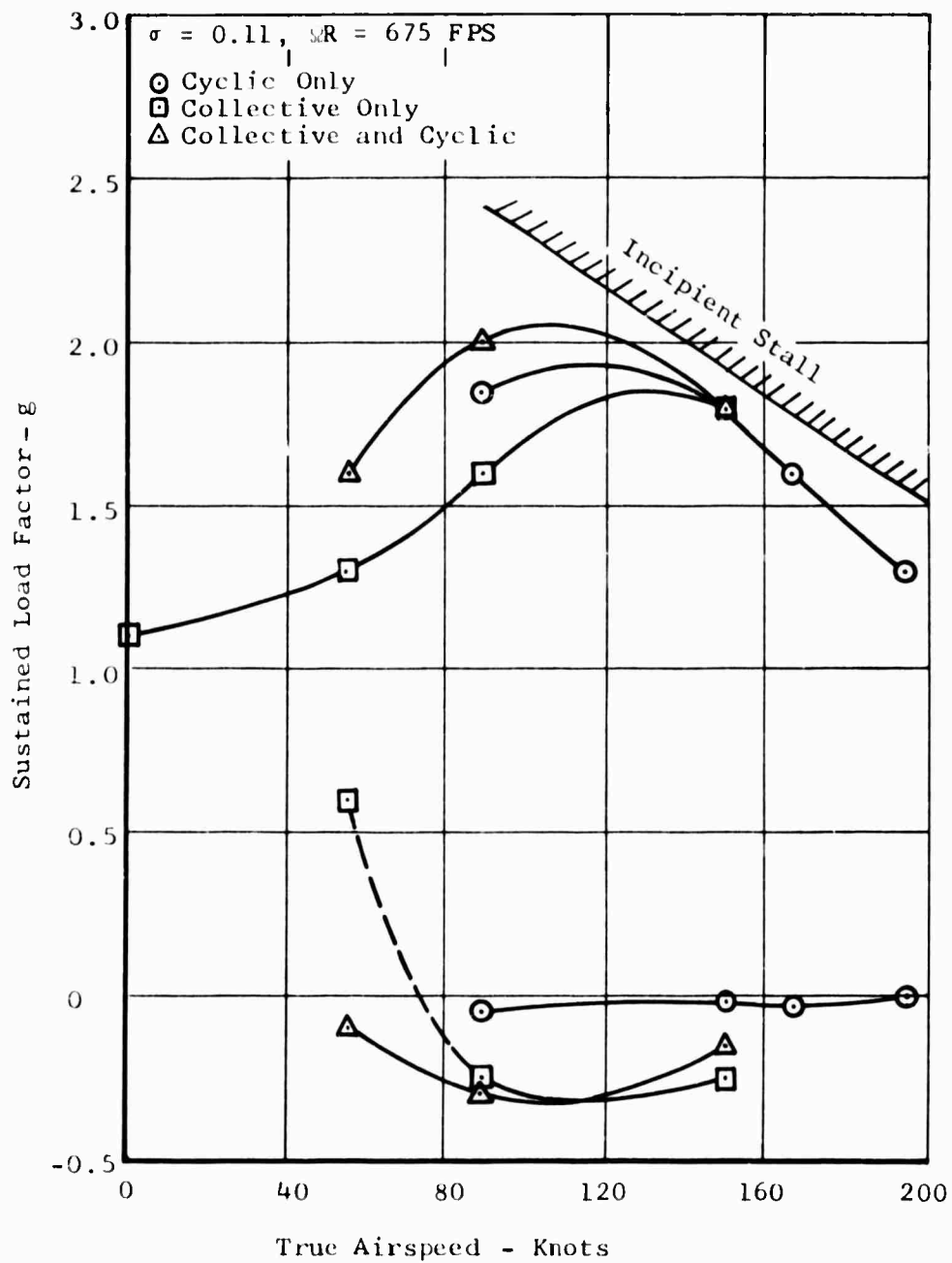
Figure 13. Task I - Maneuver Results, Low Tip Speed Configuration.
