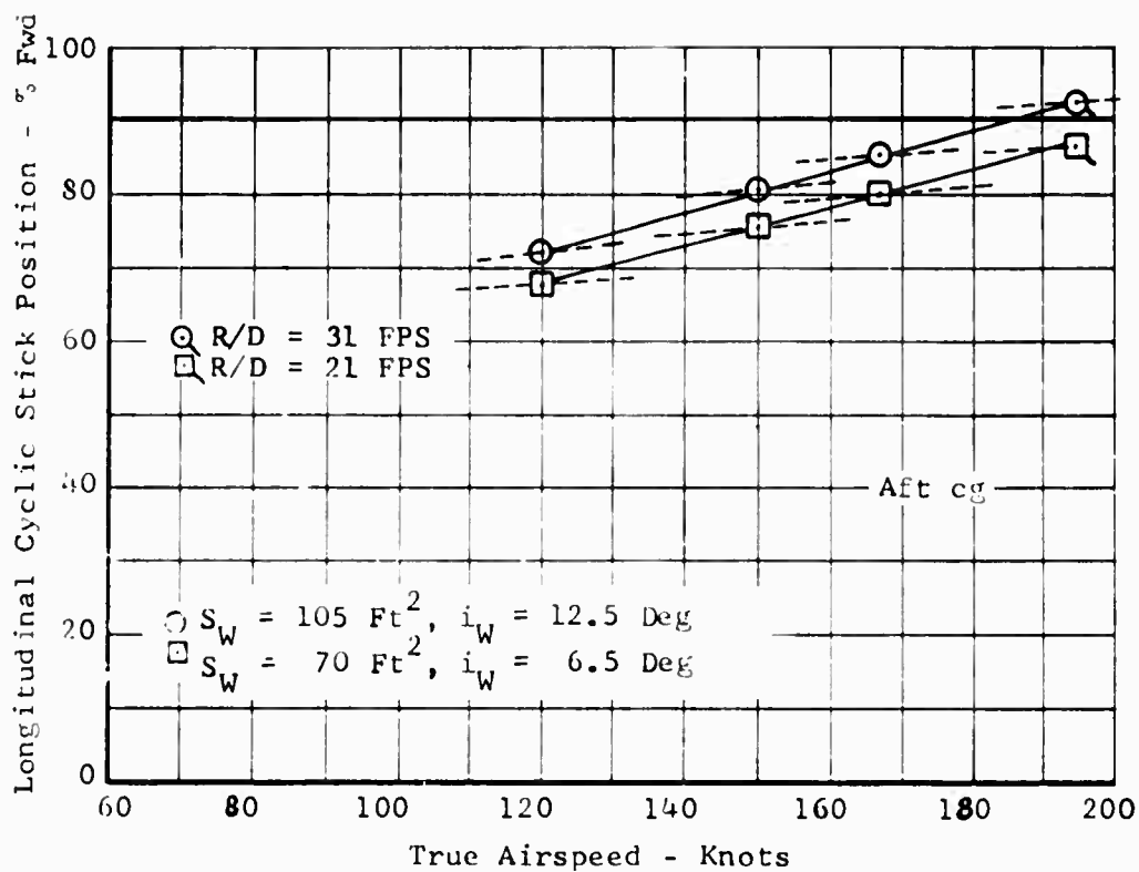
Figure 24. Task II Winged Configuration, Longitudinal Cyclic Stick Position Versus True Airspeed.
