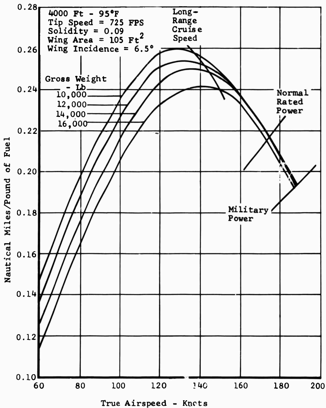
Figure 134. Task II - Winged Helicopter, Specific Range.
