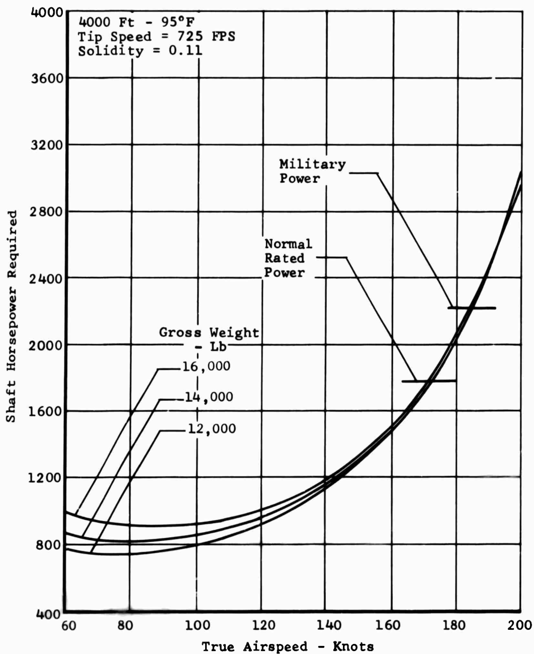
Figure 65. Task III - Wingless Helicopter, Speed Power Polar, 2.00g Design.
