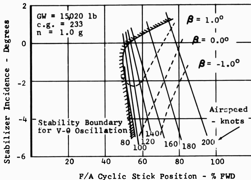
Figure 55. Sample Chart Used for Determination of Stabilizer Rigging
