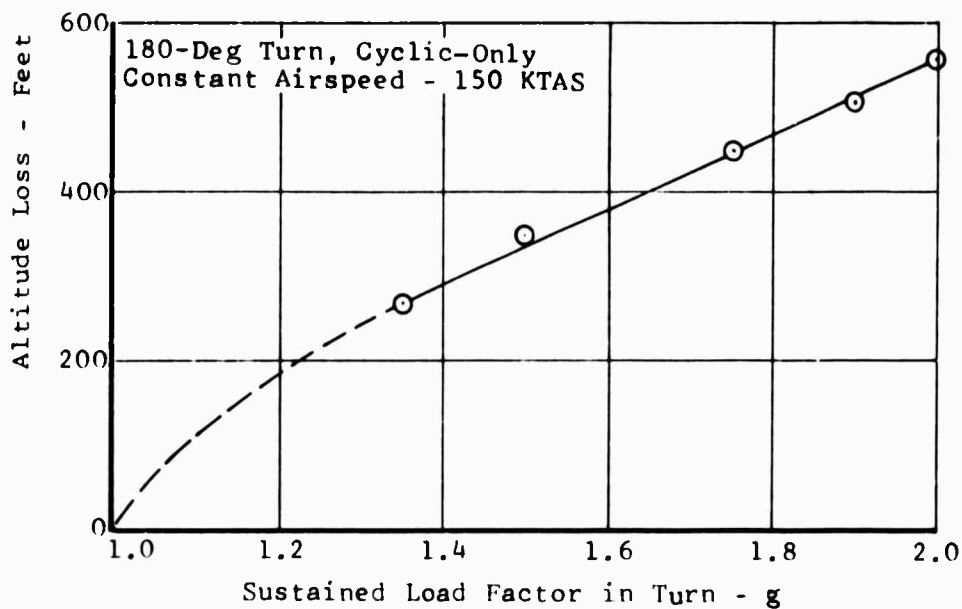
Figure 82. Task III - 2.00g Configuration, Altitude Loss in Constant Airspeed Turn.
