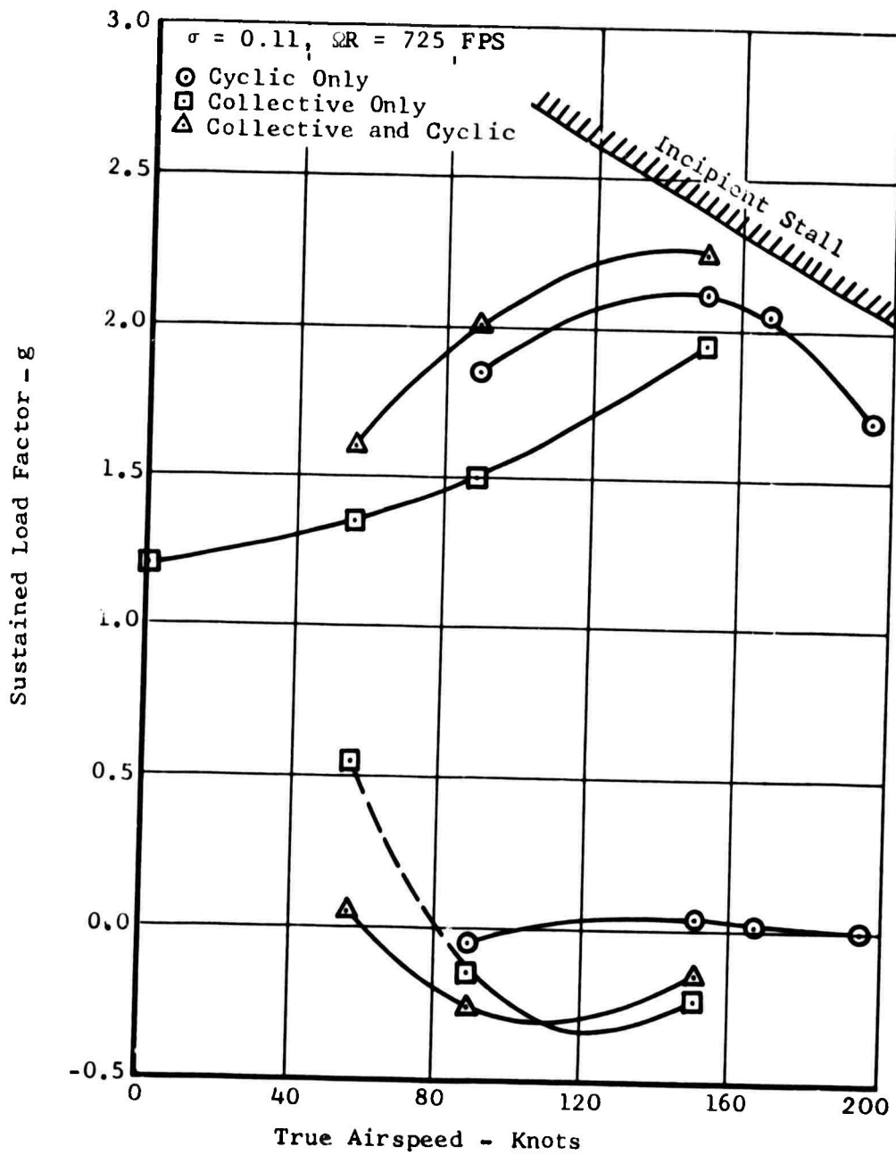
Figure 12. Task I - Maneuver Results, Baseline Configuration.
