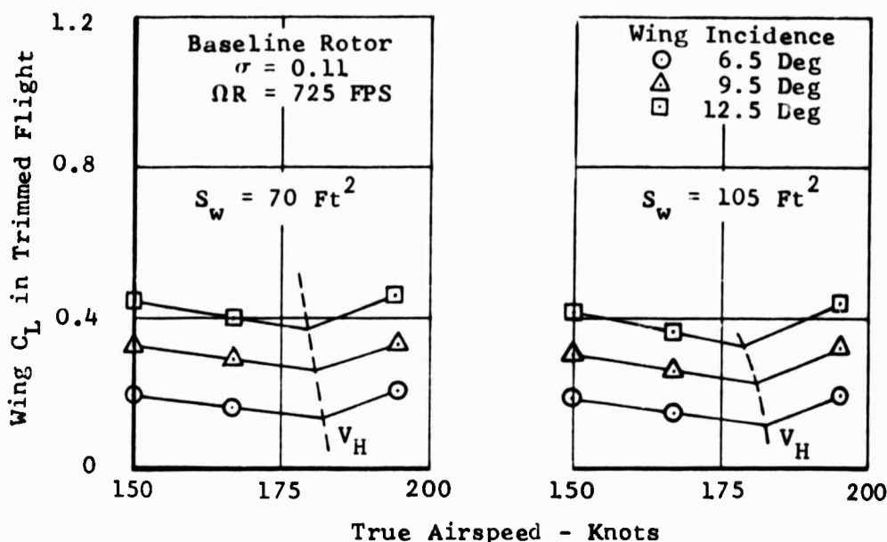
Figure 48. Wing Lift Coefficient in Trimmed Flight, Baseline Rotor, Six Wing Configurations.
