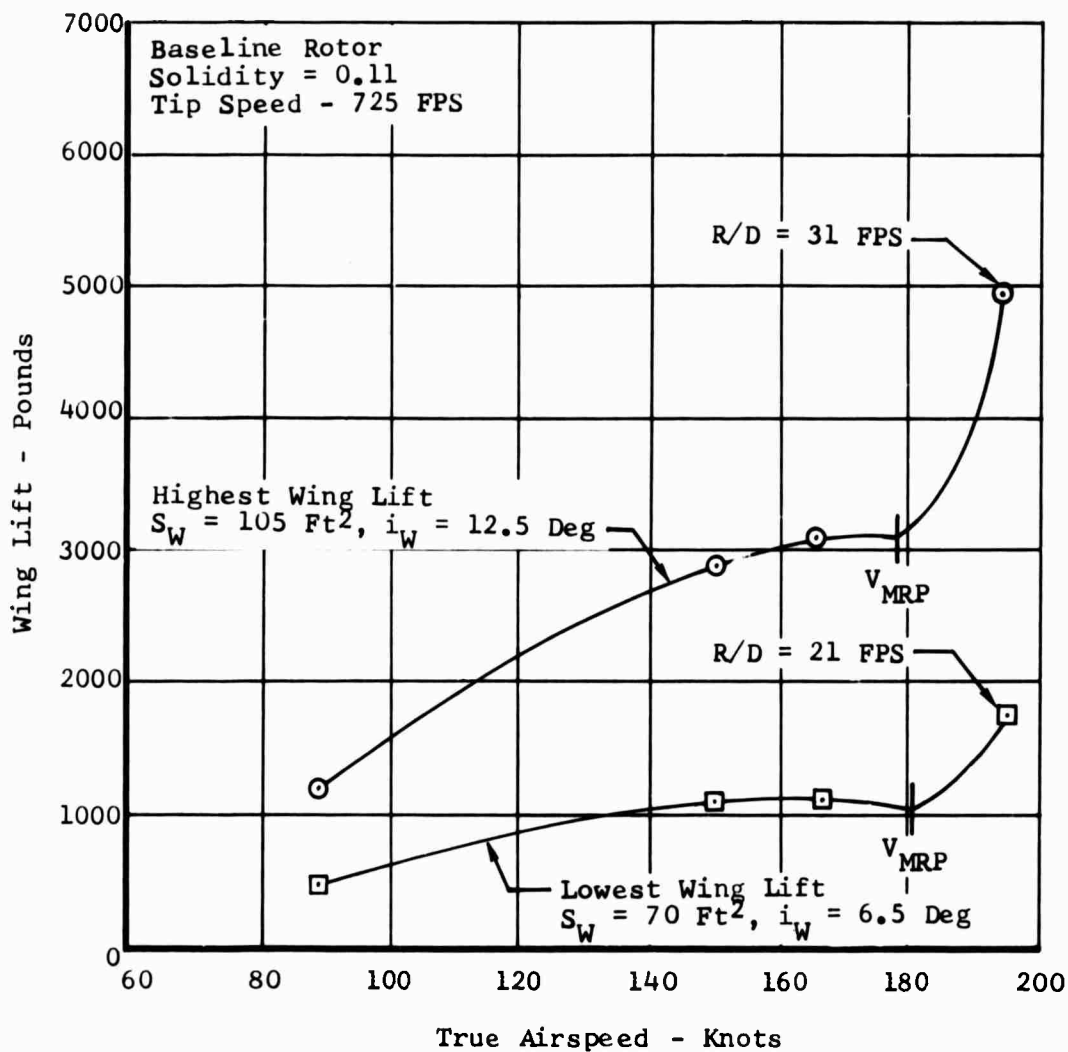
Figure 22. Wing Lift Versus True Airspeed for Task II Configurations.
