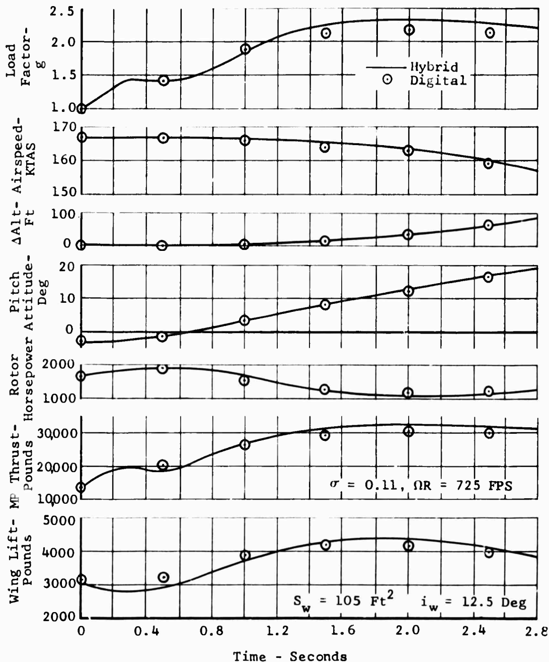
Figure 34. Comparison of Hybrid and Digital Maneuver, Baseline Rotor-Winged Configuration, 2.0-Degree Cyclic Pullup at 167 KTAS.
