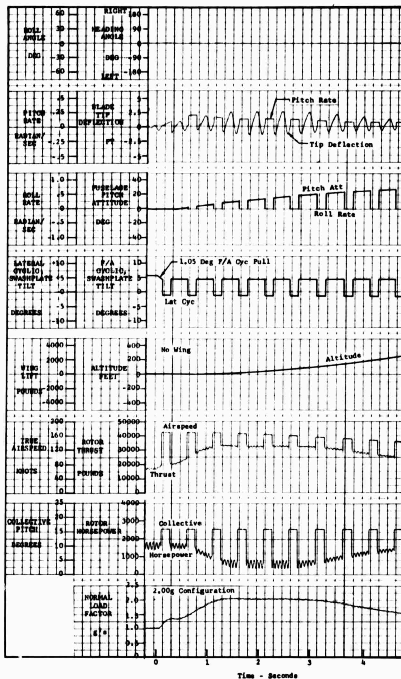
Figure 74. Maneuver Time History, 2.00g Configuration, Limiting Cyclic Pullup at V_{NRP} , Maneuver Limited by Flapping.
