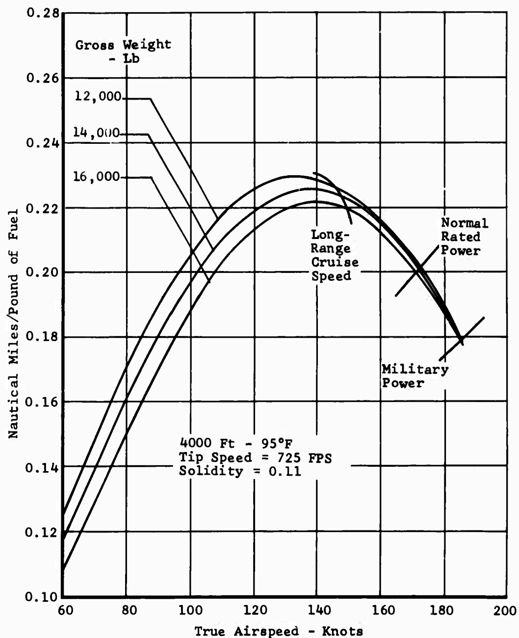
Figure 68. Task III - Wingless Helicopter, Specific Range, 2.00g Design.
