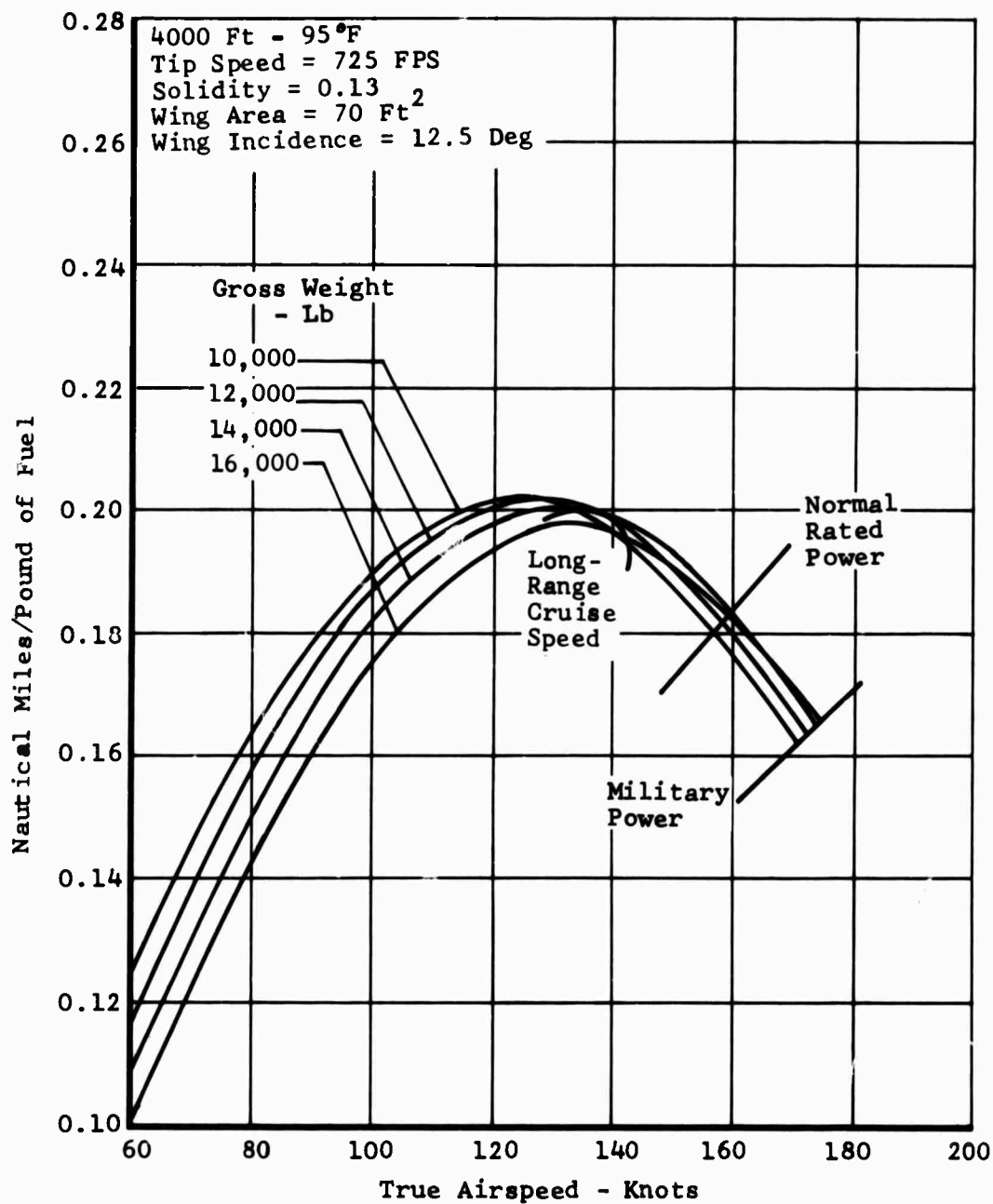
Figure 130. Task II - Winged Helicopter, Specific Range.
