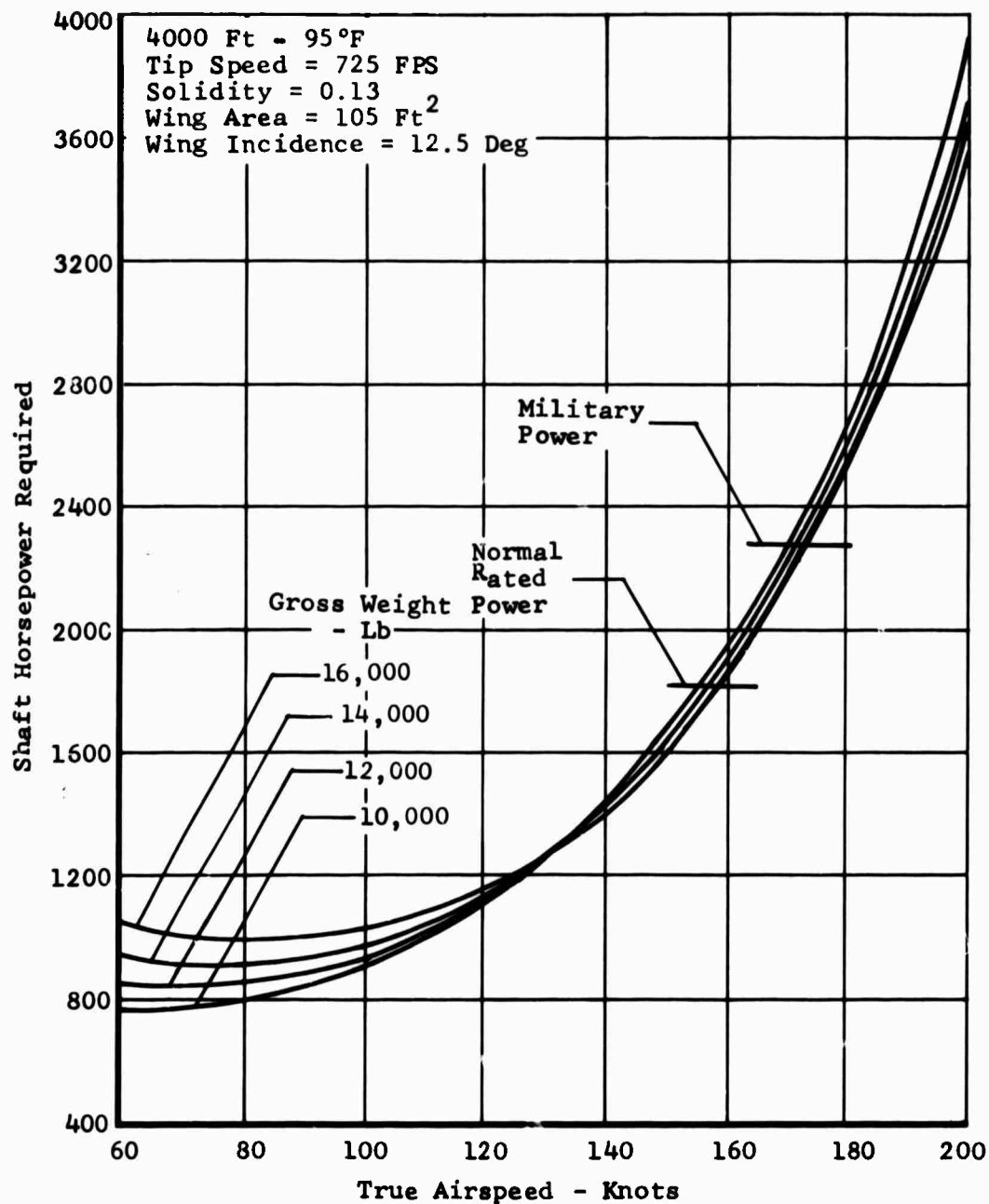
Figure 121. Task II - Winged Helicopter, Speed Power Polar.
