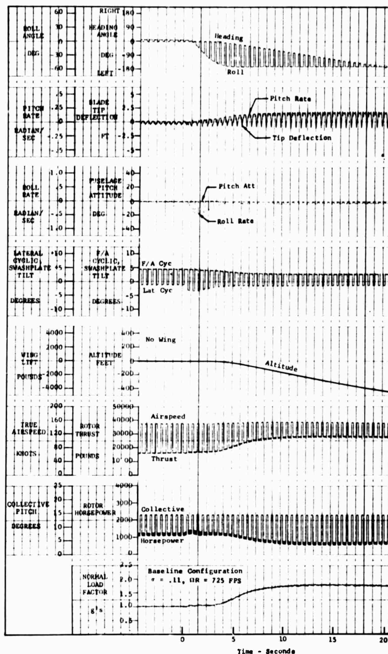
Figure 10. Maneuver Time History, 1.75g Coordinated Turn, Cyclic-Only, Constant Airspeed.
