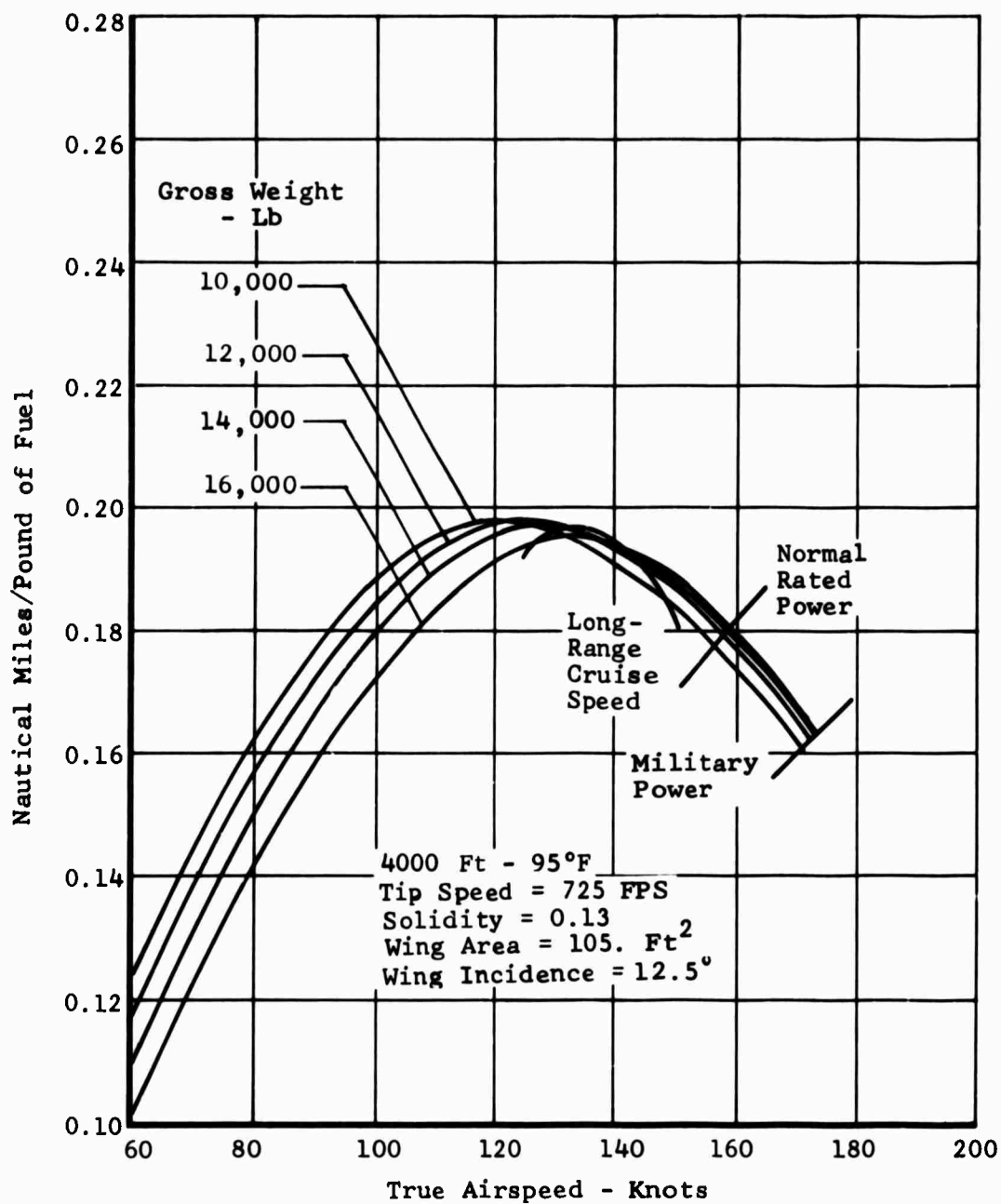
Figure 139. Task II - Winged Helicopter, Specific Range.
