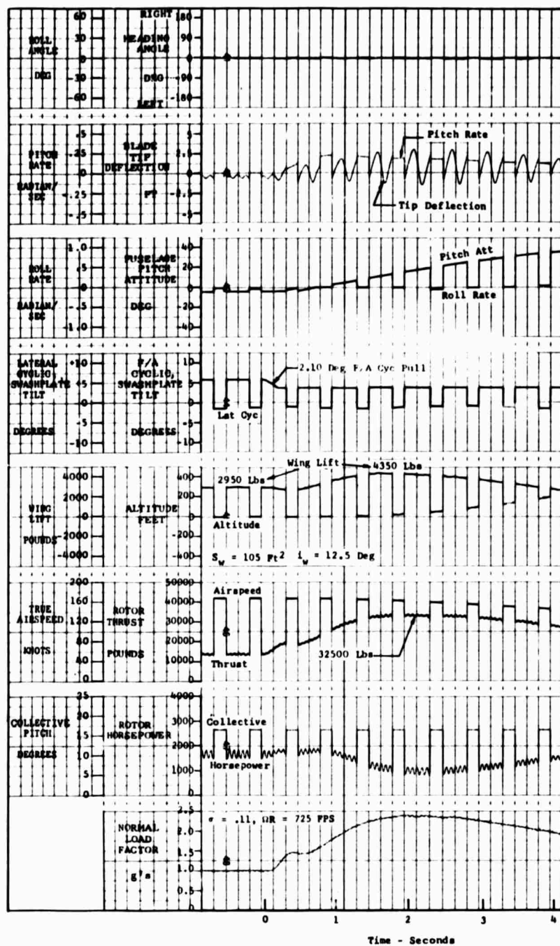
Figure 45. Maneuver Time History, F/A Cyclic Pullup, Baseline Rotor, Large Wing, Maneuver Limited by Flapping.
