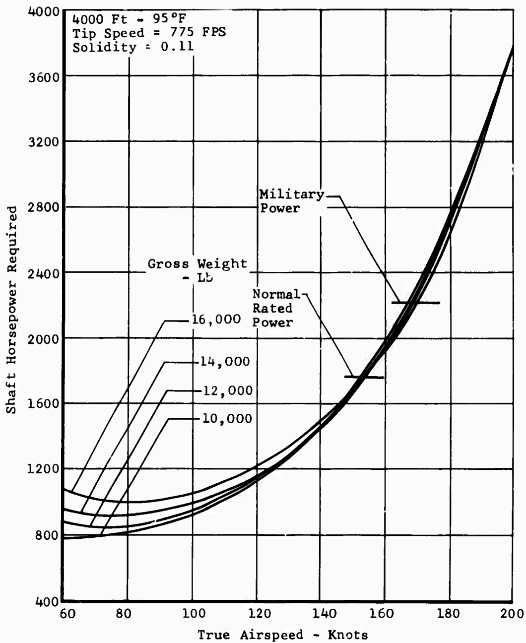
Figure 98. Task I - Wingless Helicopter, Speed Power Polar.
