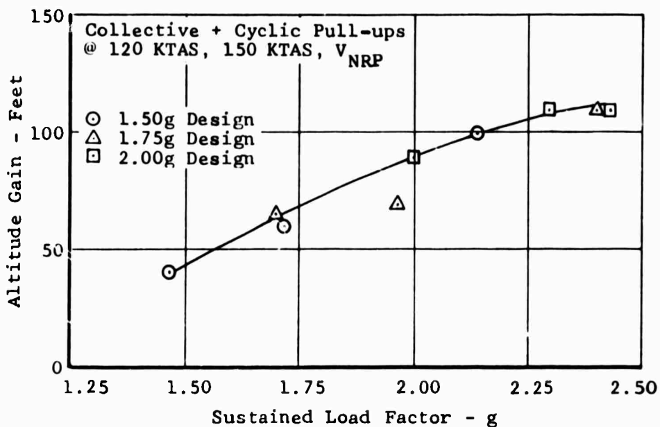
Figure 78. Task III Configurations, Altitude Gain in Pullup Maneuvers After Three Seconds.
