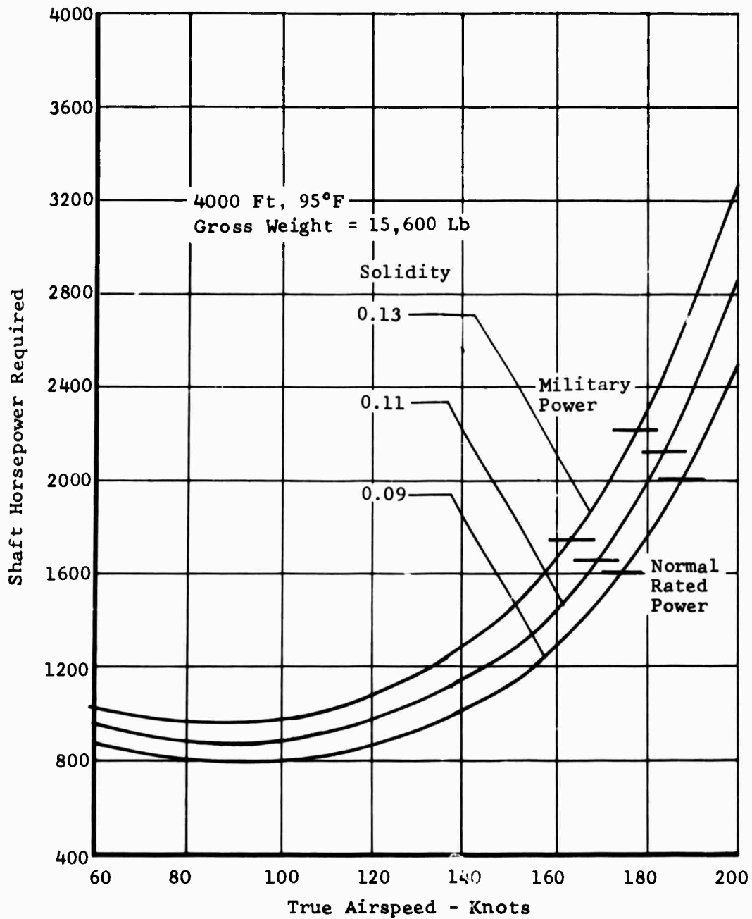
Figure 3. Task I - Wingless Helicopter, Speed Power Polar, Tip Speed = 725 FPS.
