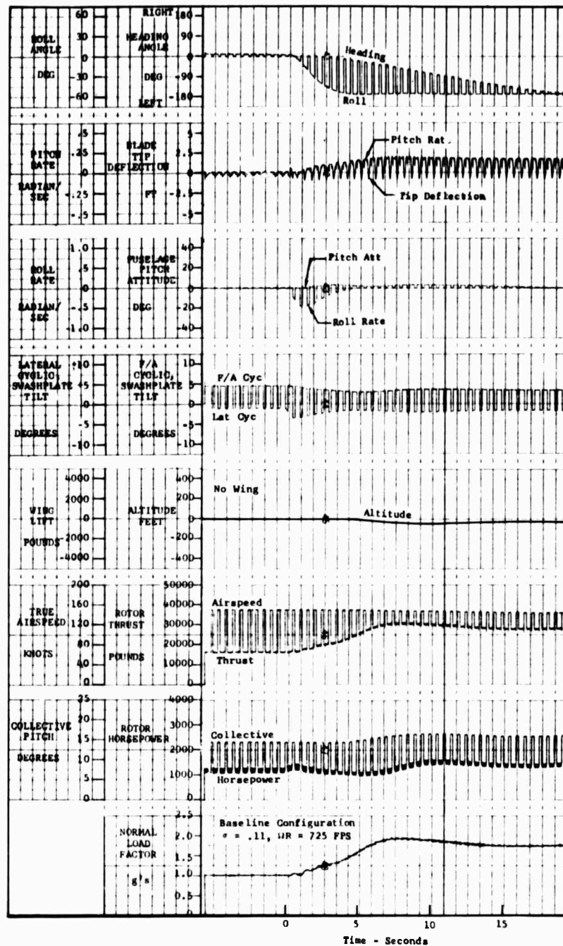
Figure 11. Maneuver Time History, 1.75g Coordinated Turn, Collective + Cyclic, Constant Altitude and Airspeed.
