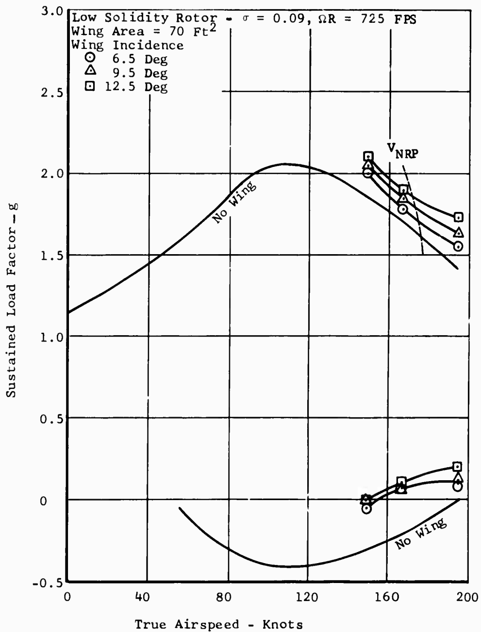
Figure 39. Task II - Maneuver Results, Low Solidity Rotor, Small Wing.
