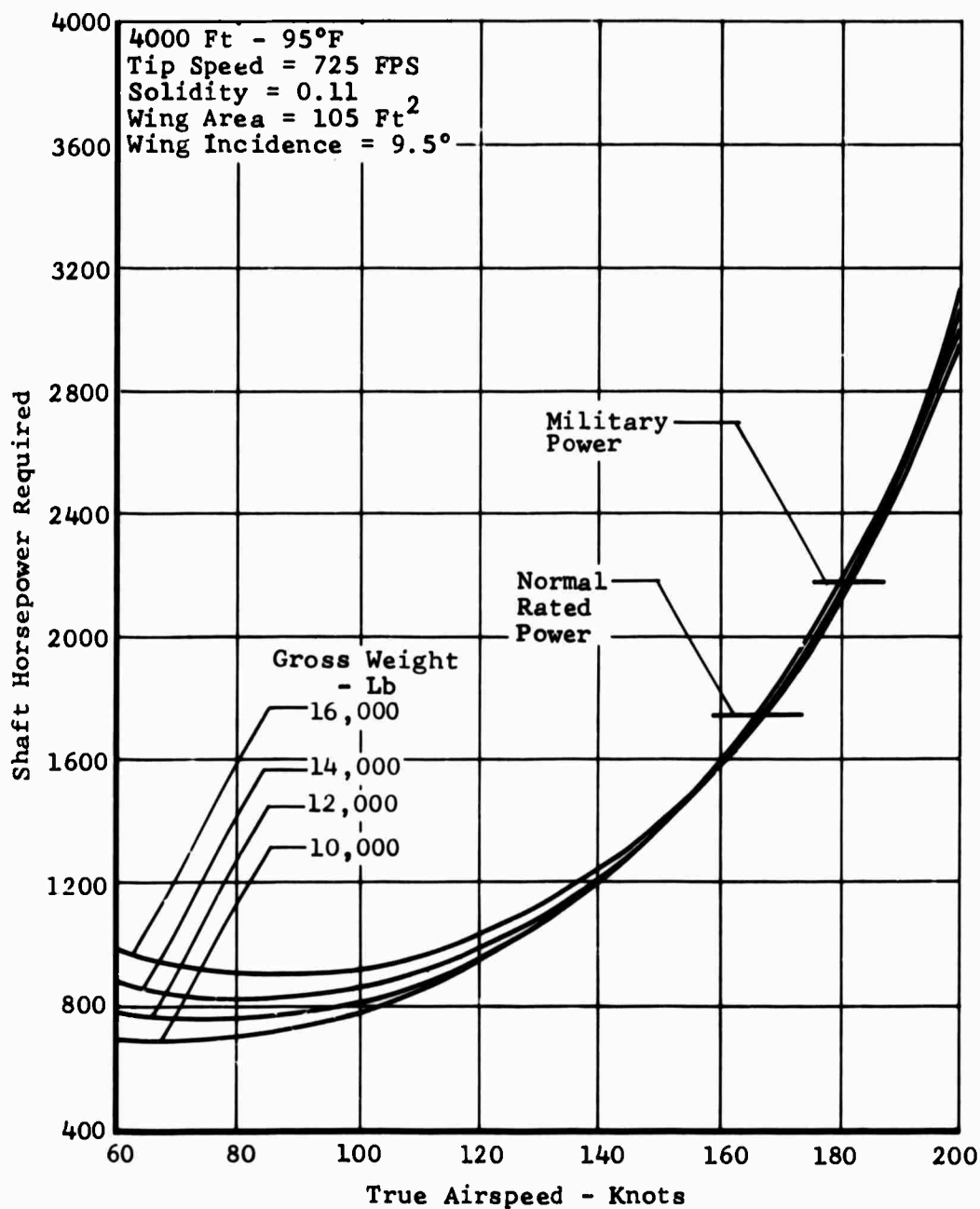
Figure 114. Task II - Winged Helicopter, Speed Power Polar.
