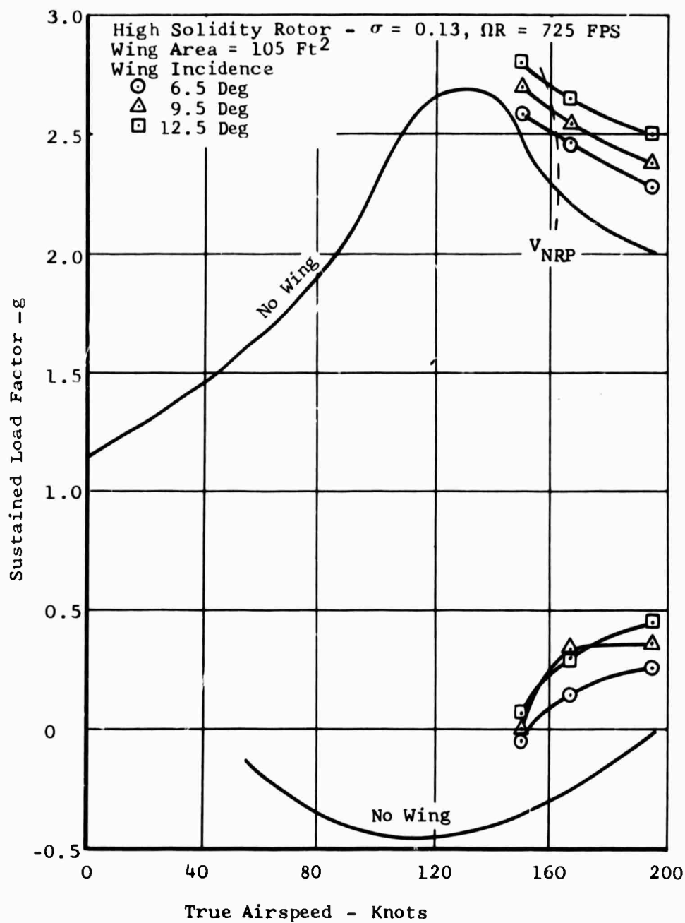
Figure 42. Task II - Maneuver Results, High Solidity Rotor, Large Wing.
