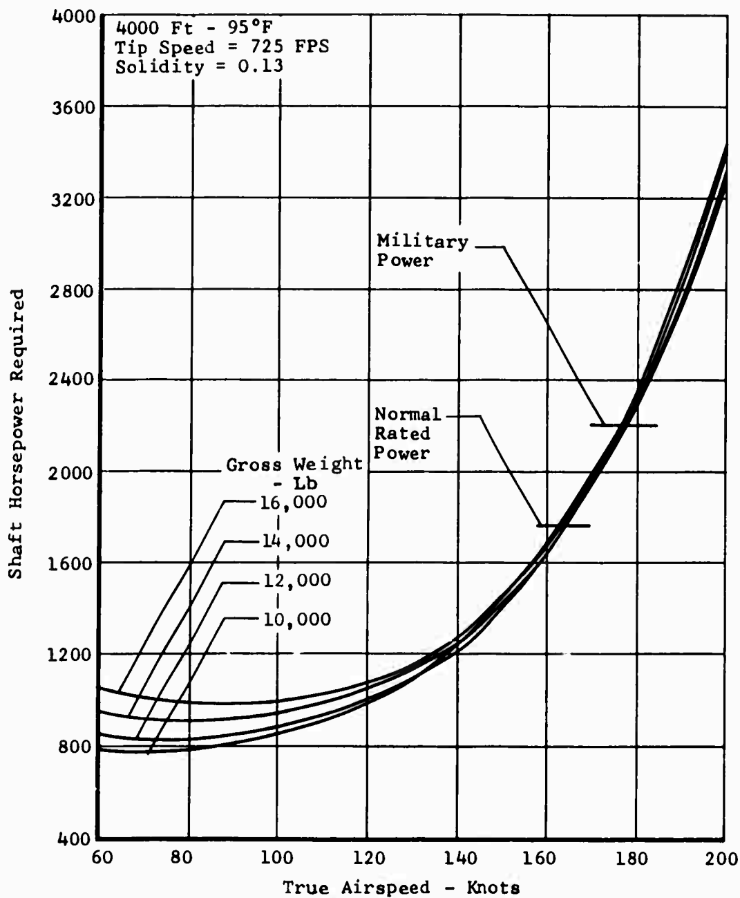
Figure 96. Task I - Wingless Helicopter, Speed Power Polar.
