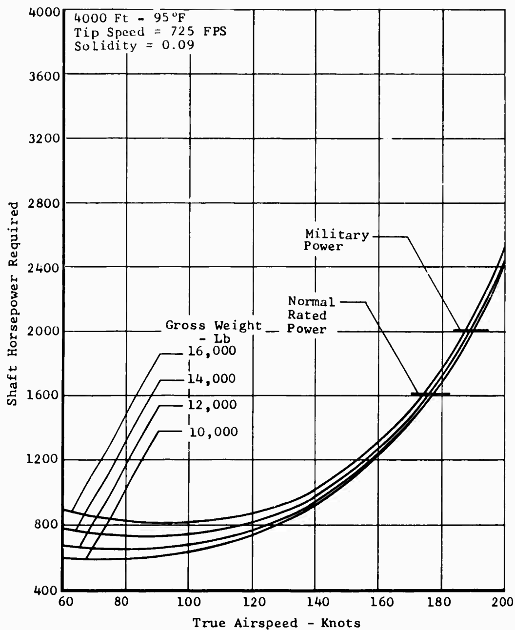
Figure 95. Task I - Wingless Helicopter, Speed Power Polar.
