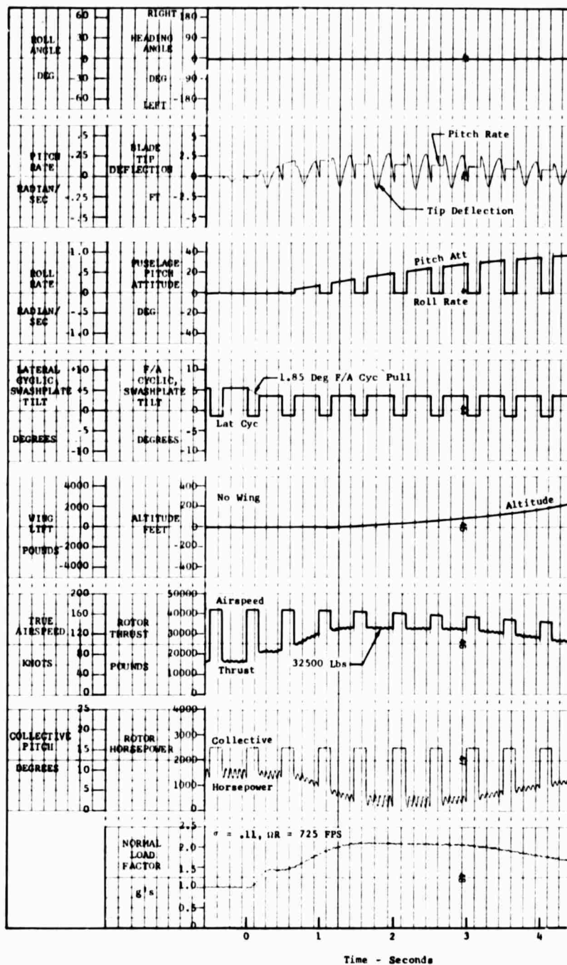
Figure 43. Maneuver Time History, F/A Cyclic Pullup, Baseline Rotor, No Wing, Maneuver Limited by Flapping.
