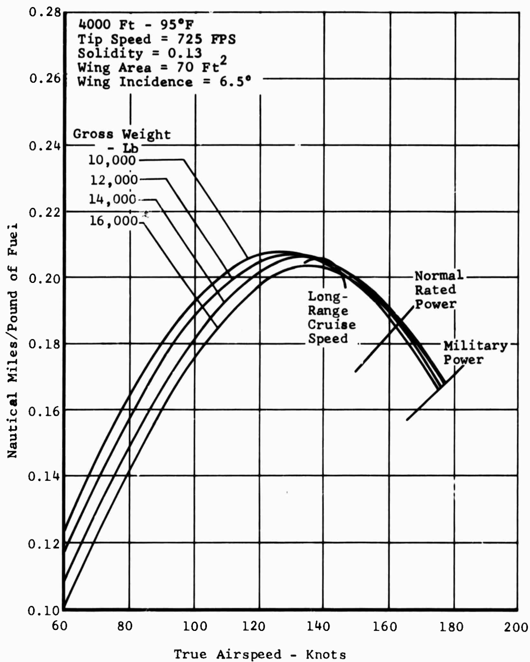
Figure 1.28. Task II - Winged Helicopter, Specific Range.
