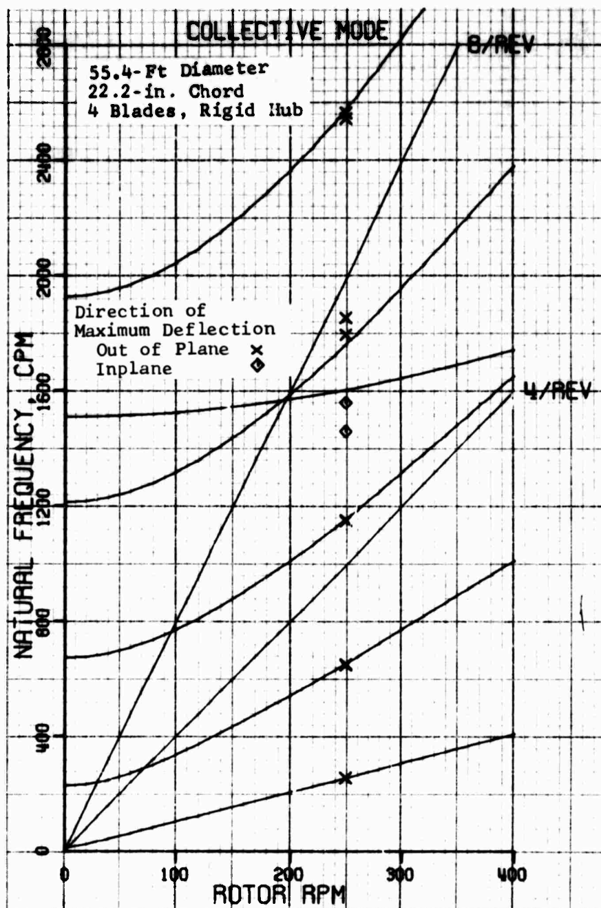
Figure 89. Collective Mode Frequencies for Alternate Rotor.
