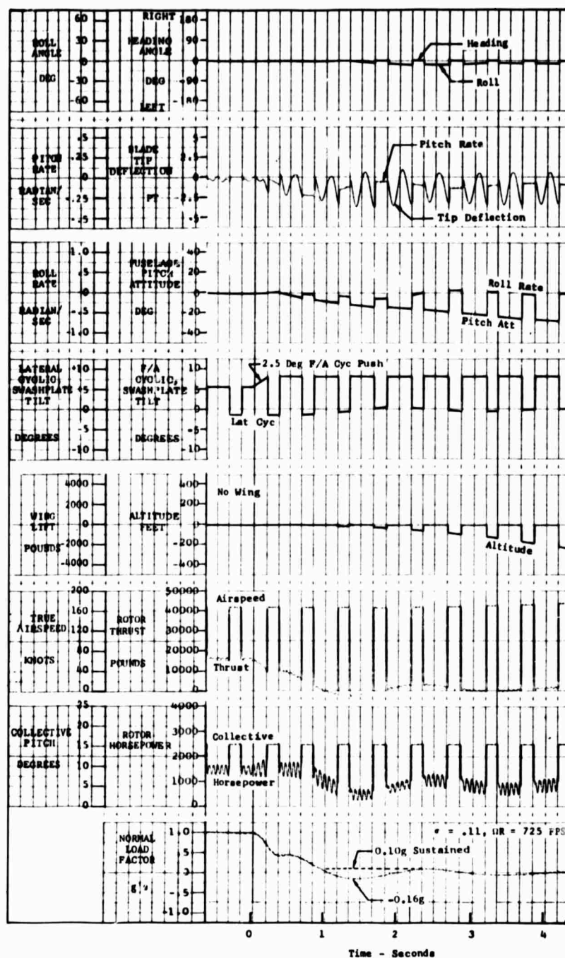
Figure 46. Maneuver Time History, F/A Cyclic Pushover, Baseline rotor, No Wing, Maneuver Limited by Flapping.
