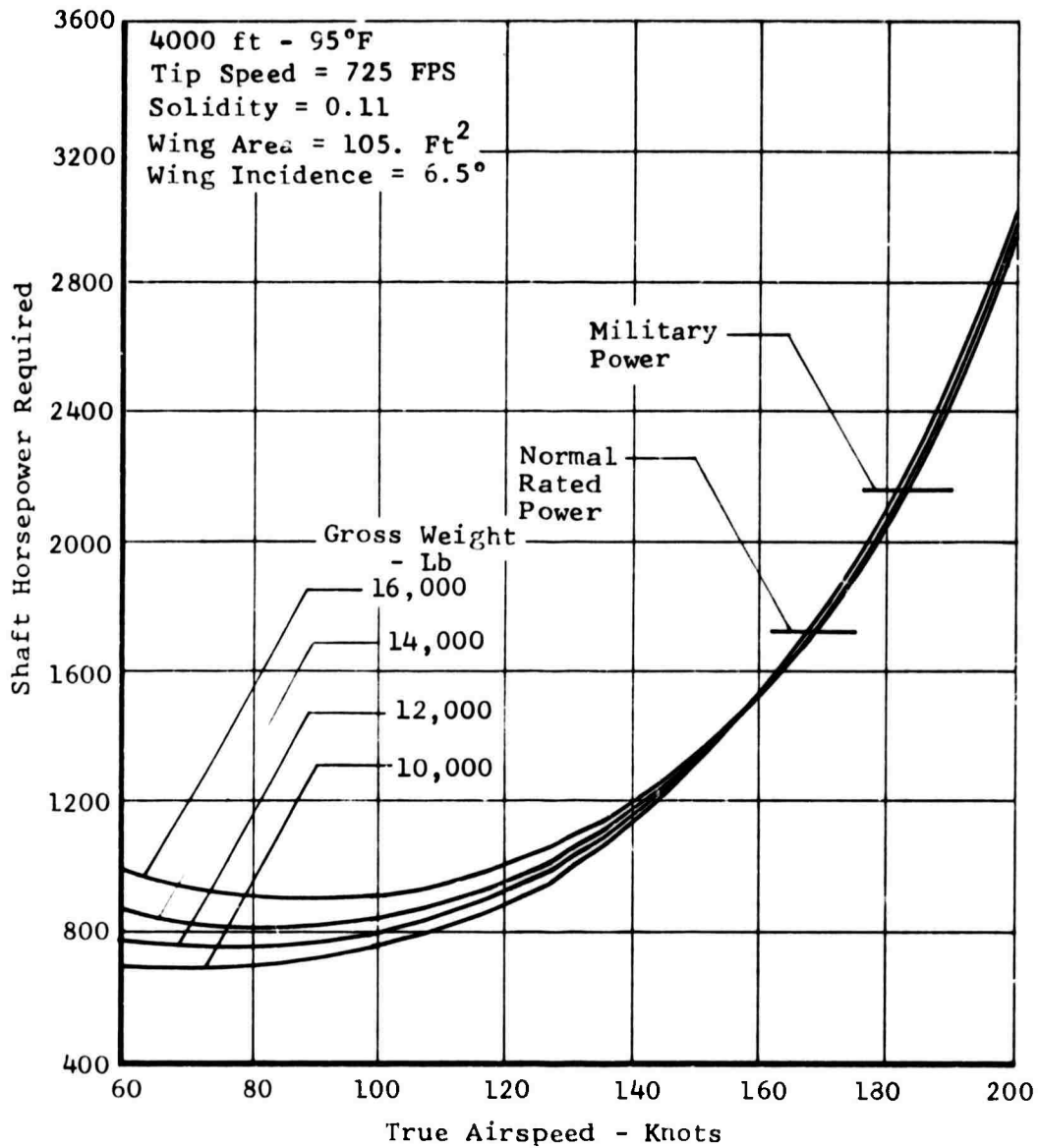
Figure 104. Task II - Winged Helicopter, Speed Power Polar.
