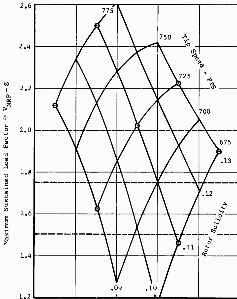
Figure 19. Effects of Rotor Solidity and Tip Speed on g-Capability at V_{NRP} .
