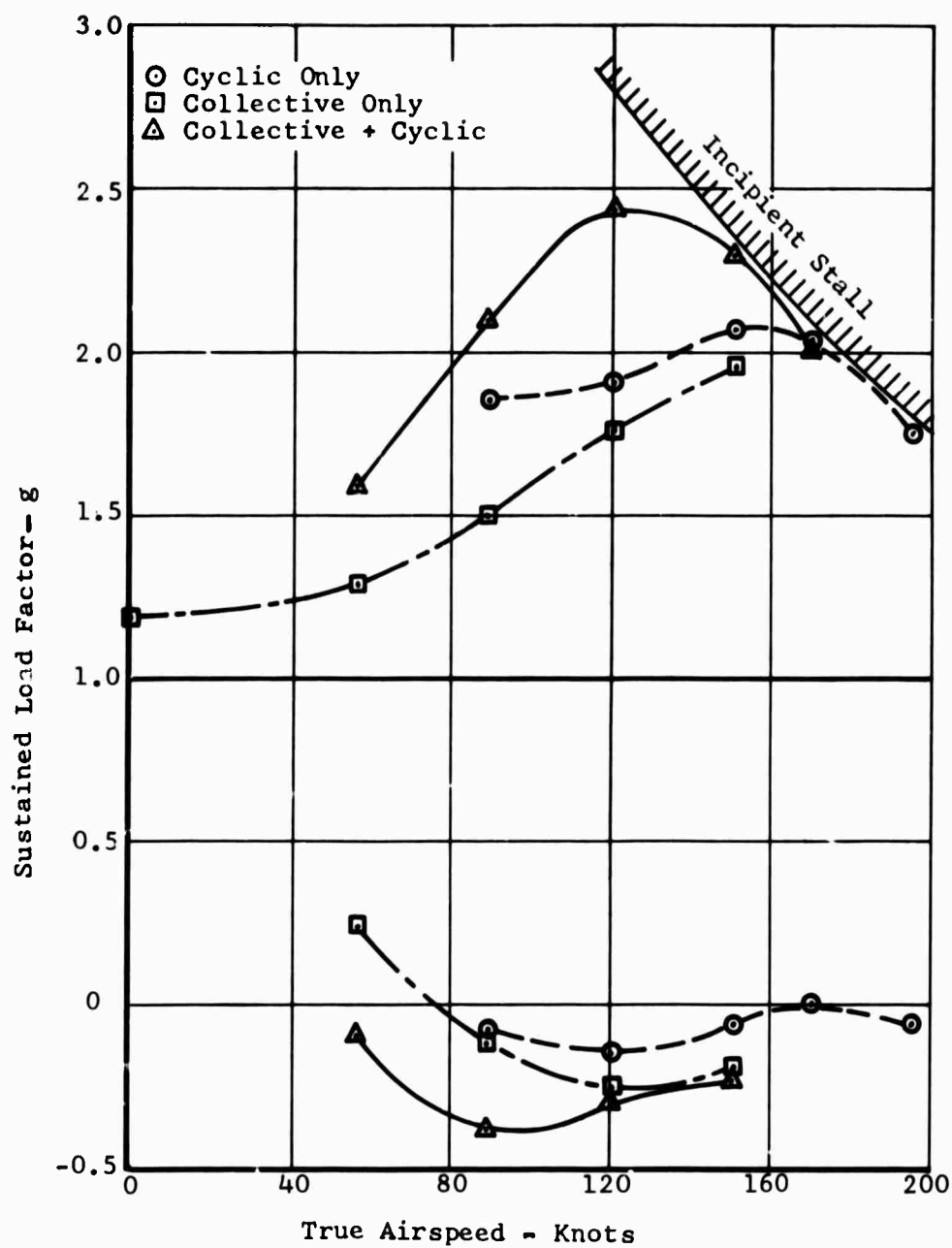
Figure 71. Task III - Maneuver Results, 2.00g Design.
