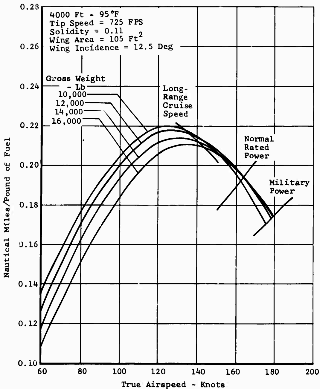
Figure 133. Task II - Winged Helicopter, Specific Range.
