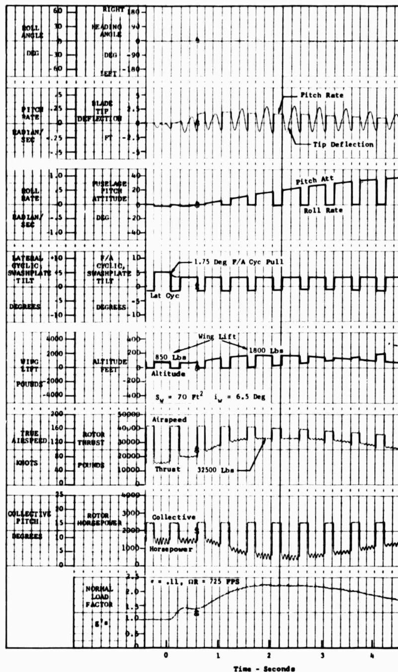
Figure 44. Maneuver Time History, F/A Cyclic Pullup, Baseline Rotor, Small Wing, Maneuver Limited by Flapping.
