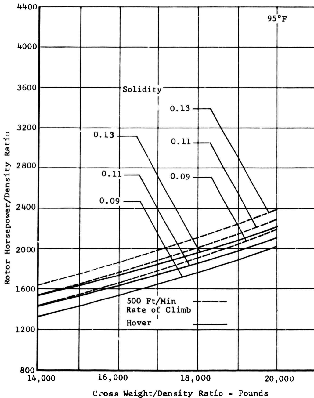
Figure 1. Task I - Wingless Helicopter, Hover Power Required, Tip Speed = 725 FPS.
