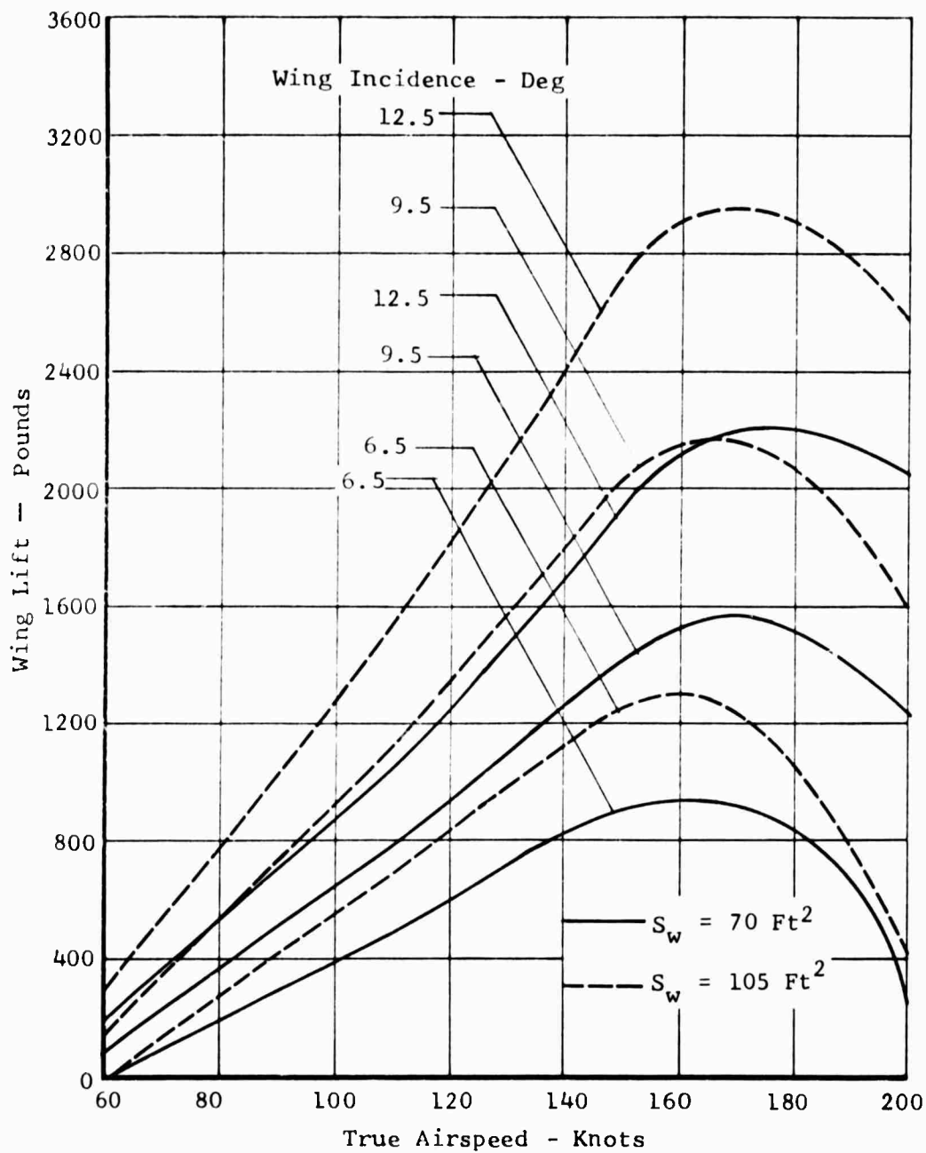
Figure 25. Task II - Winged Helicopter, Wing Lift Versus True Airspeed, Solidity = 0.11.
