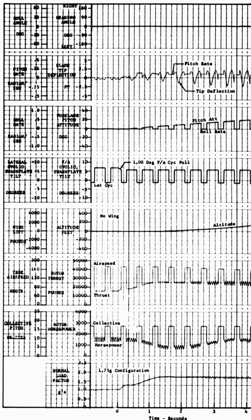
Figure 73. Maneuver Time History, 1.75g Configuration, Limiting Cyclic Pullup at V_{NRP} , Maneuver Limited by Flapping.
