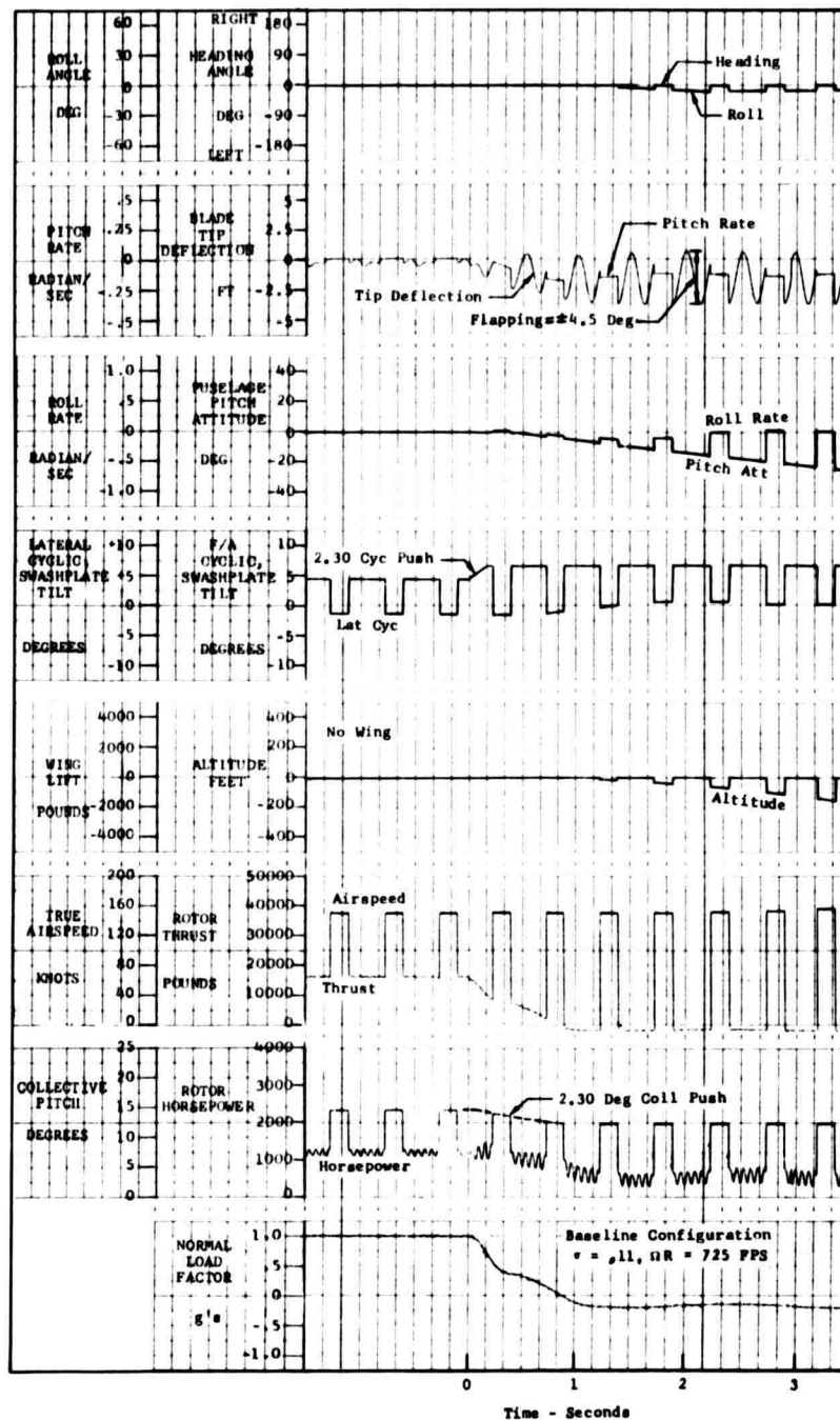
Figure 8. Maneuver Time History, Collective + F/A Cyclic Pushover, Maneuver Limited by Flapping.
