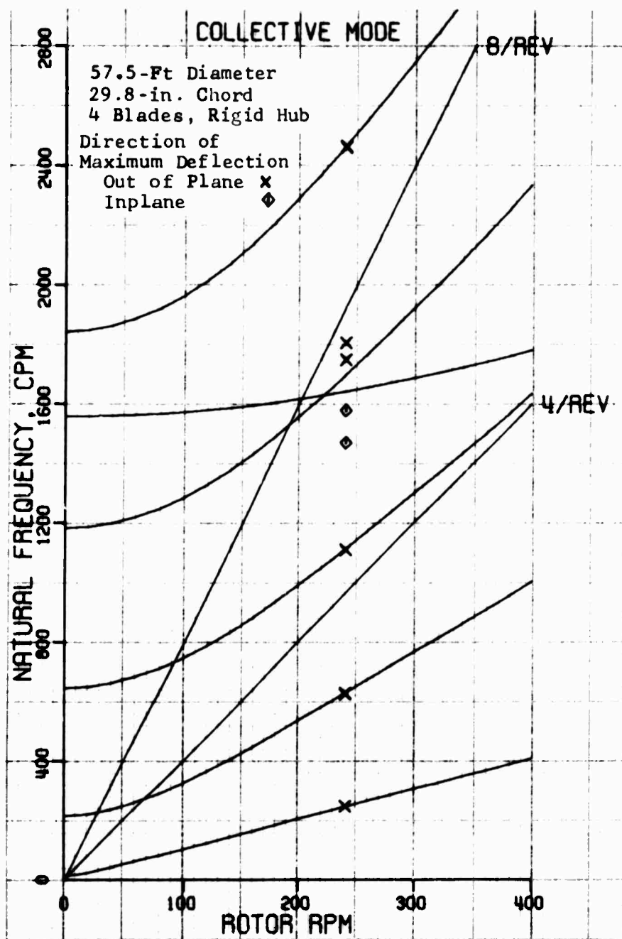
Figure 86. Collective Mode Frequencies for Baseline Rotor.
