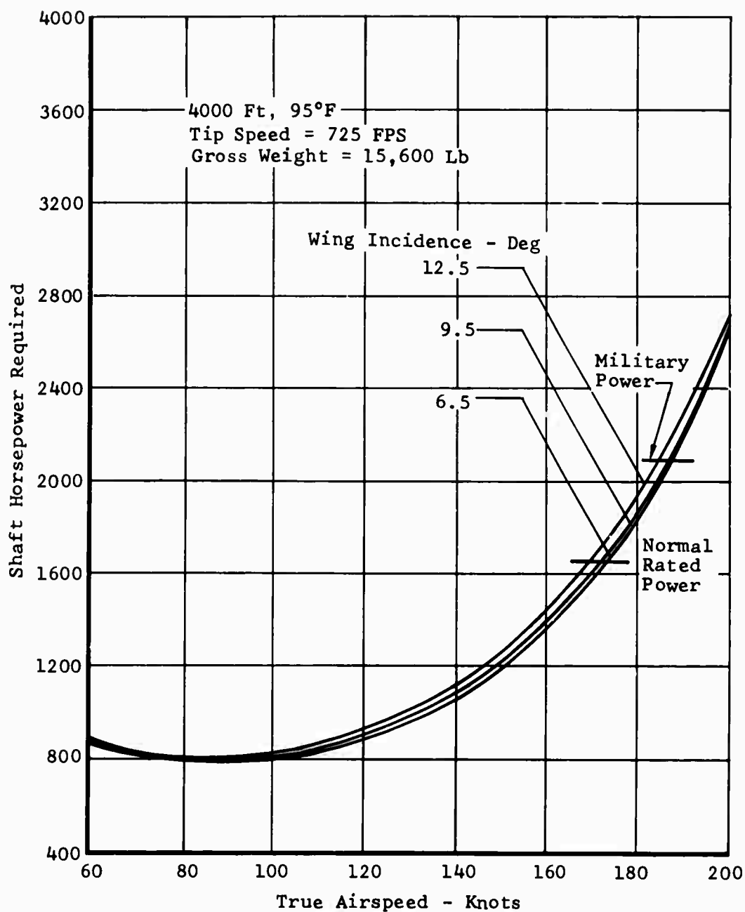
Figure 32. Task II - Winged Helicopter, Speed Power Polar, Solidity = 0.09, Wing Area = 105 Ft 2 .
