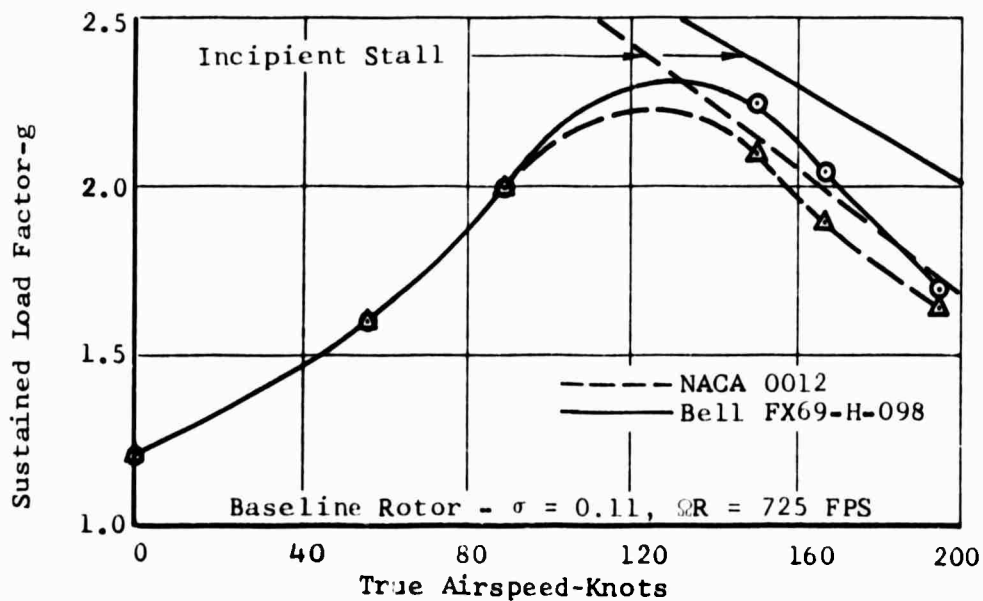
Figure 17. Comparison of Airfoil Maximum Lift Characteristics, Bell FX69-H-098 and NACA 0012.
