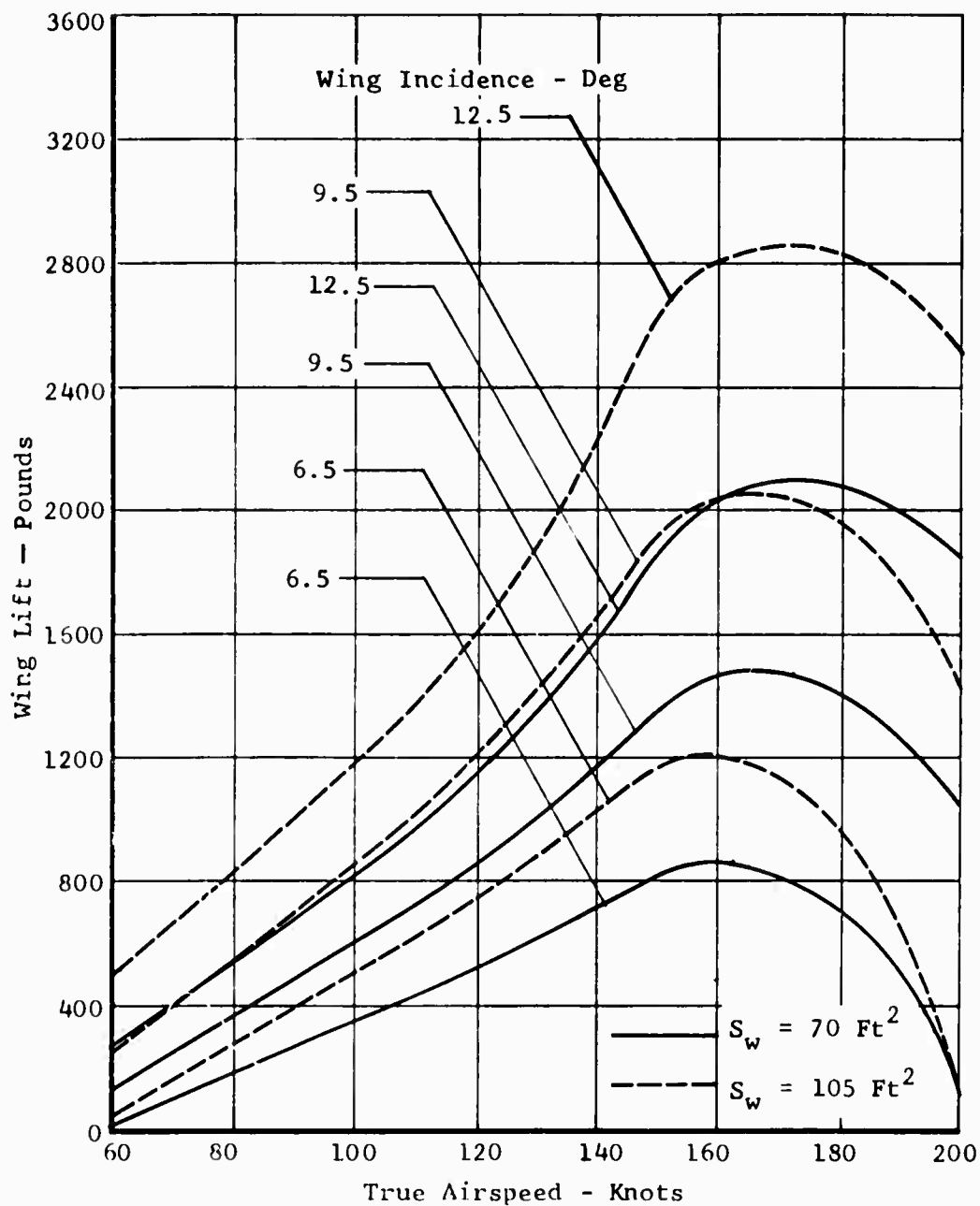
Figure 27. Task II - Winged Helicopter, Wing Lift Versus True Airspeed, Solidity = 0.13.
