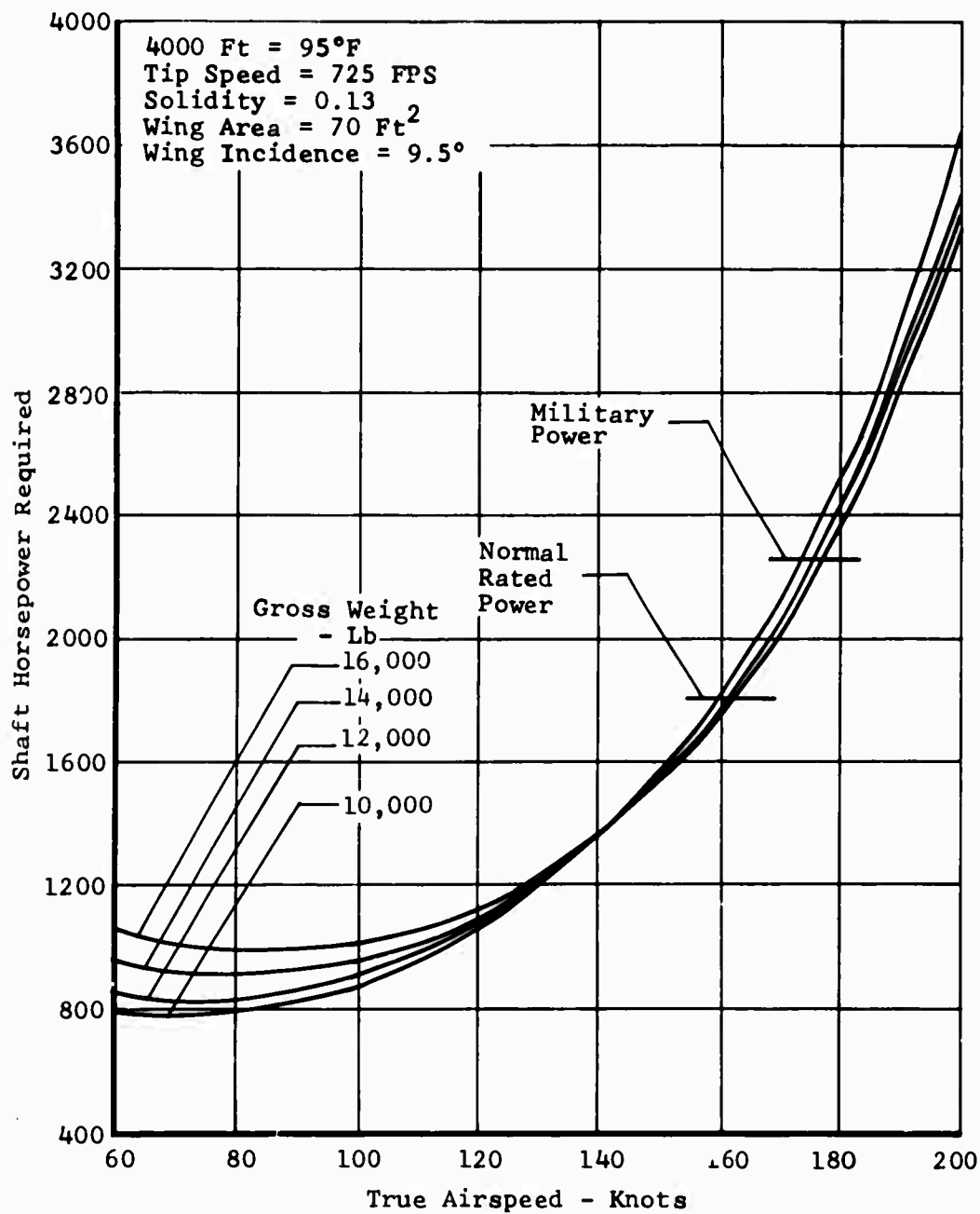
Figure 111. Task II - Winged Helicopter, Speed Power Polar.
