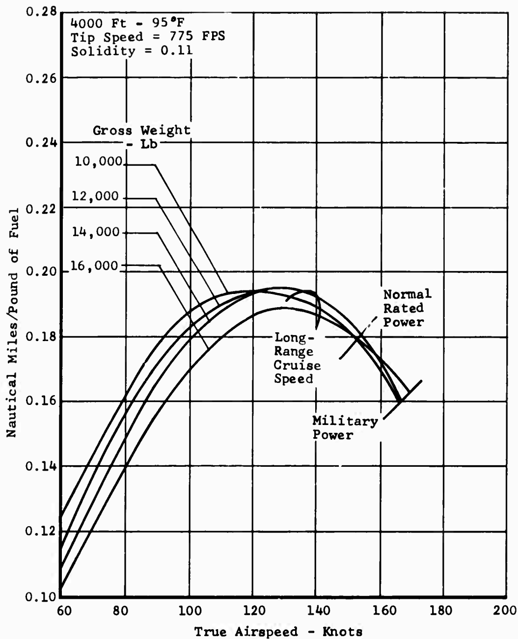
Figure 103. Task I - Wingless Helicopter, Specific Range.
