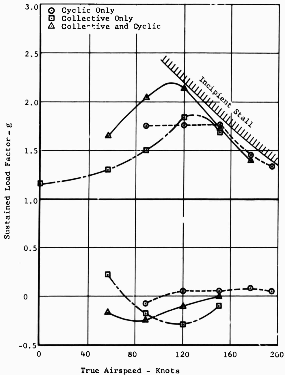
Figure 69. Task III - Maneuver Results, 1.5g Design.
