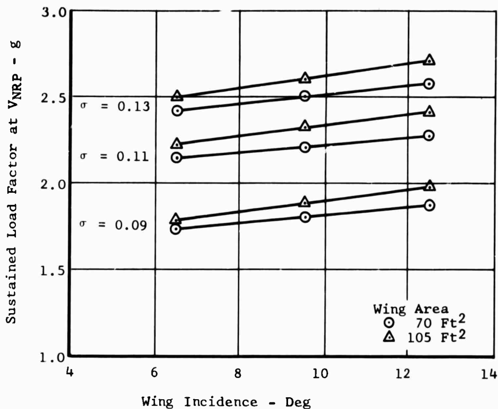
Figure 50. Effects of Wing Incidence on Load Factor Capability at V_{NRP} .
