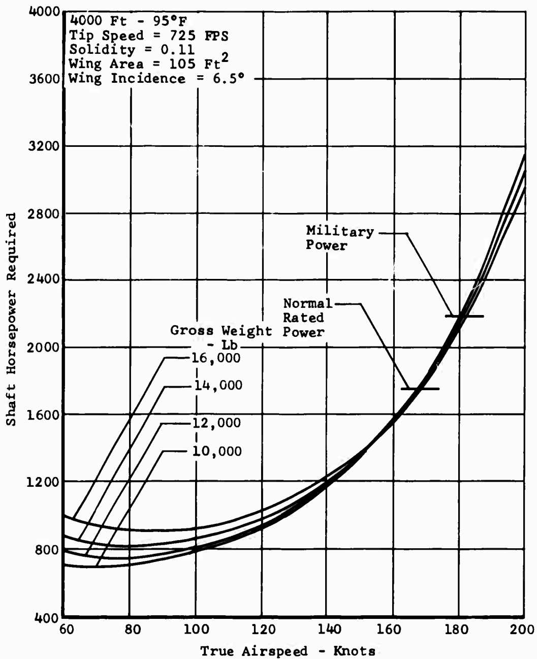
Figure 113. Task II - Winged Helicopter, Speed Power Polar.
