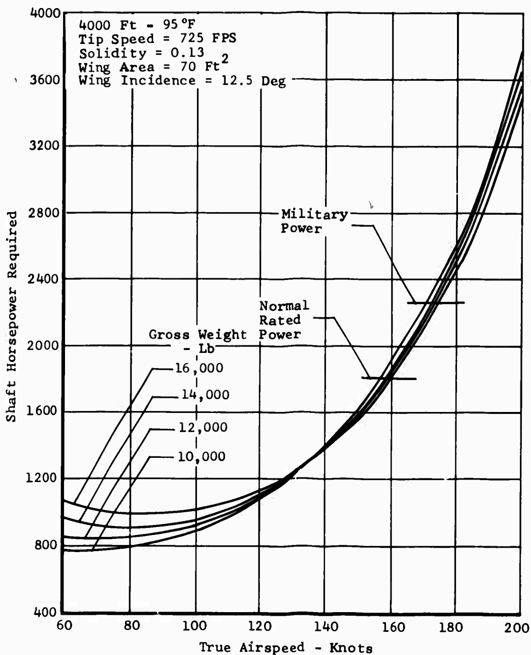
Figure 112. Task II - Winged Helicopter, Speed Power Polar.
