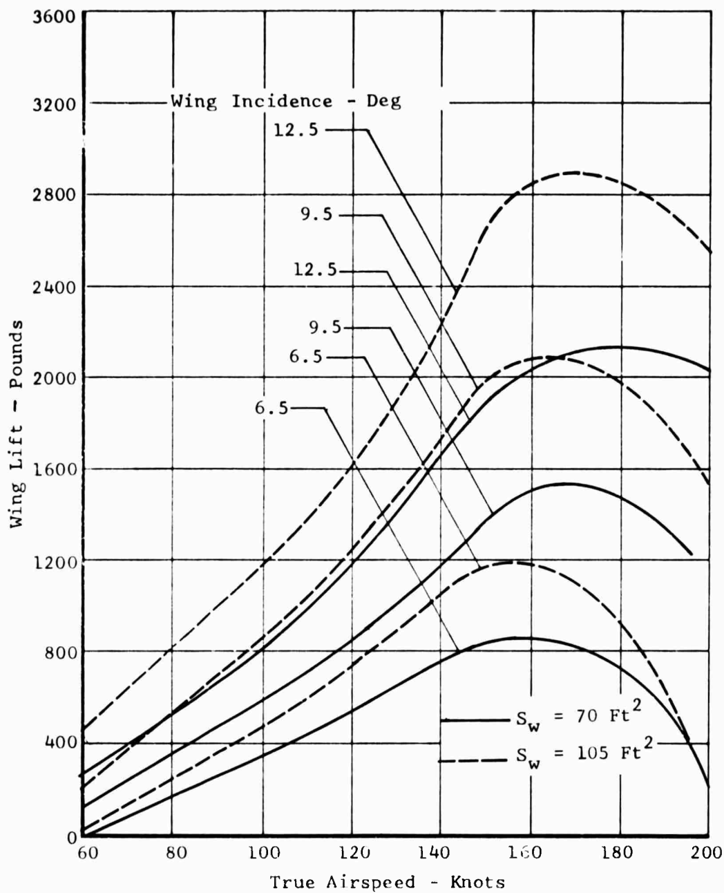
Figure 26. Task II - Winged Helicopter, Wing Lift Versus True Airspeed, Solidity = 0.09.
