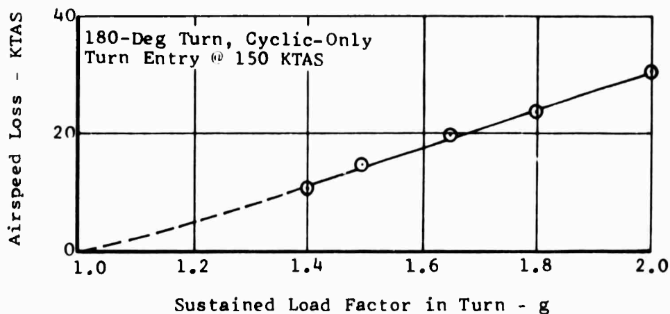
Figure 81. Task III - 2.00g Configuration, Airspeed Loss in Constant Altitude Turn.
