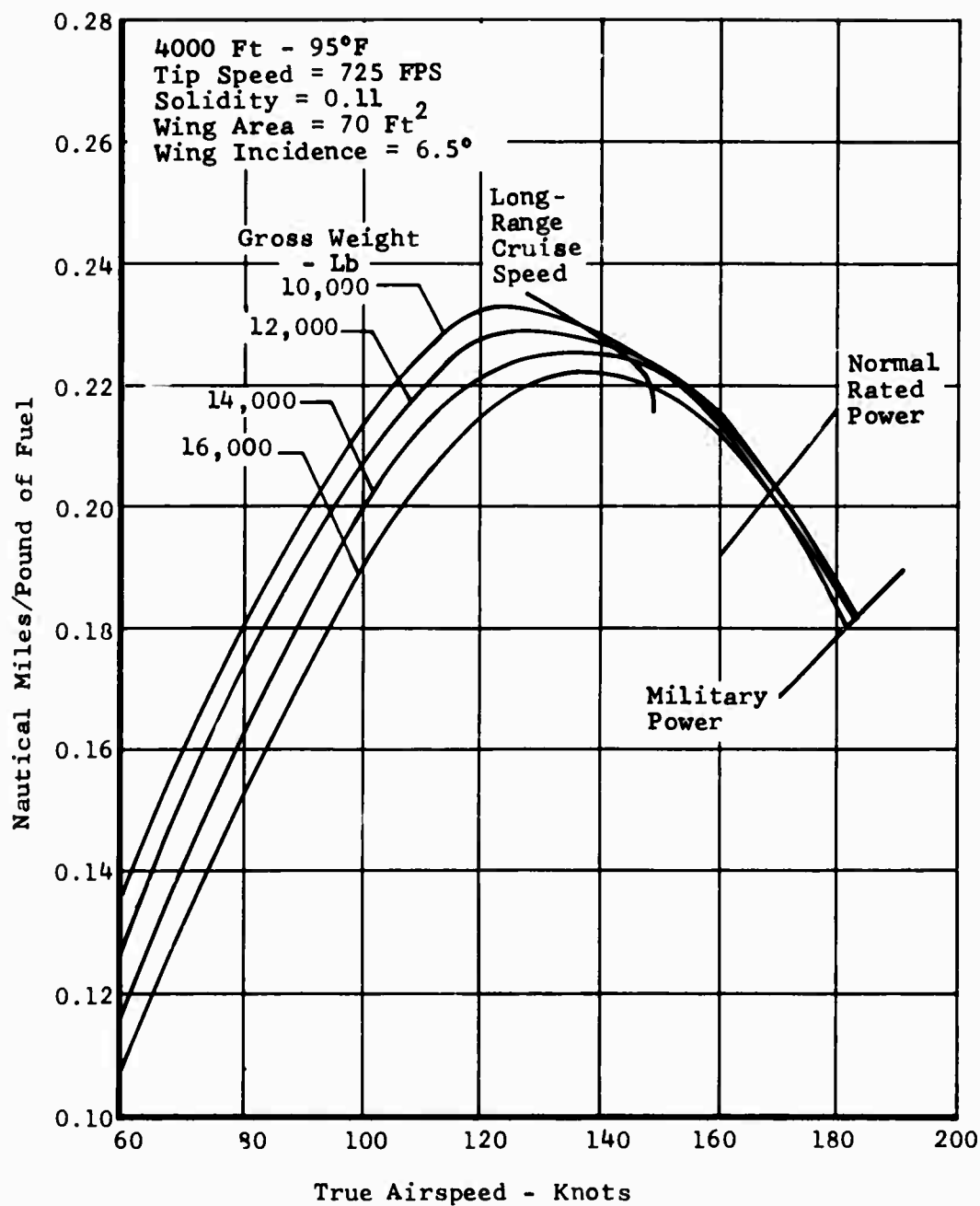
Figure 122. Task II - Winged Helicopter, Specific Range.
