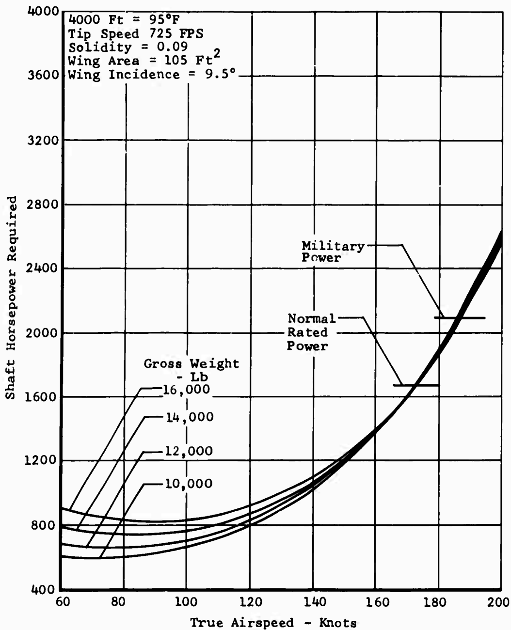
Figure 117. Task II - Winged Helicopter, Speed Power Polar,
