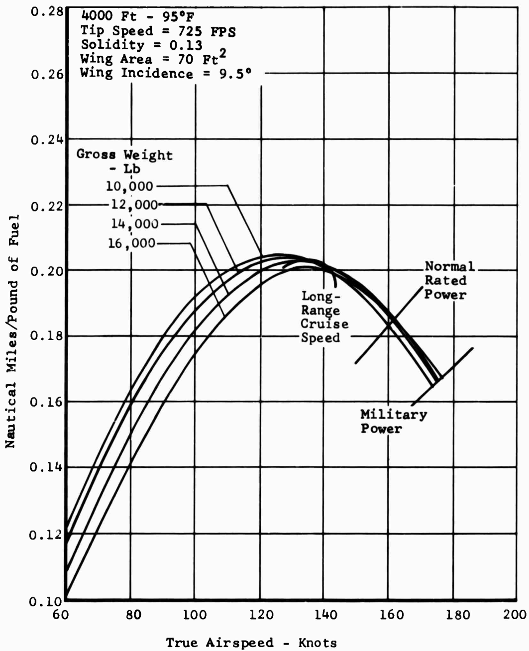
Figure 129. Task II - Winged Helicopter, Specific Range.
