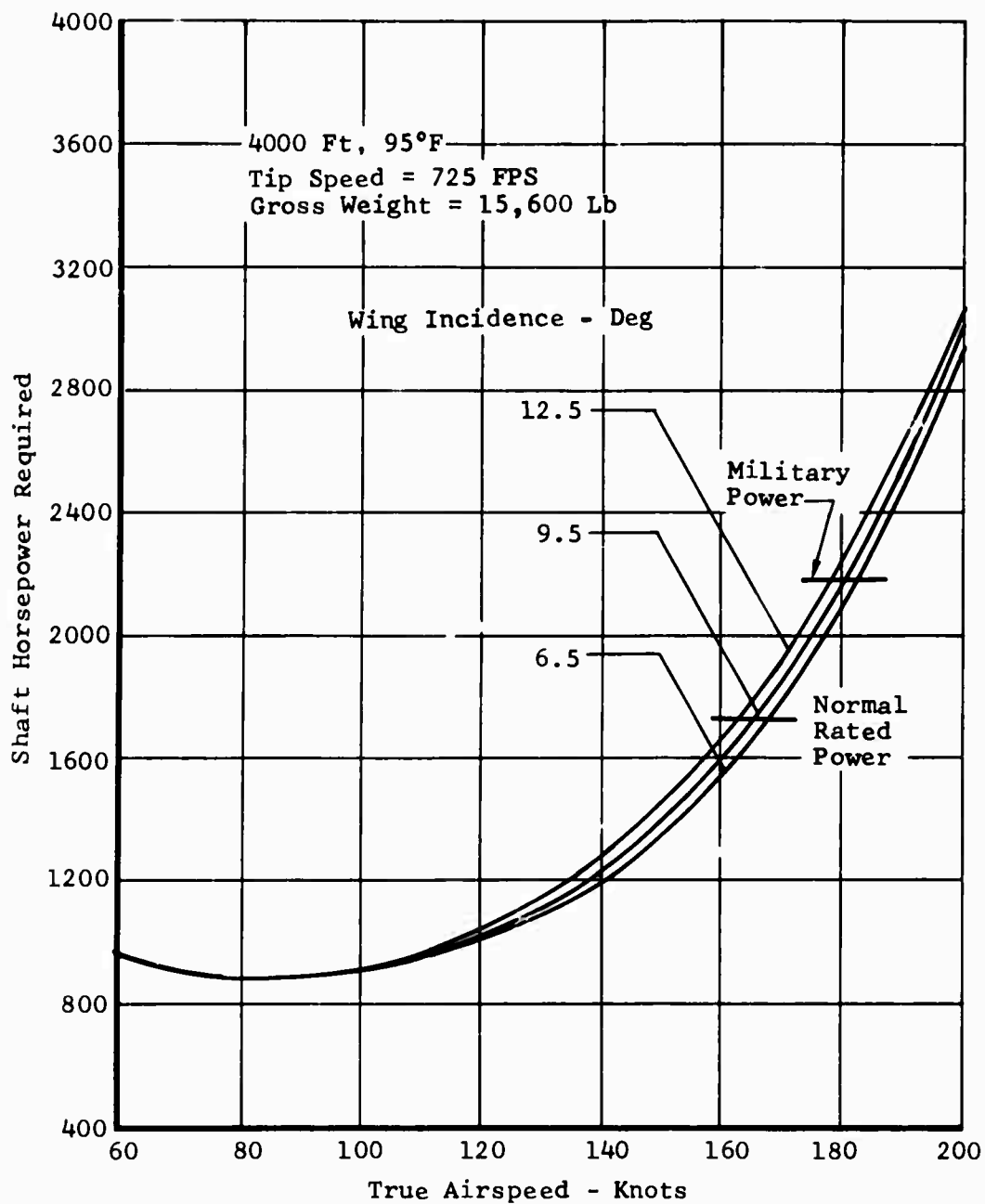
Figure 31. Task II - Winged Helicopter, Speed Power Polar, Solidity = 0.11, Wing Area = 105 Ft 2 .
