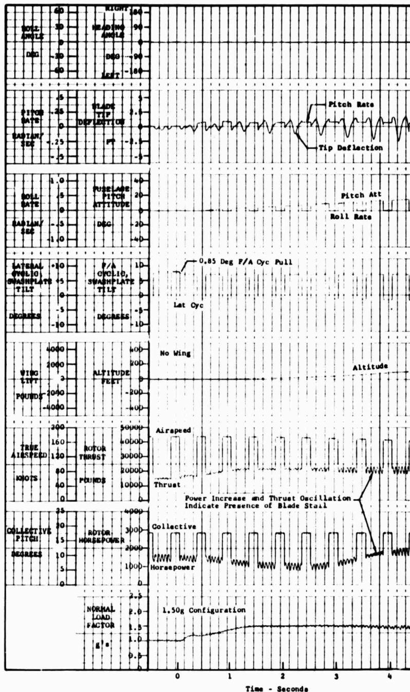
Figure 72. Maneuver Time History, 1.50g Configuration, Limiting Cyclic Pullup at V_{NRP} , Maneuver Limited by Maximum Horsepower.
