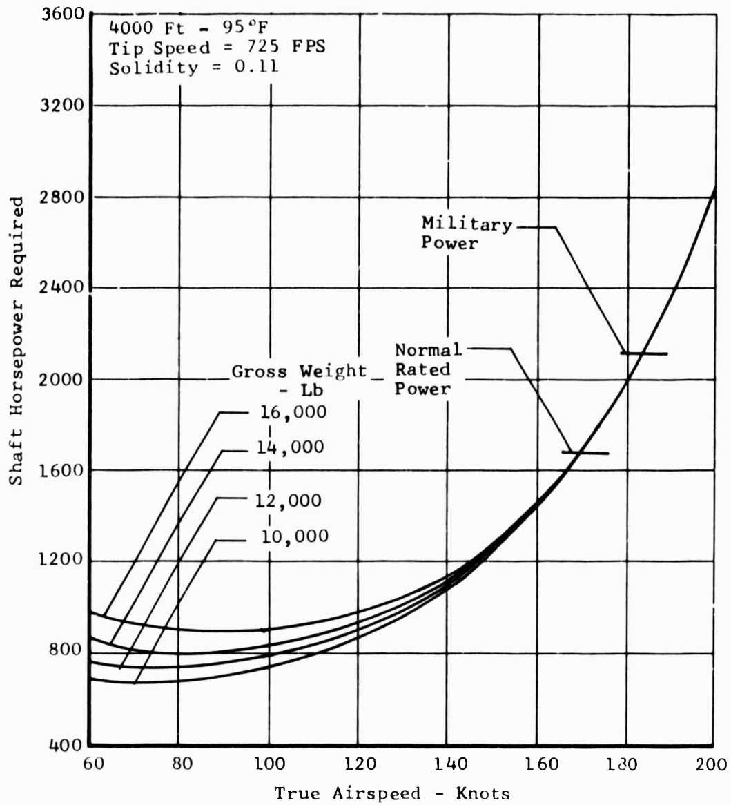
Figure 94. Task I - Wingless Helicopter, Speed Power Polar
