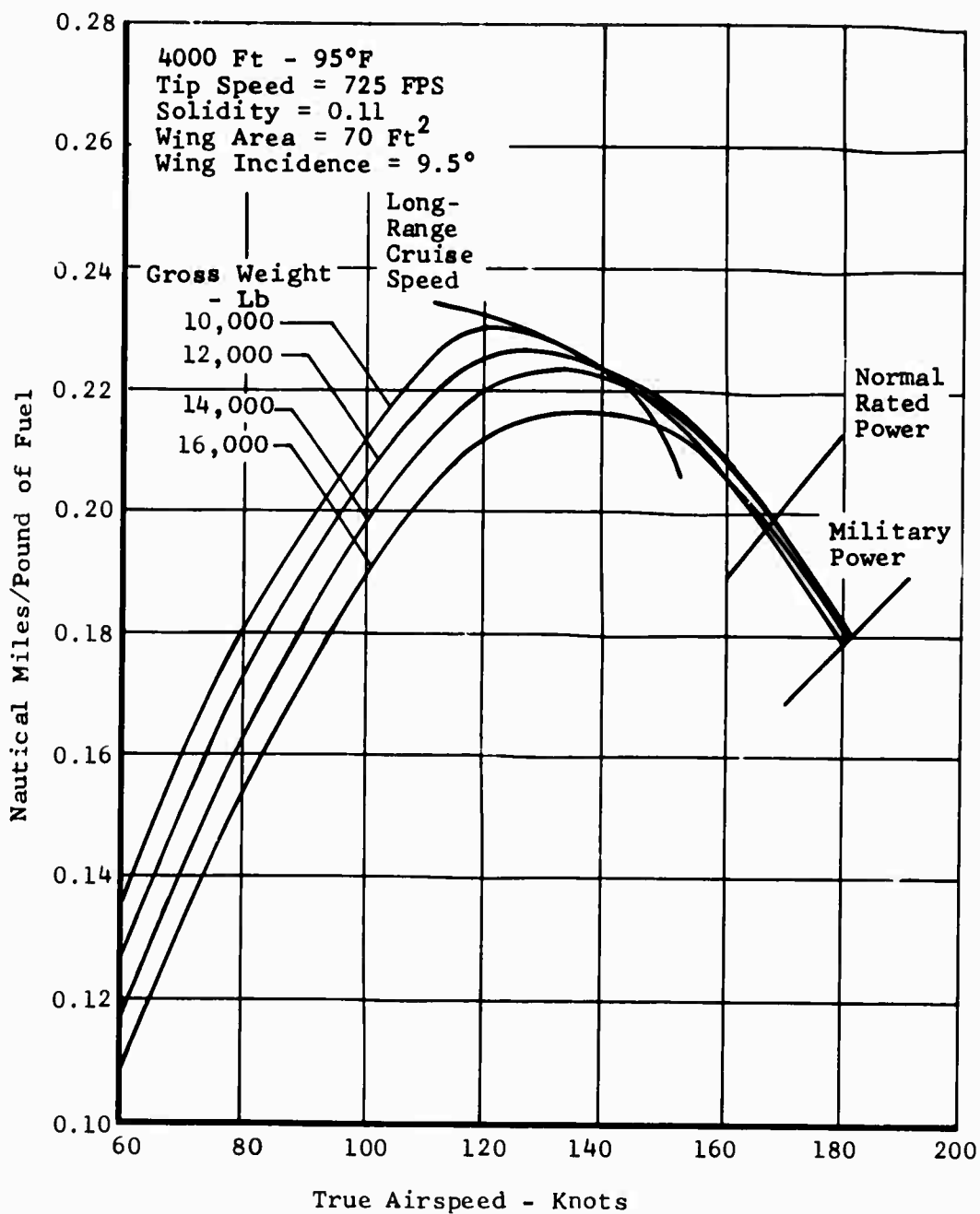
Figure 123. Task II - Winged Helicopter, Specific Range.
