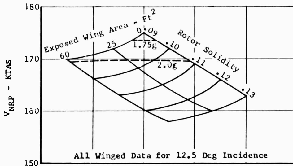
Figure 53. Effects of Rotor Solidity and Wing Area on V_{NRP} and Design g-Capability.
