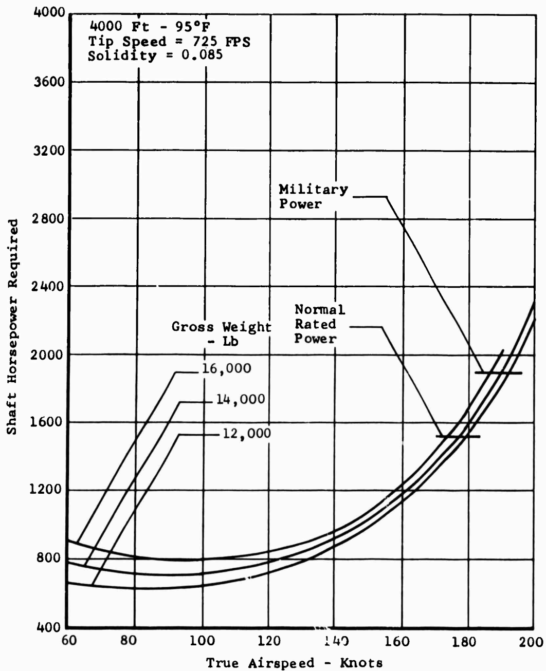
Figure 63. Task III - Wingless Helicopter, Speed Power Polar, 1.50g Design.
