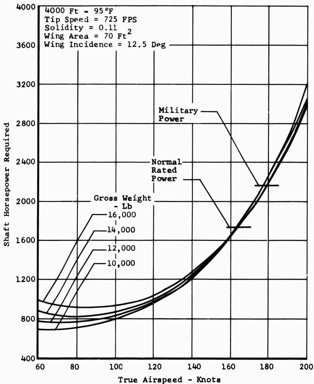
Figure 106. Task II - Winged Helicopter, Speed Power Polar.
