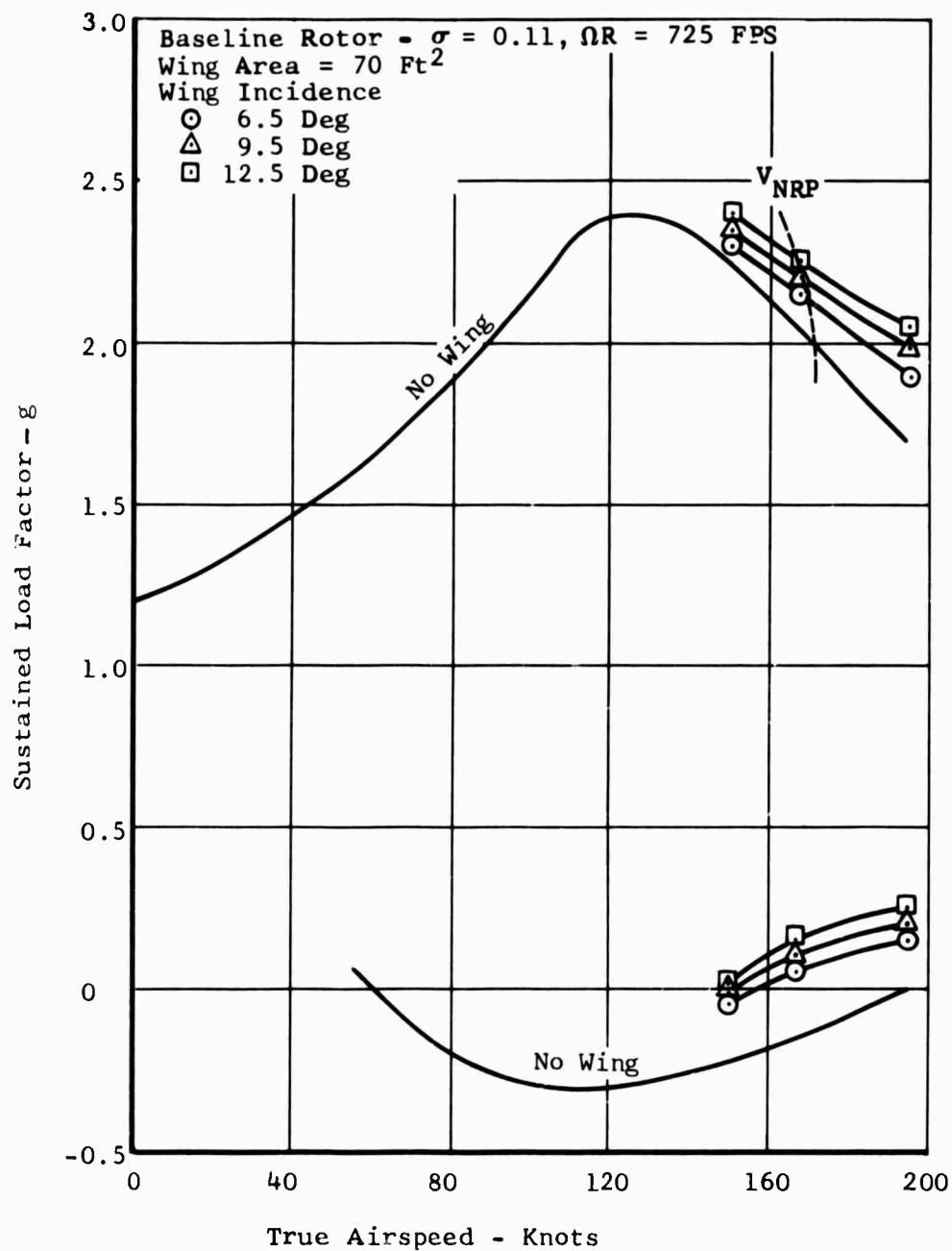
Figure 37. Task II - Maneuver Results, Baseline Rotor, Small Wing.
