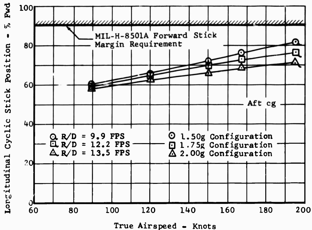
Figure 61. Task III Configurations—Longitudinal Cyclic Stick Position Versus Airspeed.
