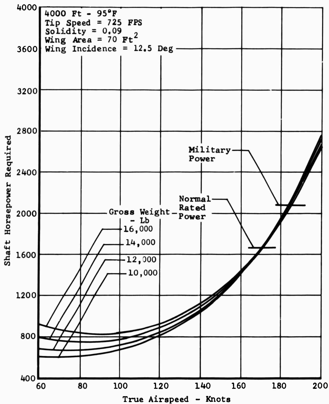
Figure 109. Task II - Winged Helicopter, Speed Power Polar.
