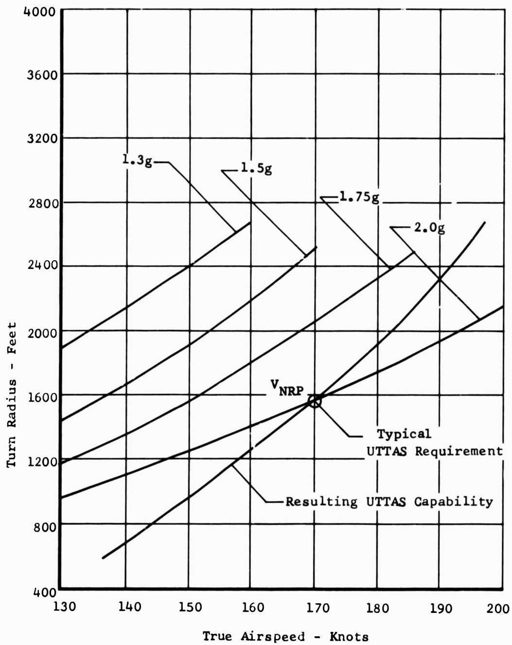
Figure 91. Turn Radius vs Speed.
