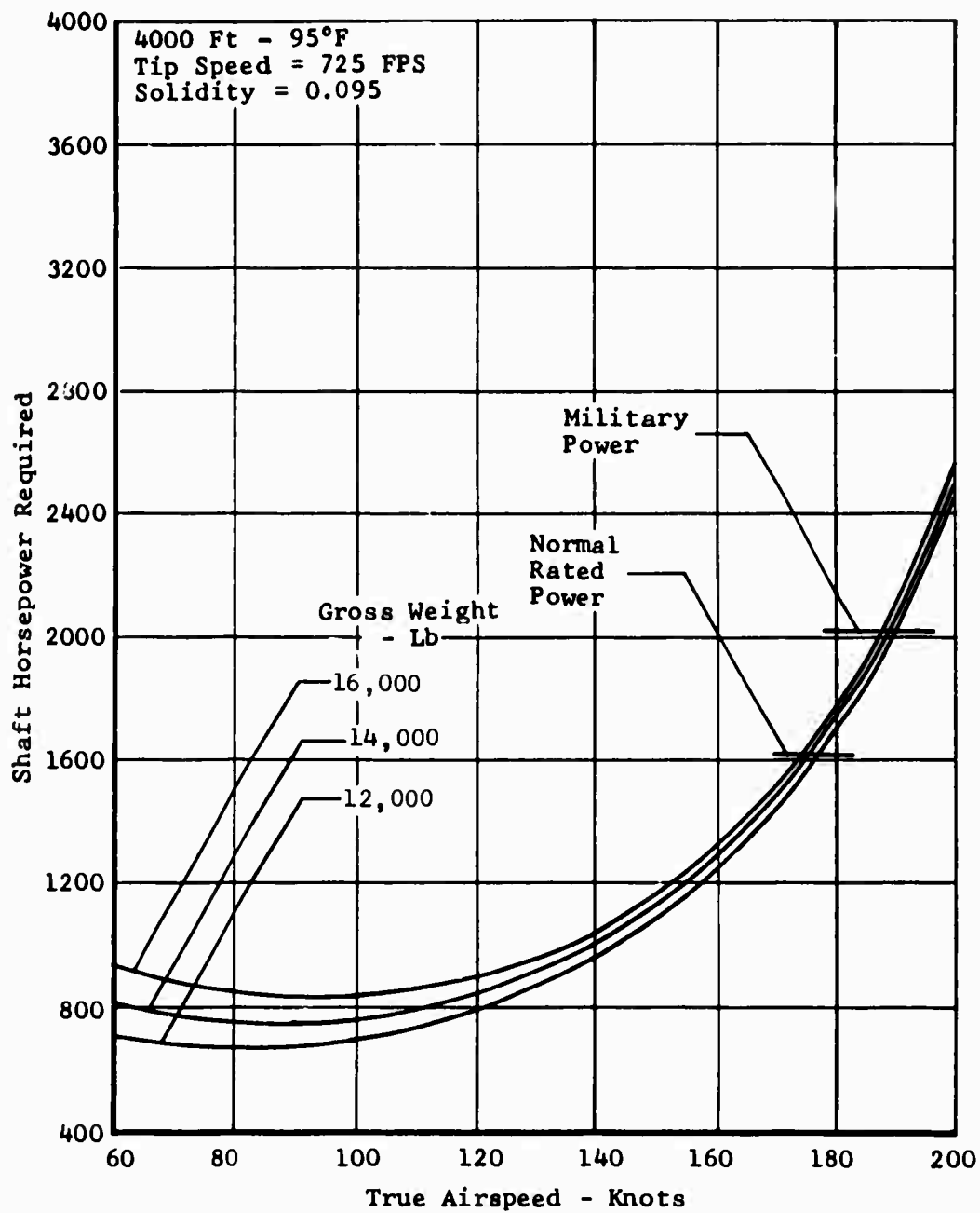
Figure 64. Task III - Wingless Helicopter, Speed Power Polar, 1.75g Design.
