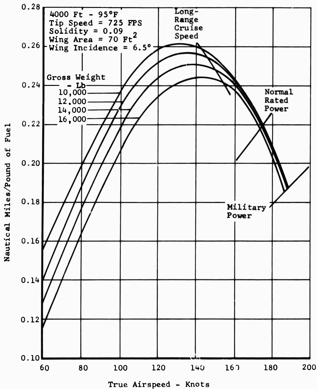
Figure 125. Task II - Winged Helicopter, Specific Range.
