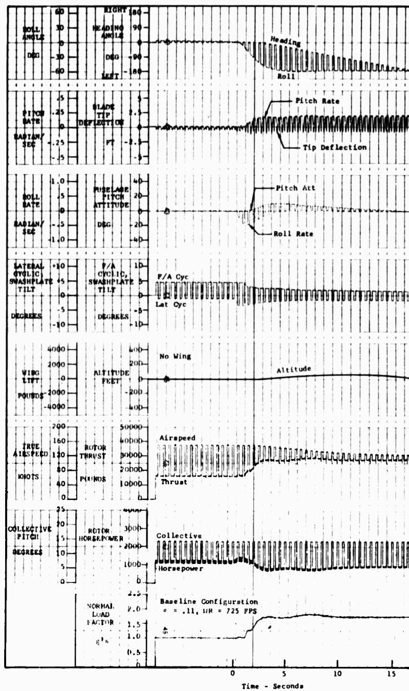
Figure 9. Maneuver Time History, 1.75g Coordinated Turn, Cyclic-Only, Constant Altitude.
