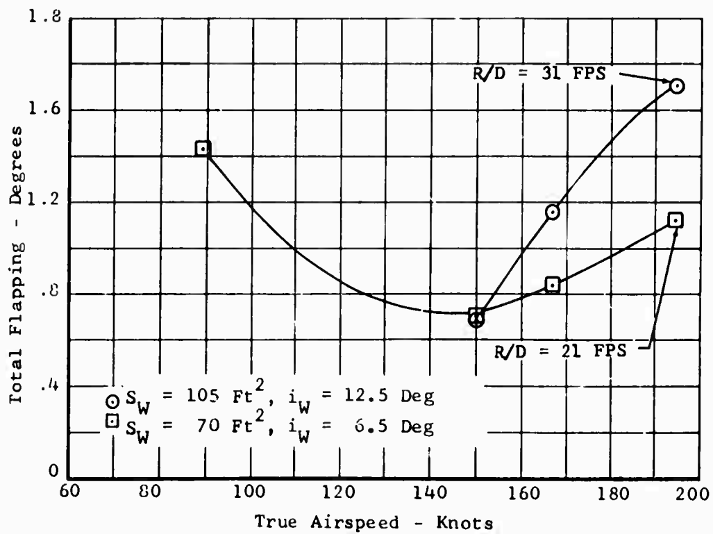
Figure 23. Task II Winged Configurations, Main Rotor Flapping.
