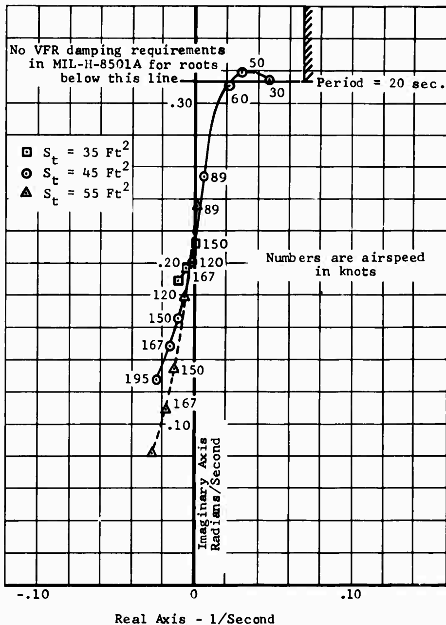
Figure 59. Phugoid Mode Root Locus Plot for 2.0g Configuration, aft cg.
