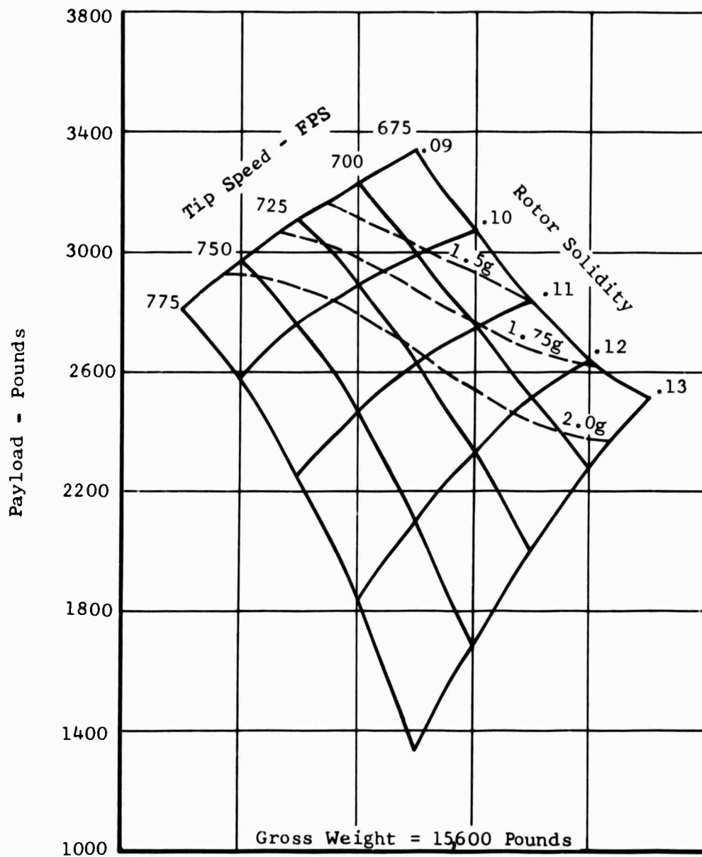
Figure 21. Effects of Rotor Solidity and Tip Speed on Payload and Design g-Capability.
