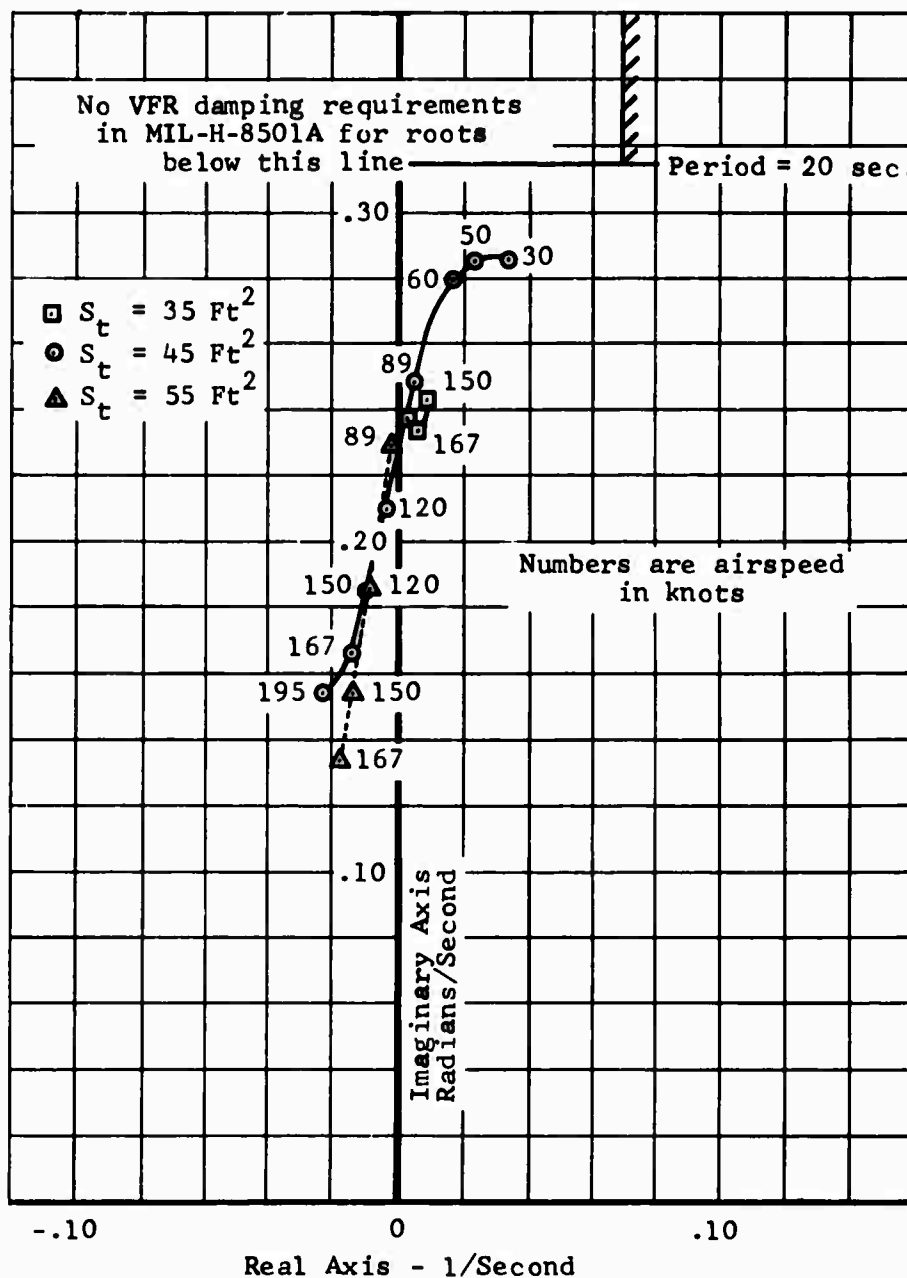
Figure 57. Phugoid Mode Root Locus Plot for 1.5g Configuration, aft cg.
