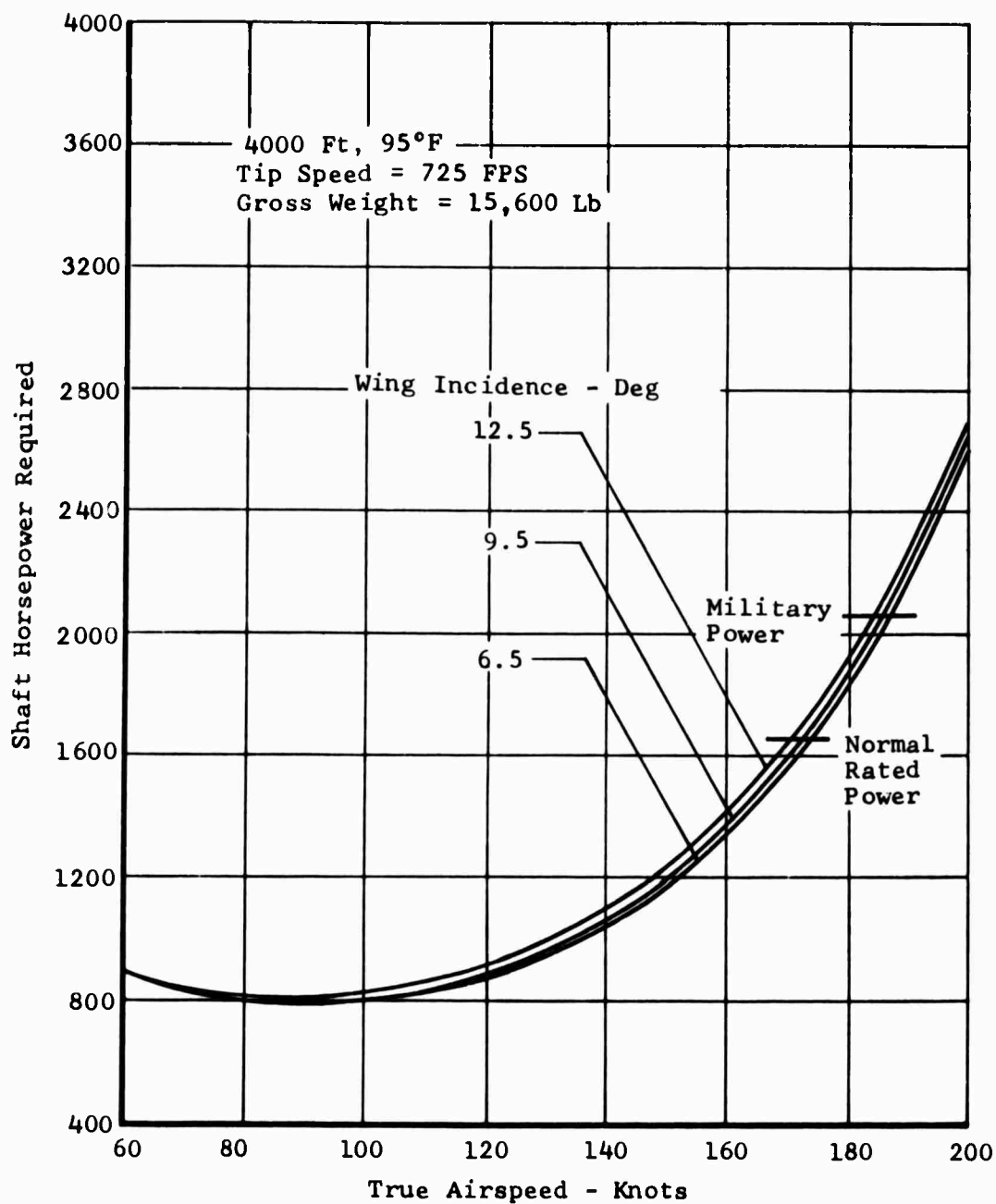
Figure 29. Task II - Winged Helicopter, Speed Power Polar, Solidity = 0.09, Wing Area = 70 Ft 2 .
