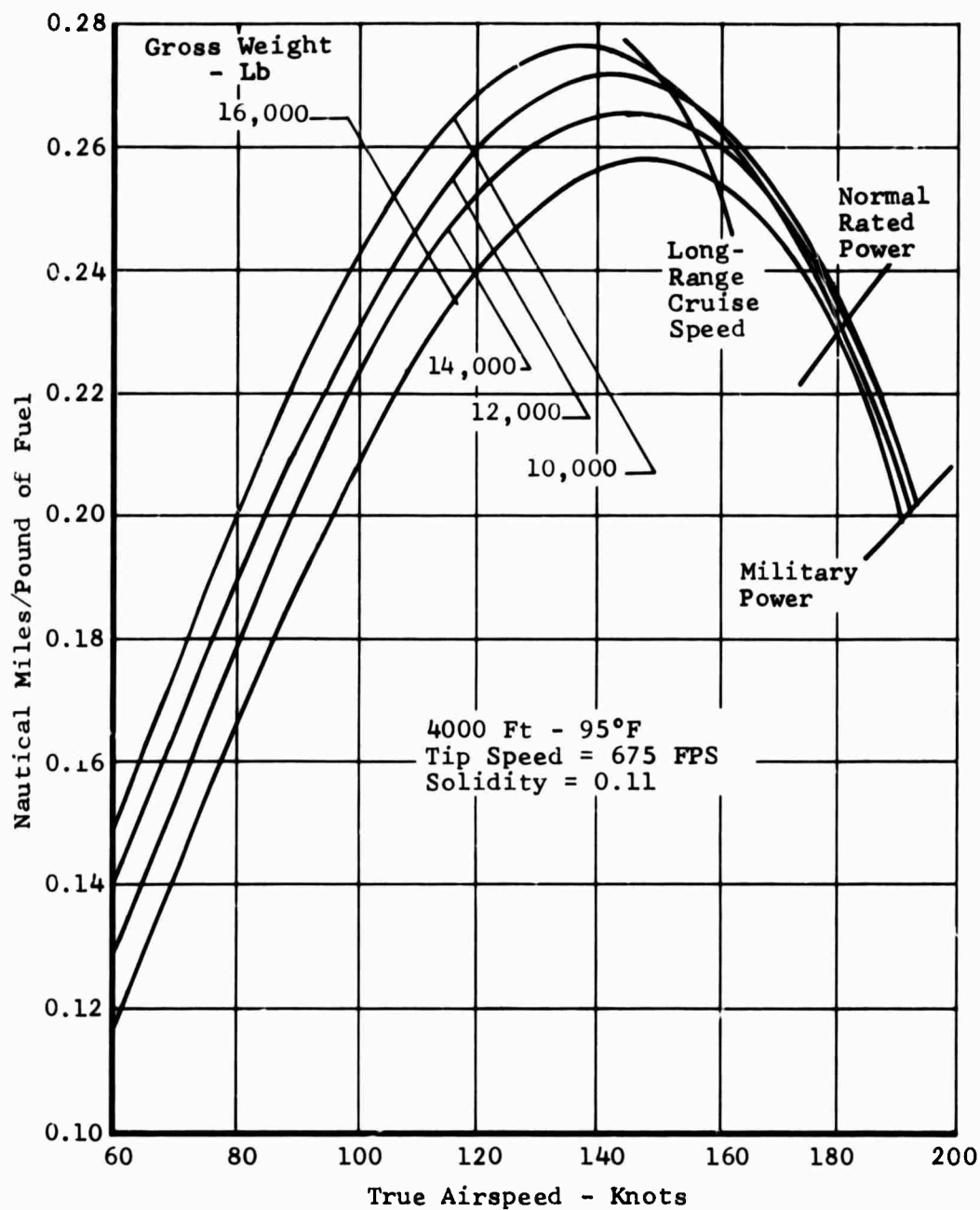
Figure 102. Task I - Wingless Helicopter, Specific Range.
