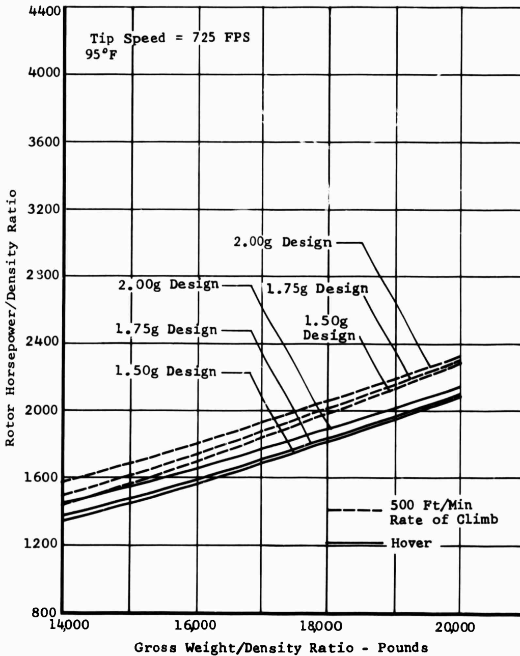
Figure 62. Task III - Wingless Helicopter Hover Power Required.
