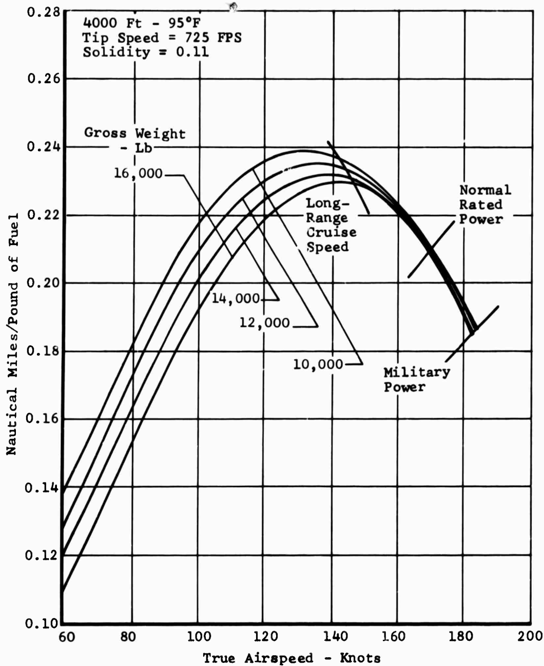
Figure 99. Task I - Wingless Helicopter, Specific Range.
