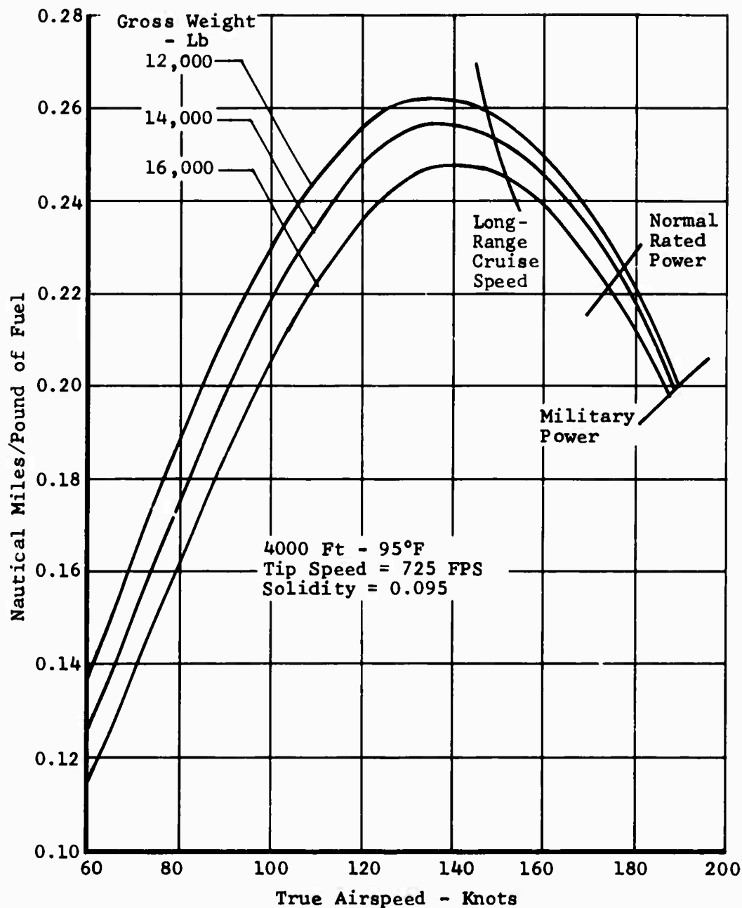
Figure 67. Task III - Wingless Helicopter, Specific Range, 1.75g Design.
