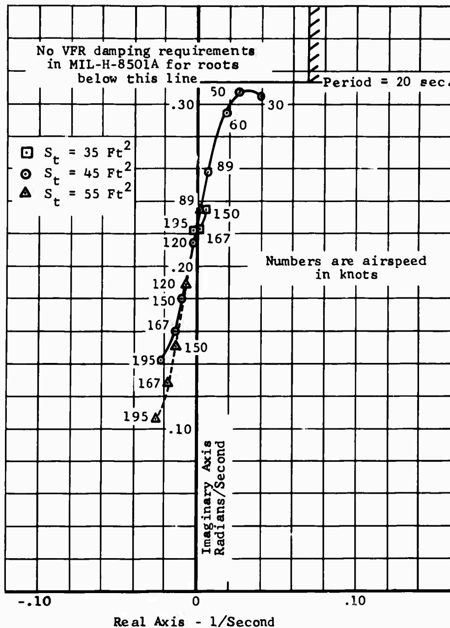
Figure 58. Phugoid Mode Root Locus Plot for 1.75g Configuration, aft cg.
