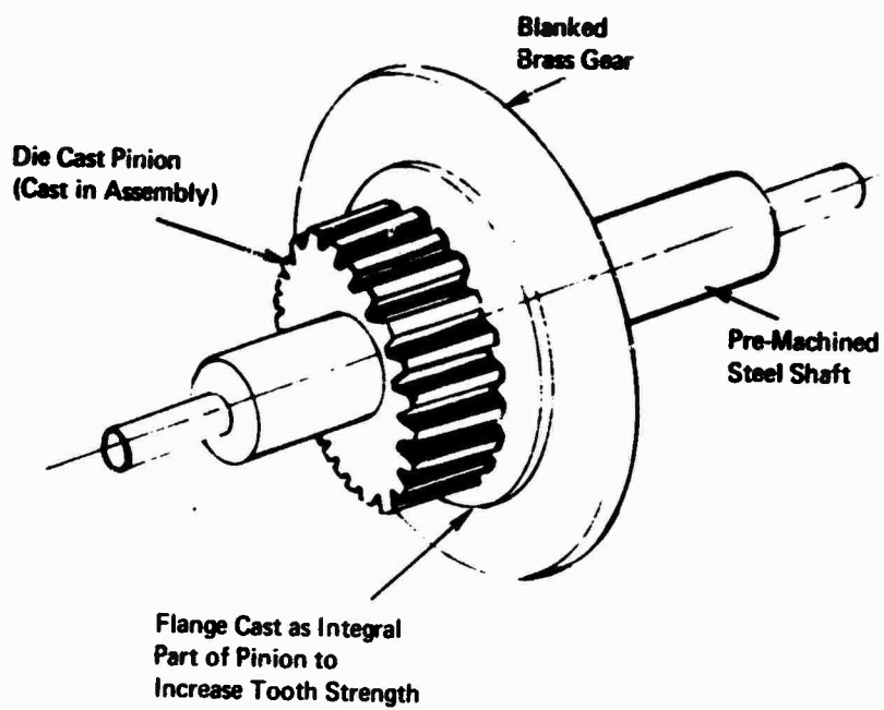
FIGURE 2 Pinion/gear assembly produced by zinc die casting process.
