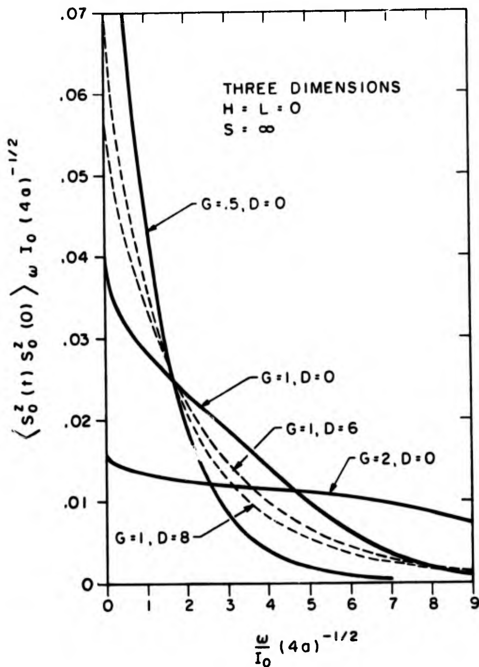
Figure 18. The Frequency Fourier Transforms of the Longitudinal Self-Correlations versus Reduced Frequency, Exchange Anisotropy G With D=0 , and Axial Anisotropy D With G=1 , for a Simple Cubic Lattice of Infinite Spins, With Only Nearest Neighbor Interactions ( H=L=0 ).
