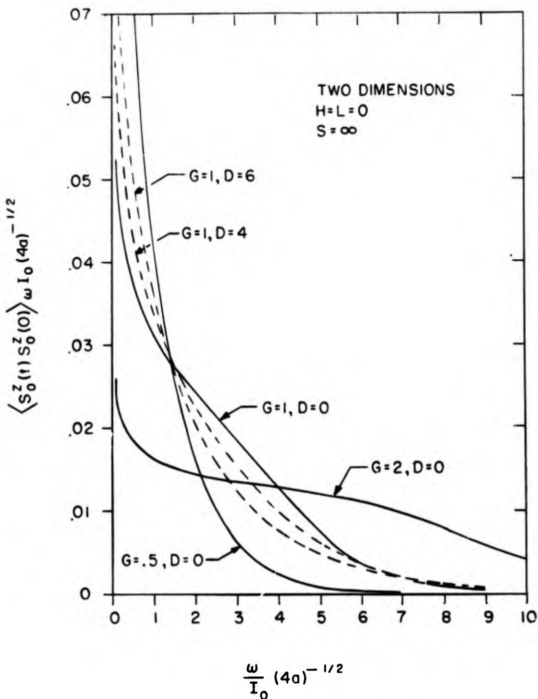
Figure 14. The Frequency Fourier Transforms of the Longitudinal Self-Correlations versus Reduced Frequency, Exchange Anisotropy G With D=0 , and Axial Anisotropy D With G=1 , for a Simple Two-Dimensional Net of Infinite Spins, With Only Nearest Neighbor Interactions ( H=L=0 ).
