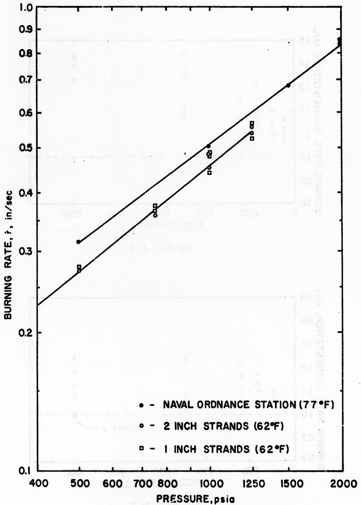
Figure 9. The Effect of Pressure on the Burning Rate of Nonmetallized Double Base Propellant.
