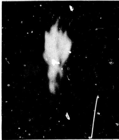
Figure 16. AP/HTPB Sandwich Combustion, 0.004 inch Binder at 0 g's, 400 psia
