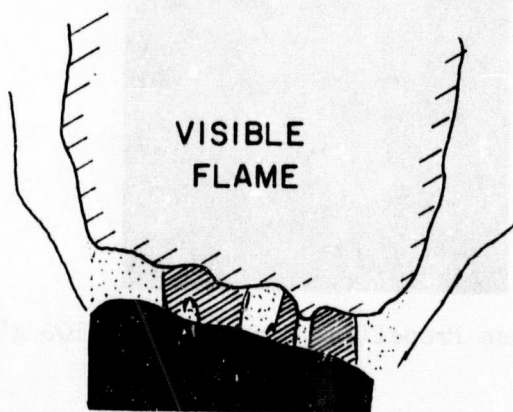
Figure 5. Schematic of Color Schlieren-Double-Base Propellant at 800 psia (horizontal density profile): // Red, . Blue.
