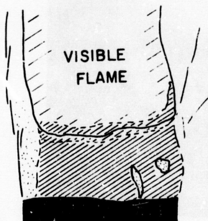
Figure 4. Schematic of Color Schlieren-Double-Base Propellant at 500 psia (vertical density profile): // Red, . Blue.
