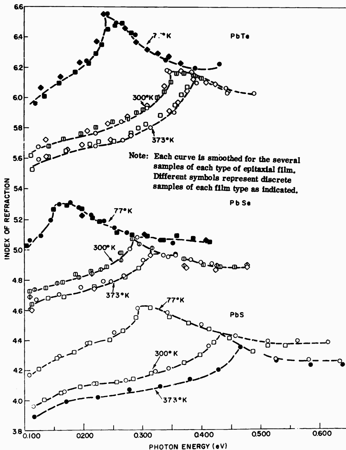
FIGURE 6.4 Variation of the refractive index of epitaxial PbS, PbSe, and PbTe with photon energy (after Zemel, et al 21 )
