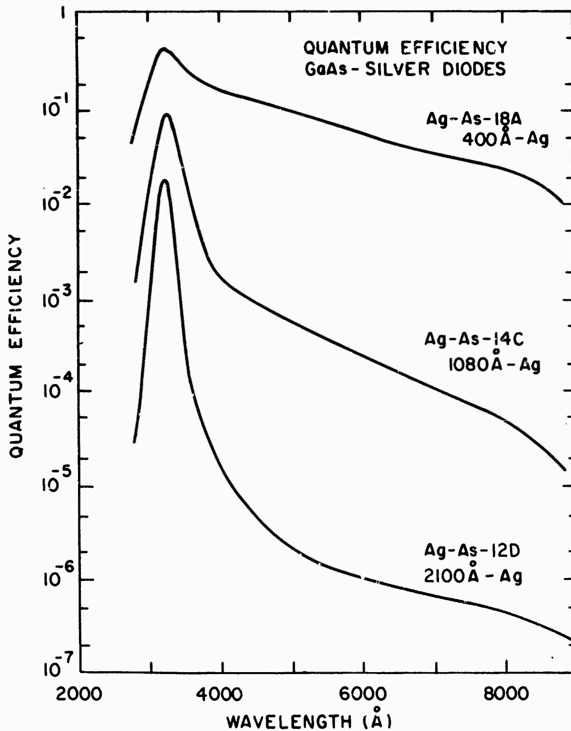
FIGURE 5.20 Spectral response of three Ag-GaAs photodiodes with different silver thickness. (63)
