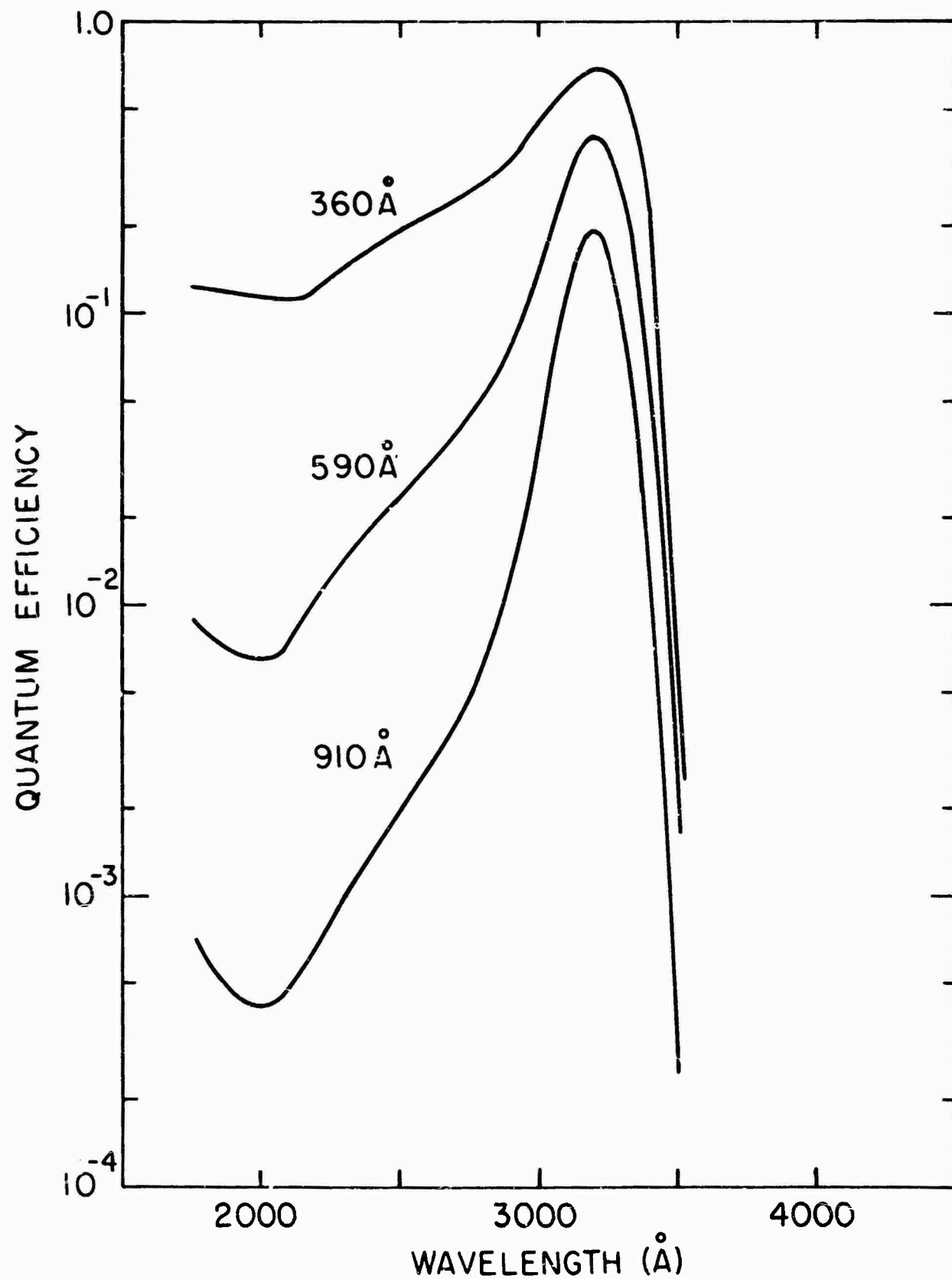
FIGURE 5.17 Measured spectral response of three silver-ZnS photodiodes with different silver thicknesses. (53)
