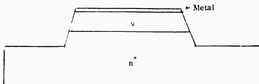
(c) Surface-Barrier (Schottky-Barrier) Photodiode
