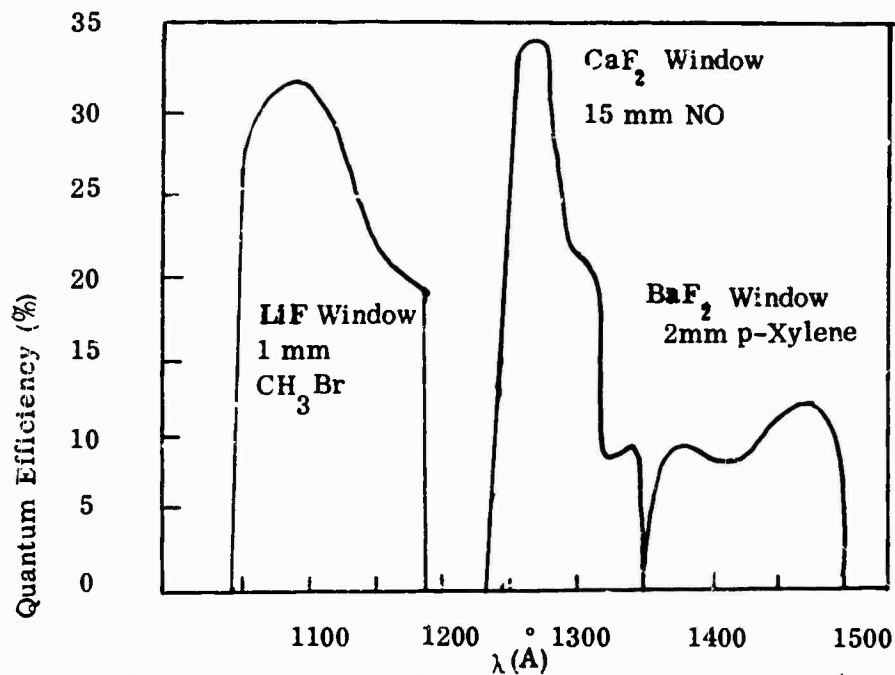
(a) Typical quantum efficiency curves for three fill-gas/window combinations (47).
