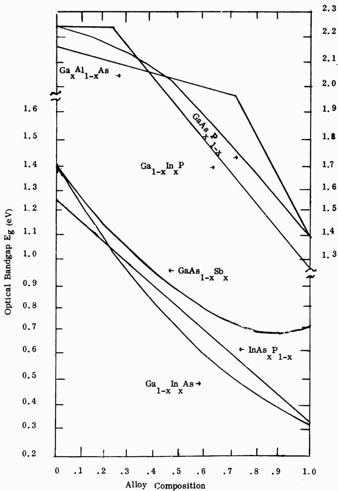
FIGURE 5.9 Bandgap variation of selected III-V alloy composition.
