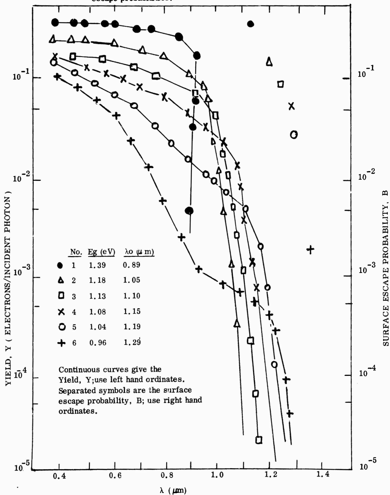
FIGURE 5.10 Spectral responses of opaque GaInAs photocathodes with calculated escape probabilities.
