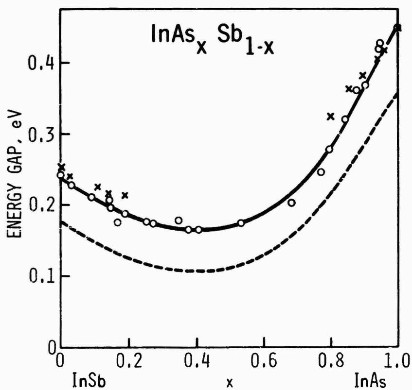
FIGURE 6.8 Dependence of Energy Gap on alloying in \text{InAs}_x \text{Sb}_{1-x} .
