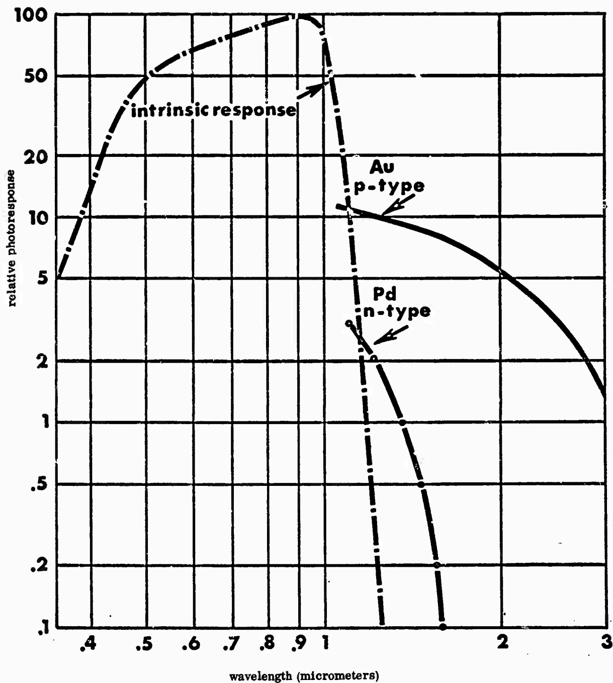
FIGURE 6.11 Extended hot-electron photoresponse.
