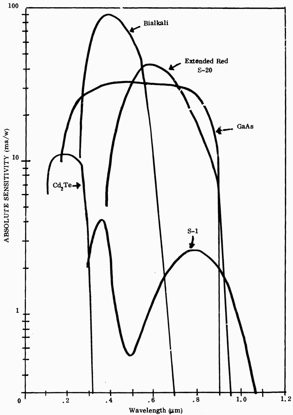
FIGURE 5.7 Spectral Response at Selected Photocathodes (35)
