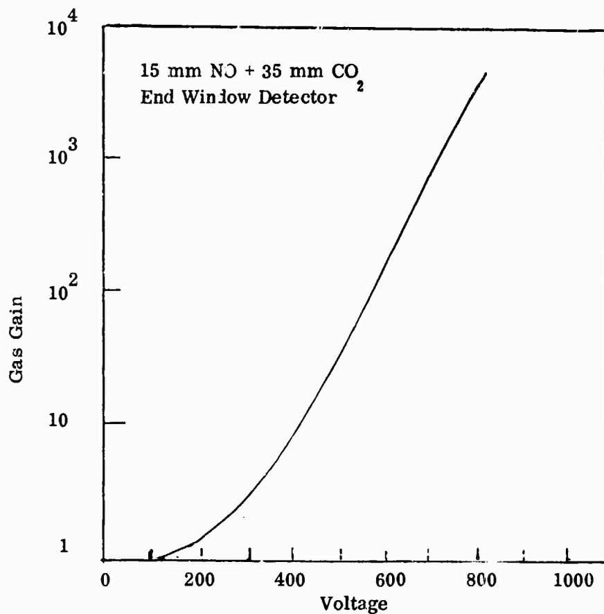
(b) Gain/voltage curve for NO/CO 2 gas ionization device (47).
