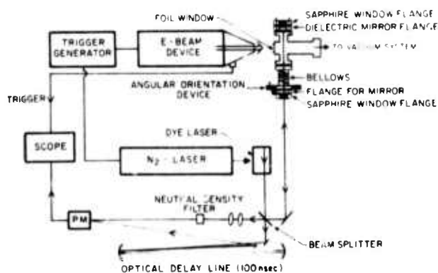
FIG. 1. Experimental system for the direct measurement of gain spectra.
