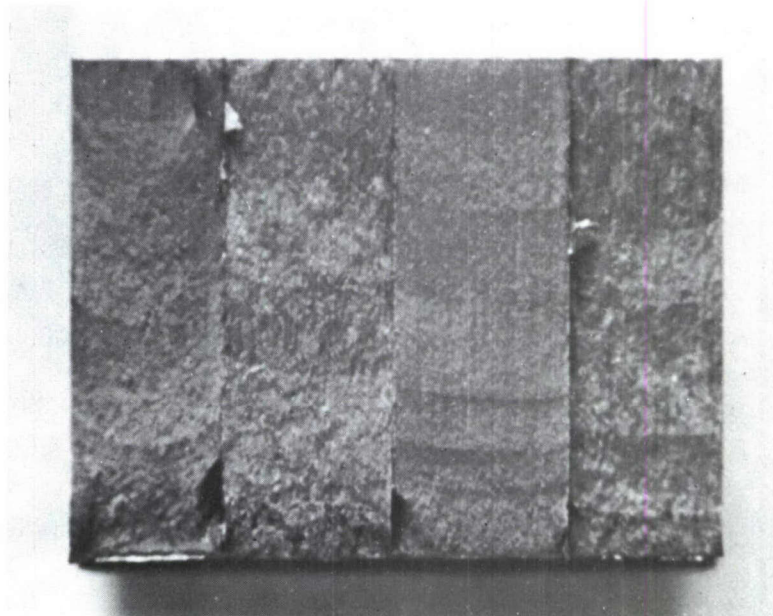
Fig. 12 Fatigue specimen from Billet A showing evidence of crack channeling.
