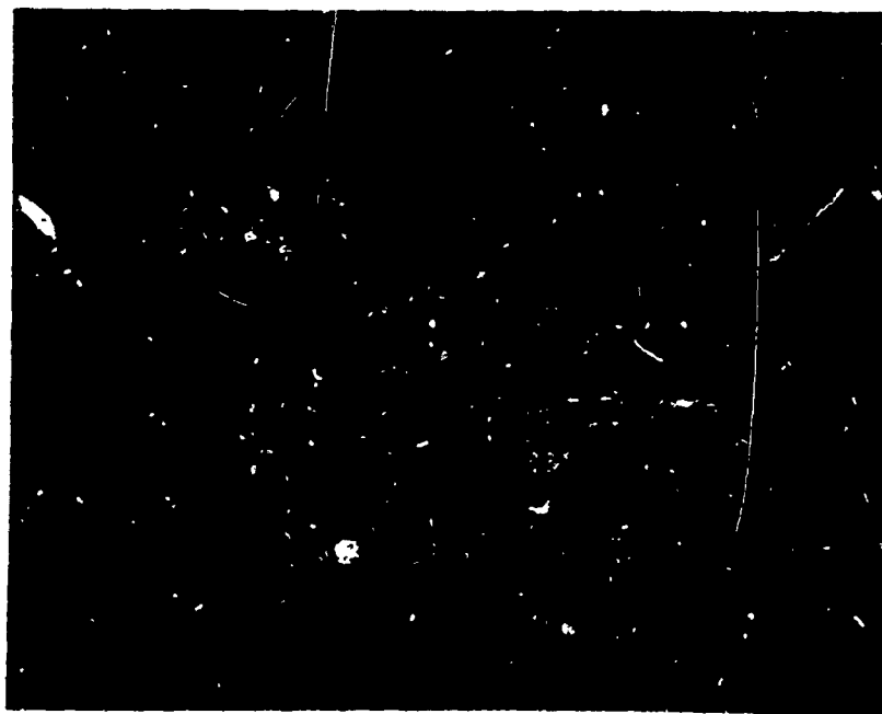
Fig. IV-61A Polishing Damage at the Surface of a Vendor-Obtained, Optically-Polished, Pure KCl Crystal. 150X.
