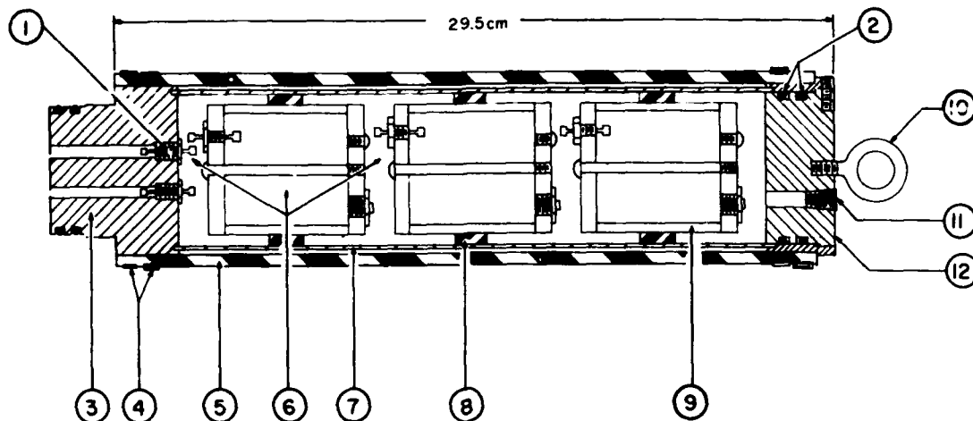
Fig. 2. Principal design features of H62 hydrophone: (1) glass-to-metal seal, Fusite 105 TB-FP; (2) O-rings; (3) anodized aluminum; (4) punch-lok clamp, SST 316; (5) butyl rubber boot; (6) Baker's DB grade castor oil; (7) expanded aluminum; (8) rubber mount; (9) ceramic sensor element; (10) eyebolt, SST 304; (11) oil filler plug; (12) anodized aluminum end plate.
