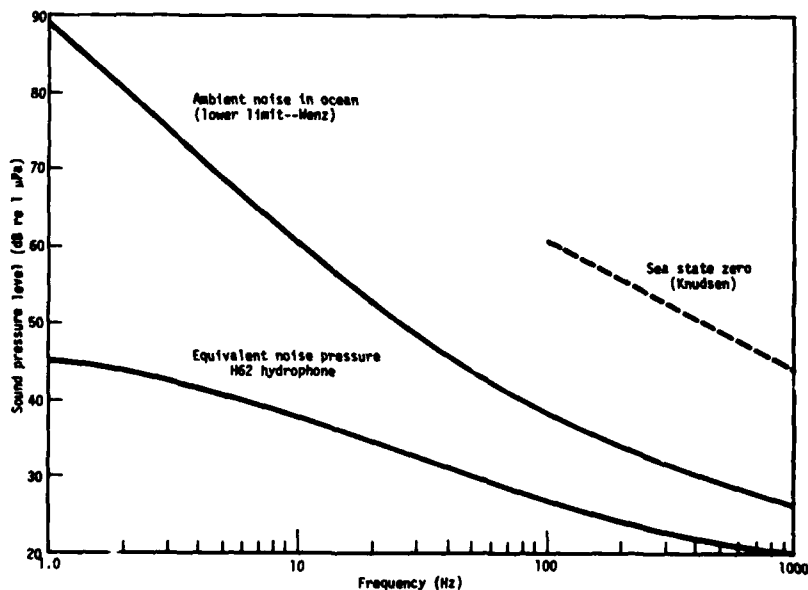
Fig. 14. Equivalent noise pressure of the H62 hydrophone when equipped with a USRD preamplifier and a sensor whose open-circuit crystal sensitivity is -180 dB re 1 V/ \mu Pa with a capacitance of 3300 pF.
