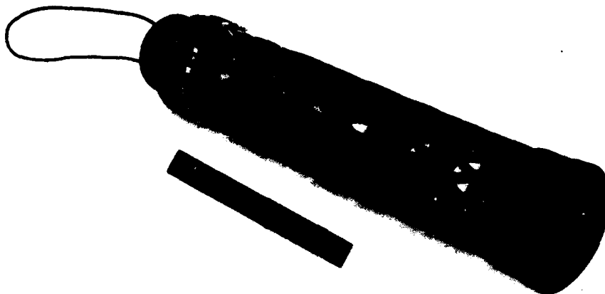
Fig. 15. Sensor head with the three ceramic cylinders mounted in the expanded aluminum tube.
