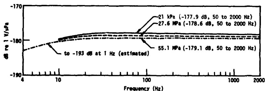
Fig. 17. Free-field voltage sensitivity of H62 hydrophone with 10-Hz cutoff at 3°C (average of serials 1Y through 8Y).
