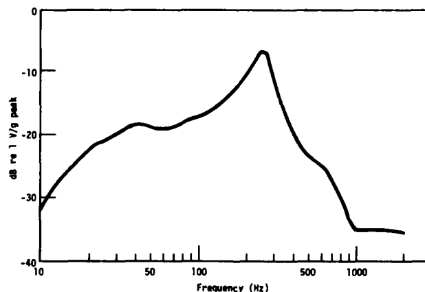
Fig. 5. Acceleration sensitivity of the type H62 hydrophone, measured parallel to the longitudinal axis (sensitivity of sensor, -177 dB re 1 V/ \mu Pa).
