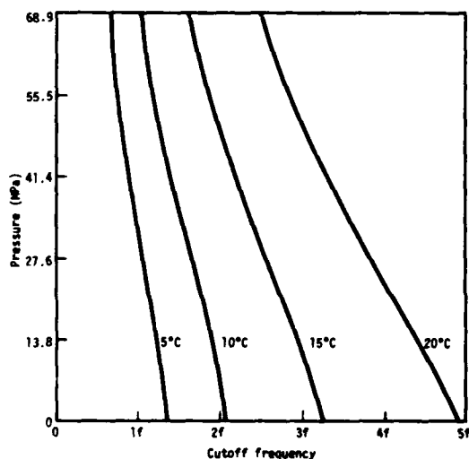
Fig. 4. Cutoff frequency of H62 hydrophone as a function of temperature and pressure ( f is cutoff frequency, 3-dB-down point, set at 5°C and 34.5 MPa).
