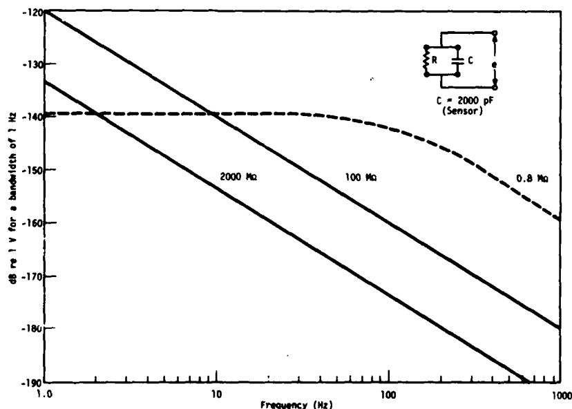
Fig. 9. Noise voltage produced in a 1-Hz bandwidth by a parallel resistance-capacitance combination equivalent to the ceramic sensor shunted by a resistor.
