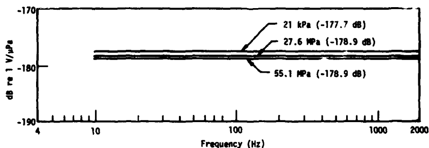
Fig. 16. Free-field voltage sensitivity of H62 hydrophone with 1-Hz cutoff at 3°C.
