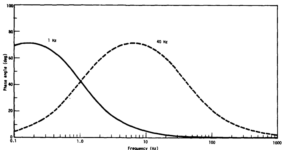
Fig. 7. Phase difference between H62 hydrophone output voltage and the sound pressure at the hydrophone with sensor elements compensated by small orifice to give 1- and 40-Hz cutoff.
