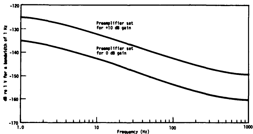
Fig. 13. Noise voltage measured at the output of the H62 hydrophone preamplifier with a source capacitance of 3300\text{ pF} and a resistance greater than 500\text{ M}\Omega .
