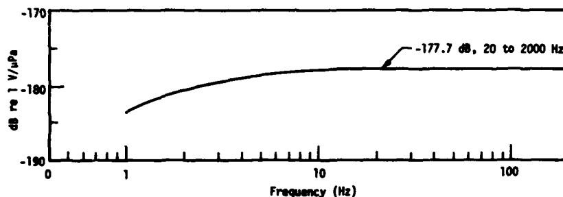
Fig. 18. Free-field voltage sensitivity of H62 hydrophones with 1-Hz cutoff at 3°C under the pressures 21 kPa and 6.89 MPa.
