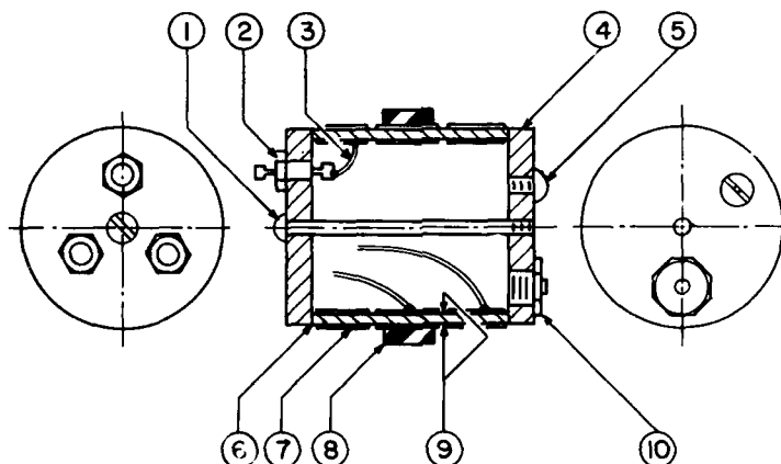
Fig. 6. Construction details for the capped ceramic cylinder used as a sensor element in the H62 hydrophone: (1) tie bolt; (2) glass-to-metal seal; (3) hookup wire; (4) end cap, SST 303; (5) orifice plug; (6) Epon VI epoxy cement; (7) silver electrode; (8) rubber mount, type W neoprene; (9) electrode removed inside and outside; (10) relief valve, Alemite No. 47640.
