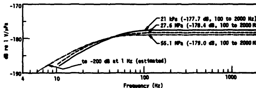
Fig. 19. Free-field voltage sensitivity of H62 hydrophone with 30-Hz cutoff at 20°C (average of serials 1Y through 8Y).
