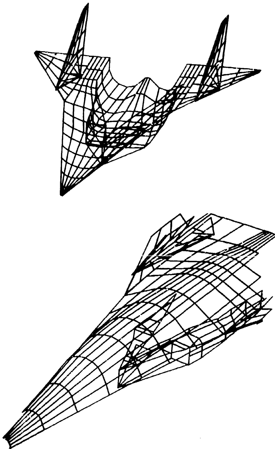
Figure B-4 (cont.) Geometry Checkout Using Off-Line SD-4060 Program.
