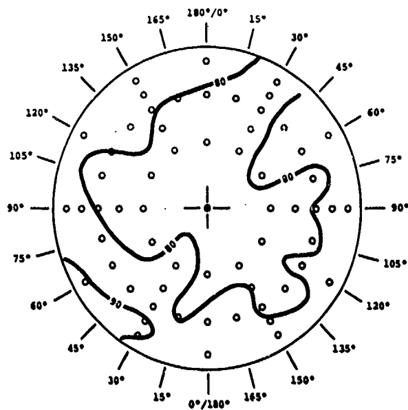
Figure 168. T55 Engine Isopleth of NO (ppm) at 100% Power.
