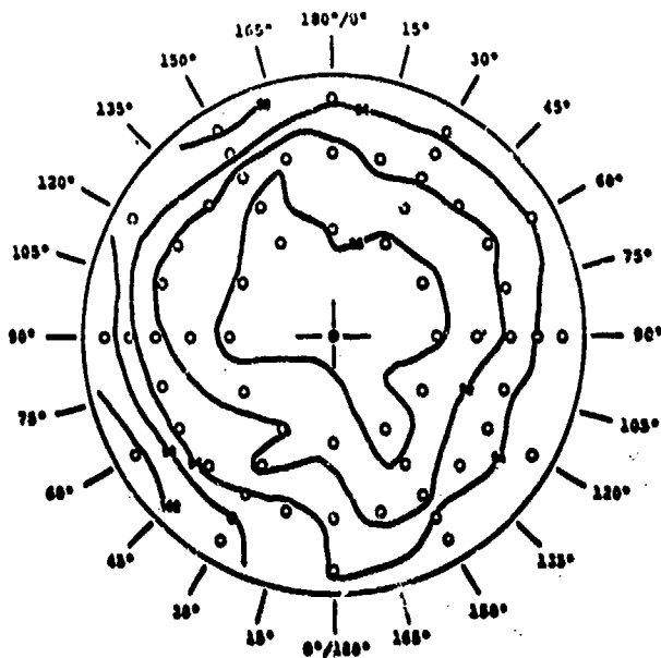
Figure 169. T55 Engine Isopleth of NO x (ppm) at 100% Power.
