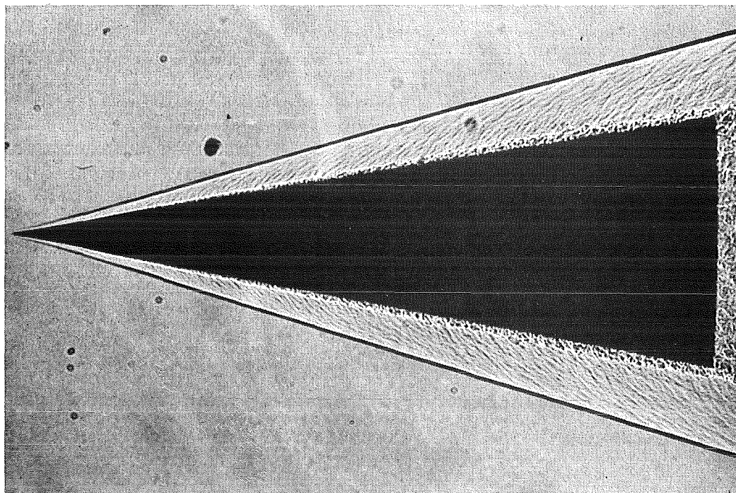
Figure 11. Cone at Mach 5.1 with distributed 1700 \mu\text{in.}-\text{rms} roughness.
