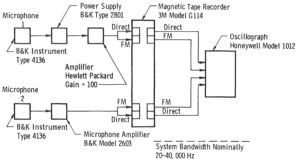
Figure 4. Sound pressure data recording system.
