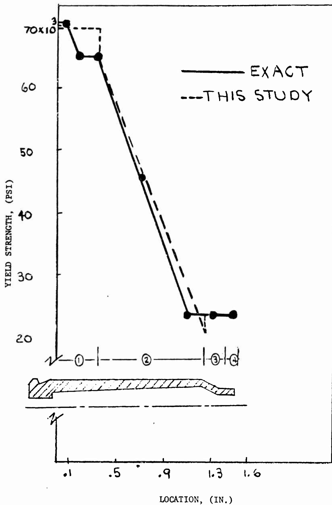
Figure 6. Yield Strength Variation Within the Aluminum Case
