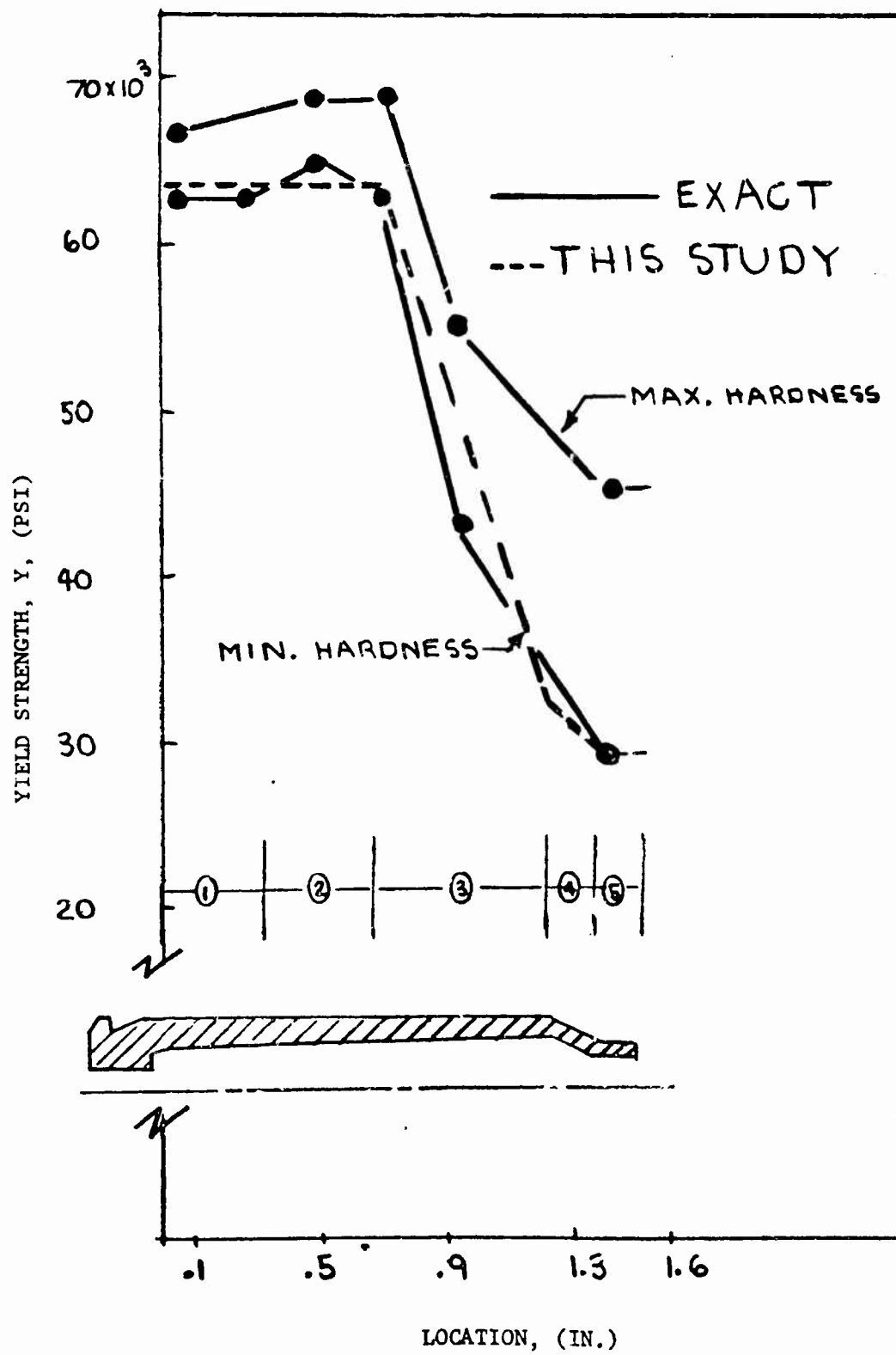
Figure 5. Yield Strength Variation Within the Brass Case
