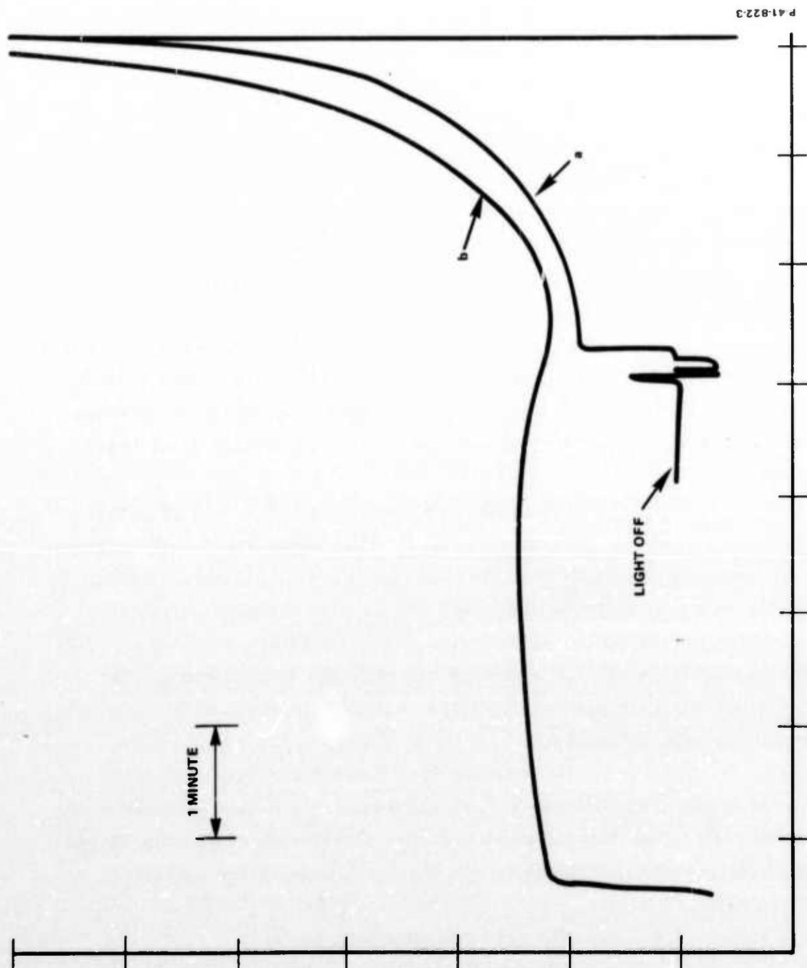
Figure 19 - OSEE from c - face of LiNbO 3 ( t_d = 0 ). Run "b" was taken immediately after "a".
