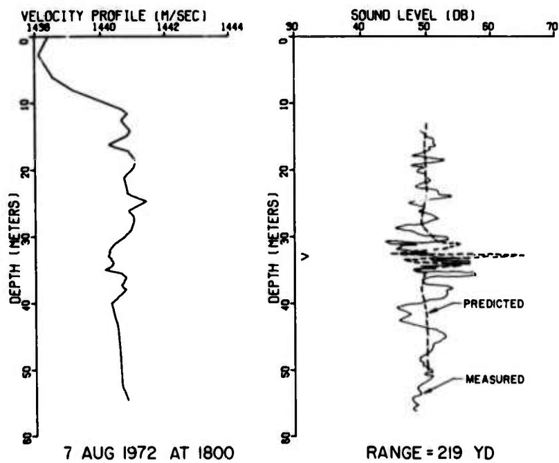
Figure 63. Comparison of measured to predicted sound level profiles, cont.
