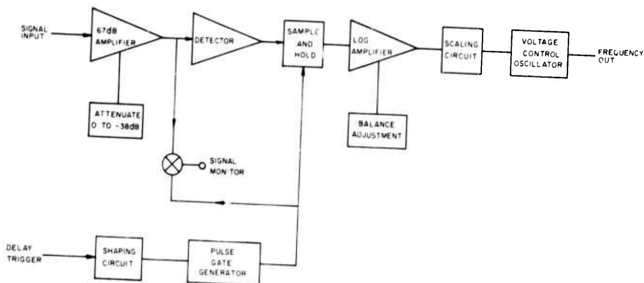
Figure 57. Block diagram of the acoustic receiver.
