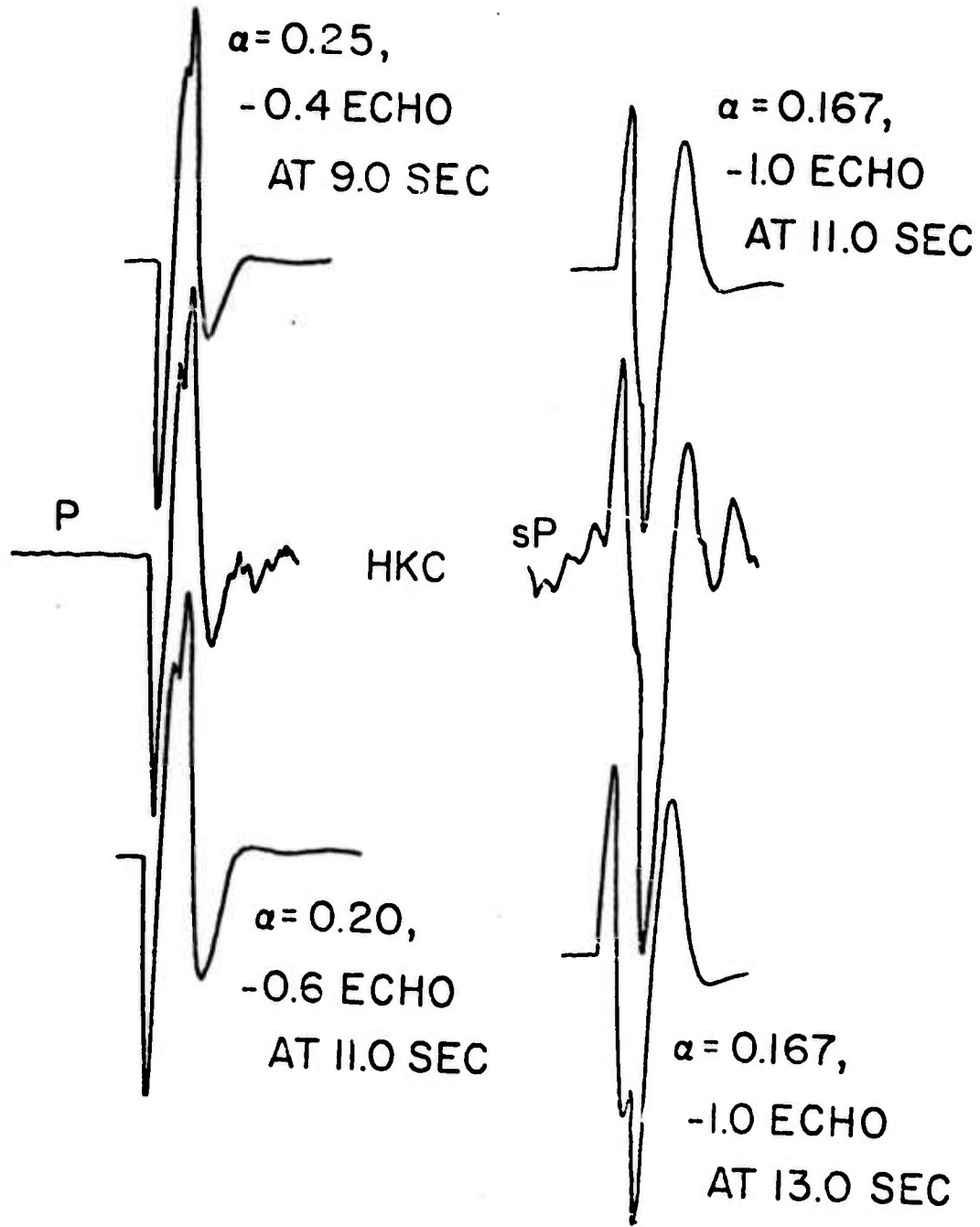
Fig. 3.6. P wave from the Aug. 30, 1970 earthquake in the Sea of Okhotsk. The LPZ record from Hong Kong (HKC) is shown as an example. On this and other records there appears to be a strong negative phase at about 12 sec after the initial arrival. Comparison among numerous high quality records from this earthquake indicate that this negative event is a source effect and not an effect of the propagation path.
