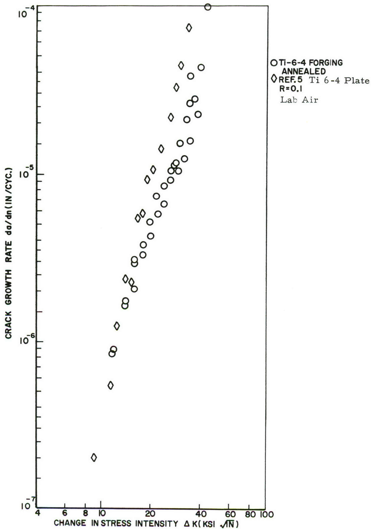
Figure 8. Crack Growth Rates of Ti-6Al-4V Forging and Plate (Reference 5).
