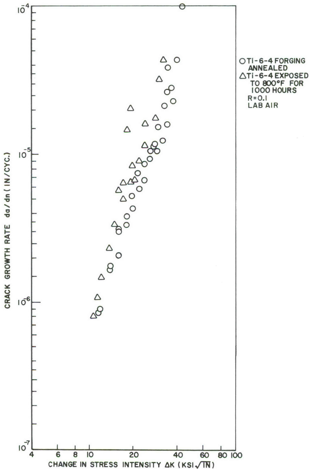
Figure 7. Crack Growth Rates of Ti-6Al-4V Forging.
