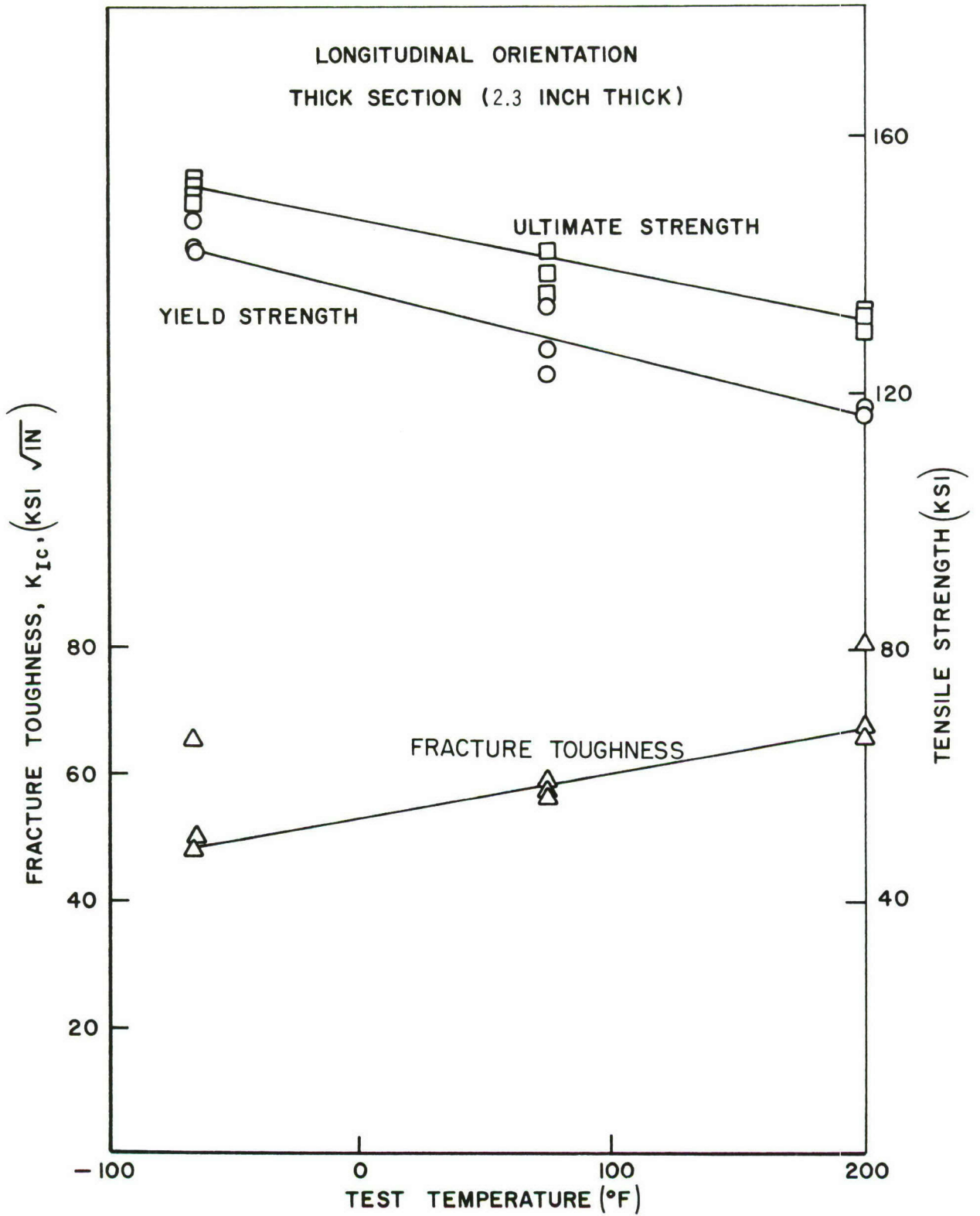
Figure 6. Ti-6Al-4V Forging Mechanical Properties variation with temperature.
