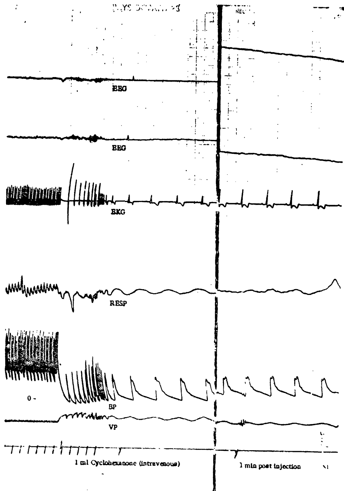
Figure A-9. Effects of Cyclohexanone Upon Physiologic Parameters of an Anesthetized Dog (1 min)
