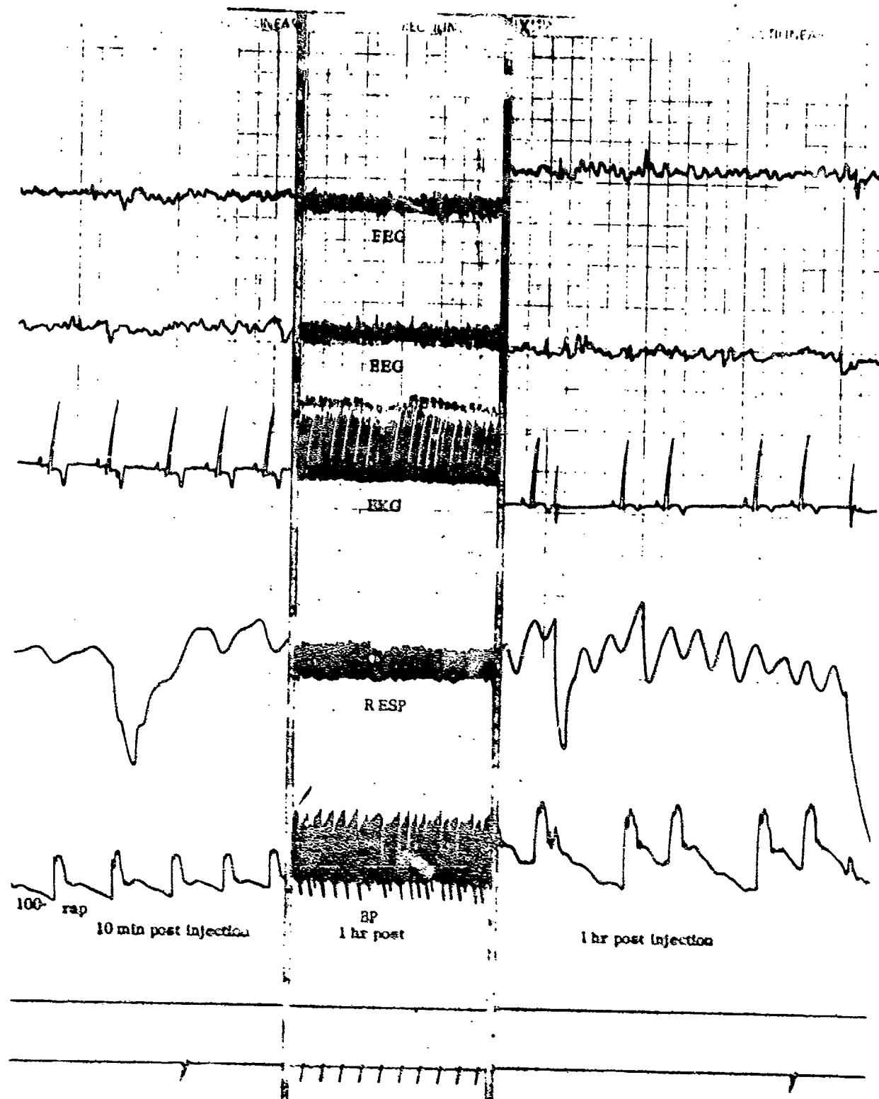
Figure A-17. Effects of Intravenous Administration of 10 mg/kg HMX-DMSO Upon Physiologic Parameters of an Unanesthetized Dog (10 min and 1 hr)
