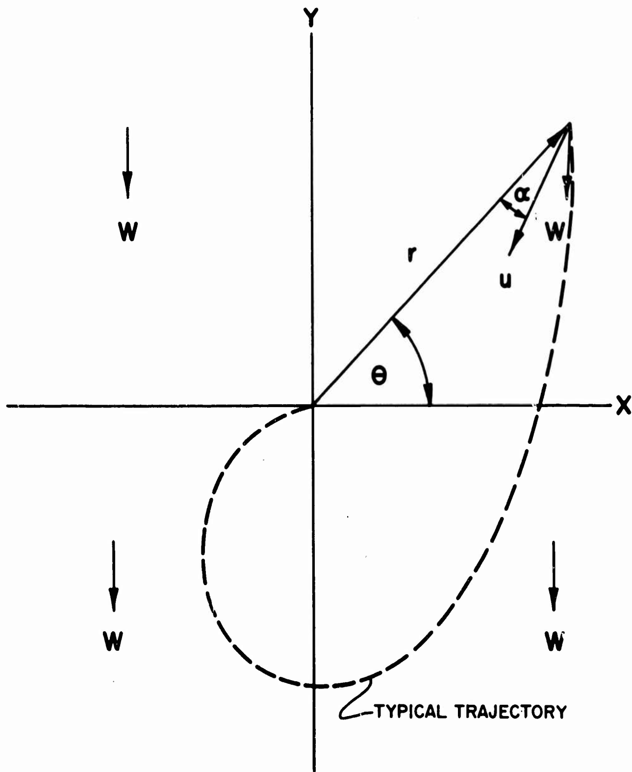
FIG. 1 Kinematics of Azimuth Homing
