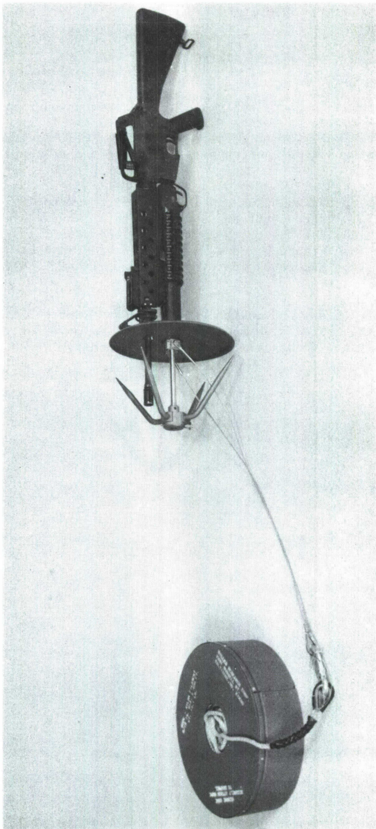
Figure 1. Grapnel System
