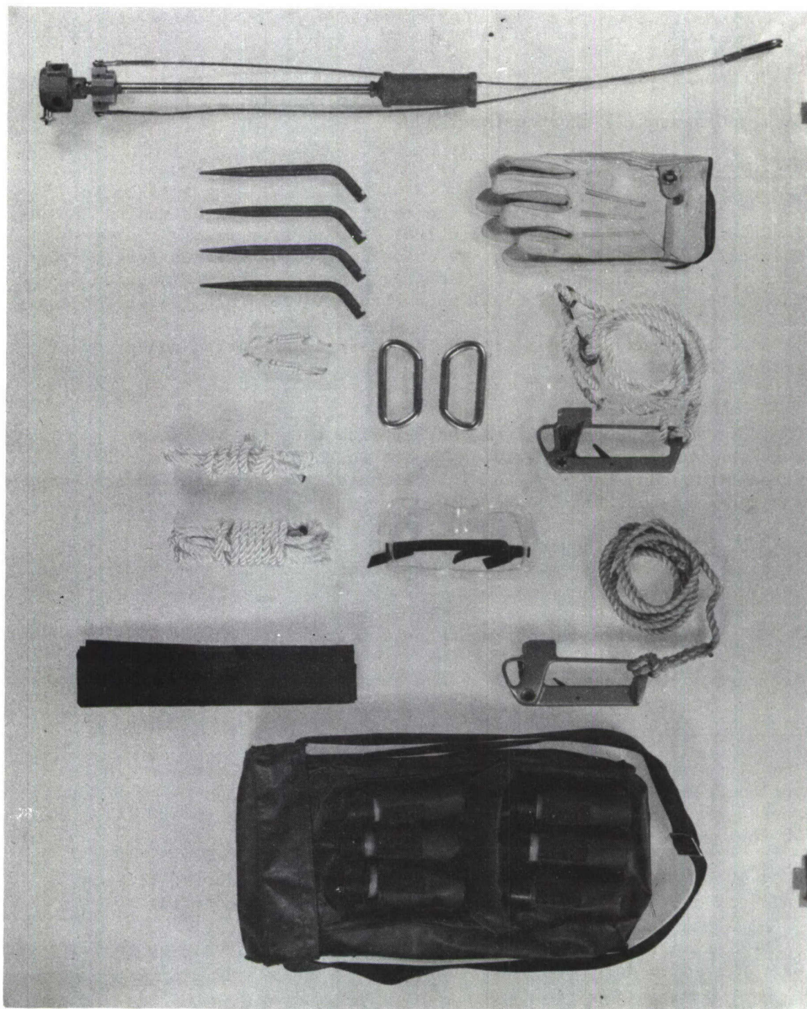
Figure 4. Grapnel Bandoleer
