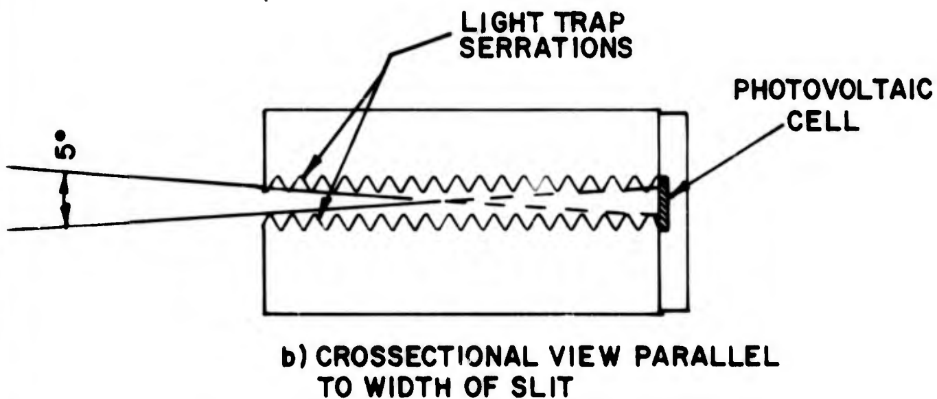
Figure 4. A Schematic of the Solar Cell and Slit Geometry
