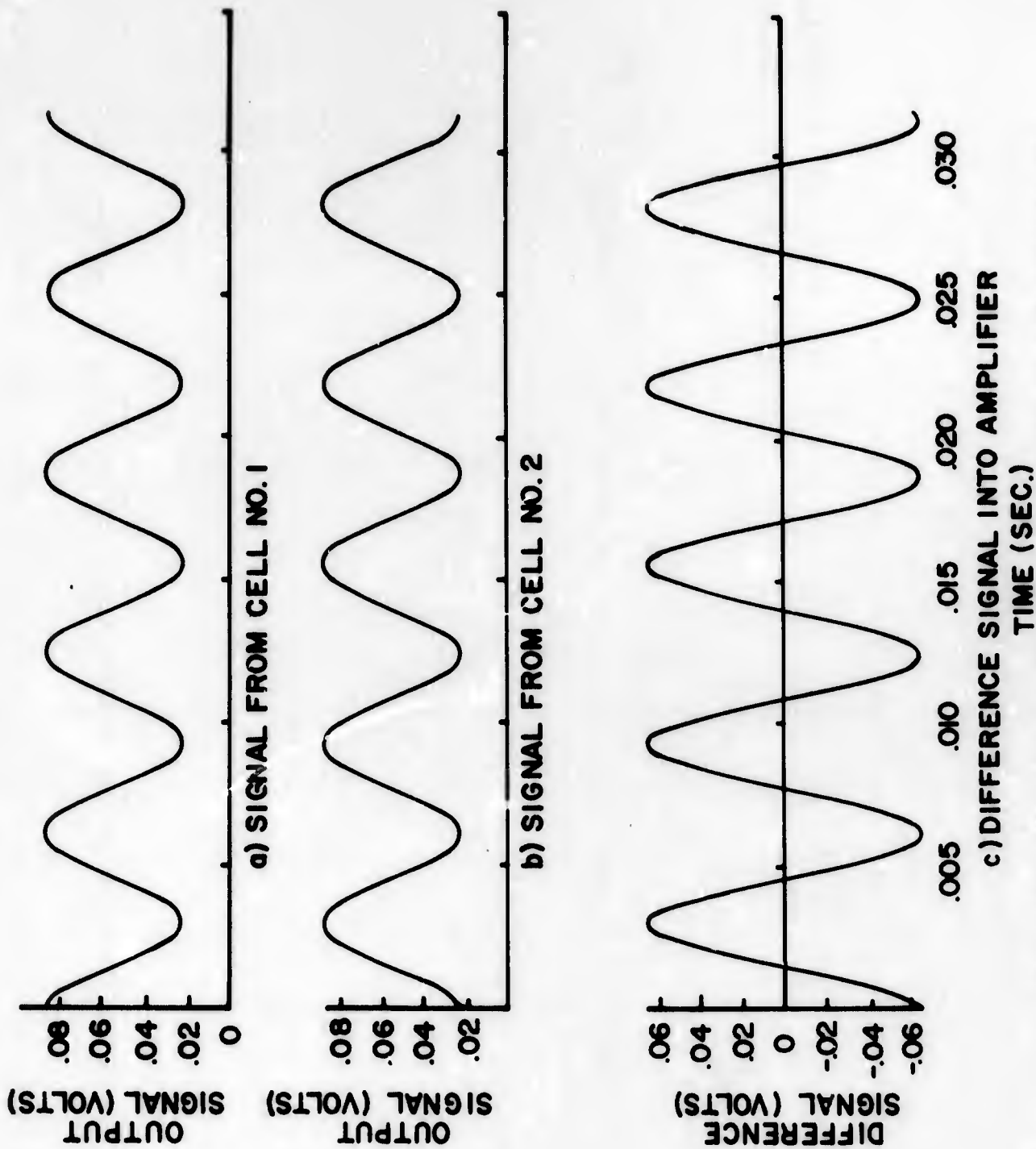
Figure 11. Idealized Waveforms from Each Cell Due to Background and the Combined Signal into the Amplifier
