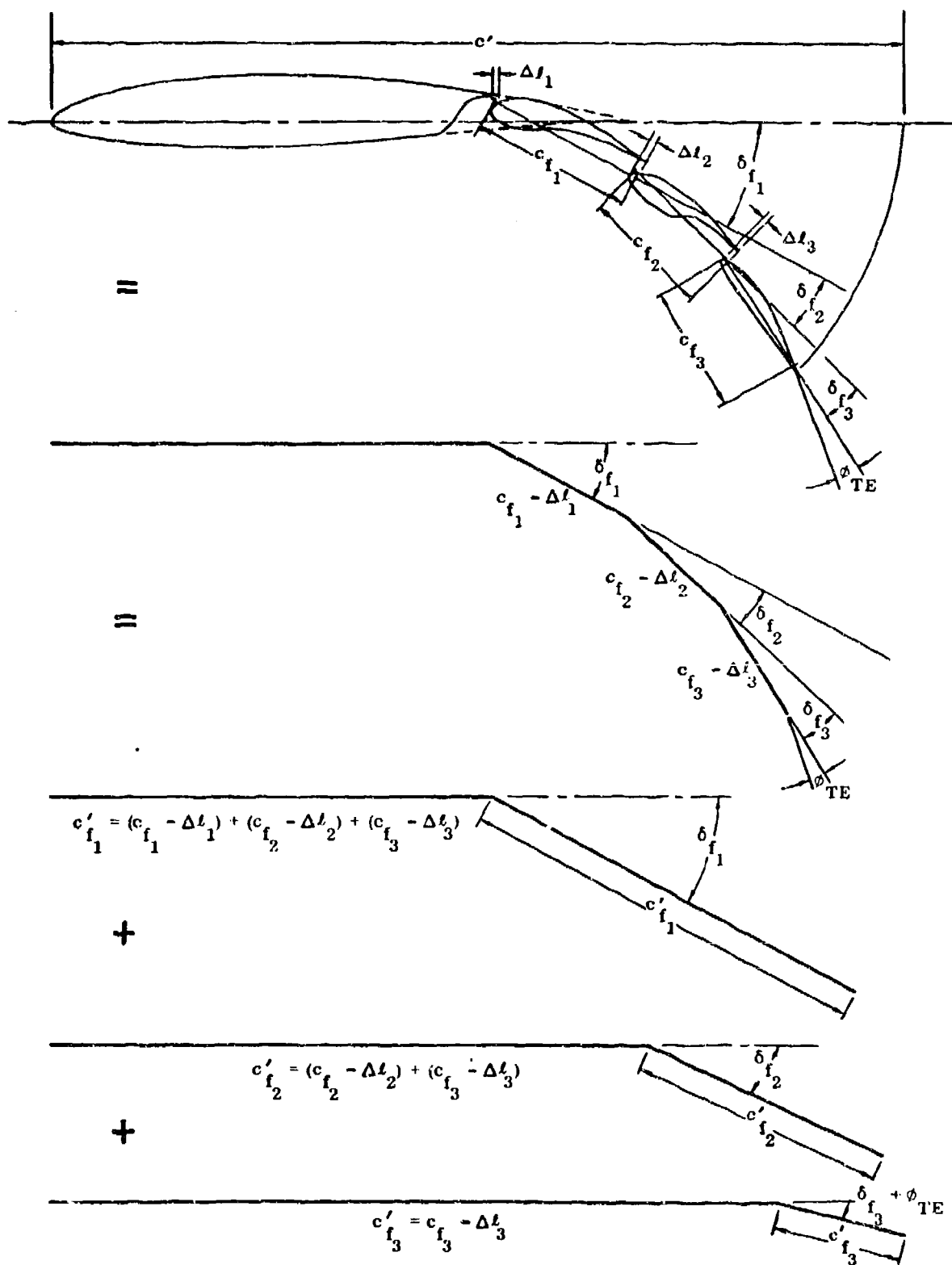
Figure 78 Principle of Superposition Theory and Extended Slotted-Flap Geometry
