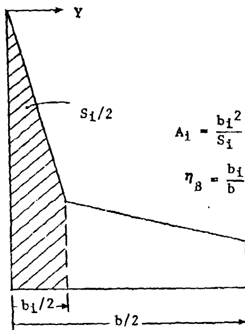
Figure 45 Definition of Cranked-Wing Planform for Calculation of Angle of Attack in Nonlinear Lift Range
