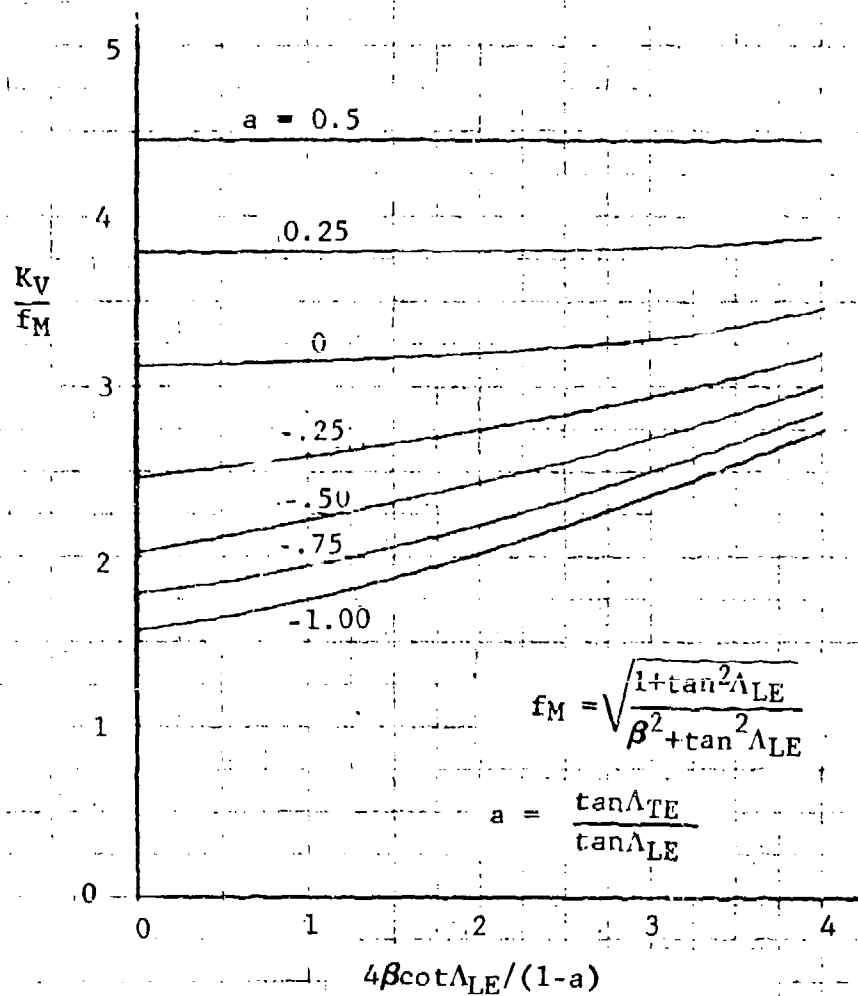
Figure 36 Variation of Vortex-Lift Constant with Planform Parameters
