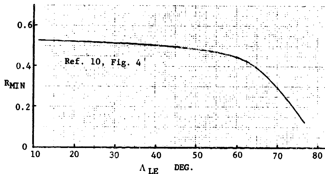
Figure 16 Leading-Edge Suction for Sharp Airfoils
