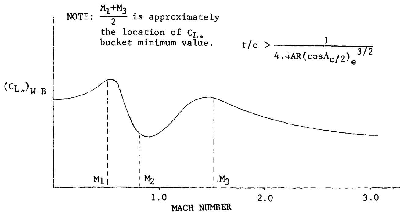
Figure 33 Typical Lift-Curve Slopes
