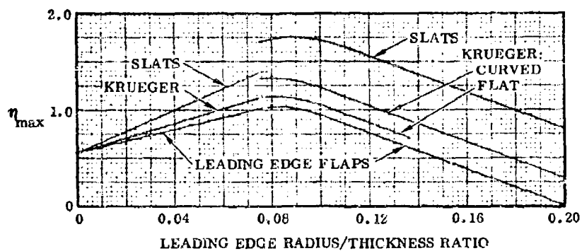
Figure 82 Maximum Lift Efficiency for Leading-Edge Devices
