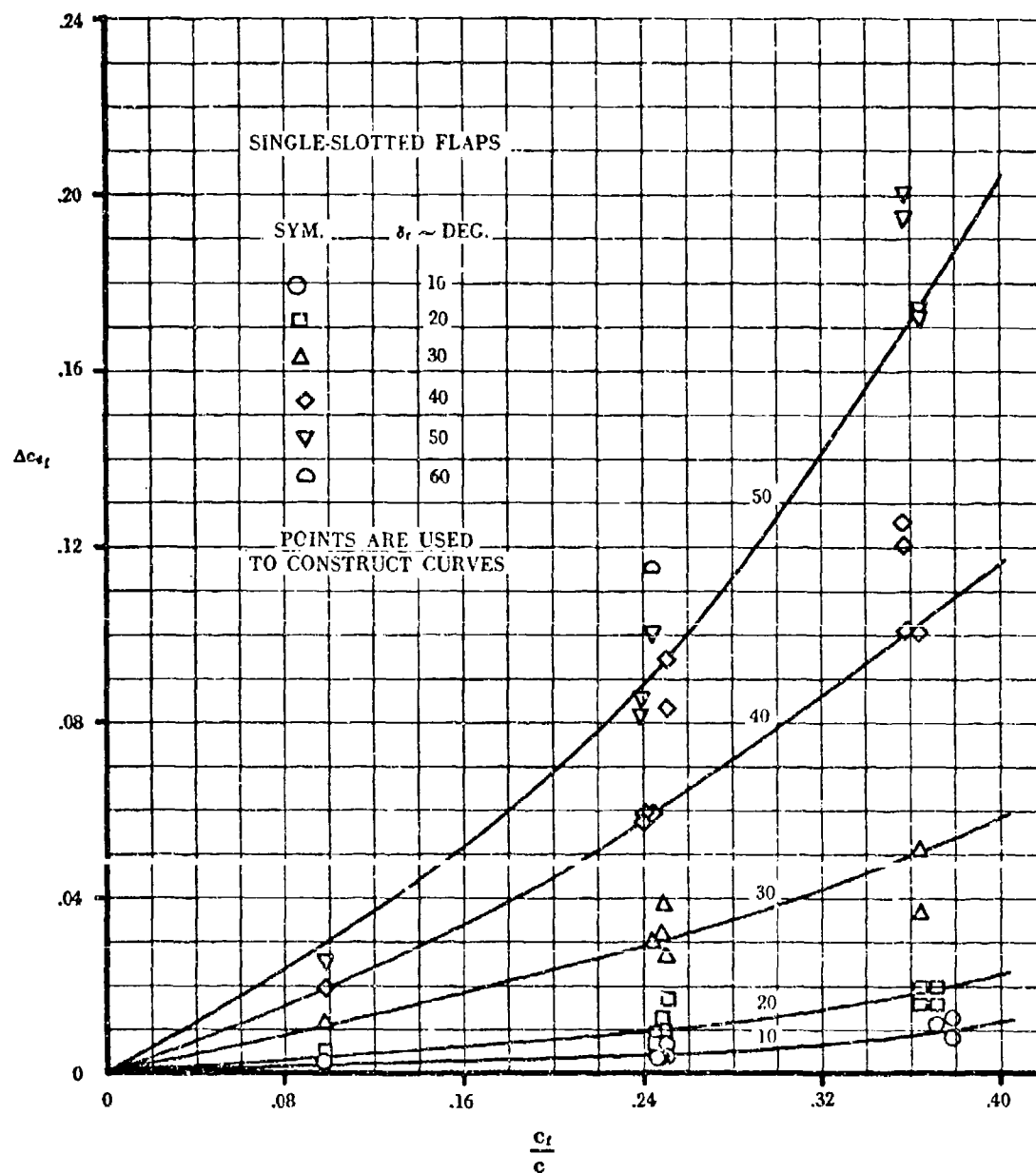
Figure 87 Two-Dimensional Drag Increment Due to Single-Slotted Flaps
