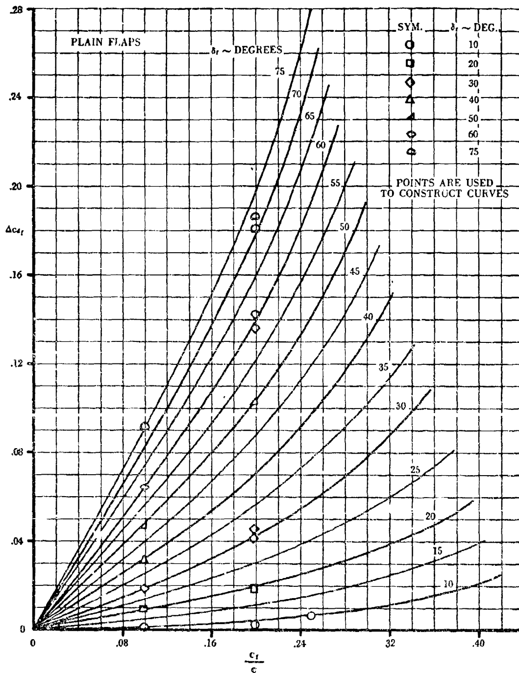
Figure 86 Two-Dimensional Drag Increment Due to Plain Flaps
