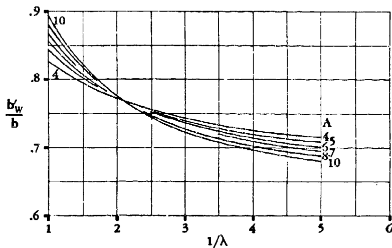
Figure 95 Effective Wing Span in the Presence of the Ground
