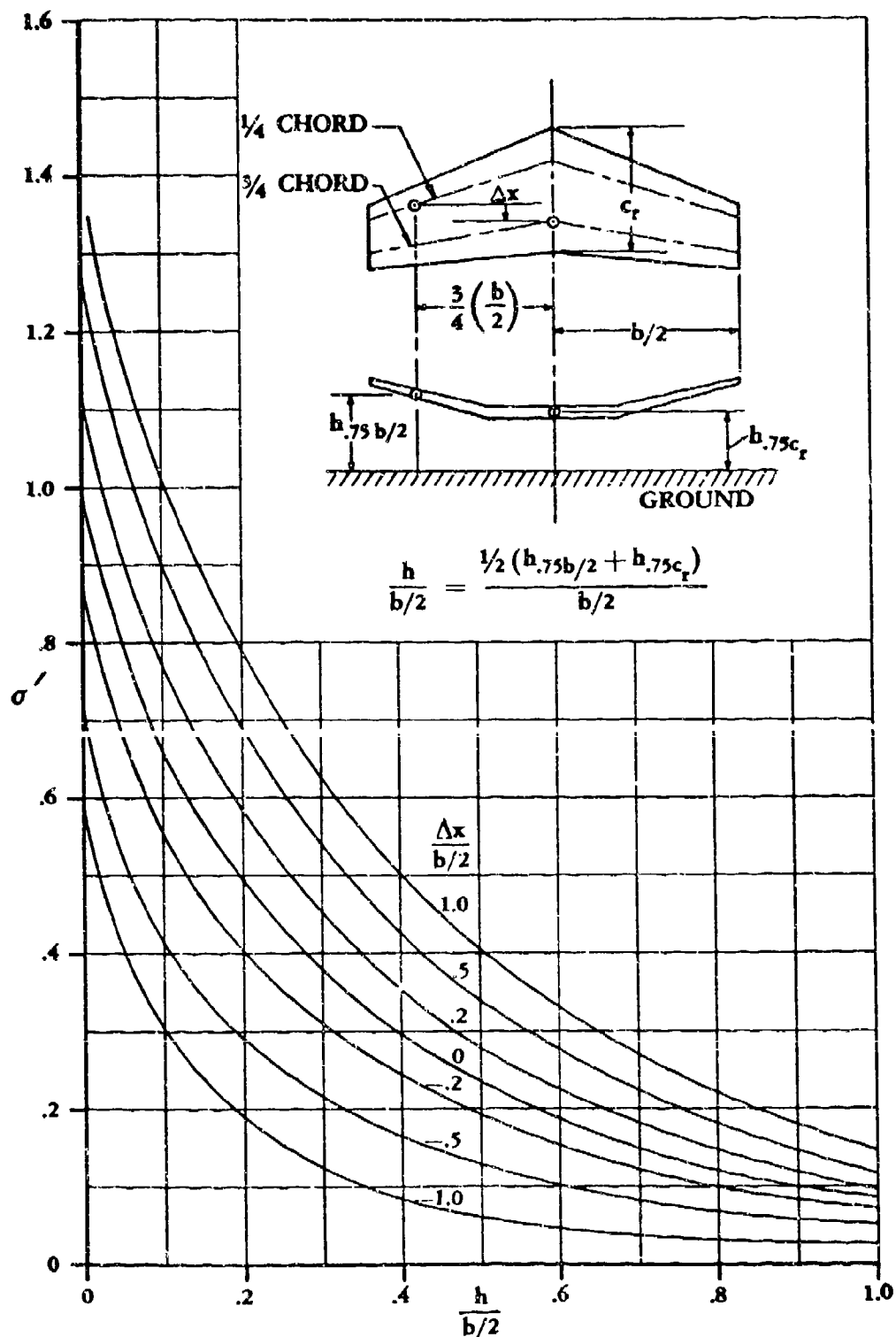
Figure 92 Parameter Accounting for Ground Effect on Lift Due to Trailing Vortices
