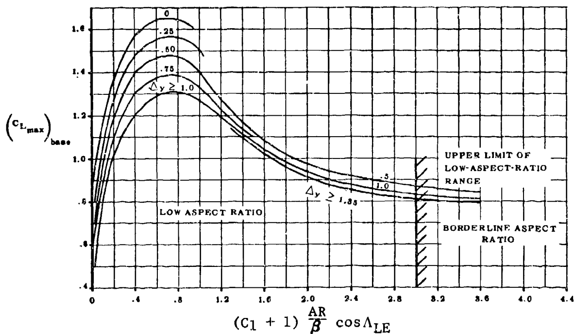
Figure 52 Subsonic Maximum Lift of Low-Aspect-Ratio Wings ( X_T < 35\% )
