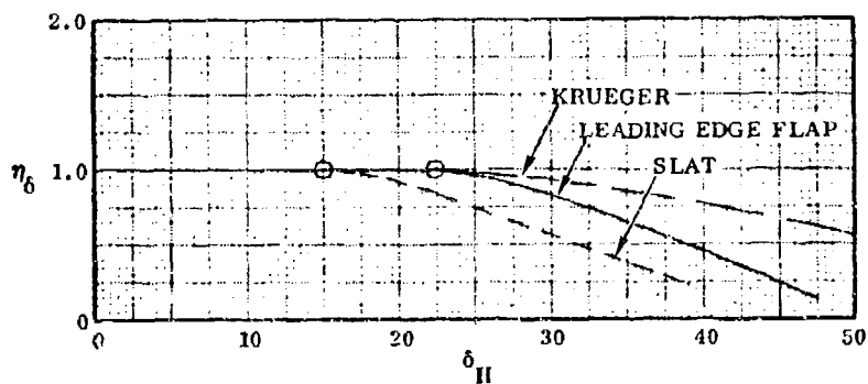
Figure 83 Leading Edge Device Deflection Angle Correction Factor
