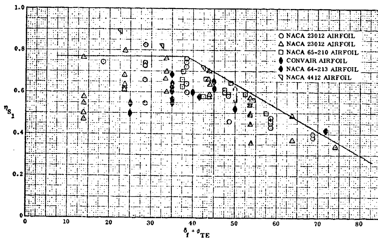
Figure 75 Turning Efficiency of Single-Slotted Flaps
