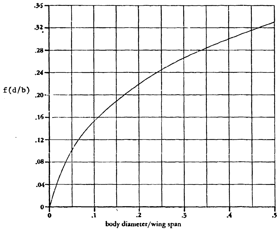
Figure 63 Parameter Used in Accounting for Wing-Lift Carryover on the Body
