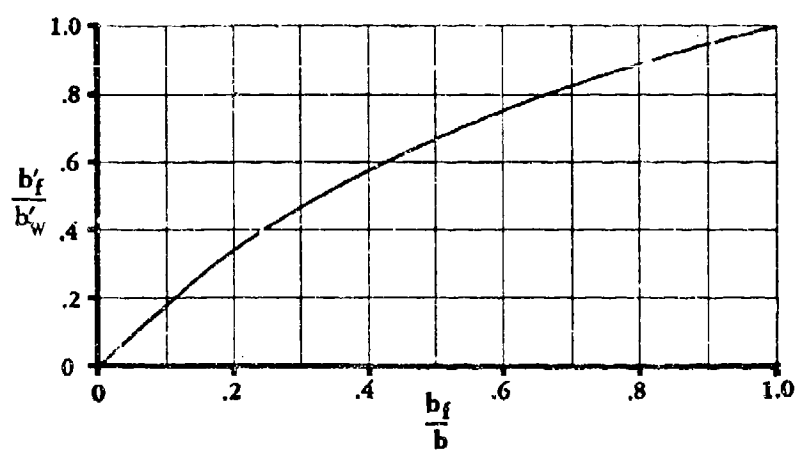
Figure 96 Effective Flap Span in the Presence of the Ground
