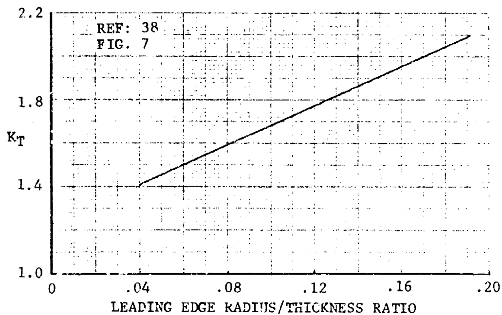
Figure 79 Maximum Lift Correlation Factor for Trailing-Edge Flaps
