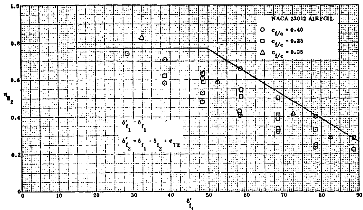
Figure 76 Turning Efficiency of Double-Slotted Flaps
