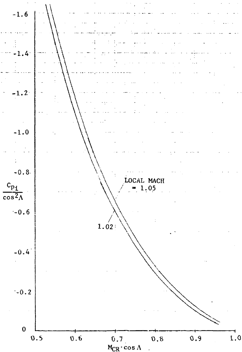
Figure 29 Mach Critical Prediction Chart
