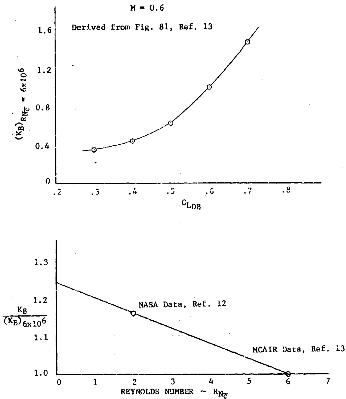
Figure 27 Separation Drag Factor
