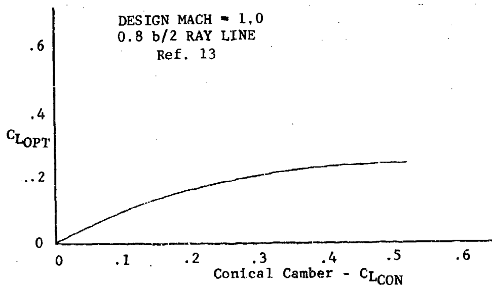
Figure 19 Lift Coefficient for Minimum Profile Drag - NACA Camber
