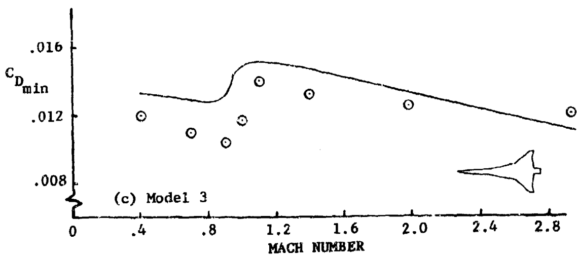
Figure 102 Minimum Drag Coefficient as a Function of Mach Number
