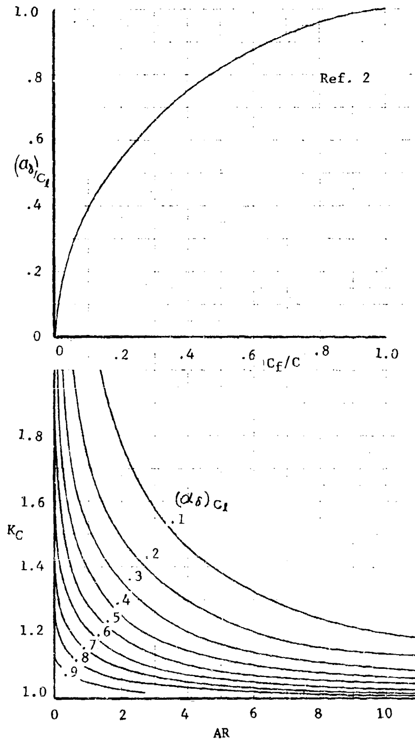
Figure 66 Flap Chord Factor
