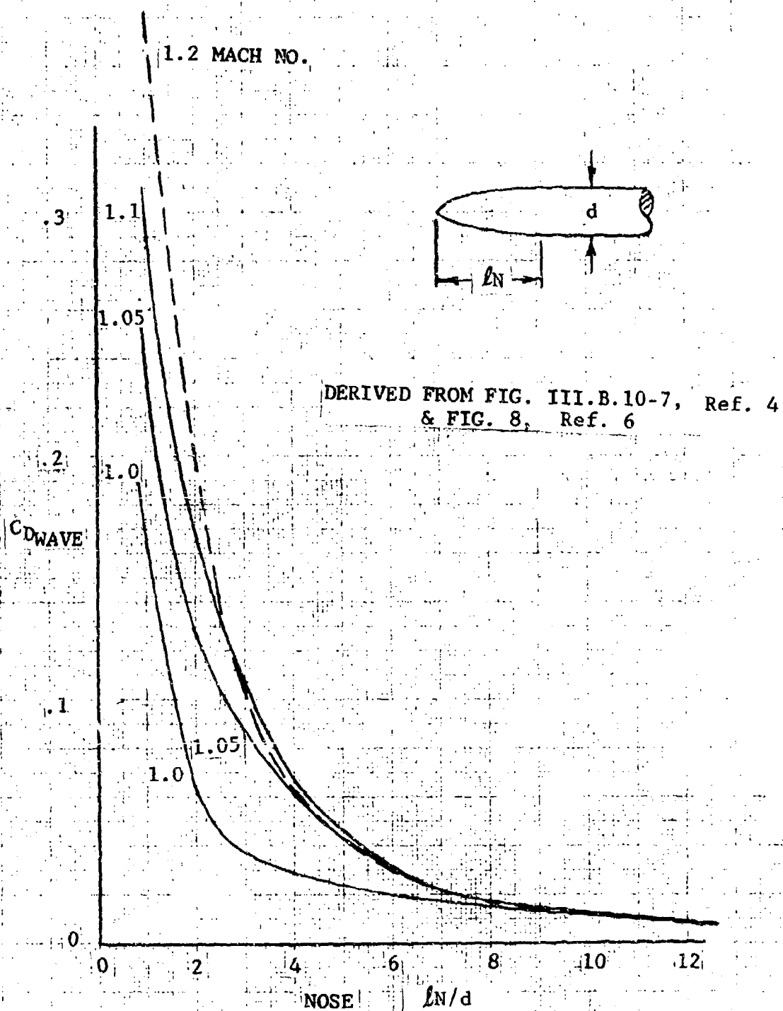
Figure 11 Transonic Wave Drag of Parabolic Noses
