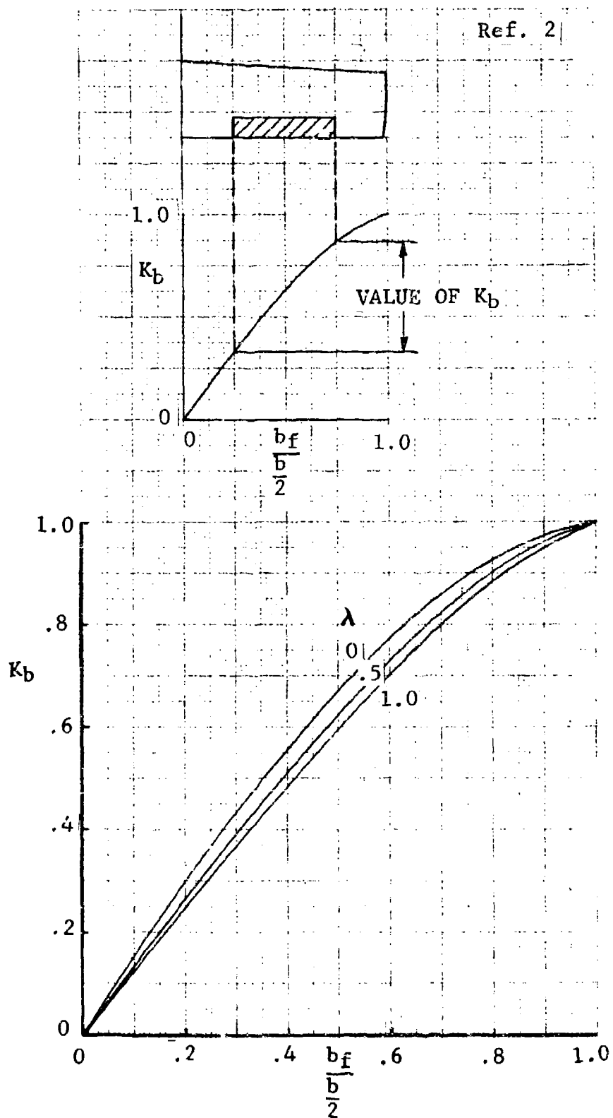
Figure 67 Flap Span Lift Factor
