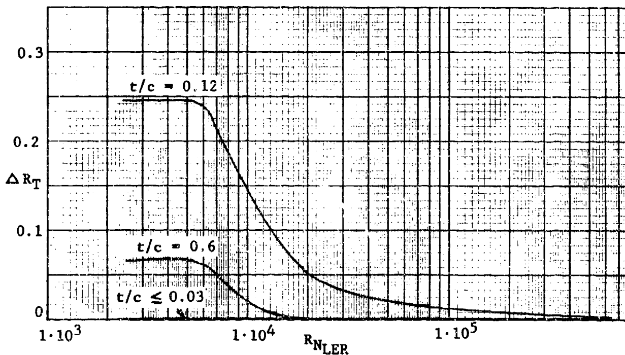
Figure 17 Effect of Reynolds Number and Thickness on the Leading-Edge Suction Factor
