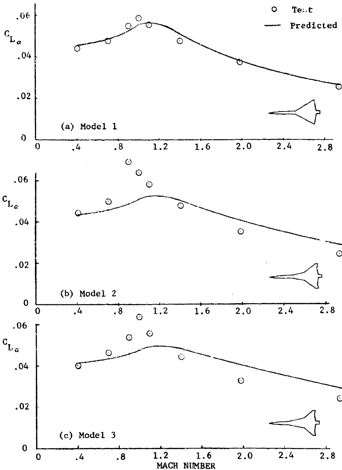
Figure 99 Lift-Curve Slope as a Function of Mach Number
