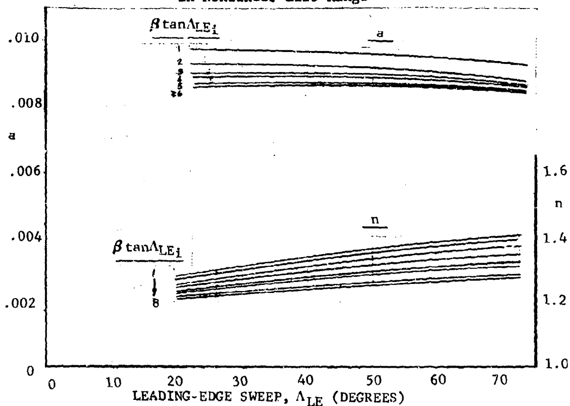
Figure 46 Parameters Used in Calculation of Angle of Attack in Nonlinear Lift Range
