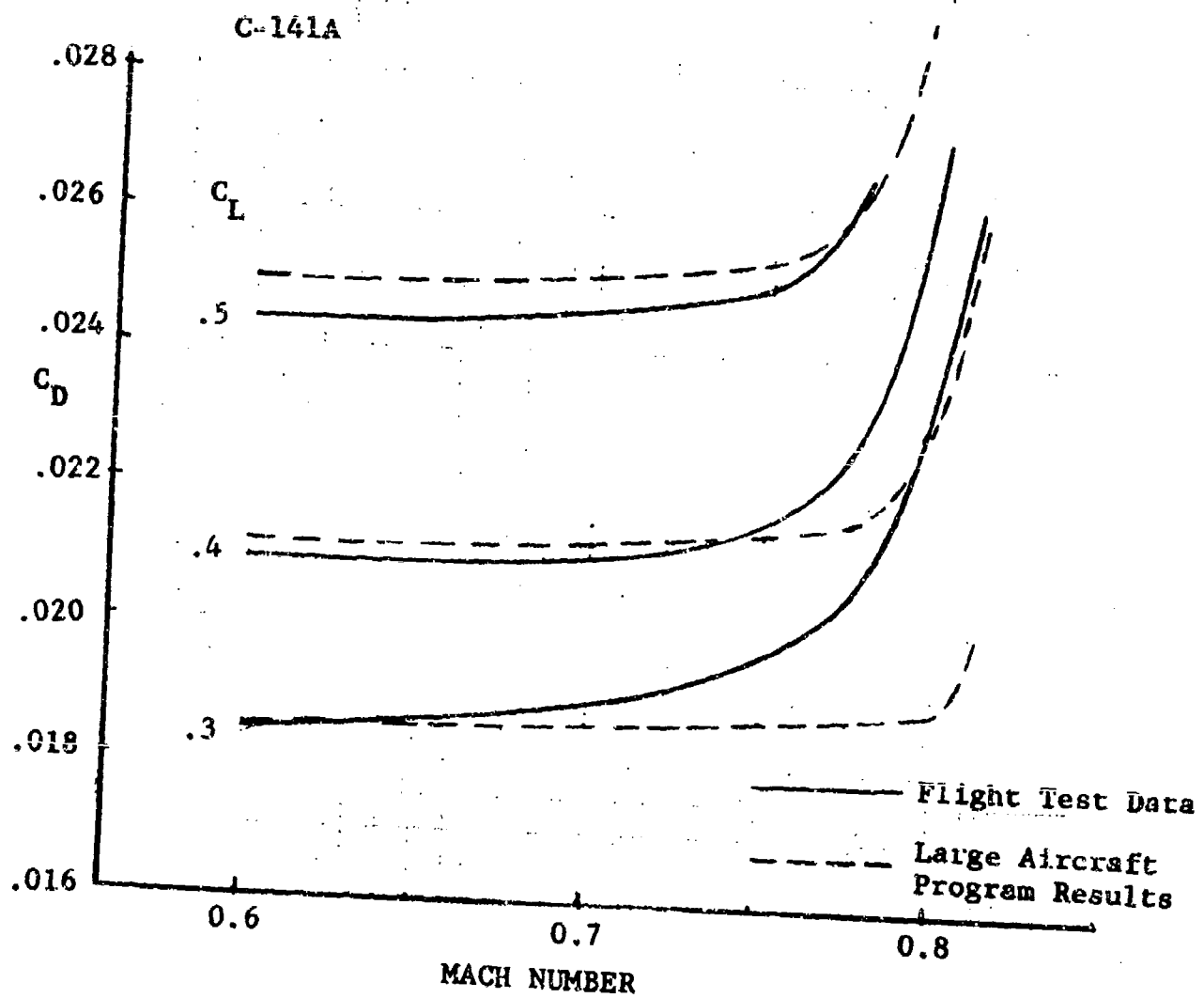
Figure 104 Drag at Constant Lift Coefficient Versus Mach Number
