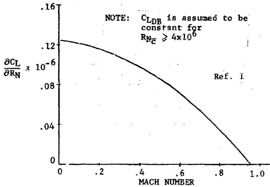
Figure 24 Reynolds Number Effect on C_{LDB}
