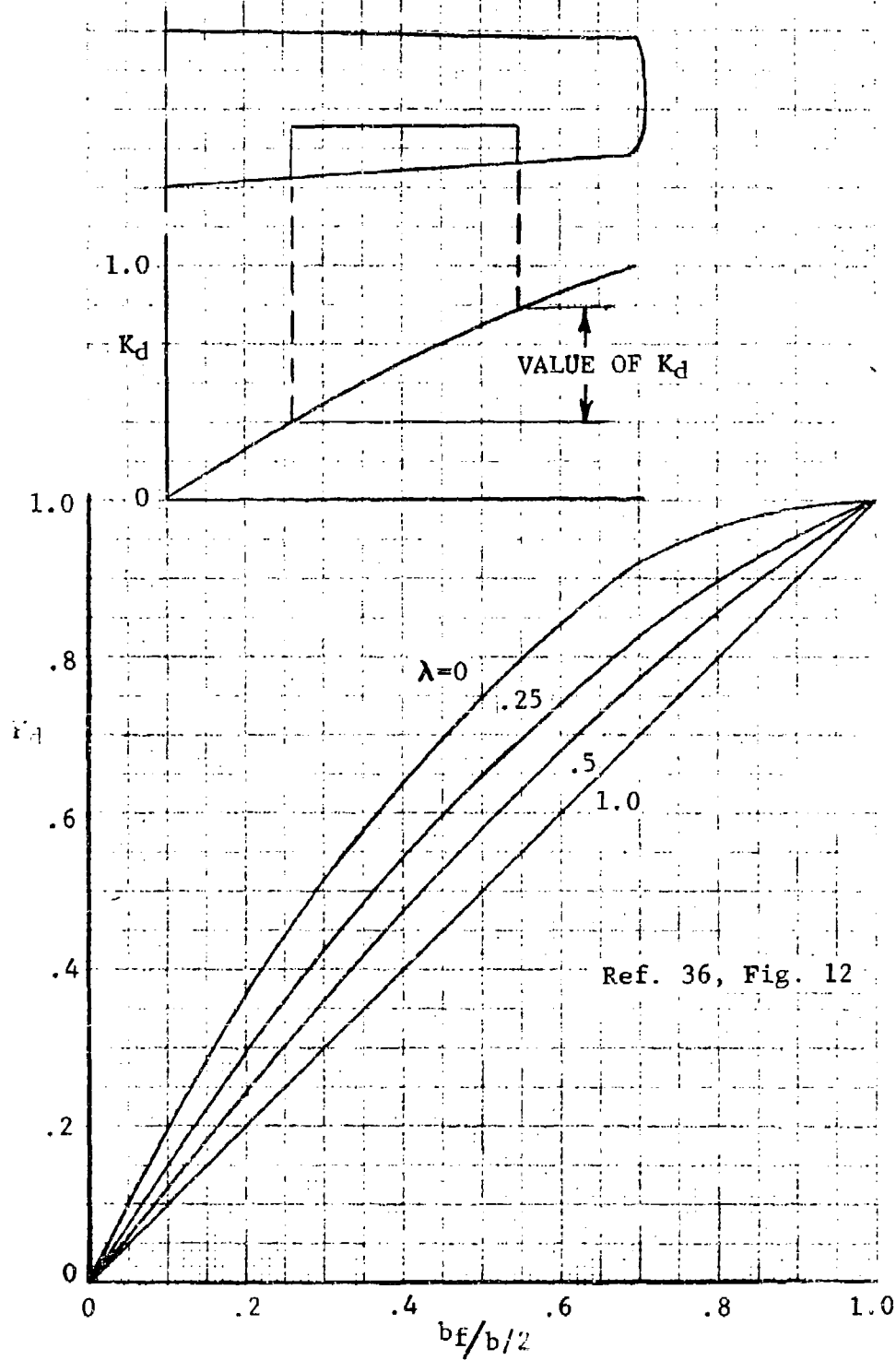
Figure 69 Flap Span Drag Factor
