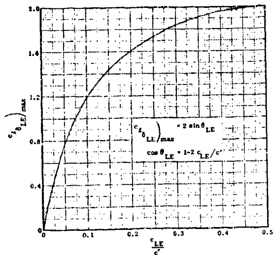
Figure 81 Leading Edge Flap Maximum Lift Effectiveness
