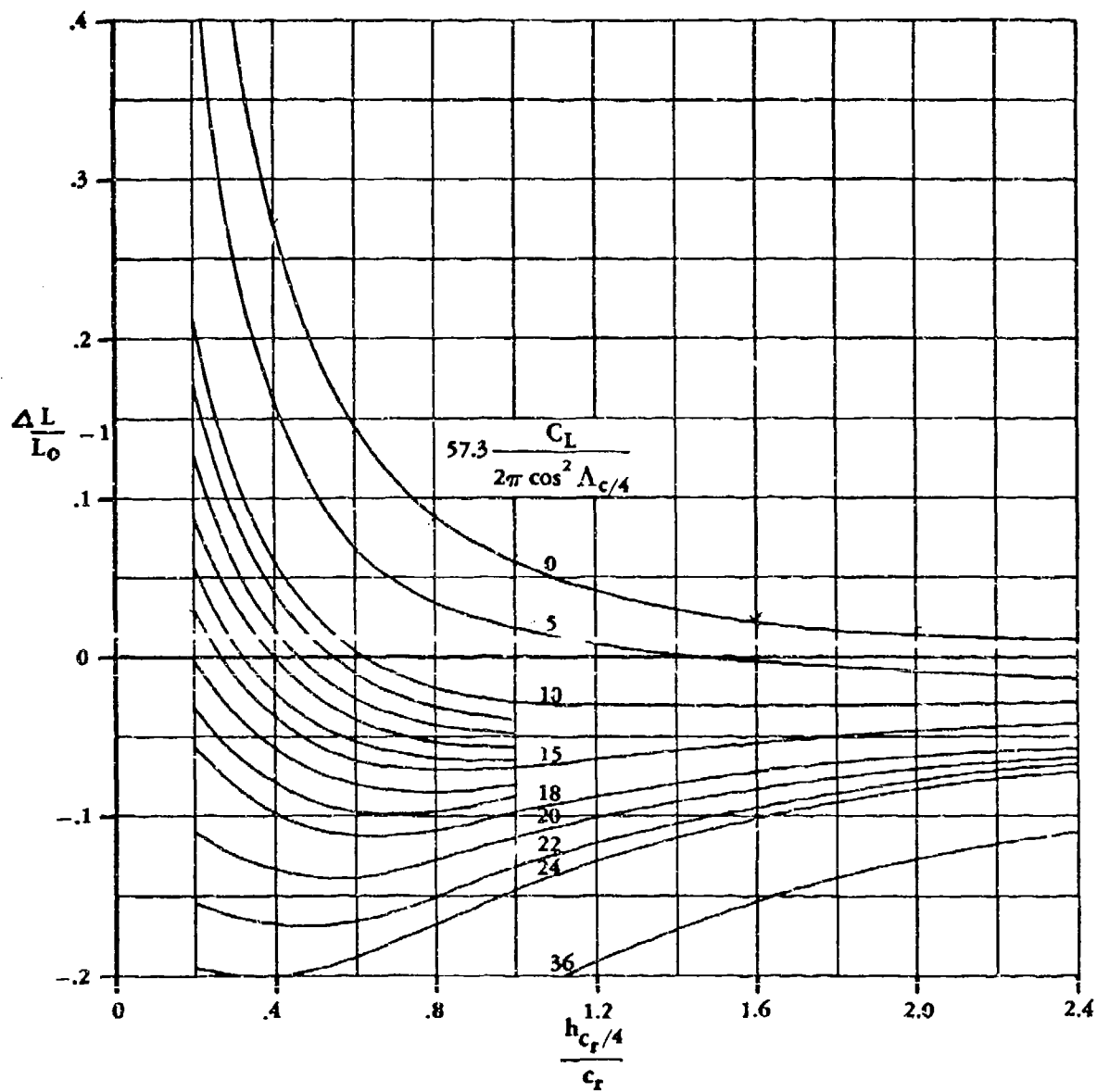
Figure 93 Parameter Accounting for Ground Effect on Lift Due to Bound Vortices
