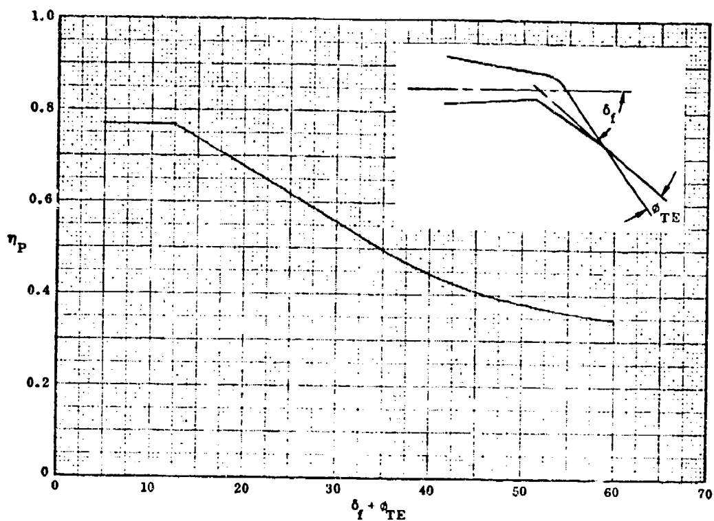
Figure 74 Turning Efficiency of Plain Trailing-Edge Flaps
