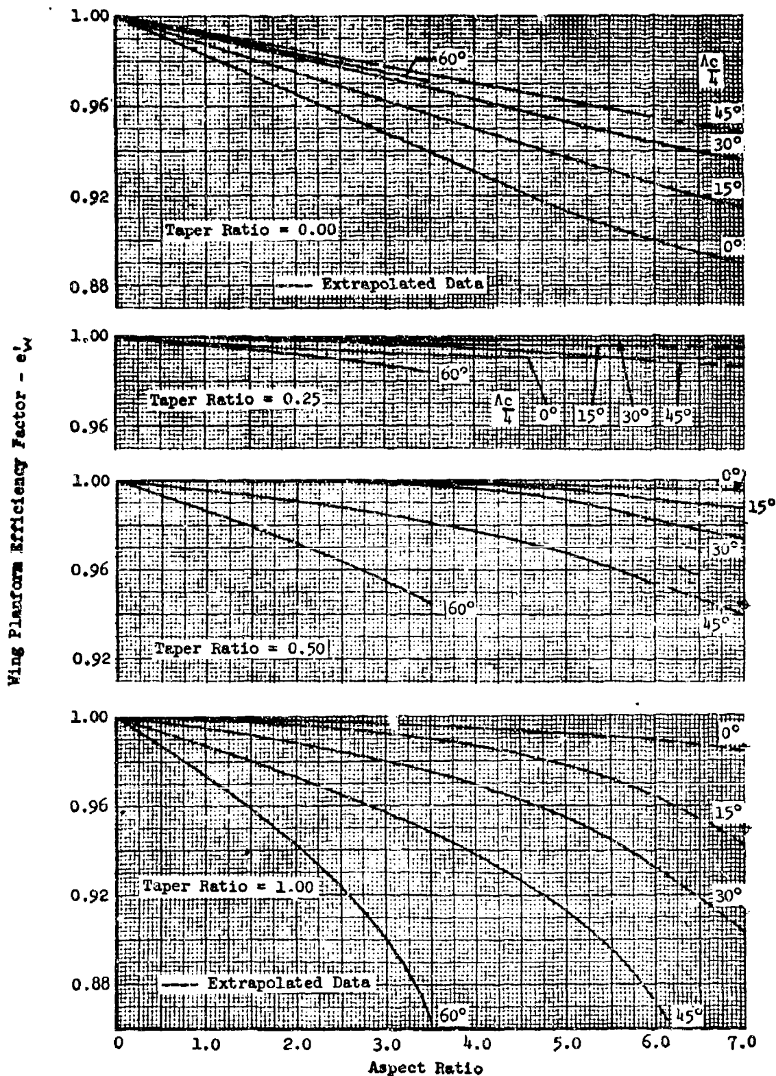
Figure 26 Weissenger Theoretical Wing Planform Efficiency Factor
