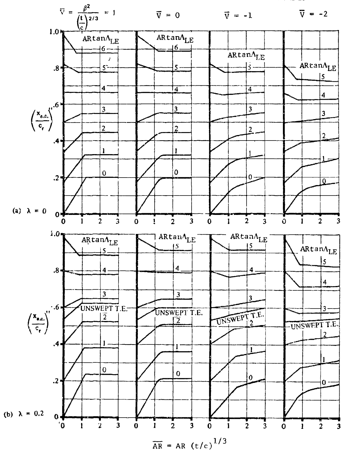
Figure 61 Transonic Wing Aerodynamic-Center Location
