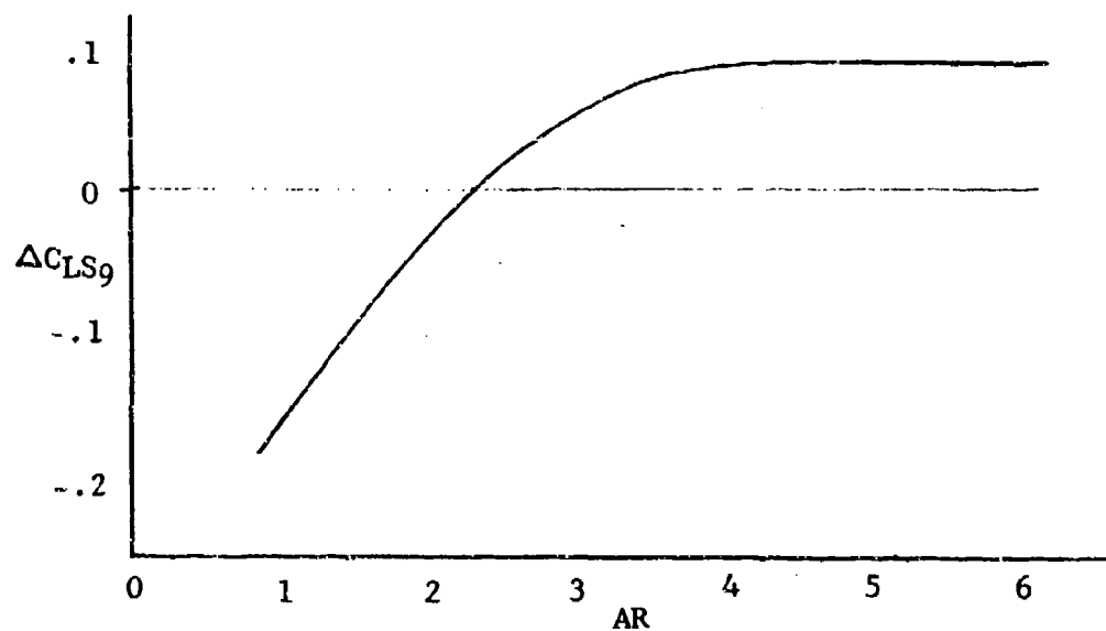
Figure 28 Supersonic Polar Break Lift Factors
