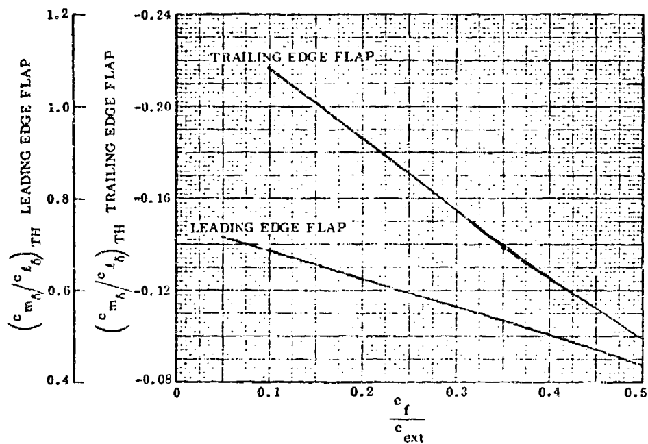
Figure 84 Flap Center of Pressure Location as given by Thin Airfoil Theory
