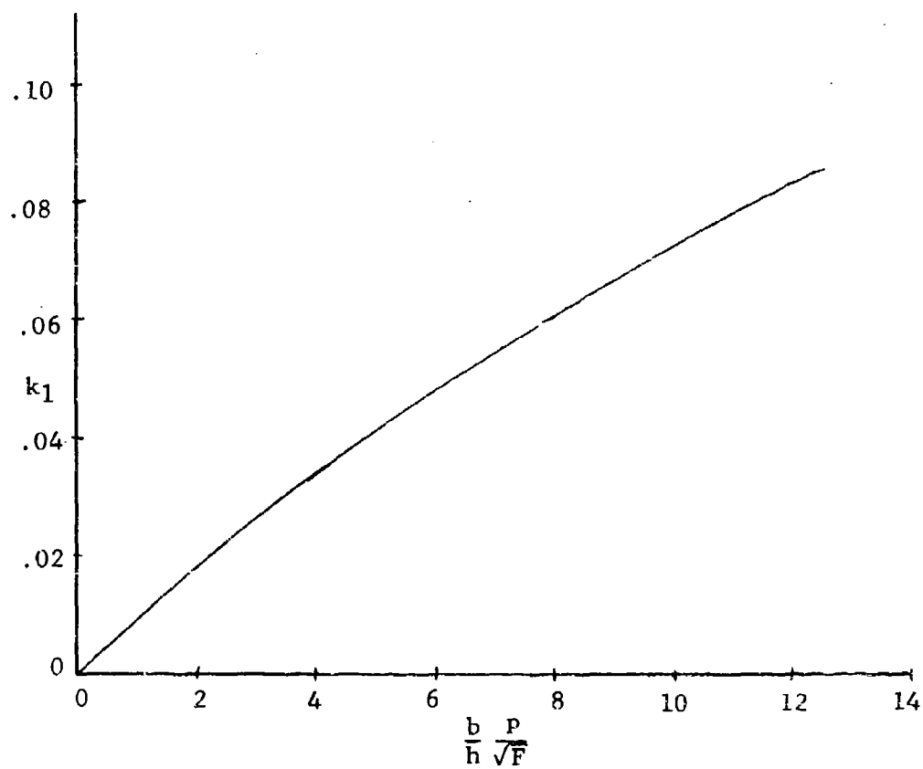
Figure 34 Factor Used in Determination of Body Lift-Curve Slope
