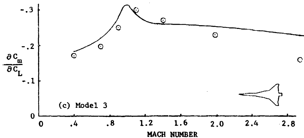
Figure 101 Pitching Moment-Curve Slope as a Function of Mach Number
