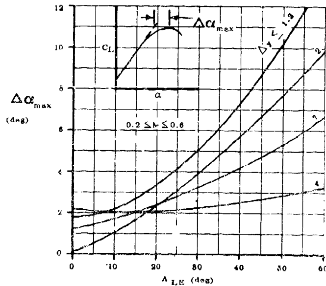
Figure 51 Angle-of-Attack Increment for Subsonic Maximum Lift of High-Aspect-Ratio Wings
