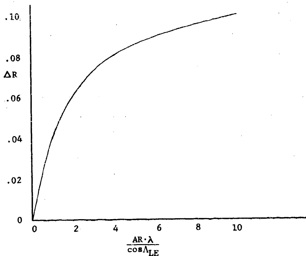
Figure 18 Effect of Wing Planform on Leading-Edge Suction
