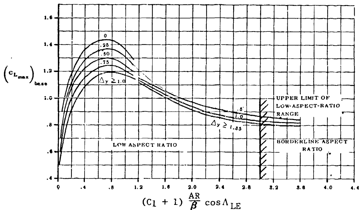
Figure 53 Subsonic Maximum Lift of Low-Aspect-Ratio Wings ( X_T \geq 35\% )
