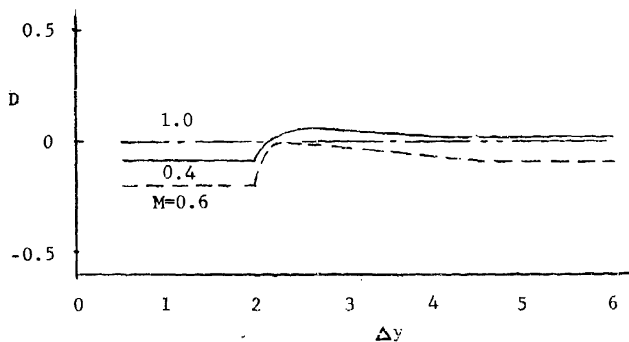
Figure 48 Factors for Determining Mach Number Correction for Maximum Lift
