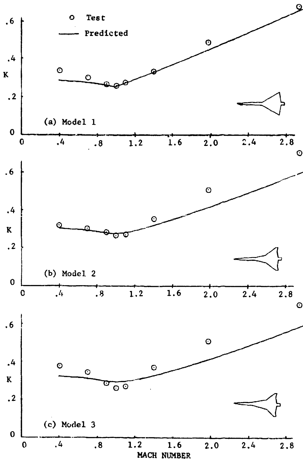
Figure 100 Drag Due-To-Lift Factor as a Function of Mach Number
