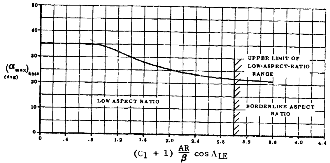
Figure 55 Angle of Attack for Subsonic Maximum Lift of Low-Aspect-Ratio Wing Maximum Lift
