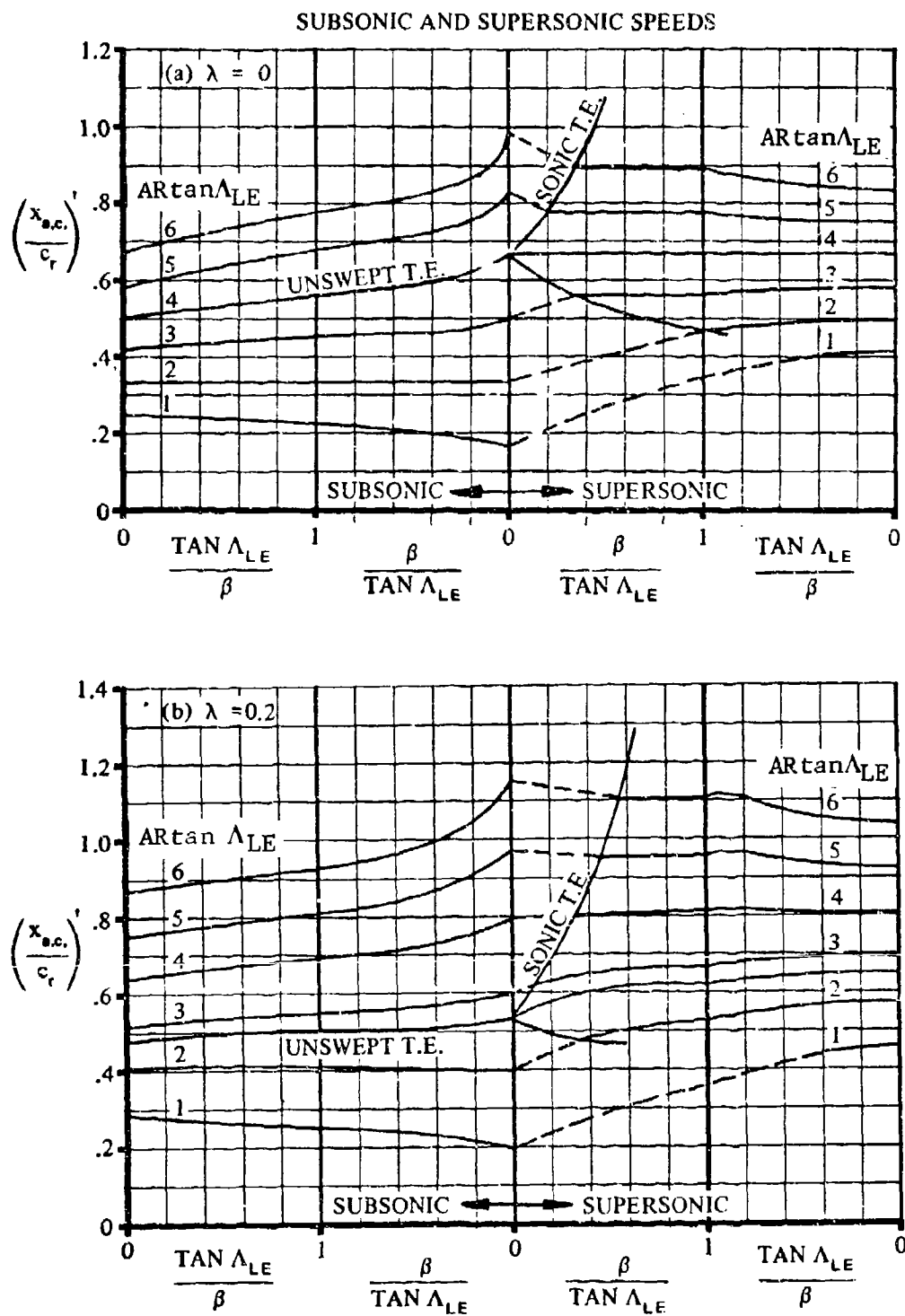
Figure 60 Wing Aerodynamic-Center Position
