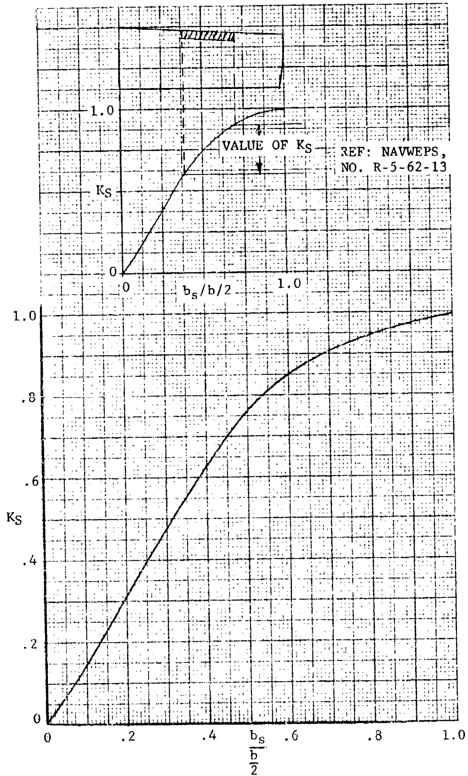
Figure 68 Slat Span Lift Factor
