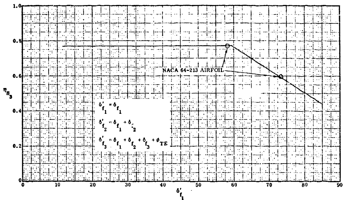
Figure 77 Turning Efficiency of Triple-Slotted Flaps
