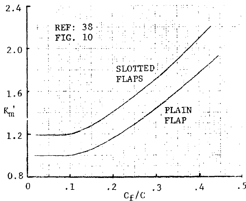
Figure 85 Moment Correlation Factor Versus Flap Chord
