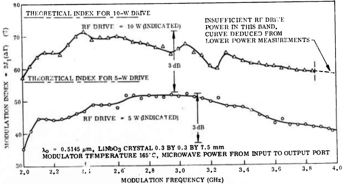
Fig. 3-2 Modulation Index Versus Frequency for 7.5-mm-Length LiNbO 3 Crystal With rf Power in Forward Direction. (Results were obtained last year and are included here for purpose of comparison)
