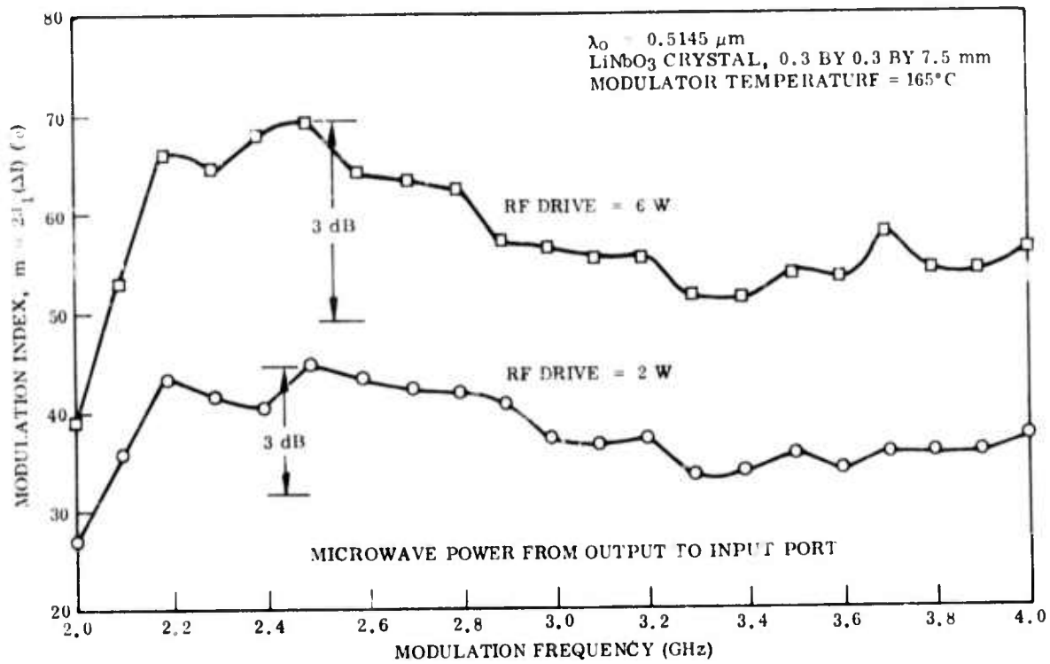
Fig. 3-1 Modulation Index Versus Frequency for 7.5-mm-Length LiNbO 3 Crystal With rf Power in Reverse Direction
