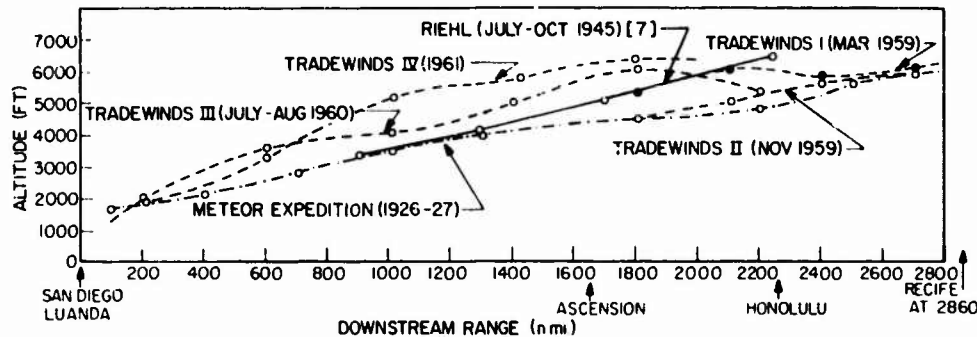
Fig. 8—Comparison of trade wind inversion heights
