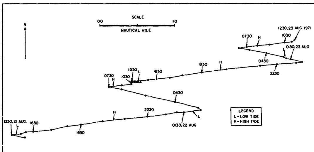
Figure 21. Progressive vector diagram of current from meter #407, 21 - 23 August 1971.
