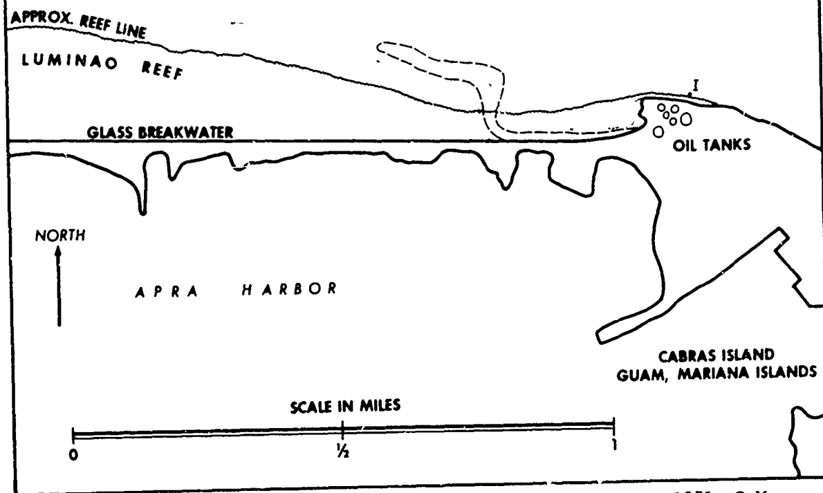
Figure 67. Dye movement at Cabras Island on 26 February 1971, P.M.
