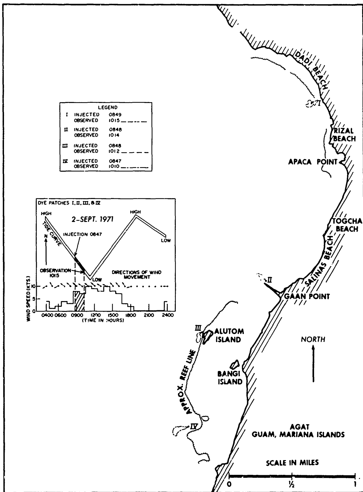
Figure 44. Dye movement at Agat Bay on 2 September 1971.
