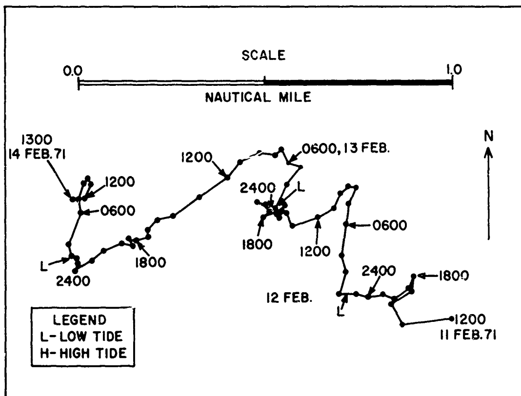
Figure 35. Progressive vector diagram of current from meter #175, 1200, 11 February to 1300, 14 February 1971.
