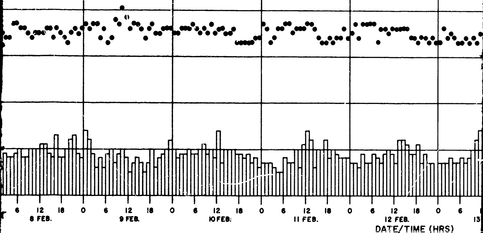
Figure 2. Speed and direction of winds observed at the Naval Air Station during the two periods and dye and drogue observation dates for the two flights.
