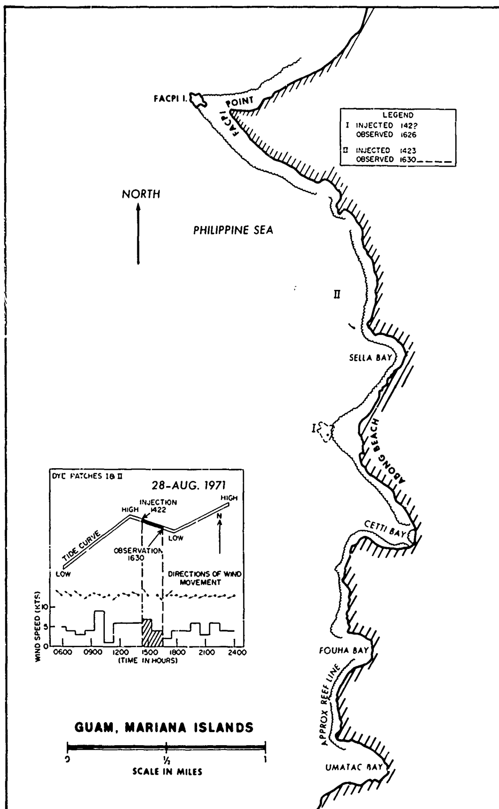
Figure 23. Dye movement at Sella Bay on 28 August 1971.
