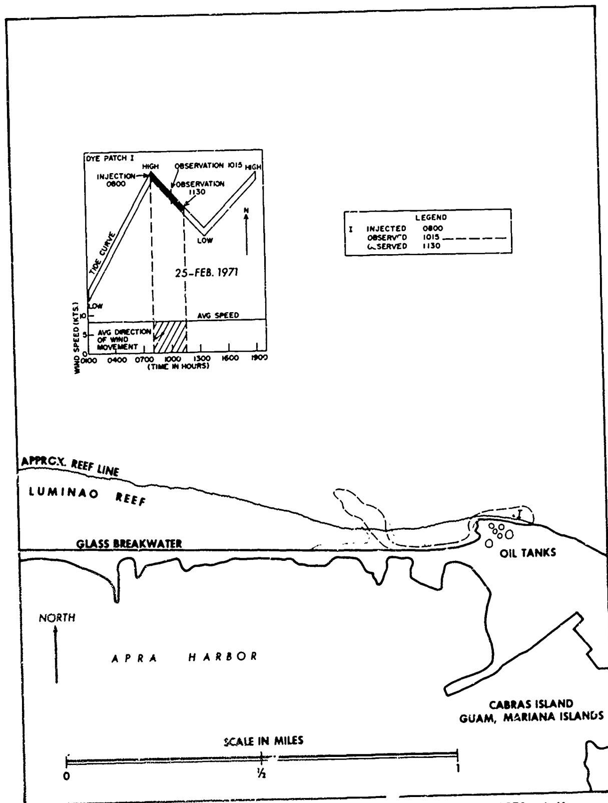
Figure 64. Dye movement at Cabras Island on 25 February 1971, A.M.
