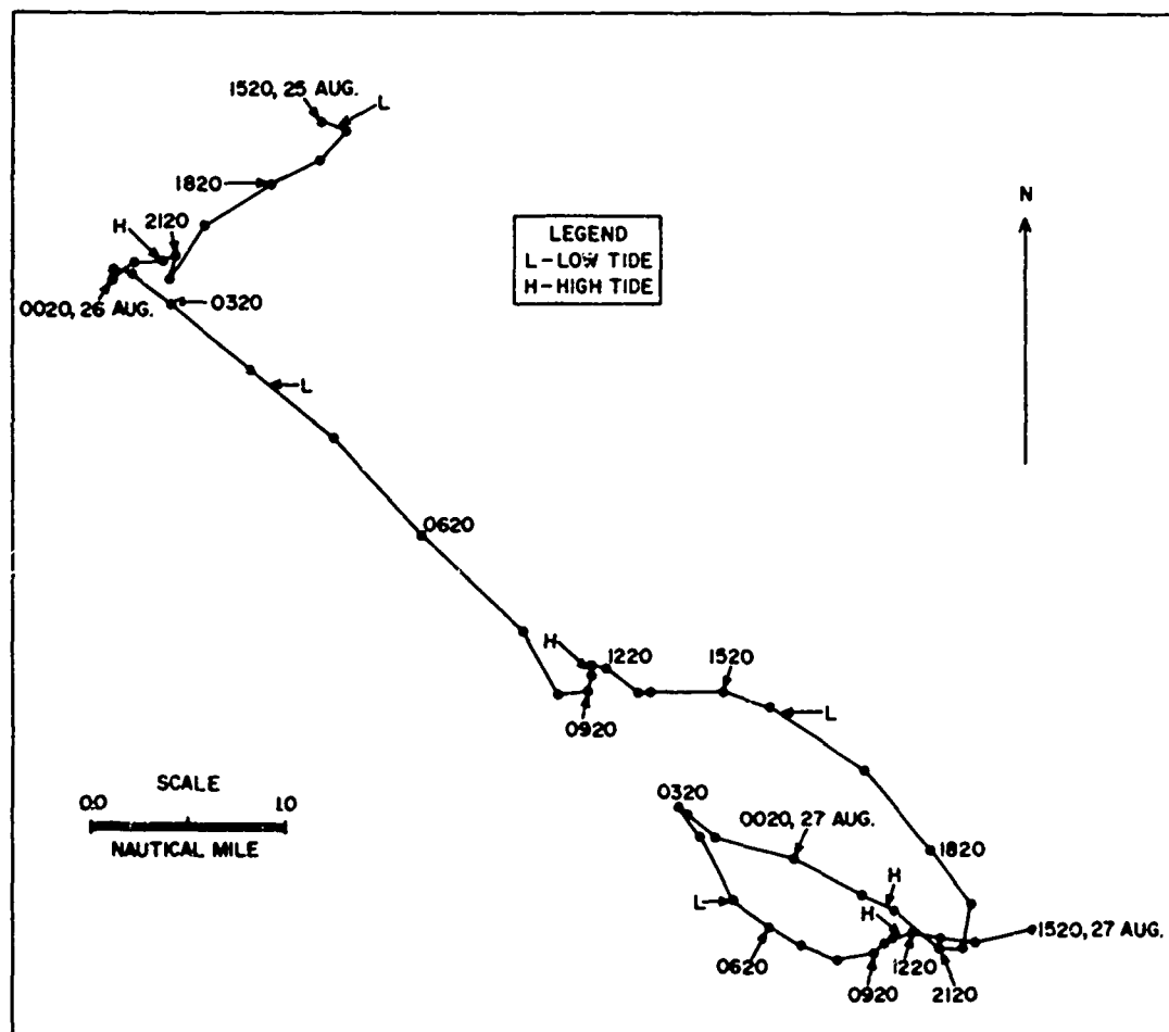
Figure 110. Progressive vector diagram of current from meter #404, 1520, 25 August to 1520, 27 August 1971.
