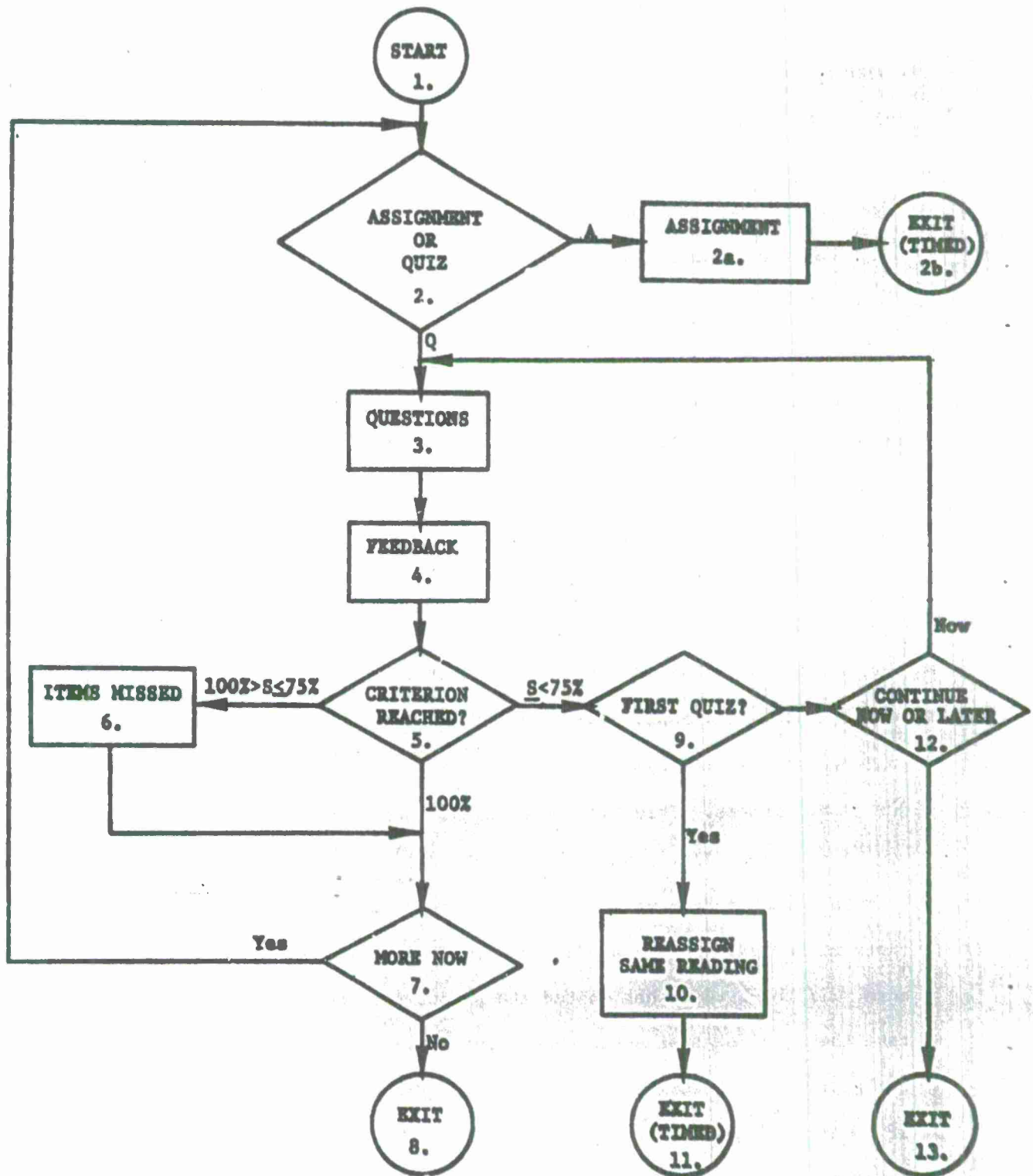
Figure III.1. A flow diagram and description of the computer based instructional process used in CAISMS.
