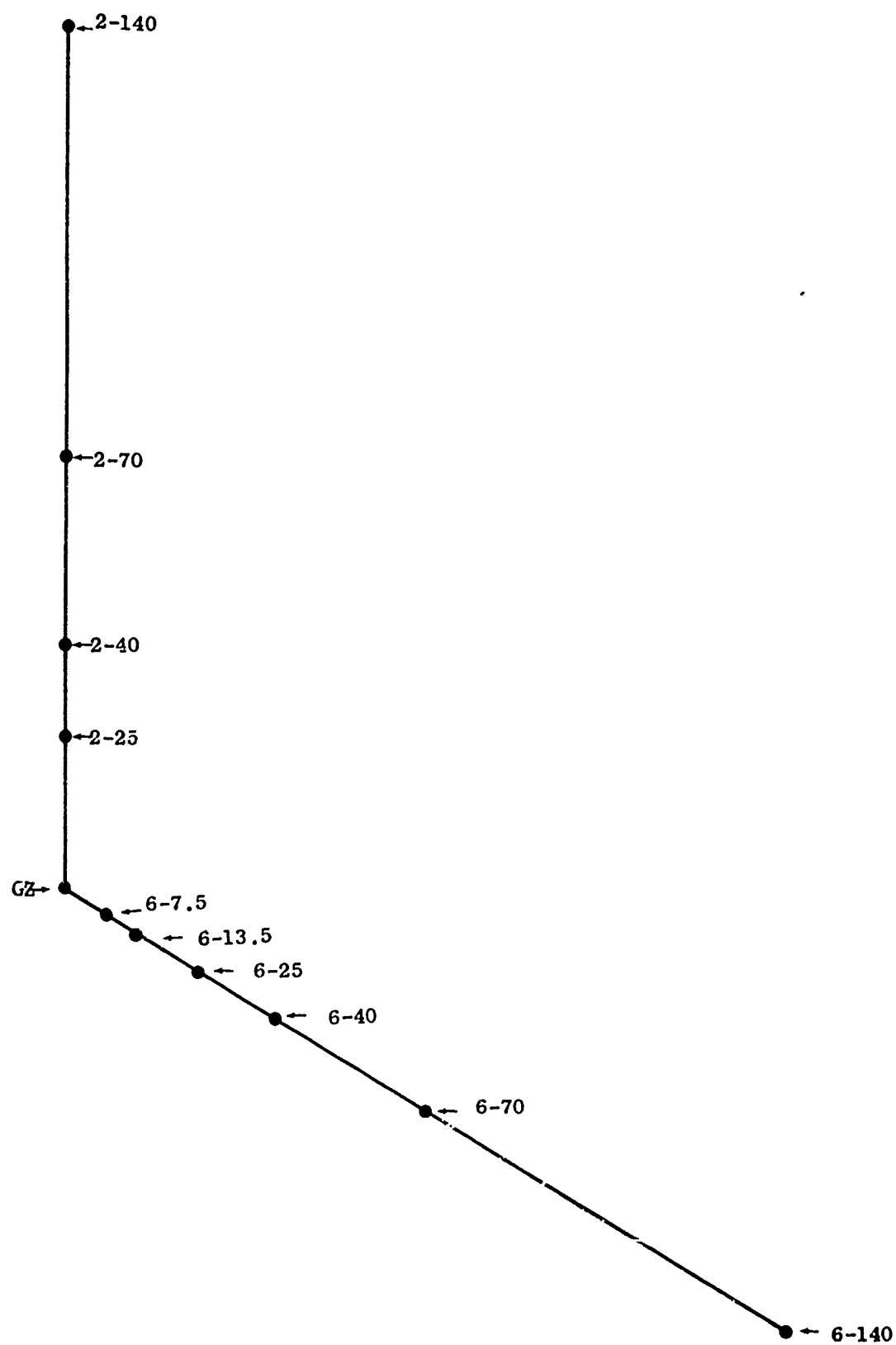
Fig. 2. Instrumentation Layout
