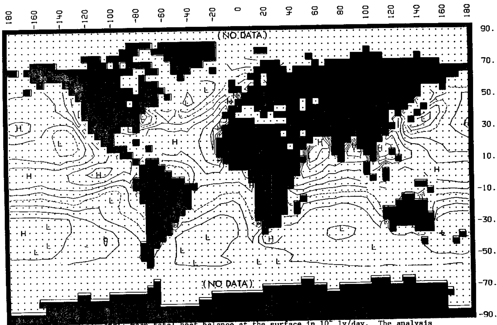
Fig. 3.11—April mean total heat balance at the surface in 10^{11} ly/day. The analysis interval is 50 ly/day and the 0 isoline is dashed. A positive value denotes a radiative heat surplus over the losses due to sensible heat flux and evaporation. Data are from Budyko (1963).
