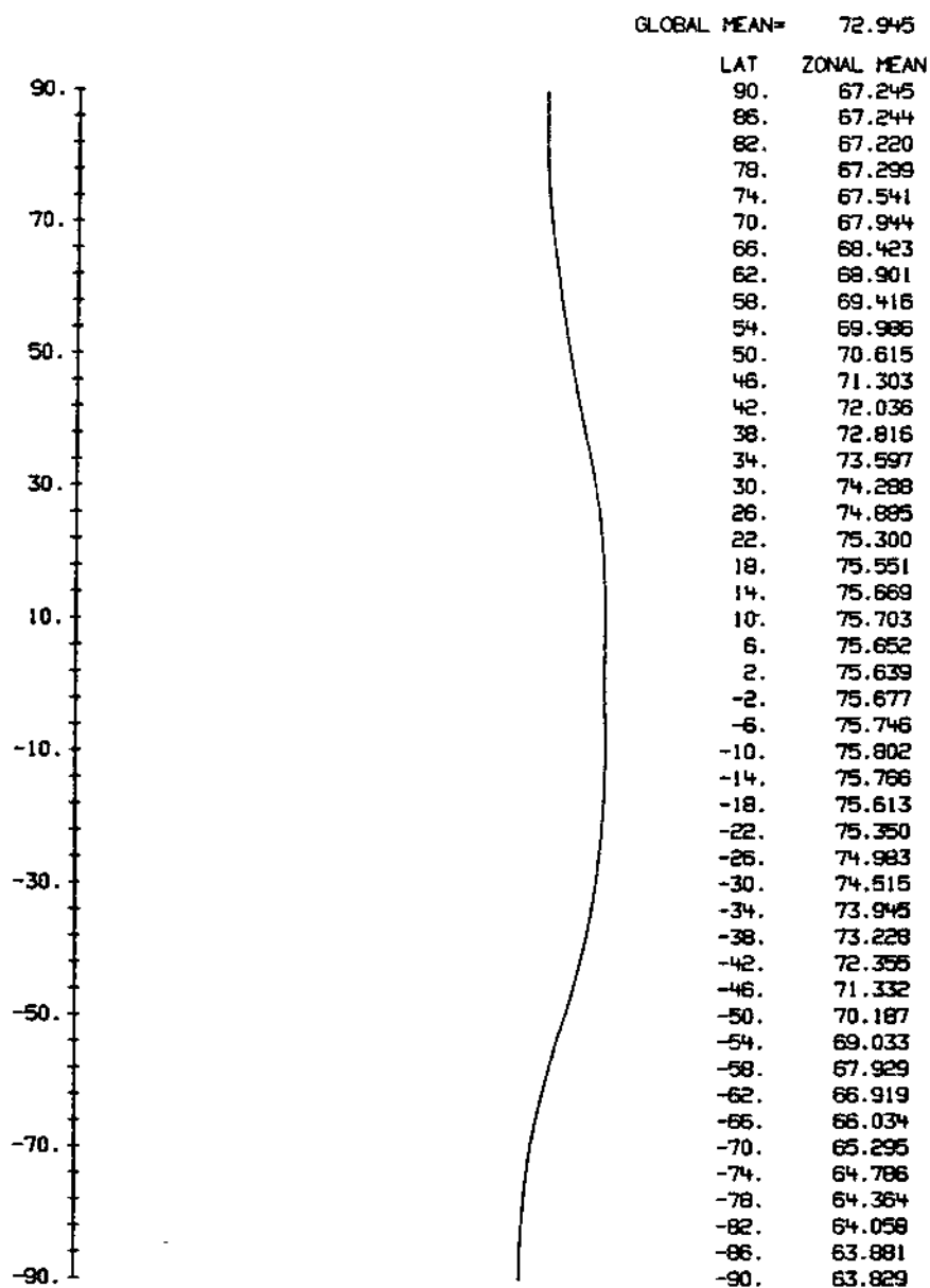
Fig. 4.20--April zonally averaged mean geopotential height at 400 mb in 10^2 m, as found from the data of Fig. 3.20.
