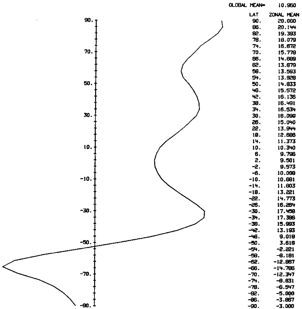
Fig. 4.1--April zonally averaged mean sea-level pressure in mb (relative to 1000 mb), as found from the data of Fig. 3.1.
