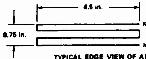
TYPICAL EDGE VIEW OF ALL THREE-CREASE FOILS. ALL FOLDS ARE SPACED EQUALLY WITH INSULATING SHEETS. (L3, L4, L5, AND L6)
