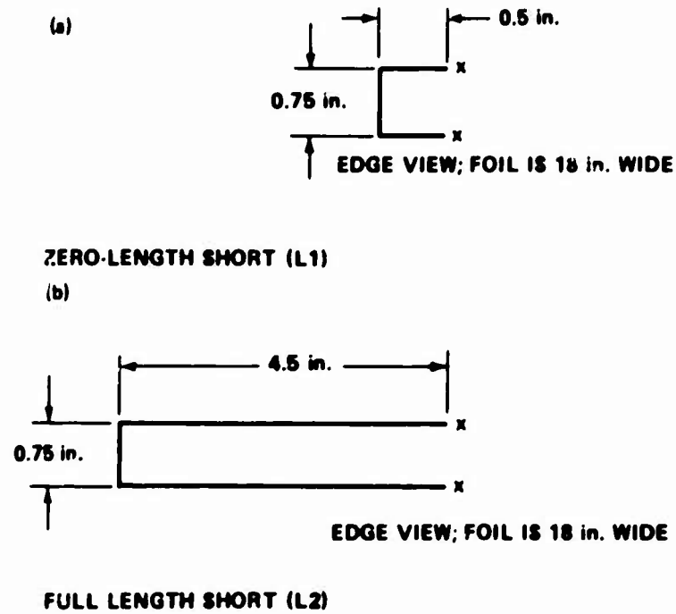
Figure 3. Baseline inductance foils.
