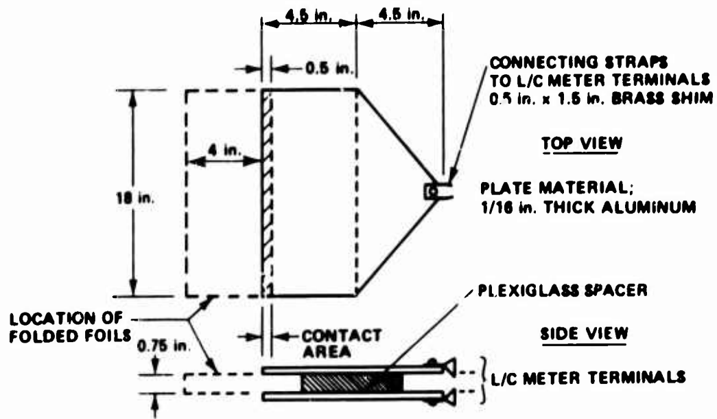
Figure 2. Low inductance test fixture.
