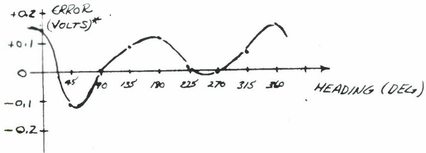
EAST COIL ERROR VS. HEADING.
