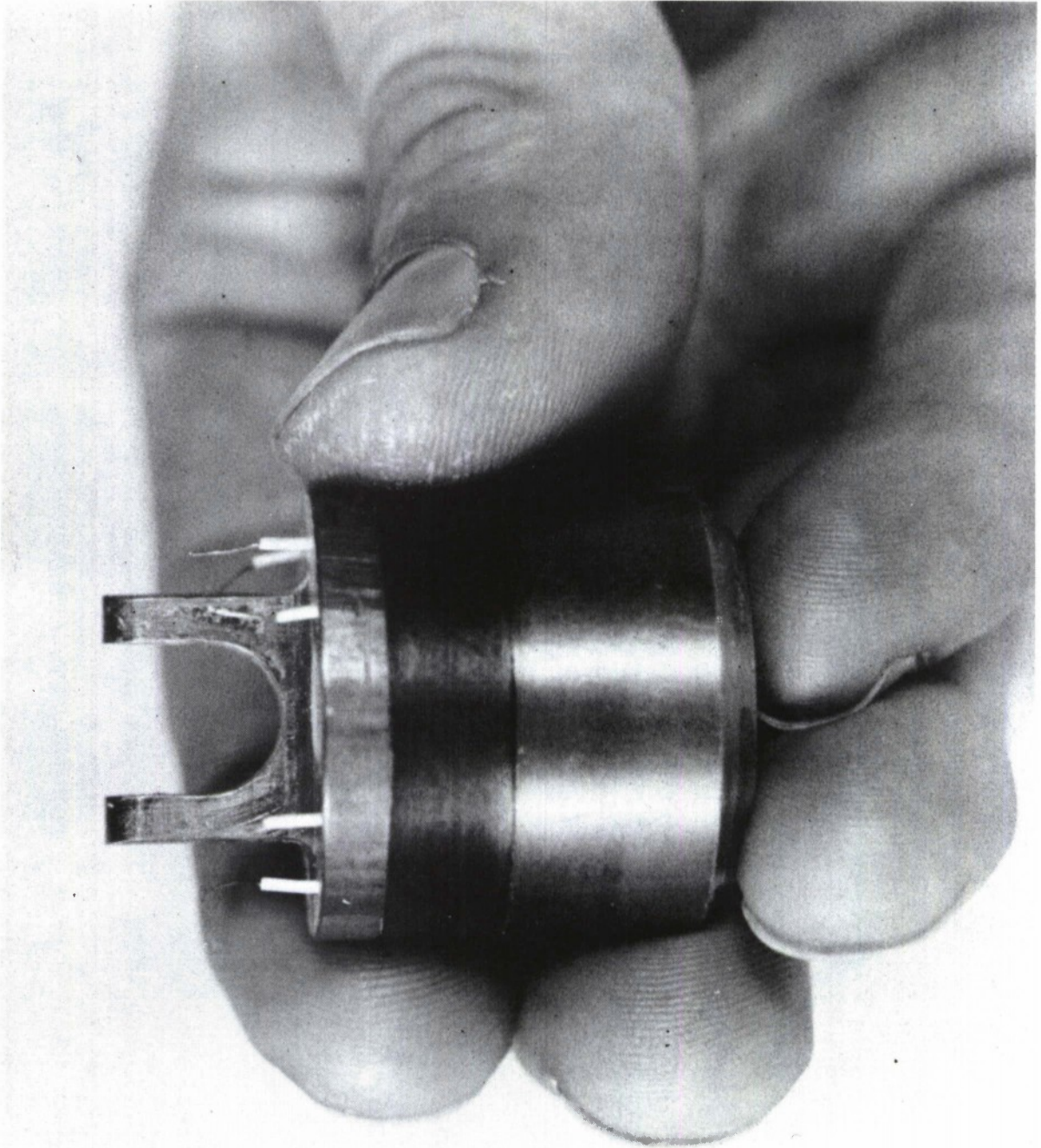
FIGURE 4-3 SENSOR ELEMENT
