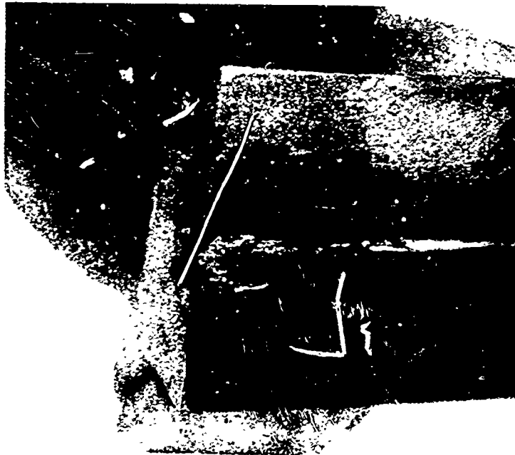
FIG. 12 Entrance of the C.G. 27 test bore after firing showing erosion and transferred gilding metal.
