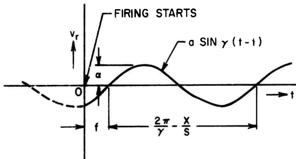
FIGURE 2. DISPLACEMENT OF REAR WHEEL BOTTOM.
