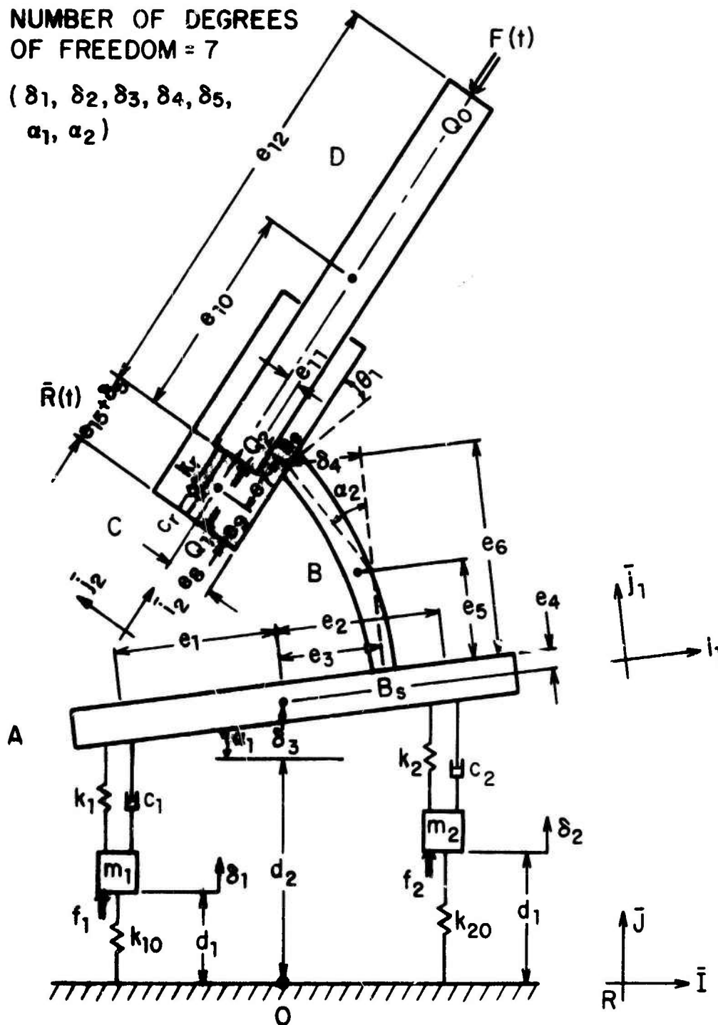
FIGURE 1. A MODEL OF WEAPON-VEHICLE SYSTEM.
