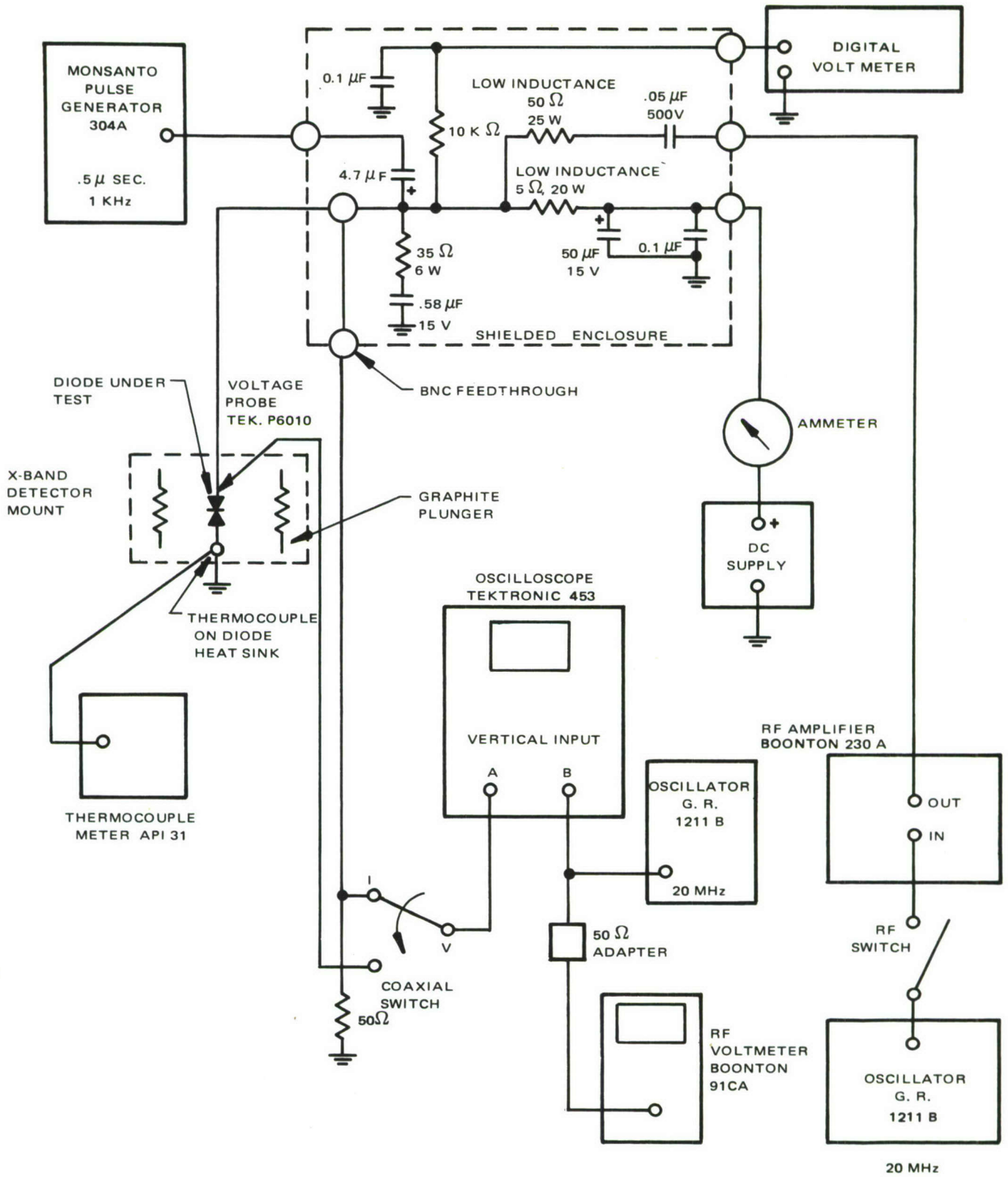
FIGURE 8 GUNN DIODE THERMAL RESISTANCE TEST SET
