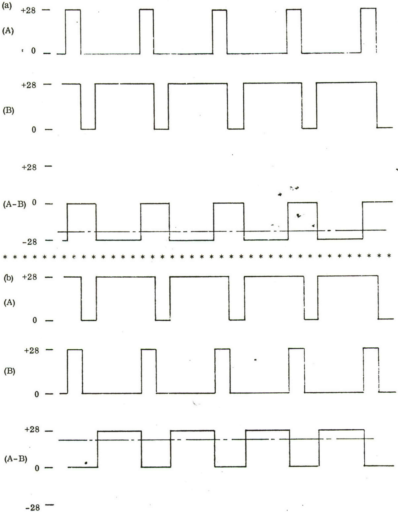
Figure A-3. Output Bridge Waveforms (illustrative only) A-10
