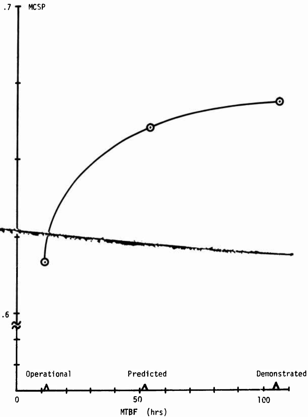
Figure 1. Mission Completion Success Probability as a Function of MTBF for the A-7D Forward Looking Radar.
