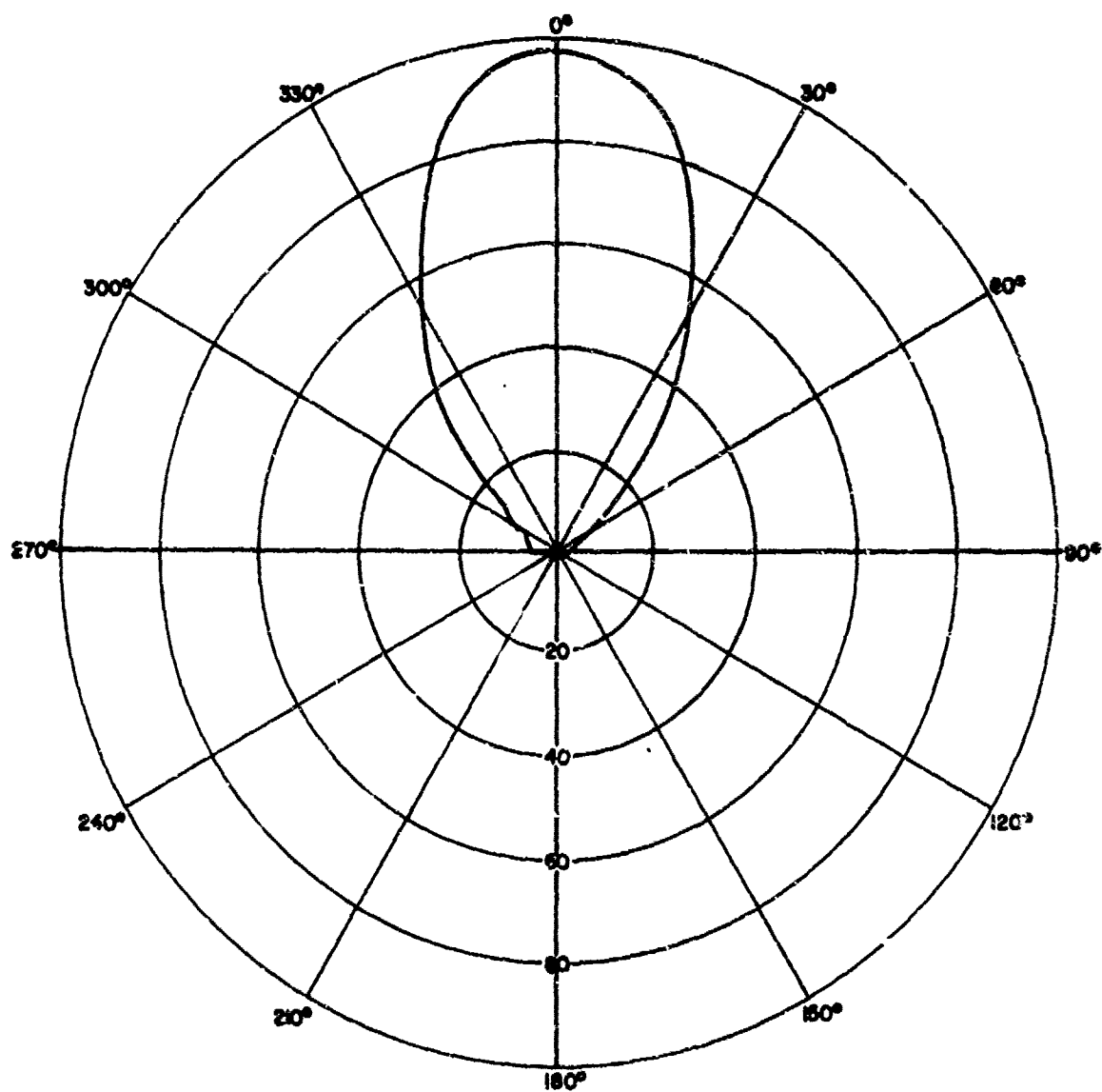
Fig. 50 RADIATION PATTERN OF APN-109B ANTENNA (H-PLANE, 700MHz)
