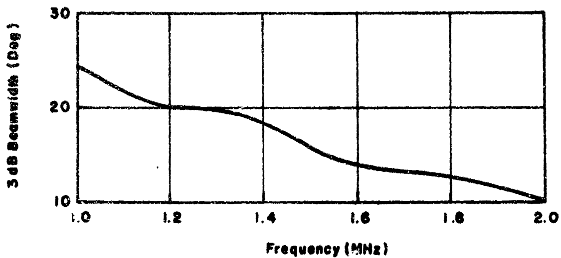
Fig. 54 BEAMWIDTH OF 4133-LI-N TOWER RECEIVING DISH ANTENNA
