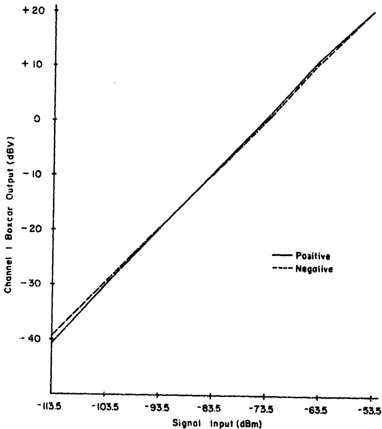
Fig 38 LINEARITY OF RECEIVER I-CHANNEL AT 923.1 MHz (IF DIAL SET AT 250)
