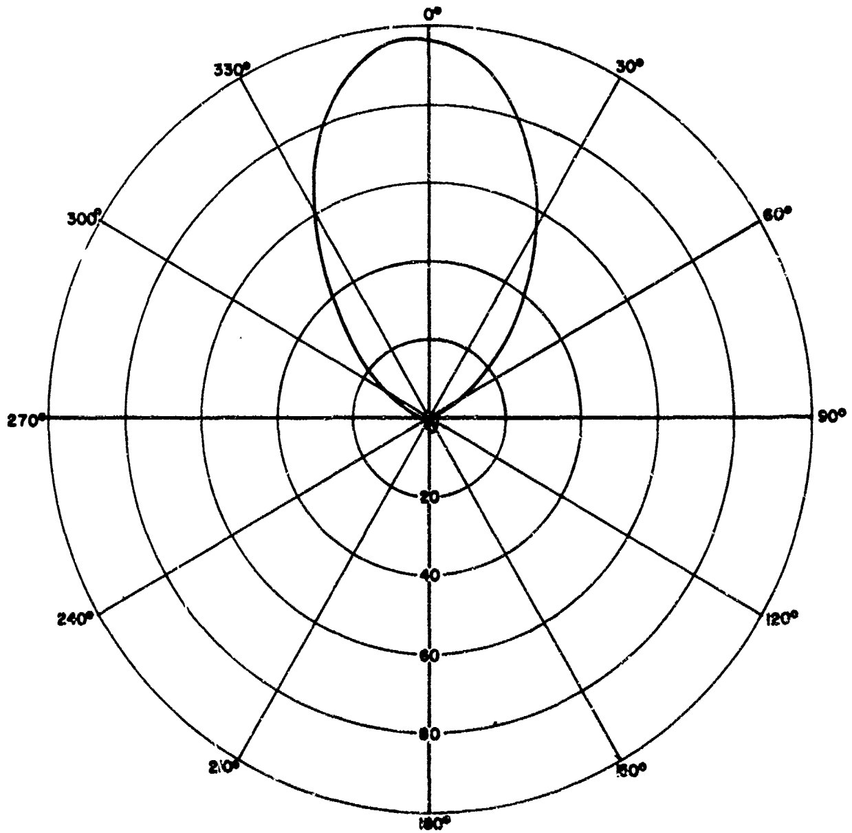
Fig. 43 RADIATION PATTERN OF APN-109B ANTENNA (E-PLANE, 200MHz)
