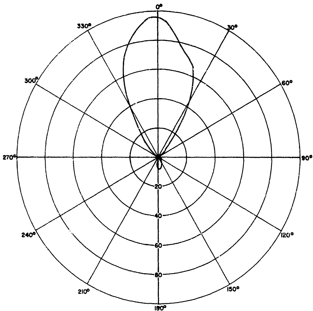
Fig.51 RADIATION PATTERN OF APN-109B ANTENNA (E-PLANE, 900MHz)
