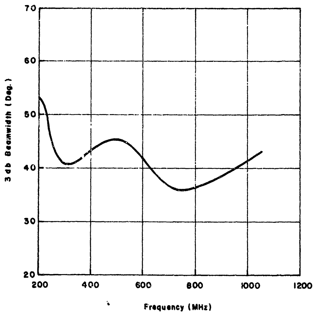
Fig.60 BEAMWIDTH OF 2305-LI-N GROUND TRANSMITTING ANTENNA
