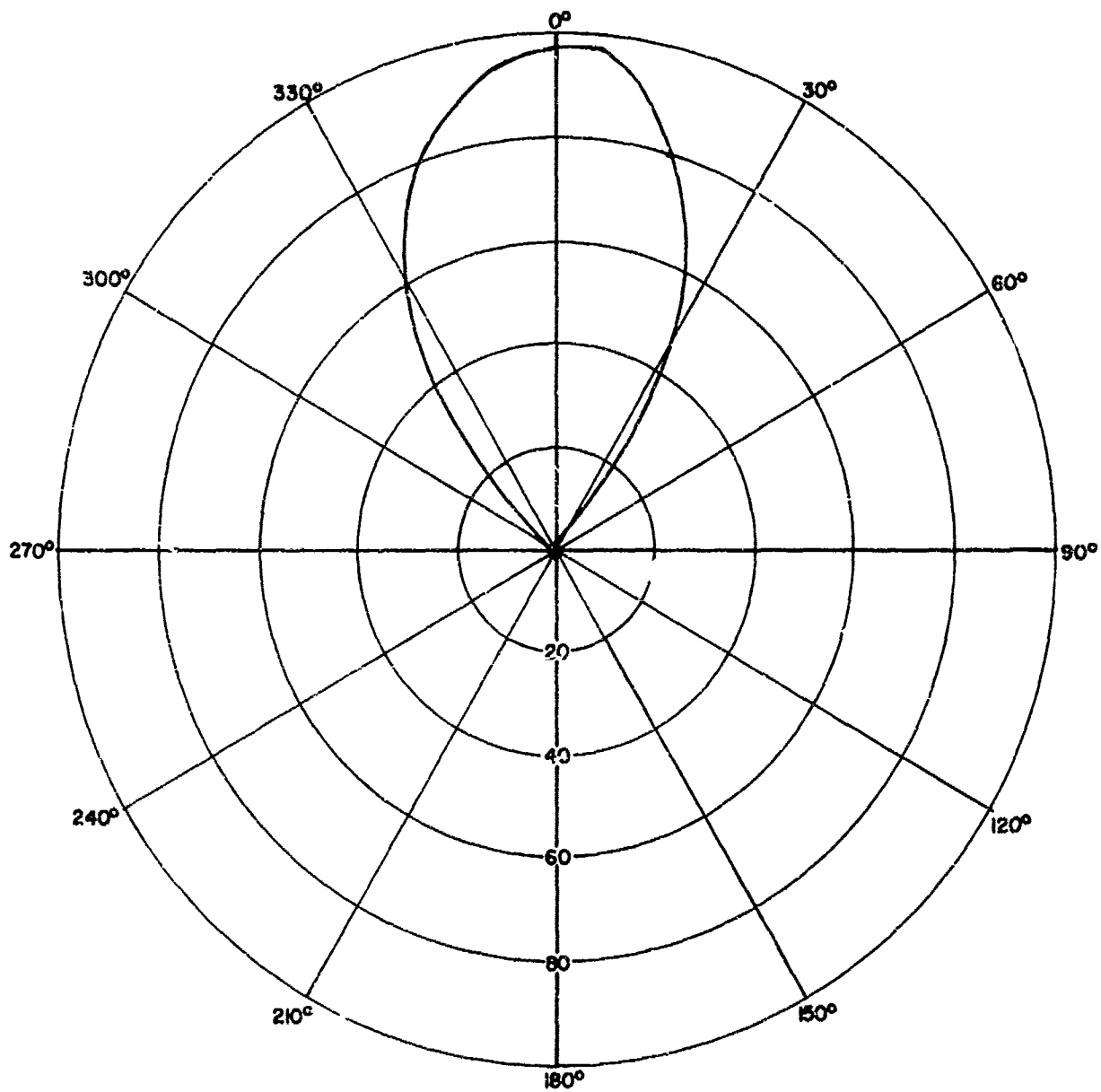
Fig.49 RADIATION PATTERN OF APN-109B ANTENNA (E-PLANE, 700MHz)
