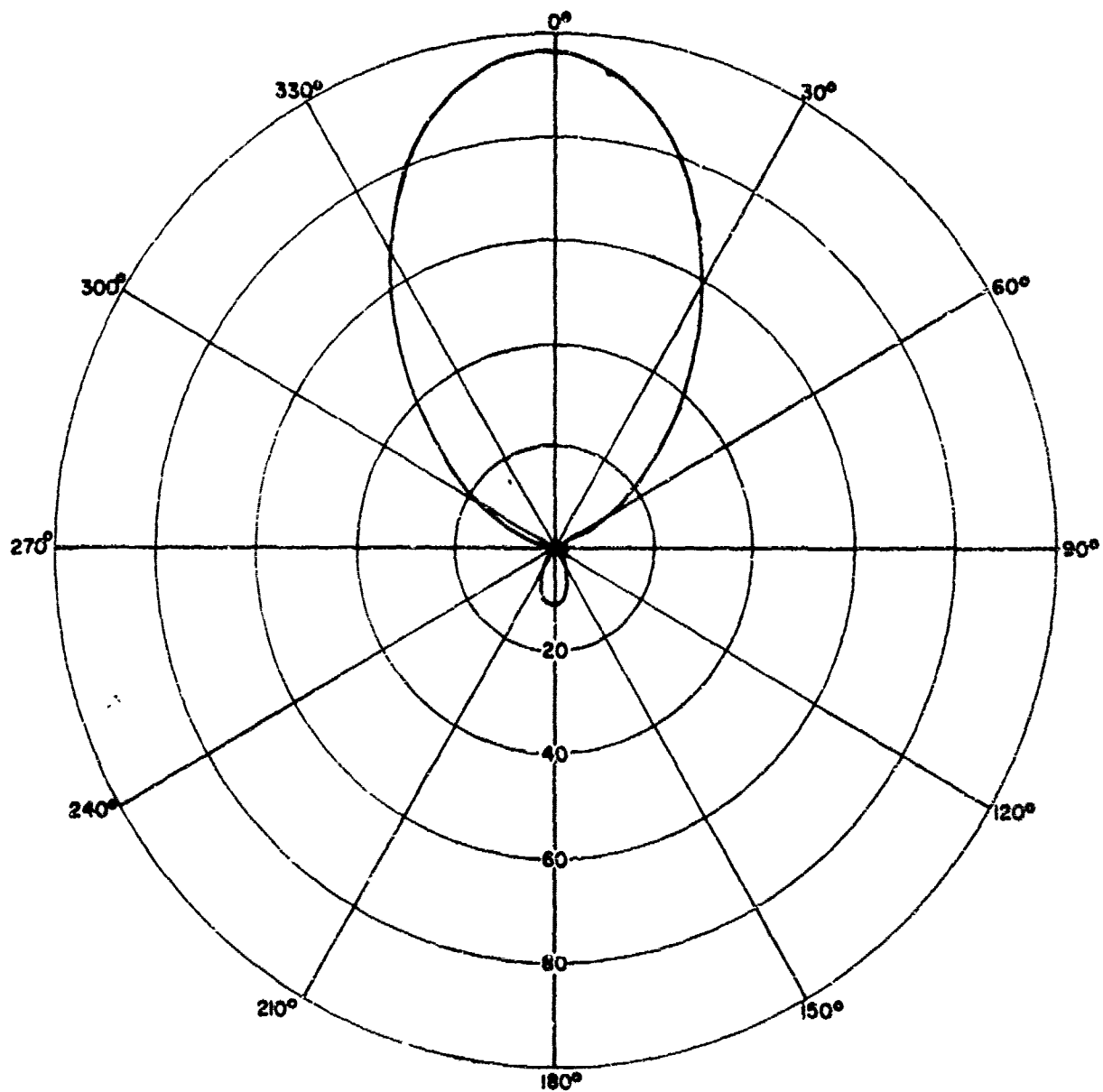
Fig 44 RADIATION PATTERN OF APN-109B ANTENNA (H-PLANE, 200 MHz)
