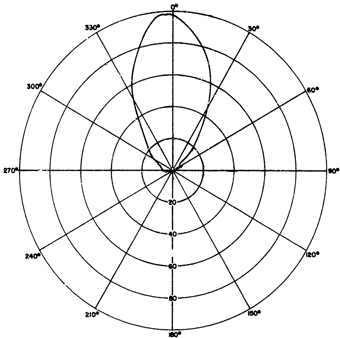
Fig.52 RADIATION PATTERN OF APN-109B ANTENNA (H-PLANE, 900MHZ)
