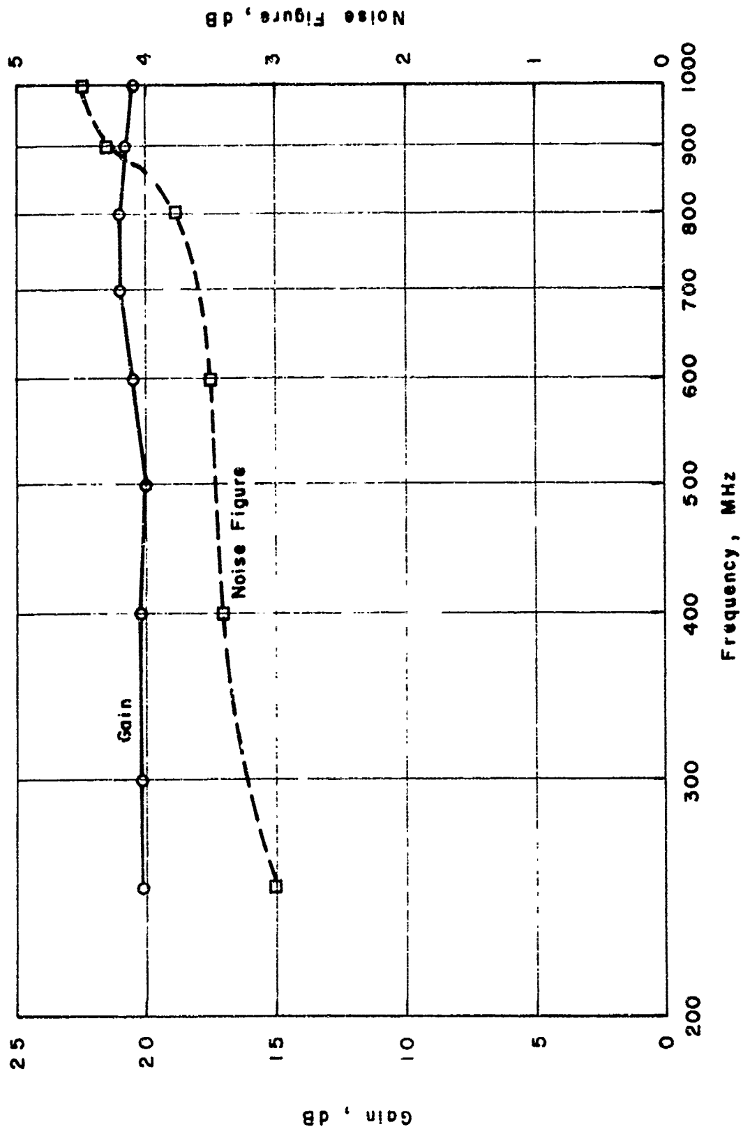
Fig. 32 PERFORMANCE OF 250-1000 MHz PRE-AMPLIFIER
