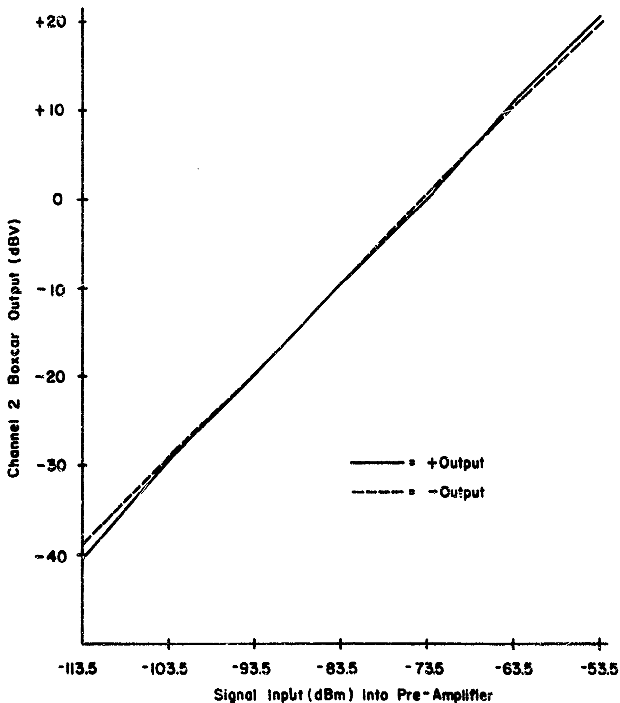
Fig 39 LINEARITY OF RECEIVER Q-CHANNEL AT 923.1 MHz (IF DIAL SET AT 250)
