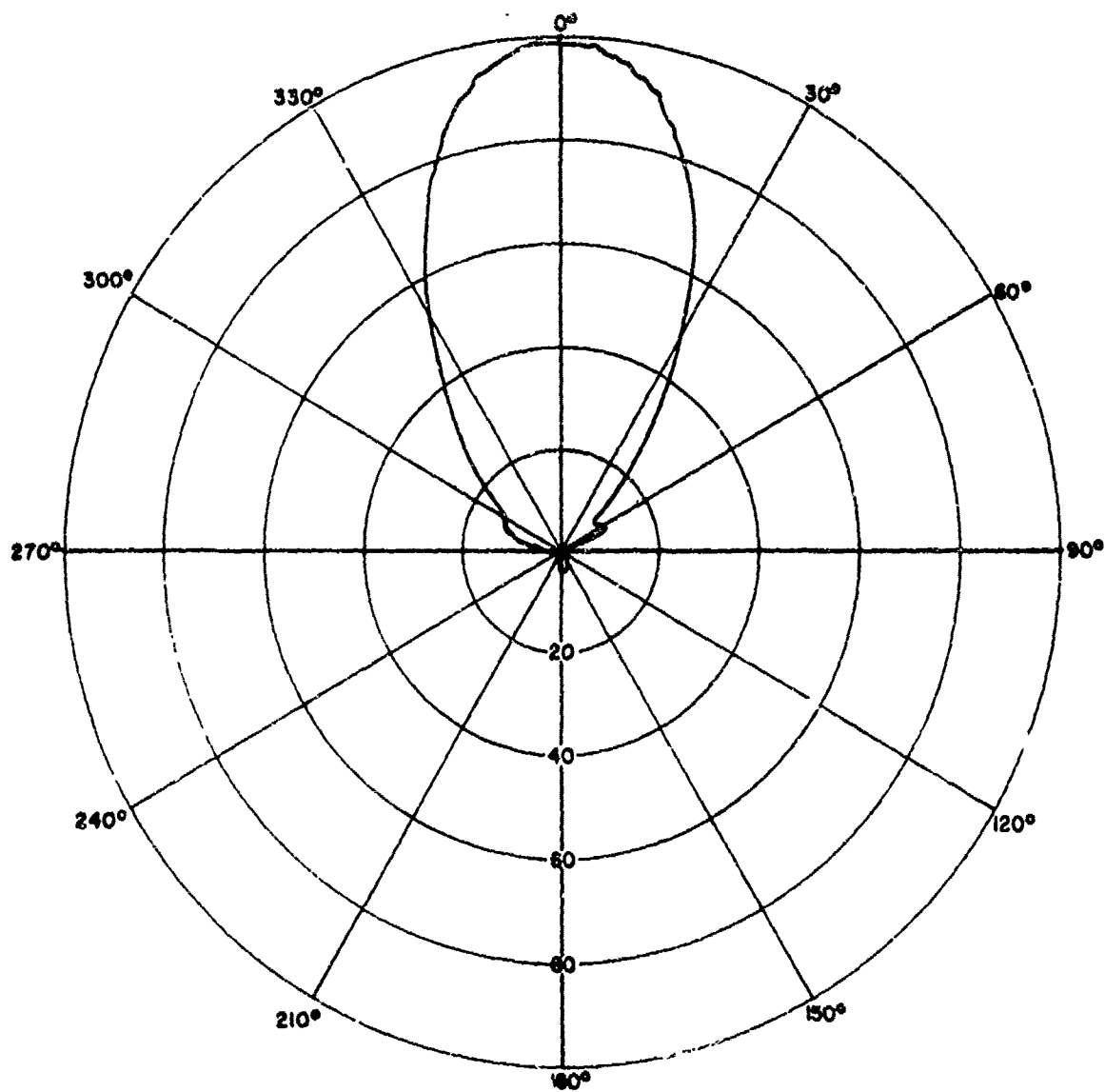
Fig. 48 RADIATION PATTERN OF APN-109B ANTENNA (H-PLANE, 500MHz)
