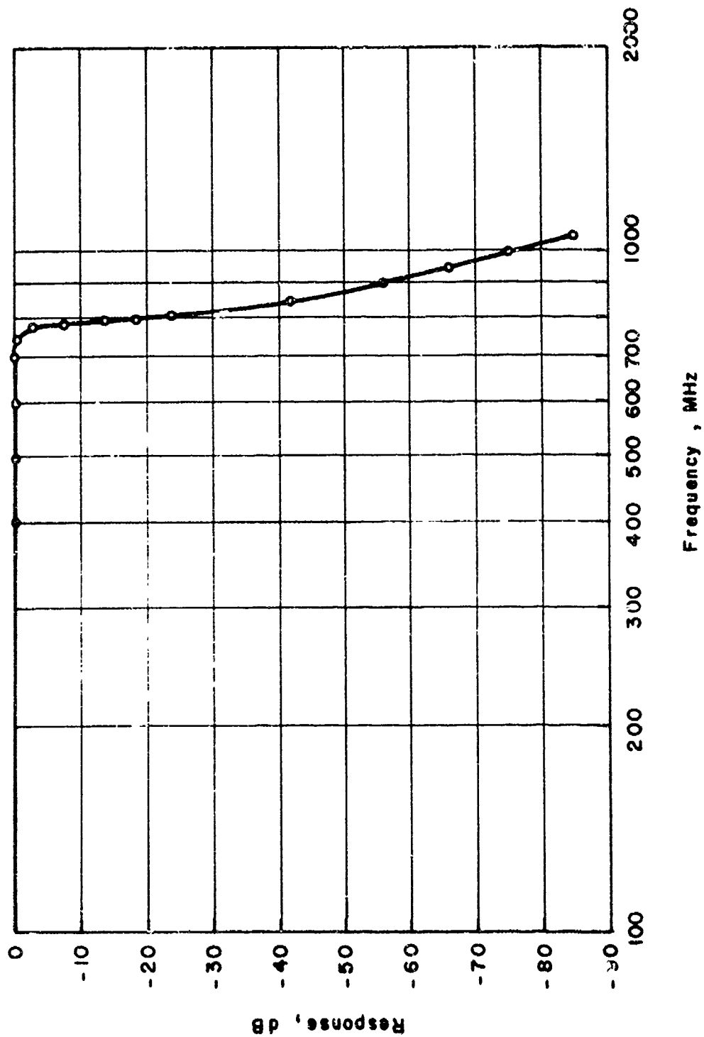
Fig. 36 RESPONSE OF TLC 750-7EE1 FILTER
