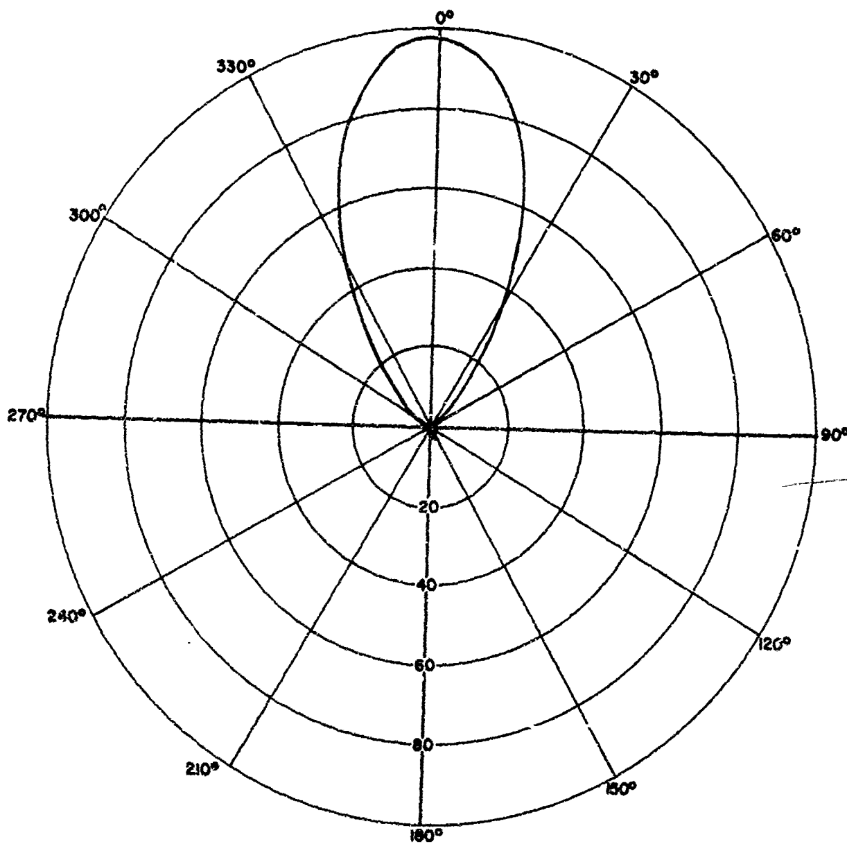
Fig.45 RADIATION PATTERN OF APN-109B ANTENNA (E-PLANE, 300MHz)
