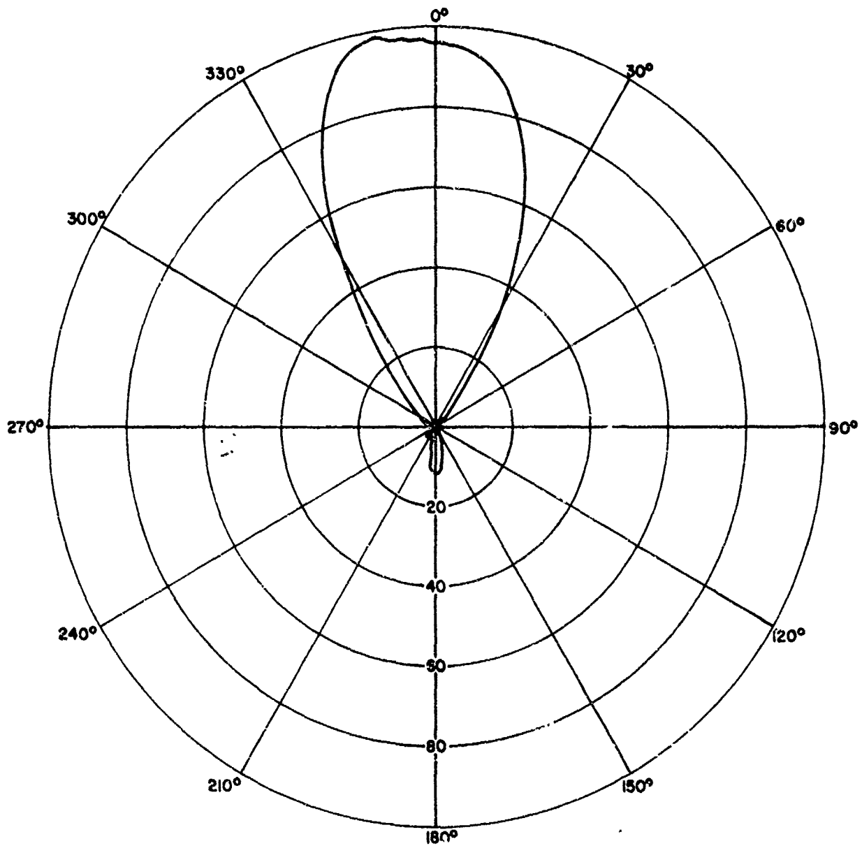
Fig. 47 RADIATION PATTERN OF APN-109B ANTENNA (E-PLANE, 500MHz)
