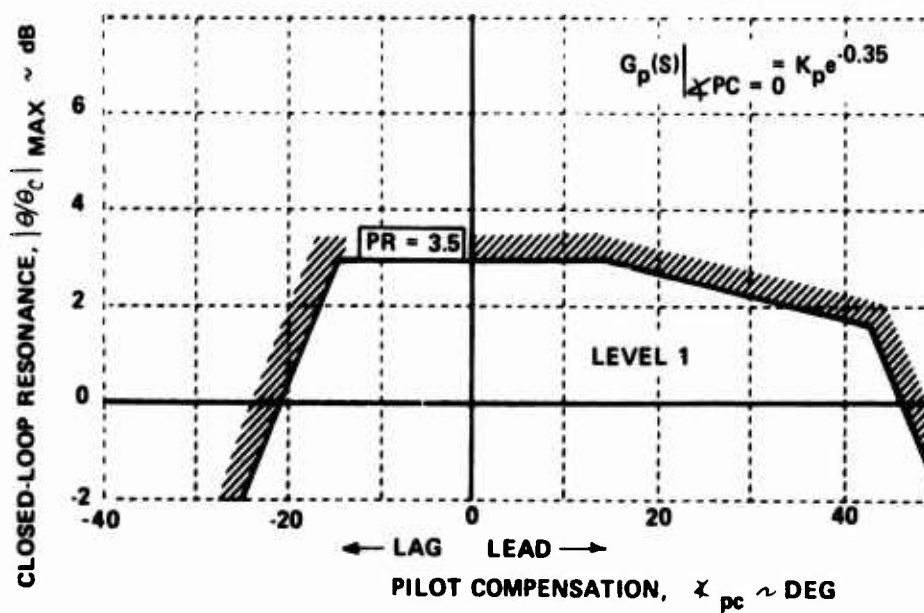
Figure 40b NEAL-SMITH PERFORMANCE CRITERION (REF. 1)
