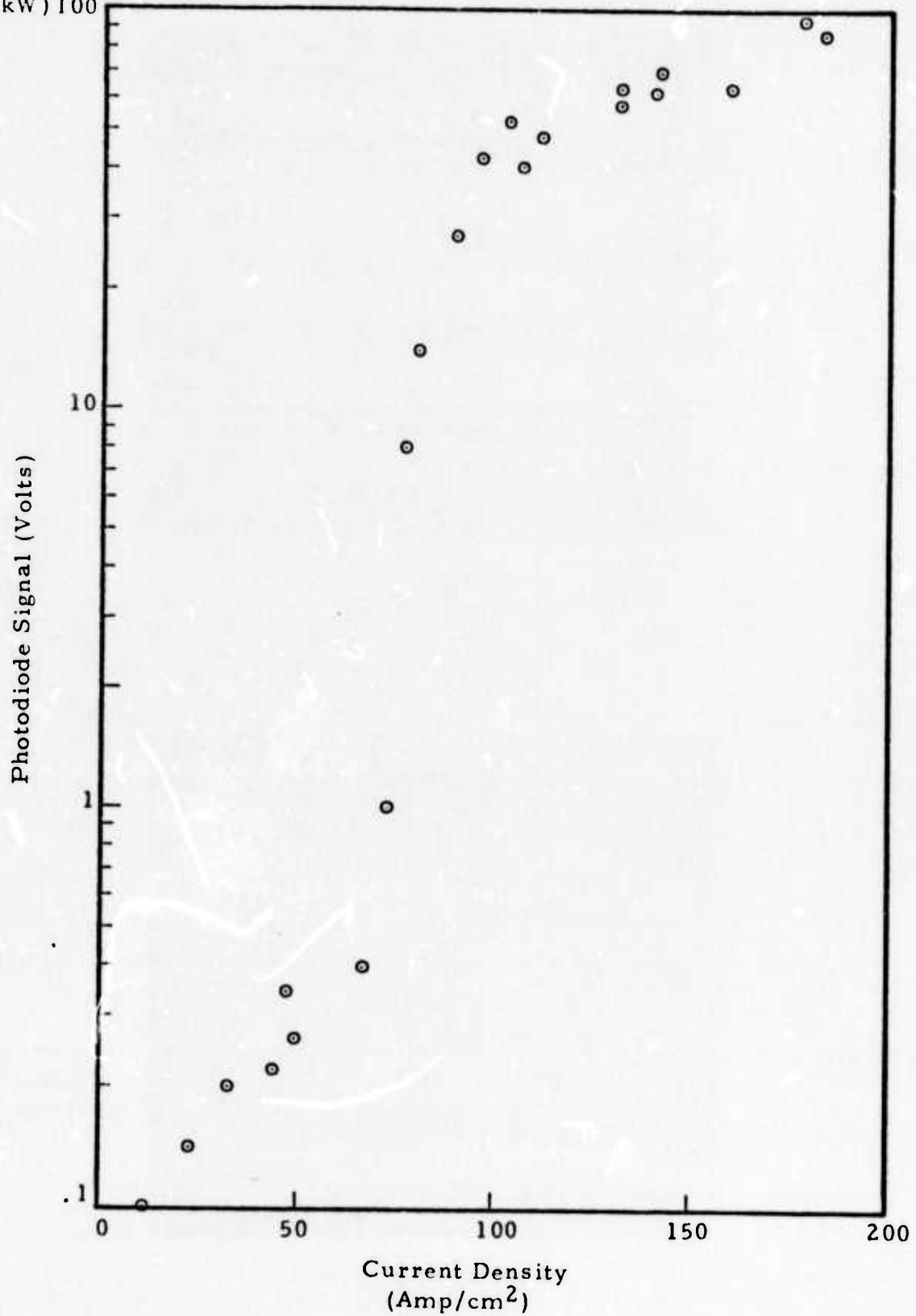
Figure 5. Peak photodiode voltage as a function of excitation current density showing laser threshold in a mixture of 92 psia Ar + 8 psia N 2 .
