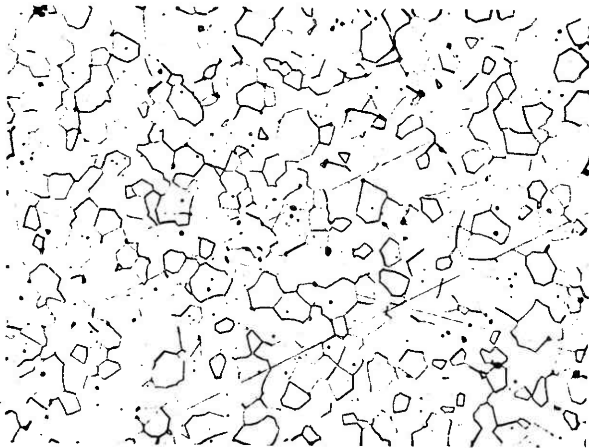
Fig. 13 Microstructure of standard Lucalox alumina test material (average surface grain size of 30 to 40 microns); (etchant- \text{H}_3\text{PO}_4 , 10 minutes). [Overetching of grain boundaries has occurred in (b).]
