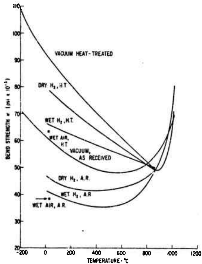
Fig. 9 Comparison of bend strengths of as-received and annealed single-crystal sapphire.
