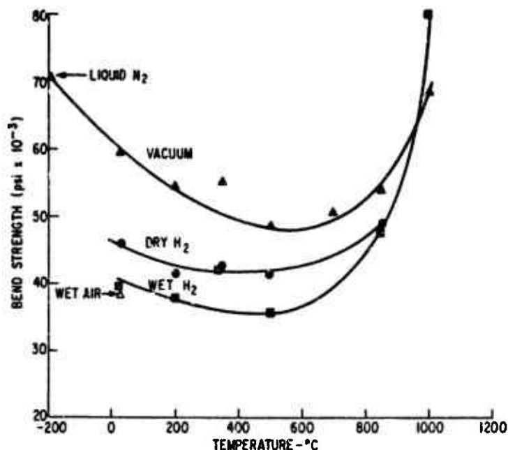
Fig. 7 Temperature-atmosphere effects on the bend strength of as-received single-crystal sapphire.
