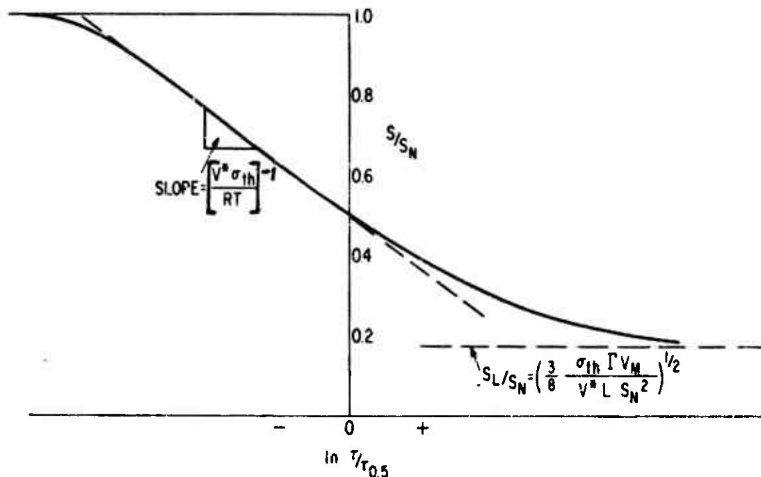
Fig. 18 Schematic fatigue curve (after Charles and Hillig, Ref. 25), where \tau is time-to-failure and \tau_{0.5} is the time-to-failure for a stress S_N/2 .
