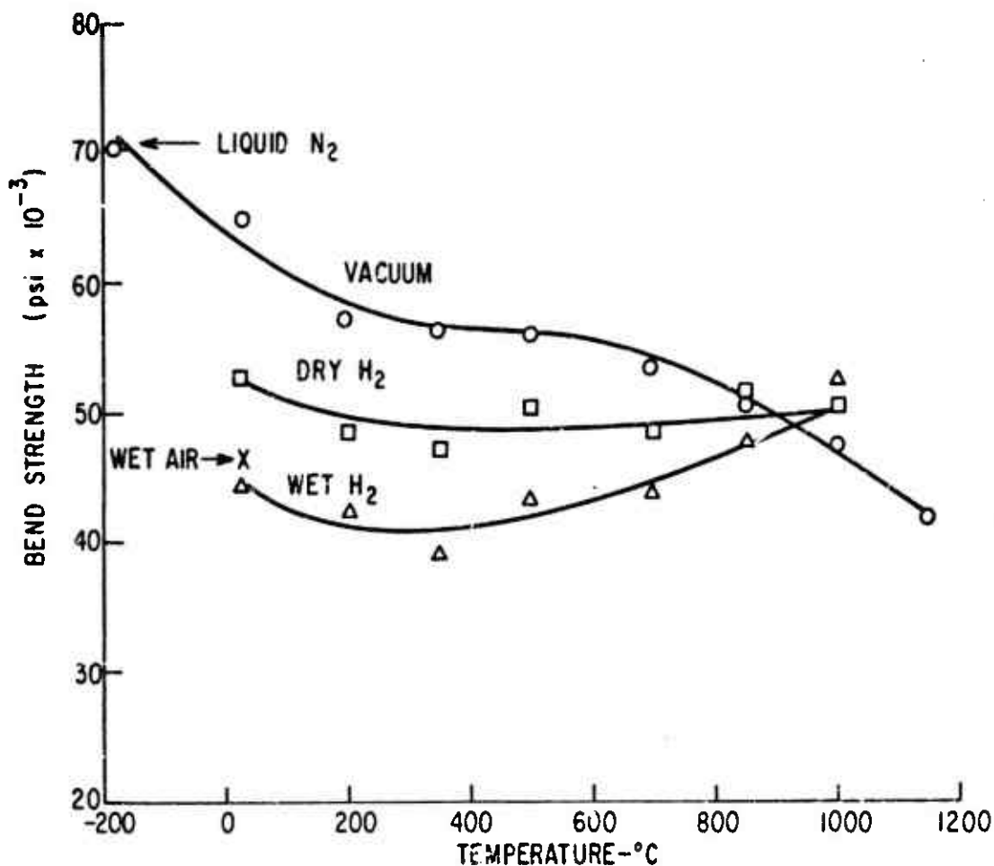
Fig. 15 Temperature-atmosphere effects on the bend strength of standard Lucalox alumina specimens.
