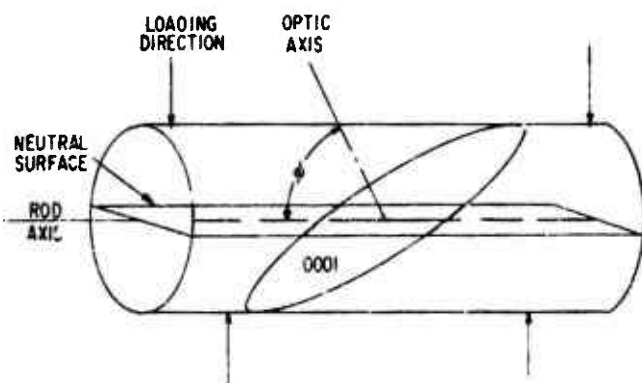
Fig. 1 Load geometry for sapphire single crystals.
