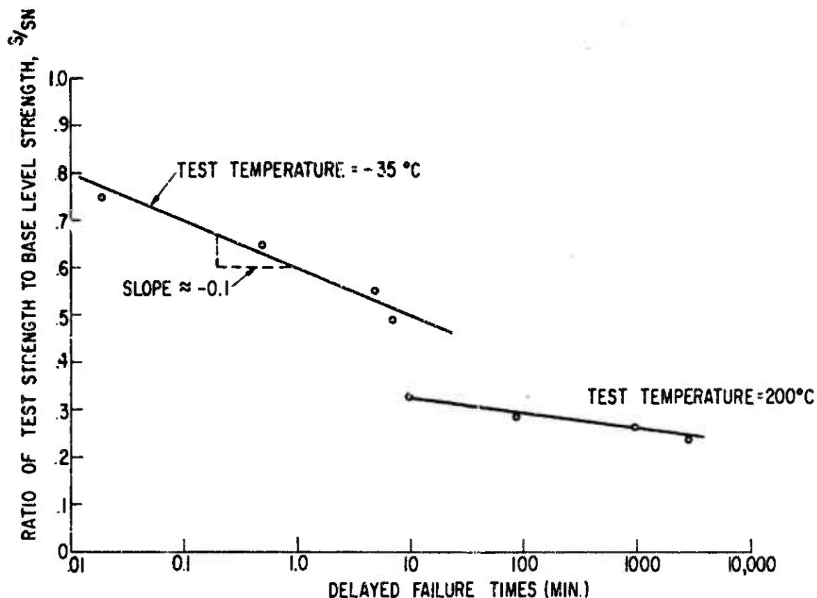
Fig. 11. Static fatigue curve for single-crystal sapphire.
