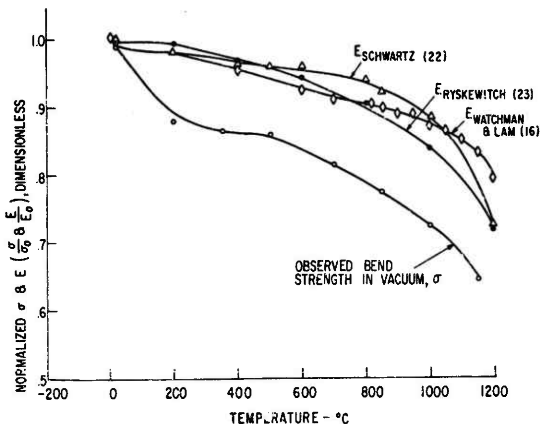
Fig. 16 Lucalox alumina vacuum bend strength and Young's modulus vs temperature.
