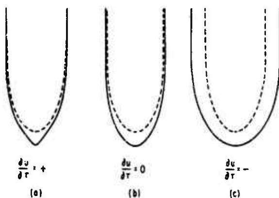
Fig. 17 Hypothetical changes in flaw geometry due to corrosion or dissolution: (a) flaw sharpening as a result of stress corrosion; (b) flaw growth such that the rounding of the tip by stress corrosion balances the lengthening of the flaw; (c) flaw rounding by corrosion or dissolution (Joffe effect). (After Charles and Hillig, Ref. 25.)
