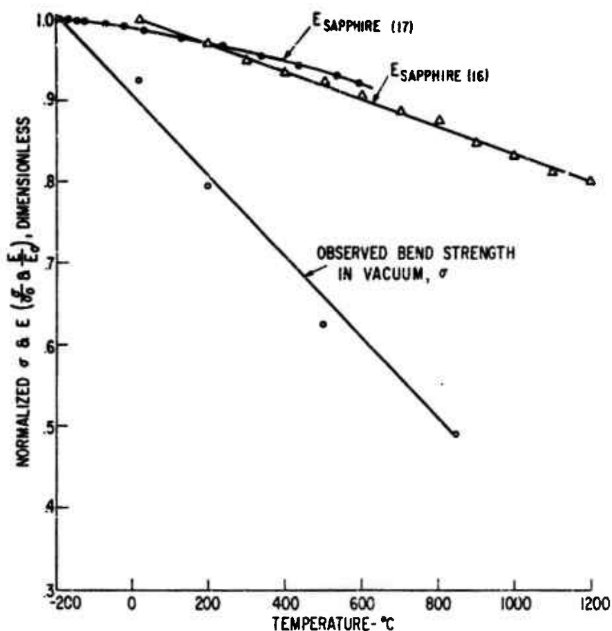
Fig. 10 Annealed sapphire single-crystal bend strength and Young's modulus vs temperature.
