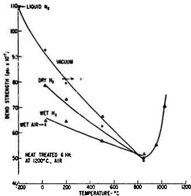
Fig. 8 Temperature-atmosphere effects on the bend strength of heat-treated single-crystal sapphire.
