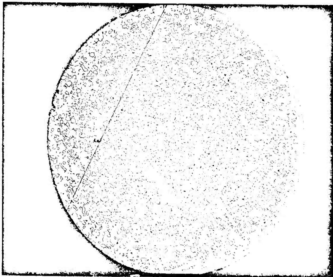
Fig. 13 Microstructure of standard Lucalox alumina test material (average surface grain size of 30 to 40 microns); (etchant- \text{H}_3\text{PO}_4 , 10 minutes). [Overetching of grain boundaries has occurred in (b).]
