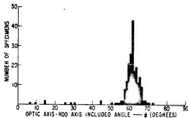
Fig. 2 Optic axis orientations for sapphire test specimens.
