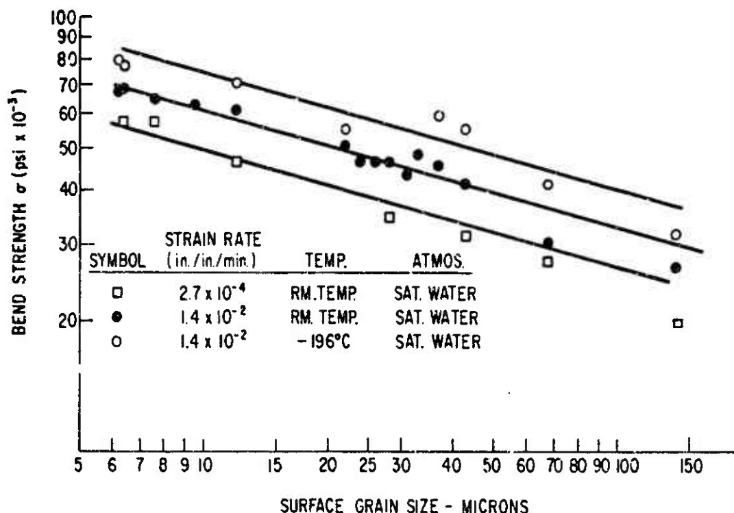
Fig. 14 Effect of surface grain size, loading rate, and temperature on the bend strength of Lucalox alumina.
