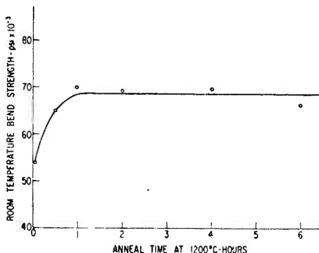
Fig. 6 Effect of anneal time at 1200°C on bend strength of sapphire single crystals.
