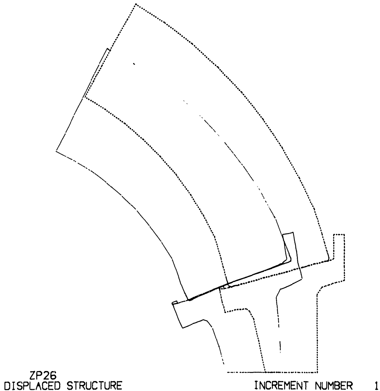
Figure B.7. Radial displacements of window and flange in Configuration A under external hydrostatic loading: problem 110, glass on steel.
