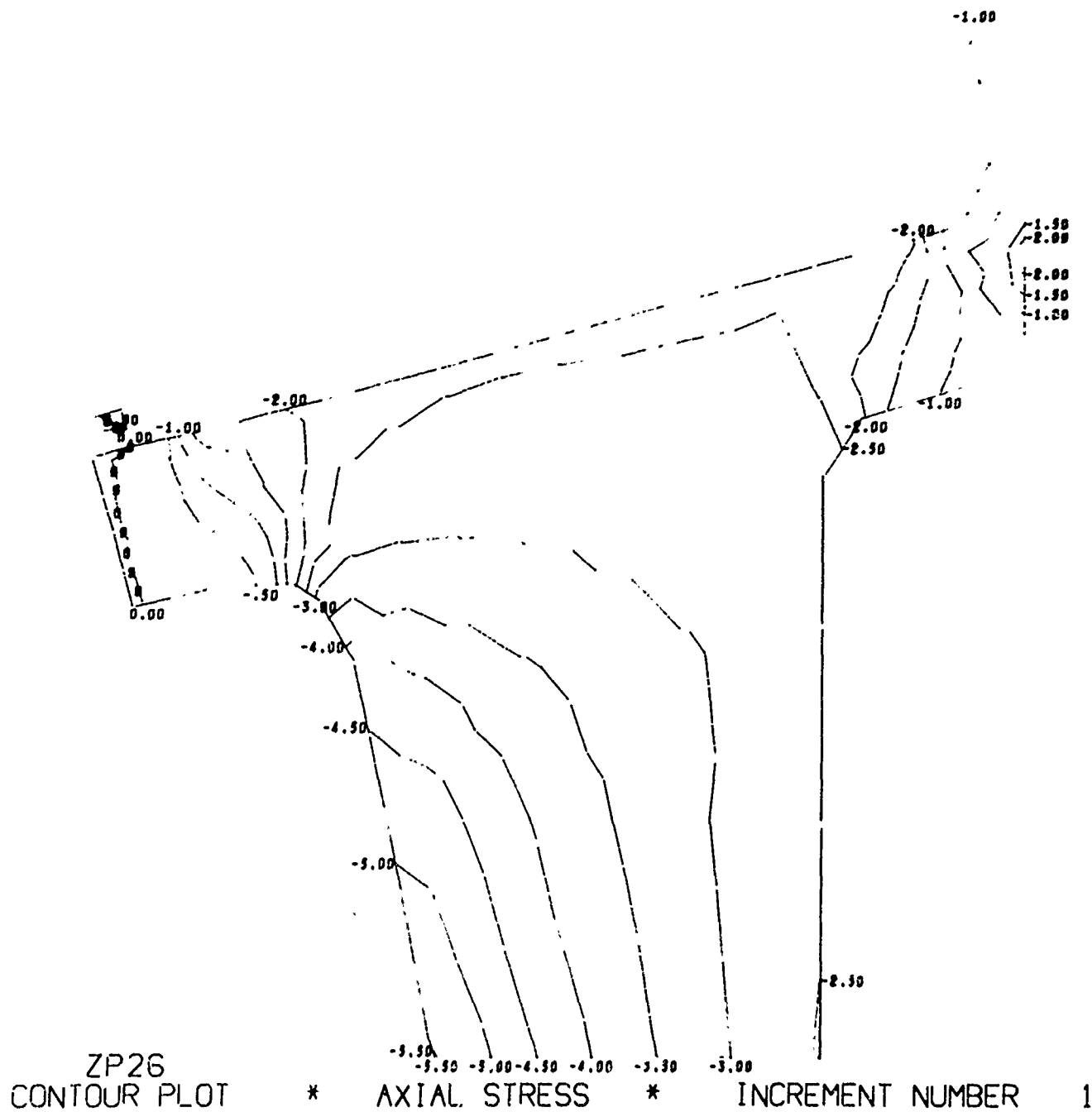
Figure B.5. Magnitude and distribution of stresses in window-flange assembly Configuration A utilizing a steel flange, fiber-reinforced-epoxy gasket, and glass ceramic window (problem 102).(sheet 7 of 7)
