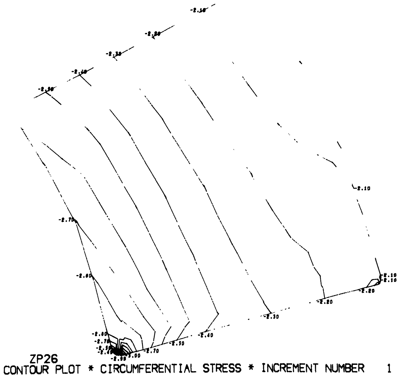
Figure B.9. Magnitude and distribution of stress in window-flange assembly Configuration B utilizing an aluminum flange, fiber-reinforced-epoxy gasket, and glass ceramic window (problem 203). (sheet 6 of 8)
