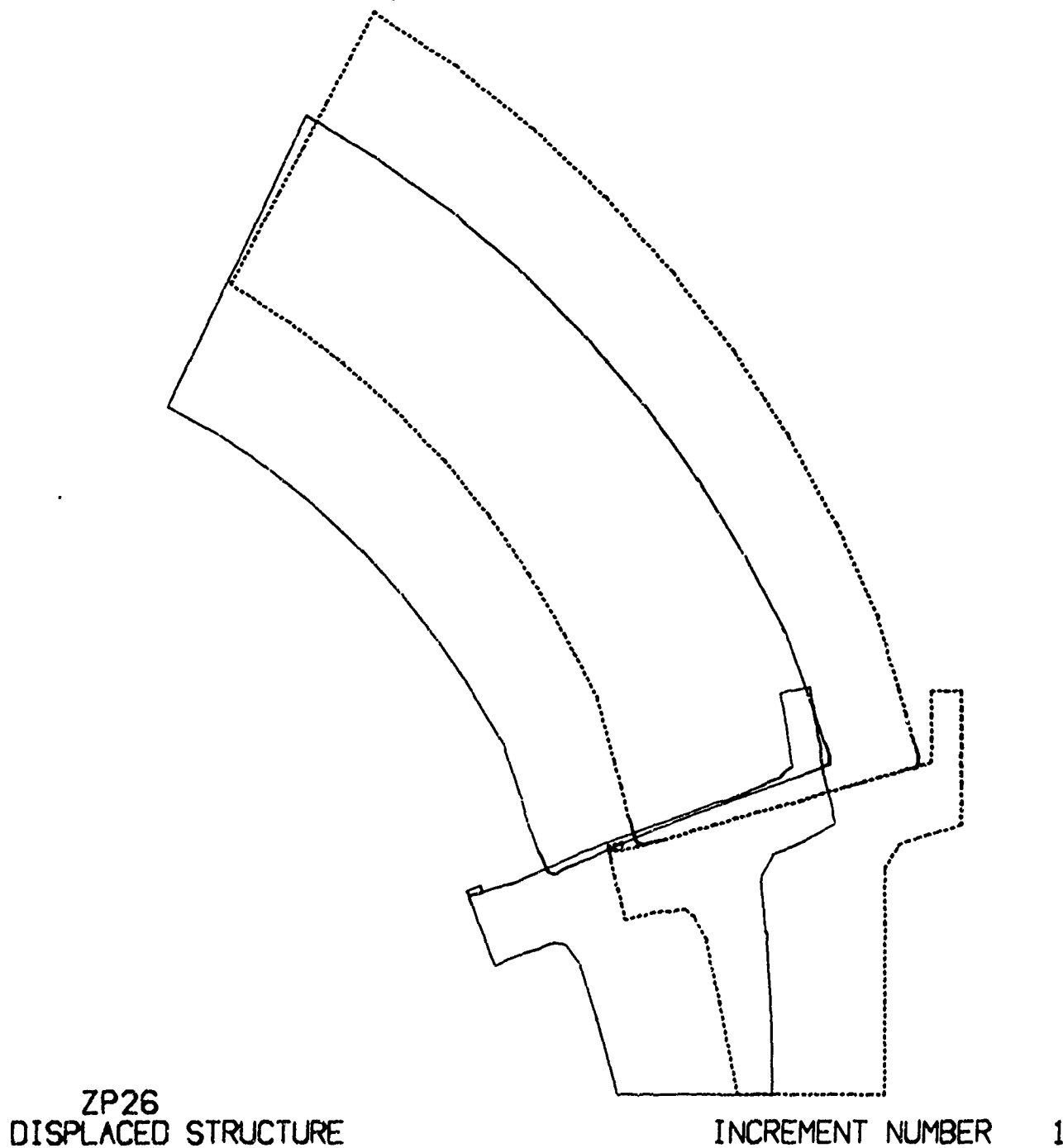
Figure E.9. Calculated displacements of Cer-Vit C-101 window and Monel K-500 flange.
