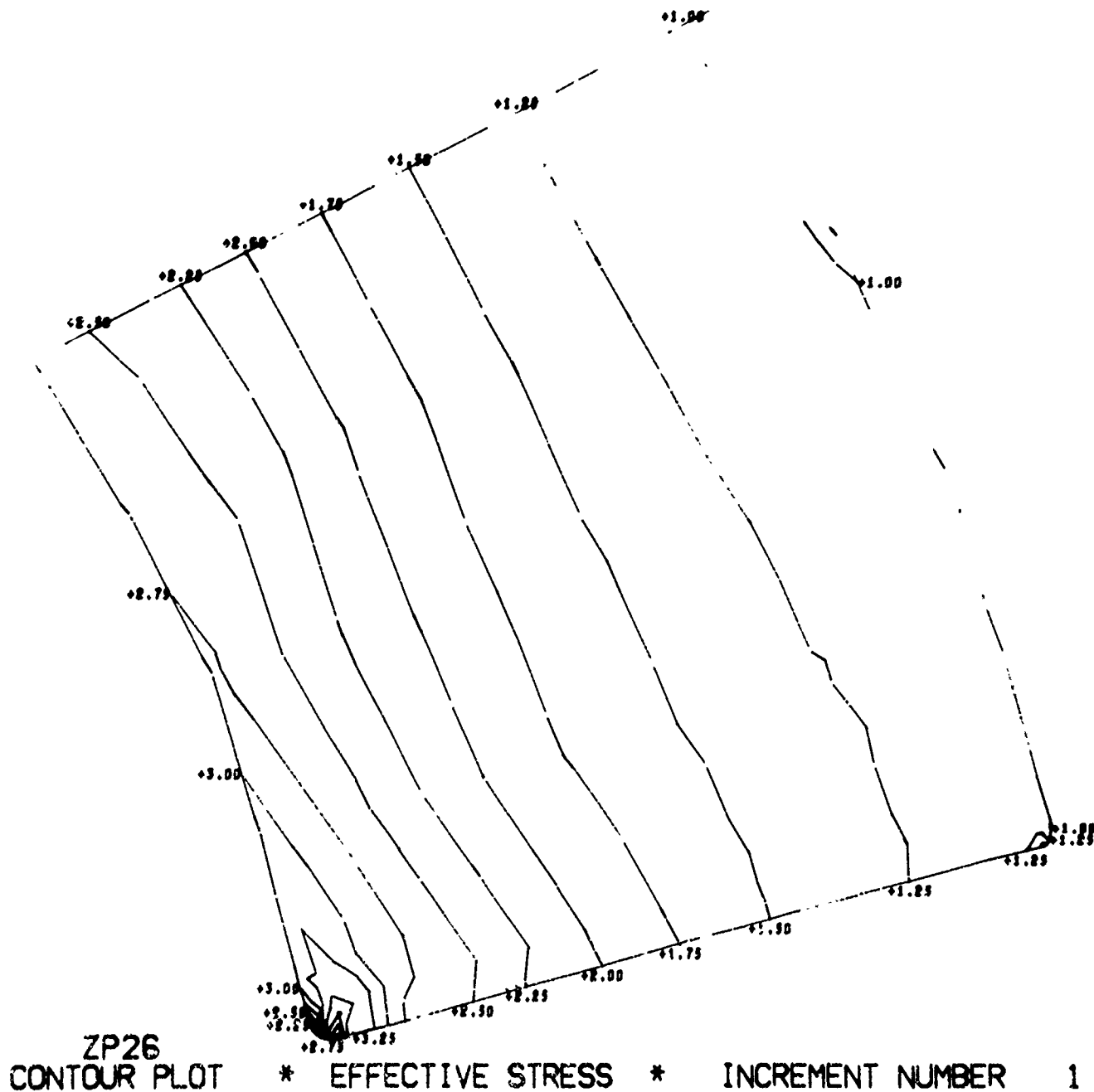
Figure B.8. Magnitude and distribution of stresses in window-flange assembly Configuration E, utilizing a glass-reinforced-plastic flange and glass ceramic window (problem 204). (sheet 2 of 8)
