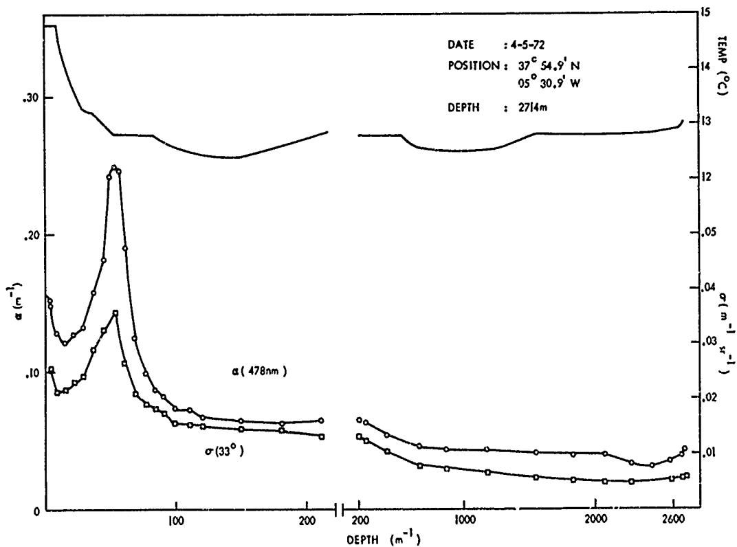
FIG. 30 OPTICAL ATTENUATION, OPTICAL SCATTERING, AND TEMPERATURE PROFILES OF DROP I-8.
