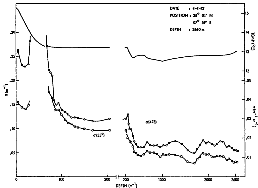
FIG. 29 OPTICAL ATTENUATION, OPTICAL SCATTERING, AND TEMPERATURE PROFILES OF DROP I-7.
