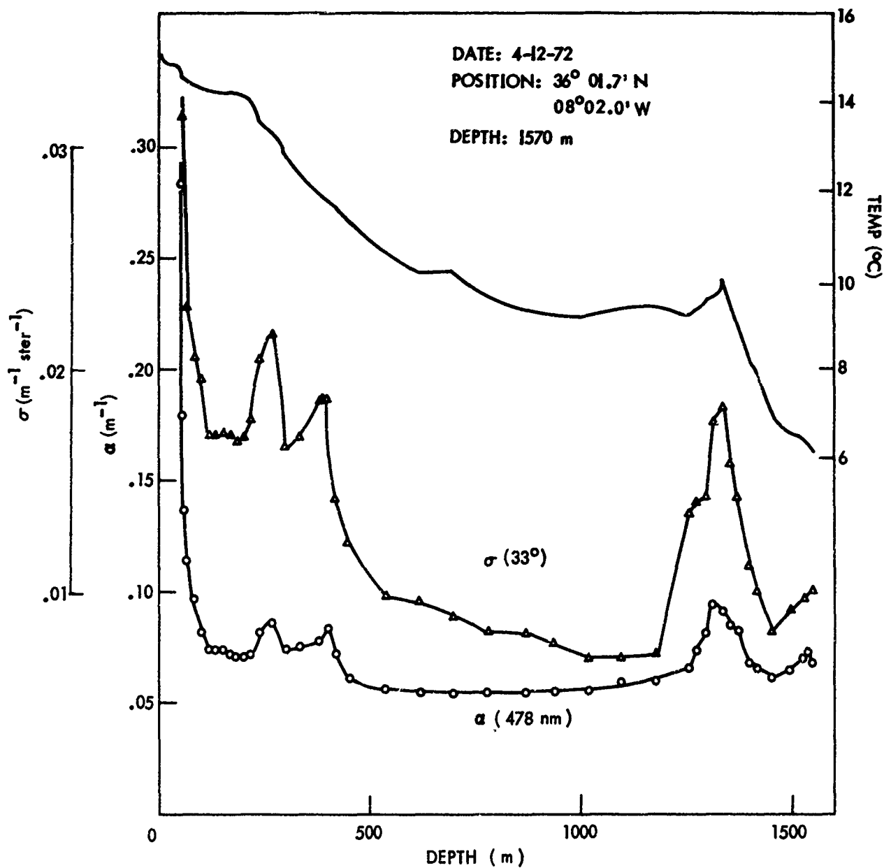
FIG. 35 OPTICAL ATTENUATION, OPTICAL SCATTERING, AND TEMPERATURE PROFILES OF DROP I-13.
