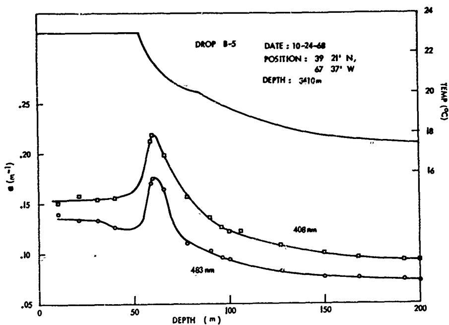
FIG. 6 OPTICAL ATTENUATION AND TEMPERATURE PROFILES FROM DROP B-5.
